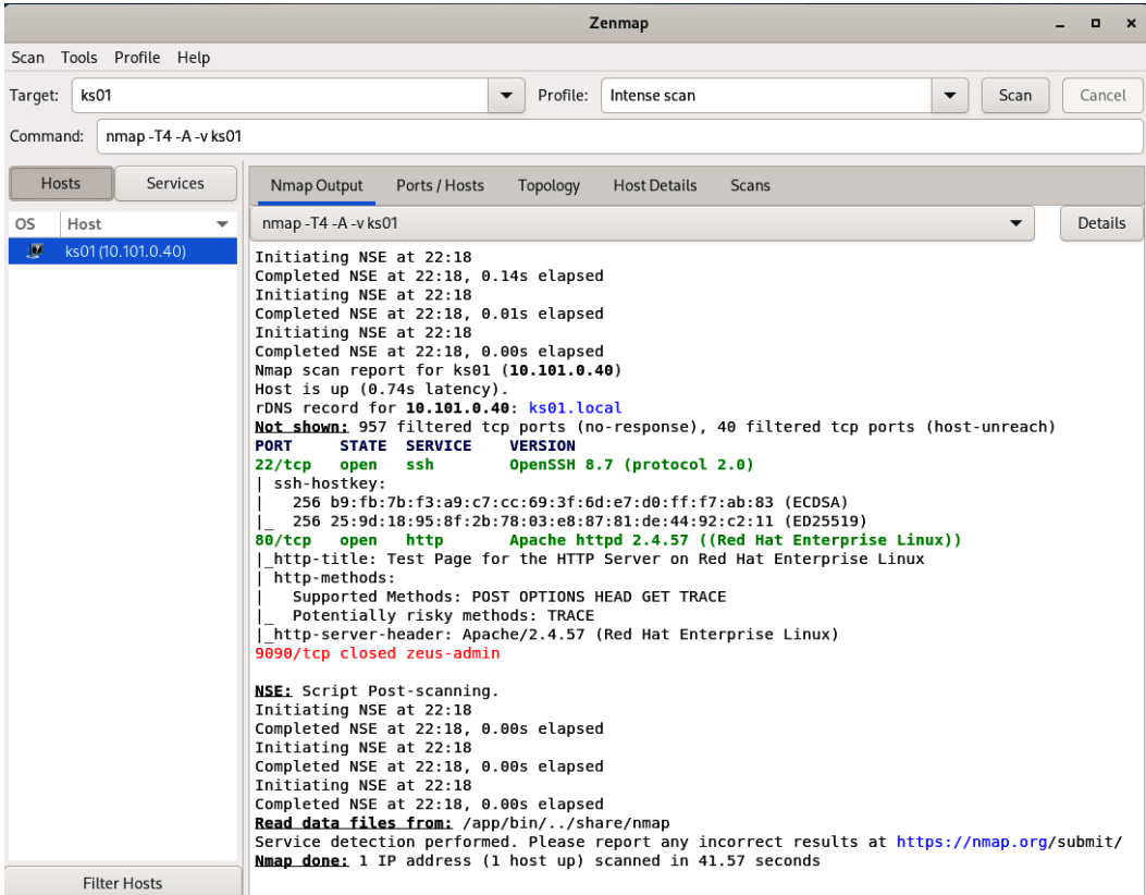
Figure 5.3 – Zenmap scan
