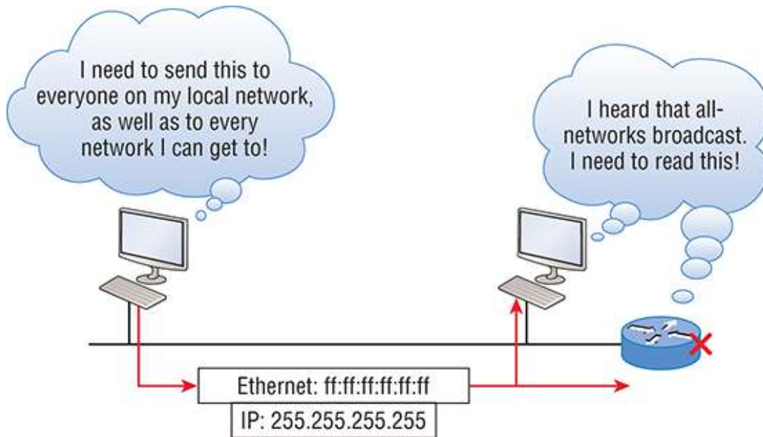
FIGURE 3.22 Layer-3 broadcasts.
