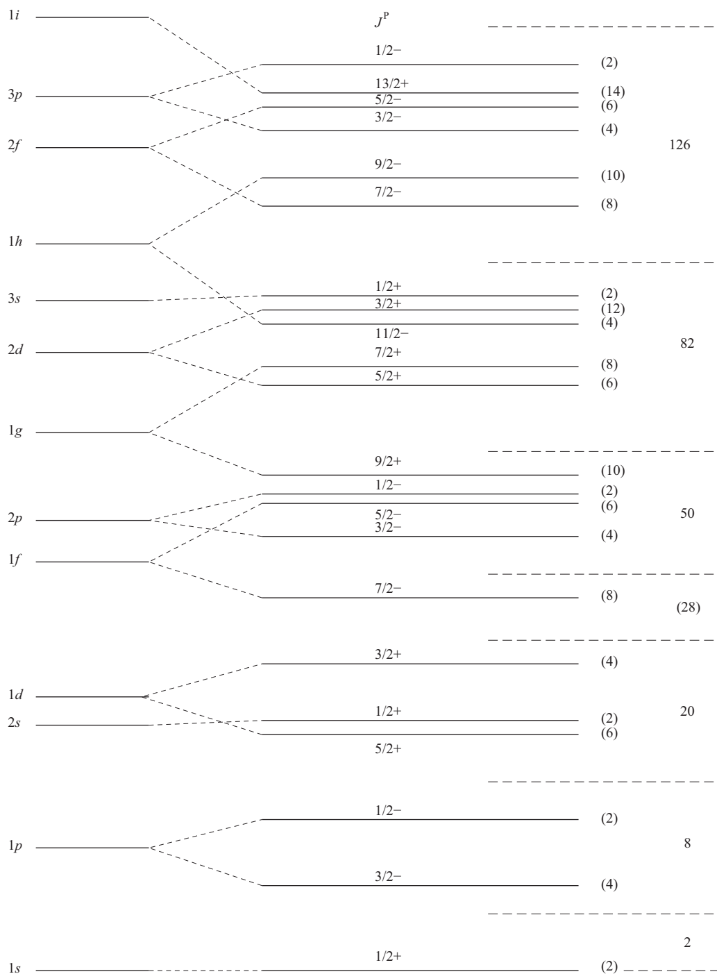
Figure 16.11 Energy levels of nucleons in an atomic nucleus according to the shell model. On the left are the values of (n/l) and in the center those of J^P ( P = parity). The dotted lines separate the layers. The penultimate column shows the number of neutrons or protons that fit into each subshell, and the column to the right shows the magic numbers predicted by this theory, which coincide with those found empirically (28 is sometimes considered “semimagic”).
