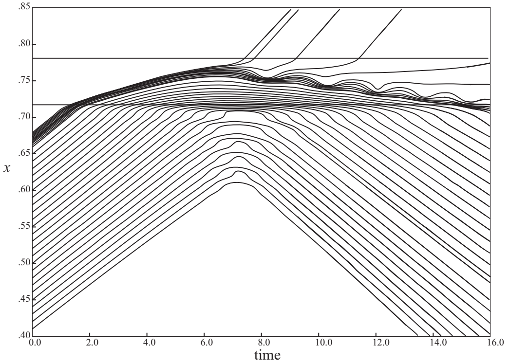
Figure 5.8 A collimated, monochromatic beam of particles scattered by a barrier, according to Bohm's theory (see Section 10.1). Note that many particles are scattered before reaching the barrier. Figure adapted from Dewdney and Hiley (1982).
