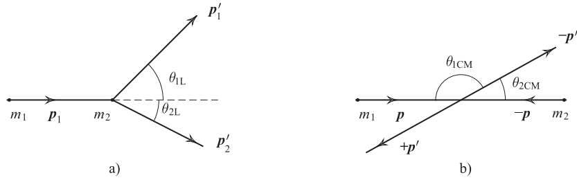
Figure 18.1 Diagram of an elastic collision between particles 1 and 2, seen from (a) the laboratory frame, (b) the CM frame.
