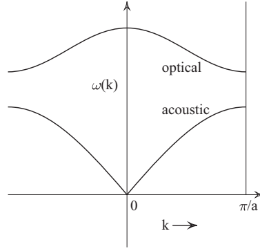
Figure 15.2 Phonon dispersion curves of a linear diatomic chain with two different types of atoms, showing an optical branch (upper curve) in addition to the acoustic branch (lower curve). The vertical axis is the energy or frequency of the phonon and the horizontal axis is the wave vector k .
