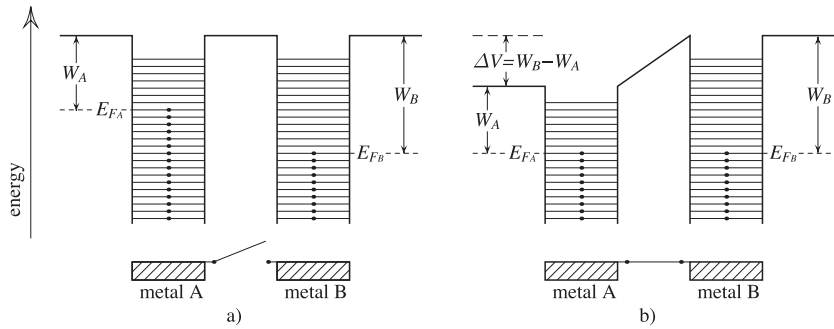
Figure 6.9 (a) Metals A and B having different work functions W_A , W_B . (b) The metals are brought into electrical contact. Tunneling occurs from A to B until the Fermi levels are equalized.
