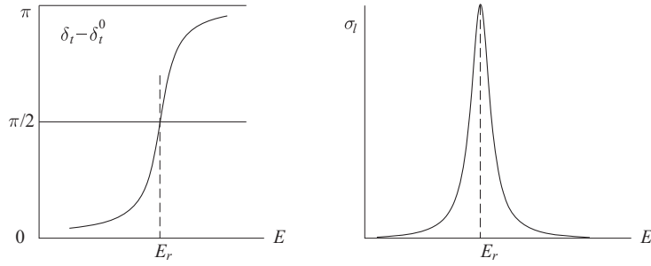
Figure 18.8 The phase shift \delta_l and the cross section \sigma as functions of the energy E , close to a resonance.
