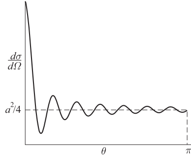
Figure 18.7 Differential cross section for a rigid sphere as a function of the scattering angle.
