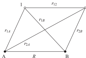
Figure 16.5 Coordinates of the particles that make up an \text{H}_2 molecule.
