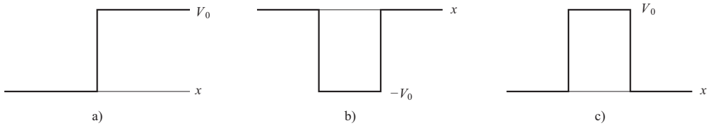
Figure 5.1 Piecewise constant potentials in one dimension. (a) The step potential, (b) The finite square well, (c) The square barrier.
