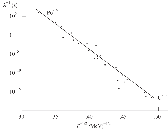
Figure 6.4 Decay constant for a wide range of radioactive isotopes as a function of alpha particle emission energy.
