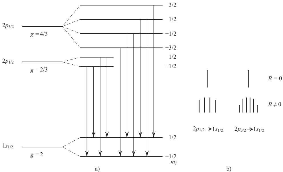
Figure 14.1 Diagram of the Zeeman spectrum showing the transitions between the lowest energy levels of the H atom. (a) The states 2p_{1/2} and 2p_{3/2} are separated by the spin–orbit coupling. (b) Line splitting for the allowed transitions 2p_{1/2} \rightarrow 1s_{1/2} and 2p_{3/2} \rightarrow 1s_{1/2} .
