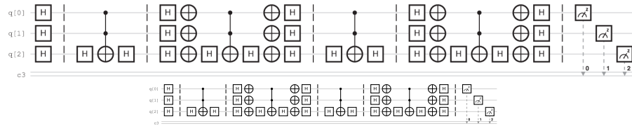
Figure 8.12. Grover’s algorithm for |G\rangle = |7\rangle , created using IBM Quantum.
