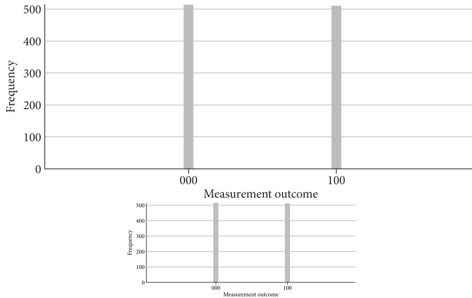
Figure 9.6. Results from the circuit in Fig. 9.5 , created using IBM Quantum.
