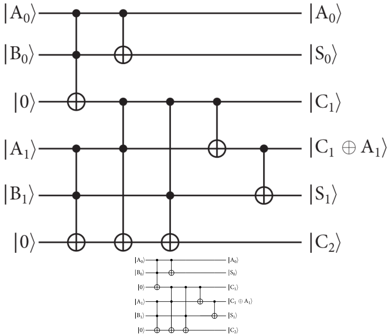
Figure 7.12. A circuit that sums two two-bit numbers, created using the Quantikz LaTeX package.
