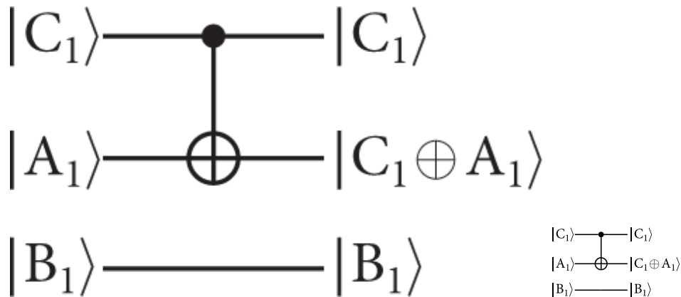
Figure 7.6. Building up to a circuit that computes the sum of three bits, created using the Quantikz LaTeX package.
