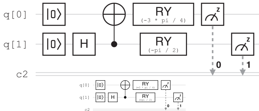
Figure 6.7. A circuit to measure \langle A_2 B_2 \rangle , created using IBM Quantum. Adapted from Jed Brody and Robert Avram, “Testing a Bell Inequality with a Remote Quantum Processor,” The Physics Teacher , March 2023, https://doi.org/10.1119/5.0069073 .
