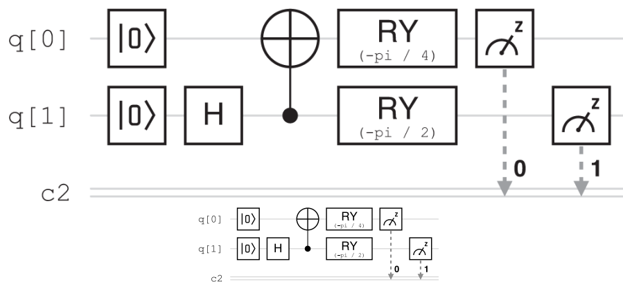
Figure 6.6. A circuit to measure \langle A_2 B_1 \rangle , created using IBM Quantum. Adapted from Jed Brody and Robert Avram, “Testing a Bell Inequality with a Remote Quantum Processor,” The Physics Teacher , March 2023, https://doi.org/10.1119/5.0069073 .
