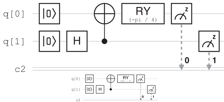
Figure 6.4. A circuit to measure \langle A_1 B_1 \rangle , created using IBM Quantum. Adapted from Jed Brody and Robert Avram, "Testing a Bell Inequality with a Remote Quantum Processor," The Physics Teacher , March 2023, https://doi.org/10.1119/5.0069073 .
