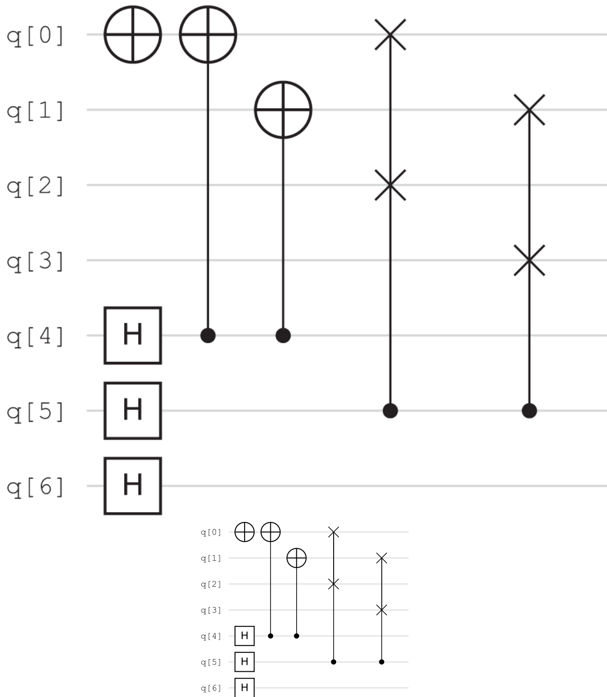
Figure 10.15. The circuit to determine the order of 2 mod 15, excluding the IQFT, created using IBM Quantum.
