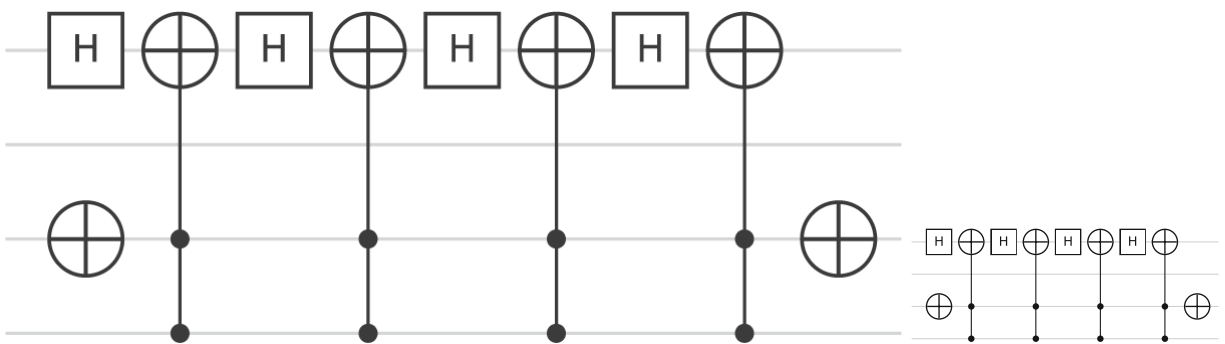
Figure 8.18. The same circuit as Fig. 8.17 , constructing the doubly controlled Z gates as shown in Fig. 8.6 , created using IBM Quantum.
