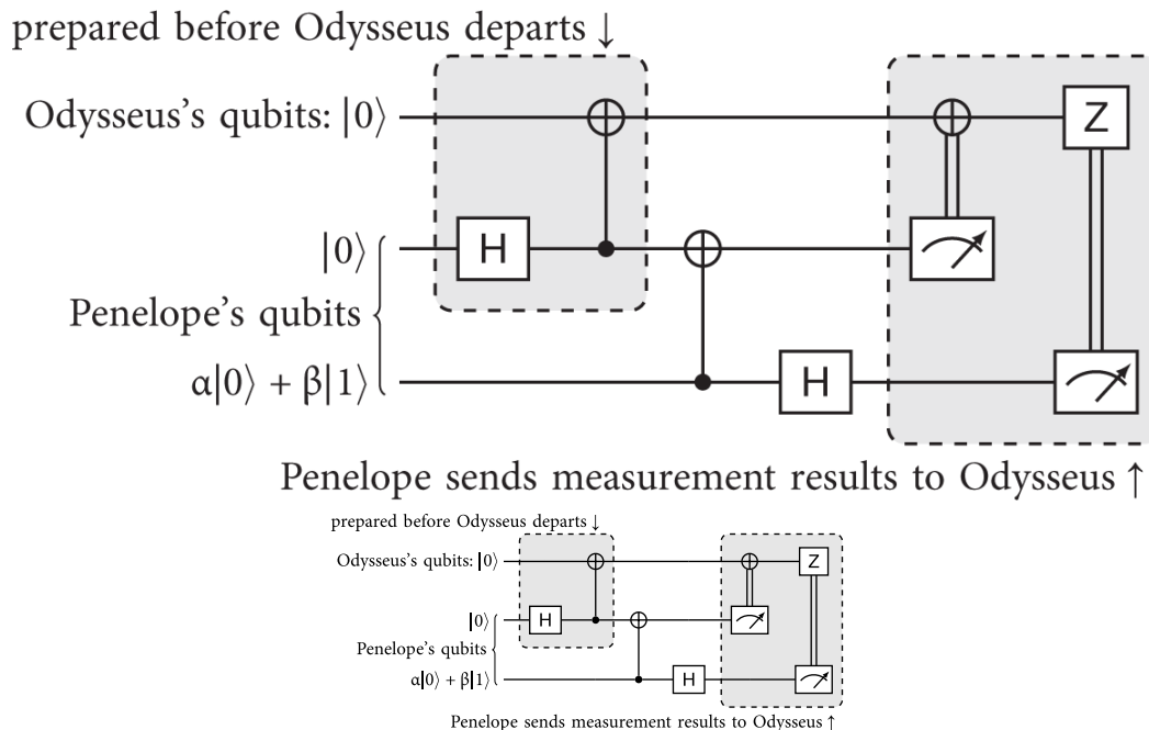
Figure 4.1. Quantum teleportation, created using the Quantikz LaTeX package.
