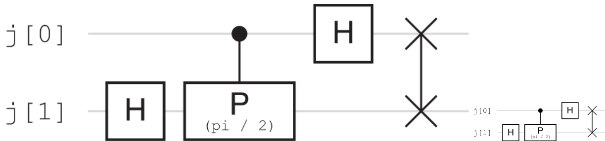
Figure 9.1. The two-qubit quantum Fourier transform, created using IBM Quantum.
