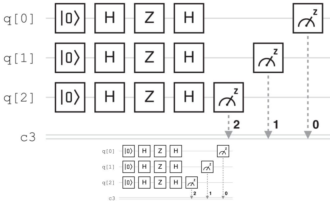
Figure 3.9. The Deutsch-Jozsa algorithm for a balanced function of three bits, created using IBM Quantum.
