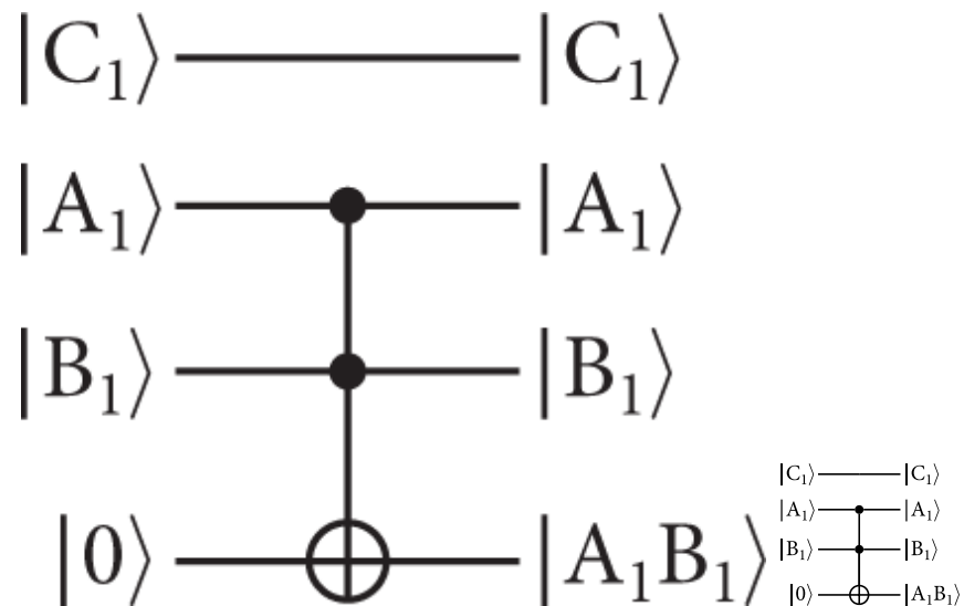
Figure 7.8. Building up to a circuit that computes the carry bit from a sum of three bits, created using the Quantikz LaTeX package.
