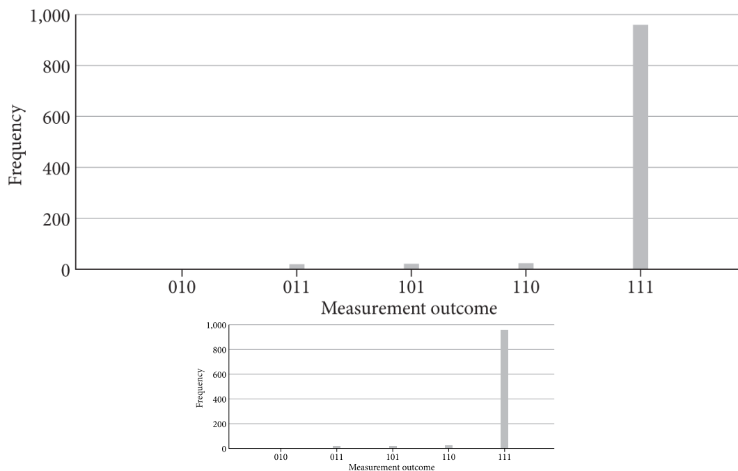
Figure 3.10. Results from the circuit in Fig. 3.9 , created using IBM Quantum.
