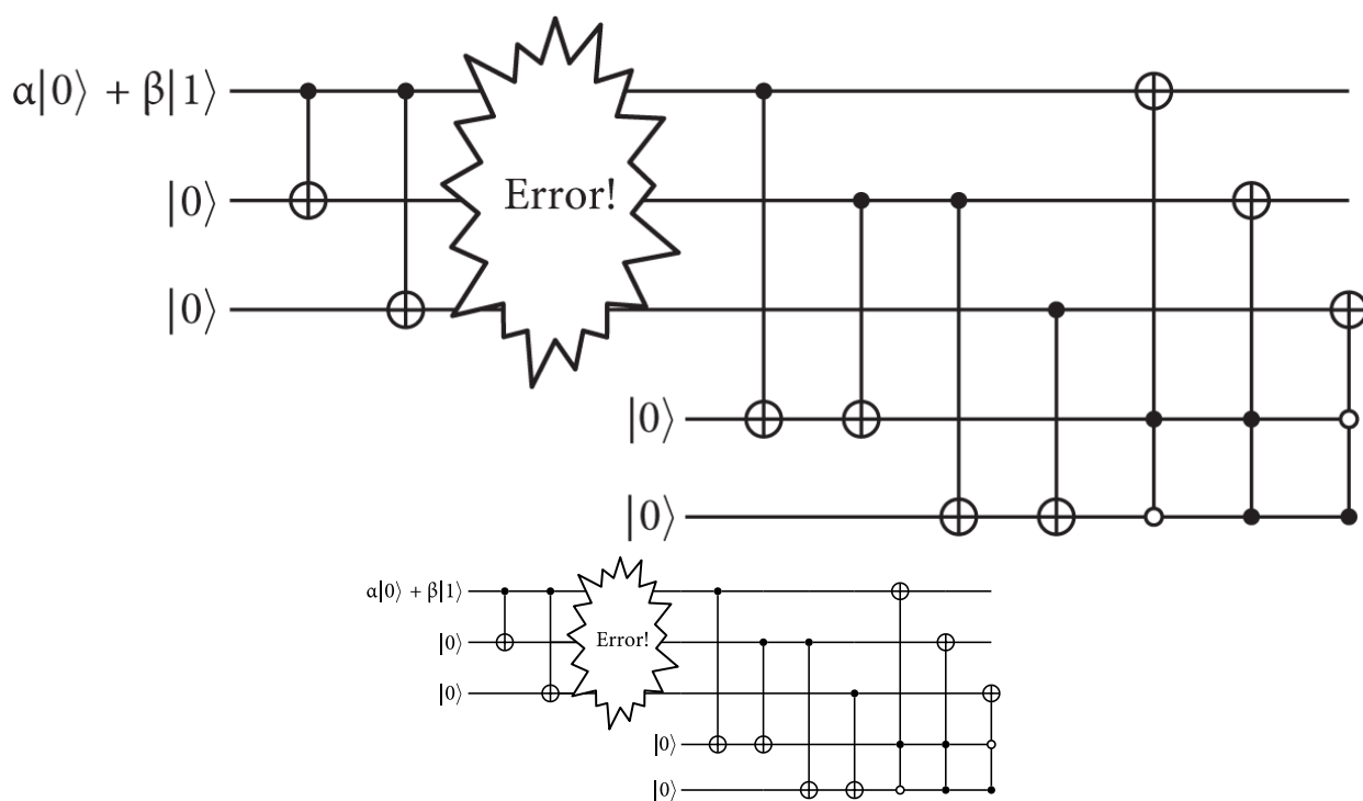
Figure 12.1. Correcting a bit-flip error, created using the Quantikz LaTeX package, including some of the code in the Quantikz tutorial by Alastair Kay ( https://arxiv.org/pdf/1809.03842 ).
