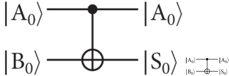
Figure 7.1. A circuit to compute a sum bit, created using the Quantikz LaTeX package.
