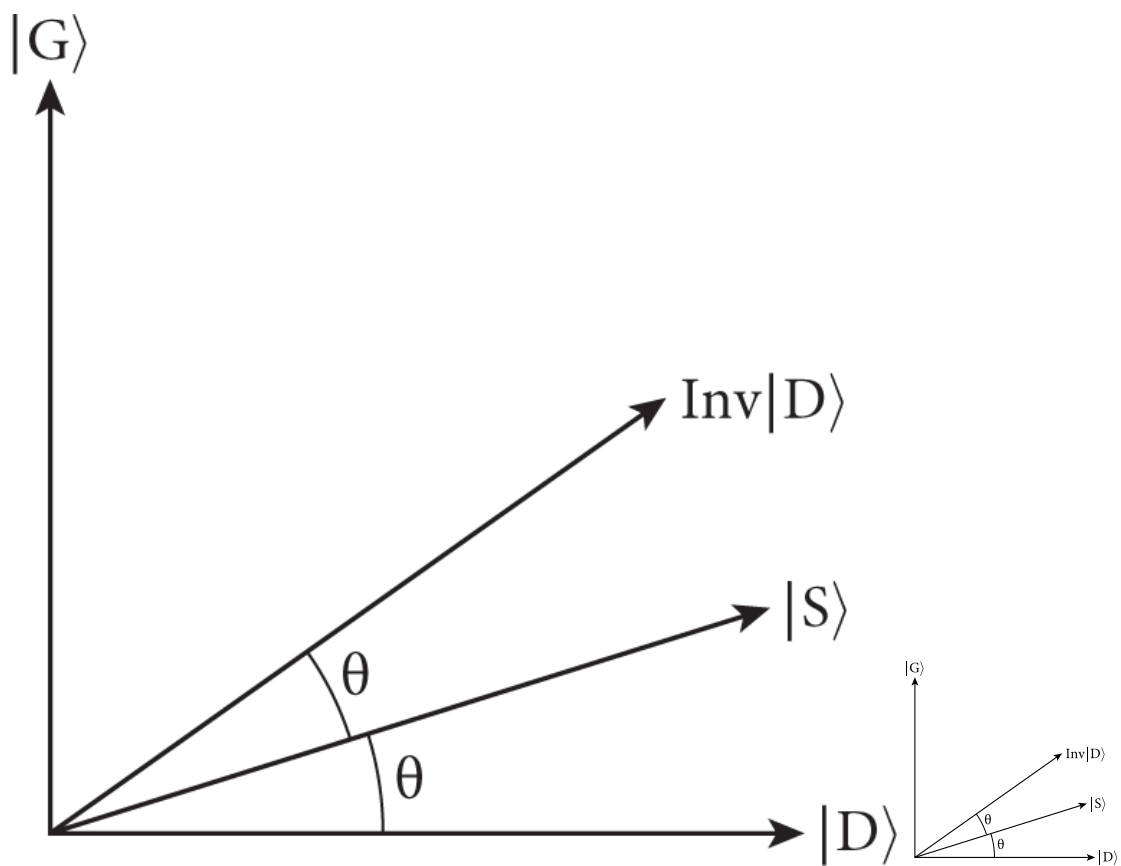
Figure 8.4. \text{Inv} acting as a reflection about |S\rangle .
