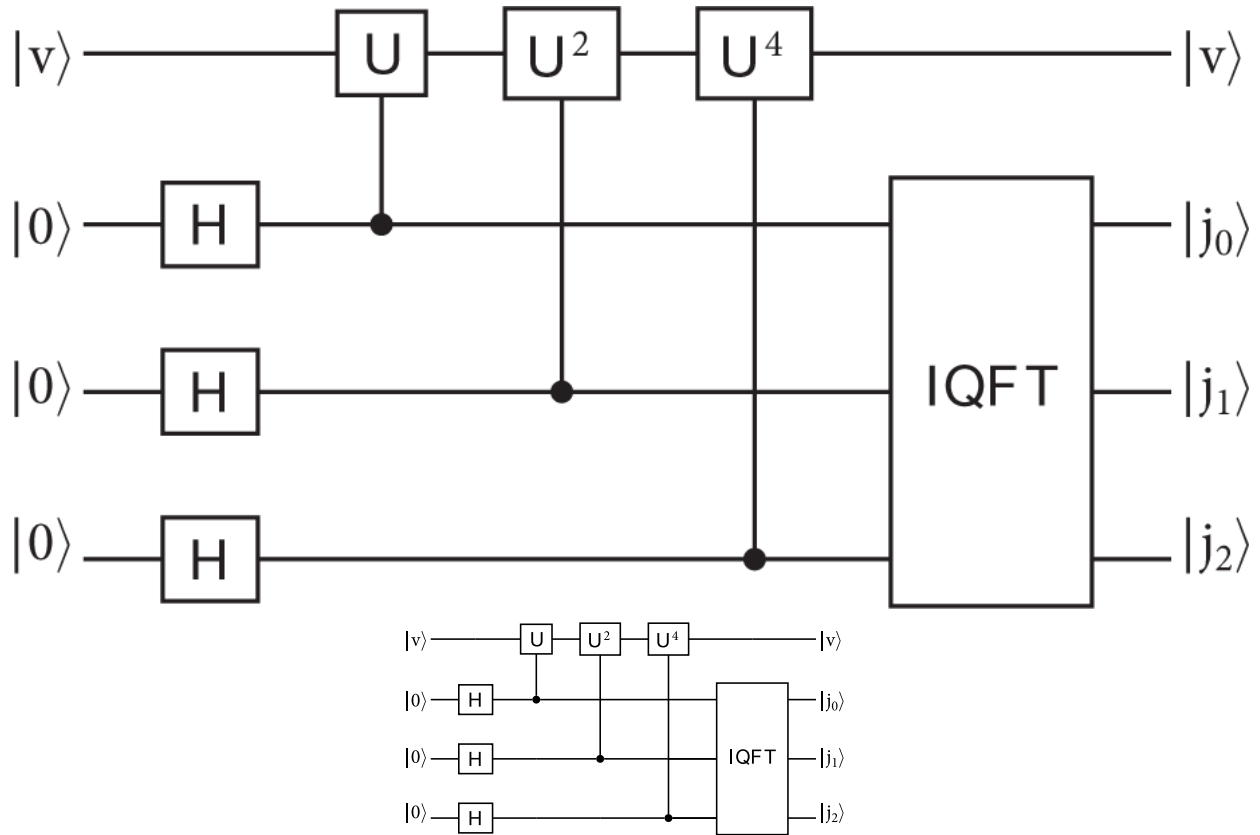
Figure 10.4. Quantum phase estimation, created using the Quantikz LaTeX package.
