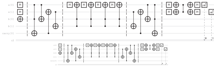
Figure 8.24. Grover's algorithm to solve A + 1 = 3 , created using IBM Quantum.
