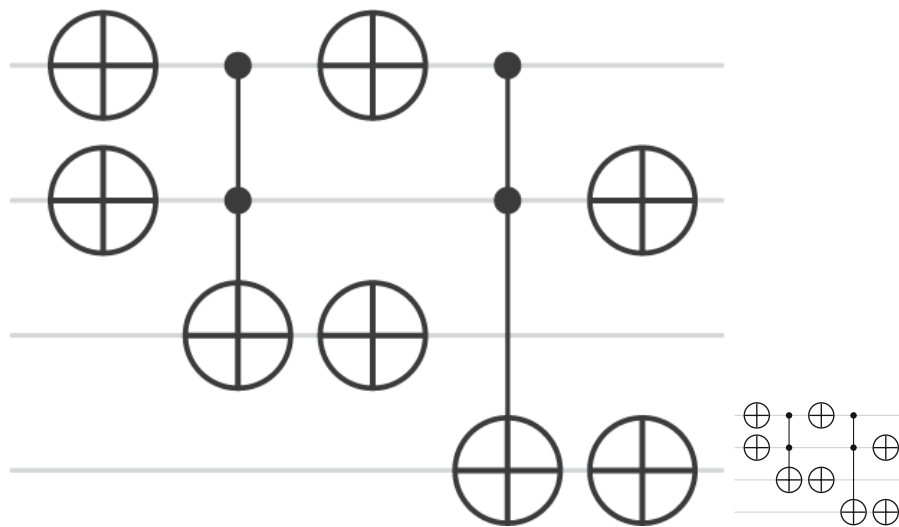
Figure 8.19. The inverse the of the phone book operation shown in Fig. 8.14 , created using IBM Quantum.
