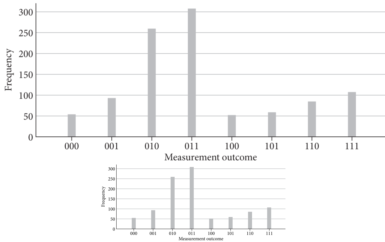
Figure 7.18. Results from the circuit in Fig. 7.17 , created using IBM Quantum.
