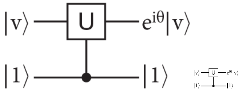
Figure 10.2. A controlled operator that acts on its eigenvalue because the control is |1\rangle , created using the Quantikz LaTeX package.
