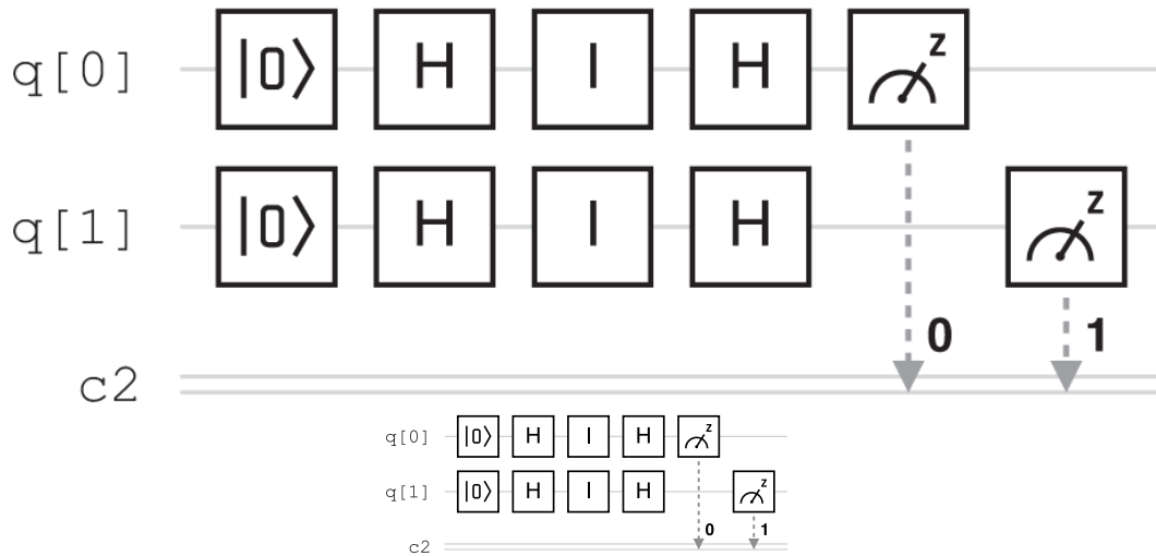
Figure 3.3. The Deutsch-Jozsa algorithm for a constant function, created using IBM Quantum.
