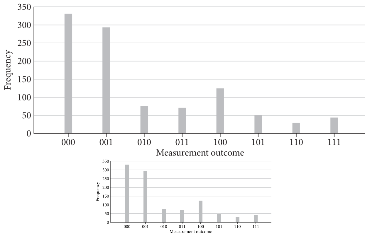
Figure 10.12. Results from the circuit in Fig. 10.11 , created using IBM Quantum.
