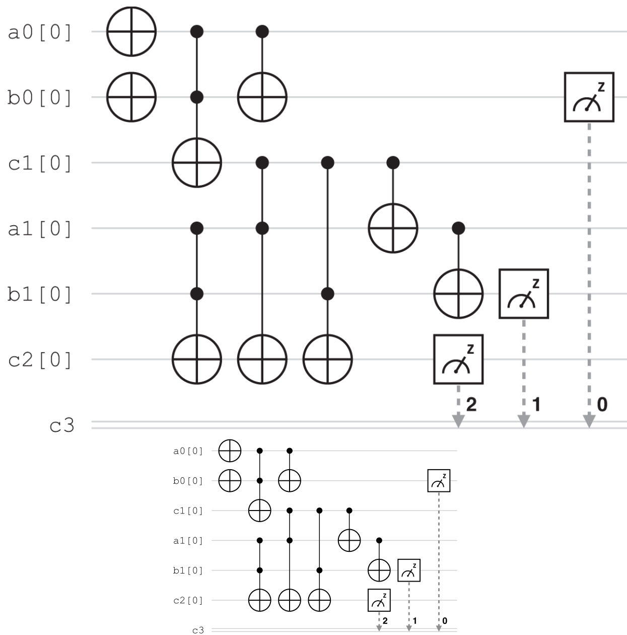
Figure 7.15. A circuit that calculates 1 + 1 , created using IBM Quantum.
