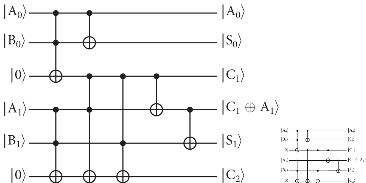
Figure 8.21. A circuit that sums two two-bit numbers, created using the Quantikz LaTeX package.
