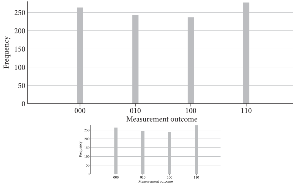
Figure 9.4. Results from the circuit in Fig. 9.3 , created using IBM Quantum.
