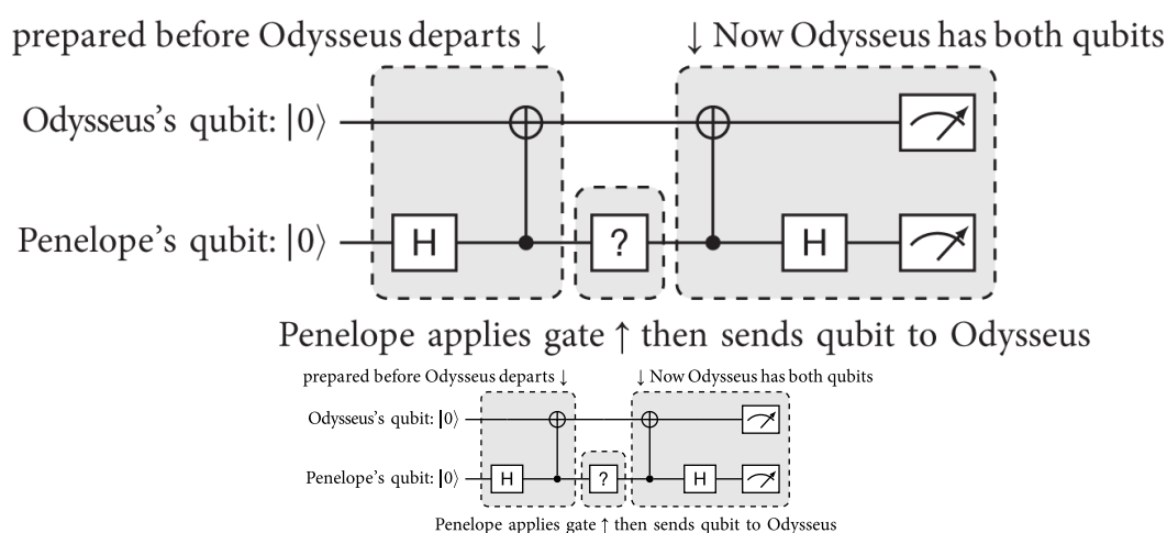
Figure 4.2. Quantum dense coding, created using the Quantikz LaTeX package.
