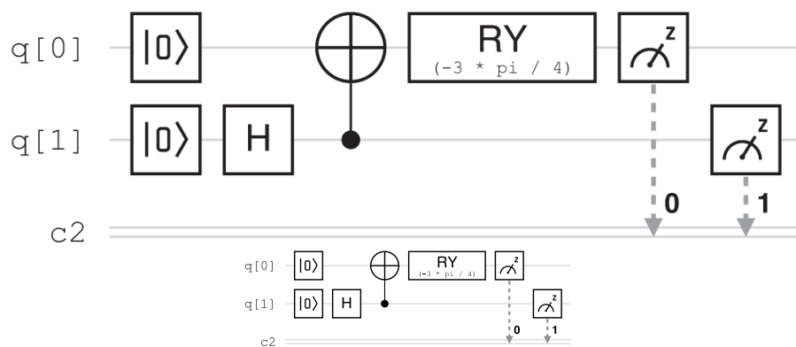
Figure 6.5. A circuit to measure \langle A_1 B_2 \rangle , created using IBM Quantum. Adapted from Jed Brody and Robert Avram, “Testing a Bell Inequality with a Remote Quantum Processor,” The Physics Teacher , March 2023, https://doi.org/10.1119/5.0069073 .
