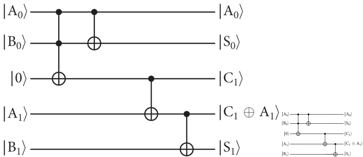
Figure 8.22. A circuit that sums two two-bit numbers without generating a final carry bit, created using the Quantikz LaTeX package.
