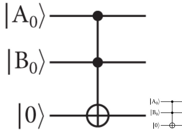
Figure 7.3. The Toffoli gate configured to compute a carry bit, created using the Quantikz LaTeX package.
