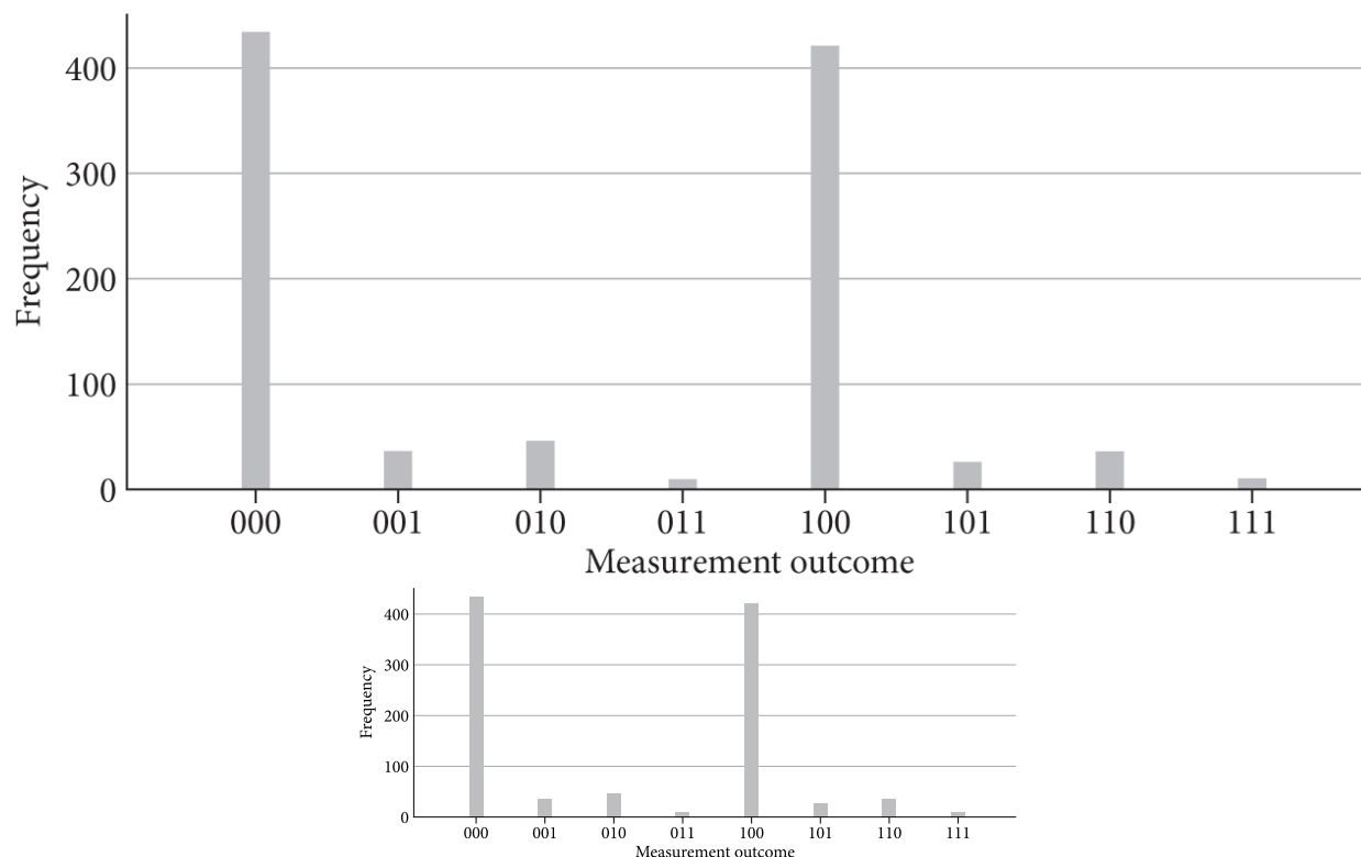
Figure 10.23. Results from the circuit in Fig. 10.17 , created using IBM Quantum.
