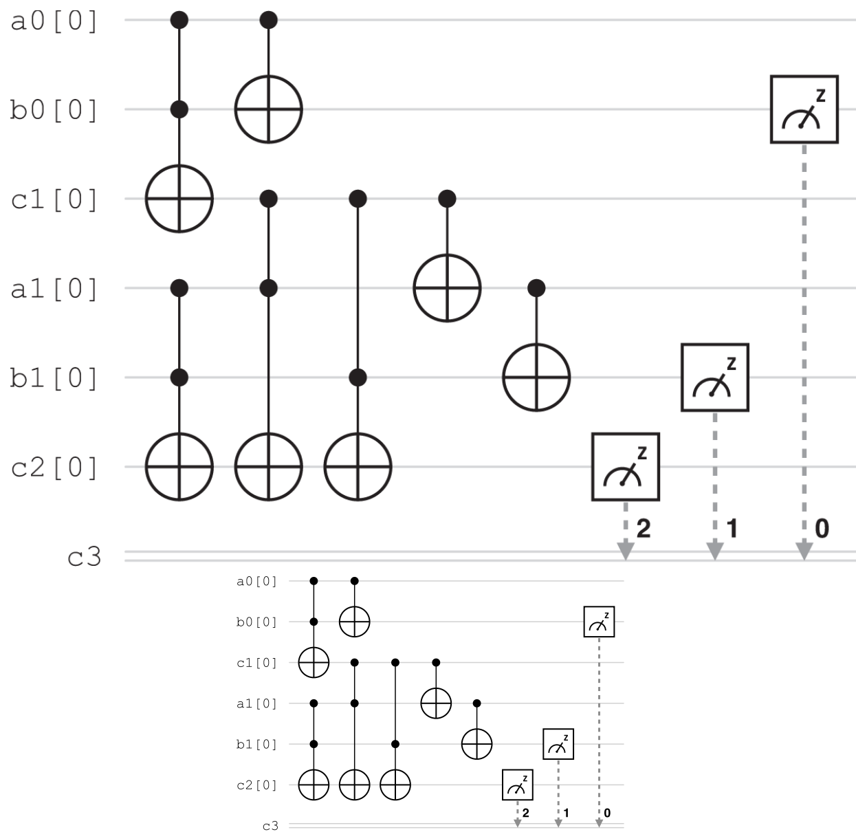
Figure 7.13. A circuit that calculates 0 + 0 , created using IBM Quantum.
