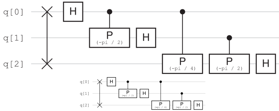
Figure 9.7. The three-qubit inverse quantum Fourier transform, created using IBM Quantum.
