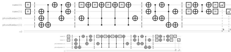
Figure 8.20. Grover's algorithm applied to the quantum phone book, created using IBM Quantum.
