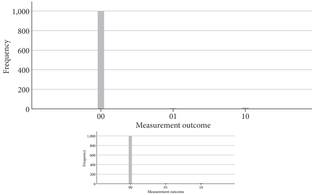
Figure 3.4. Results from the circuit in Fig. 3.3 , created using IBM Quantum.
