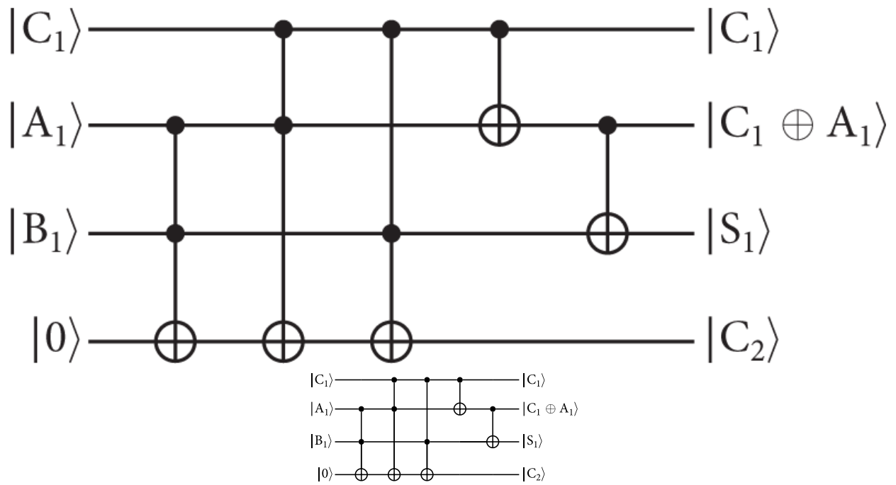
Figure 7.11. A full adder, created using the Quantikz LaTeX package.
