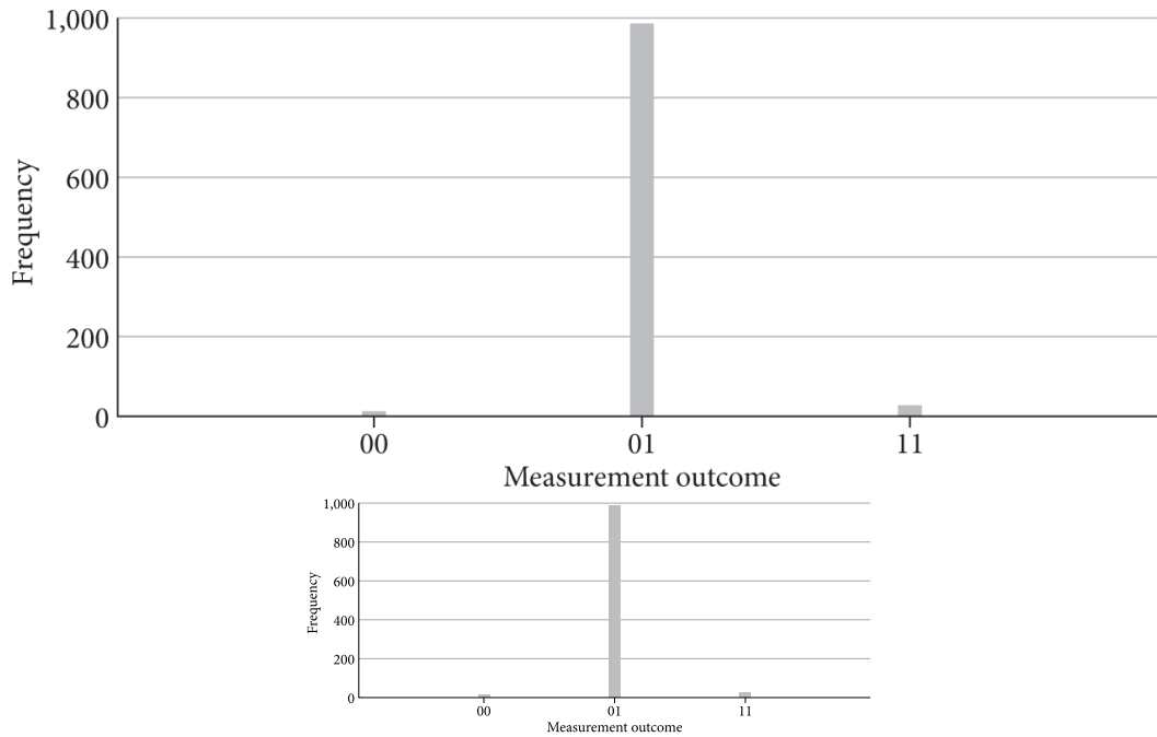
Figure 3.6. Results from the circuit in Fig. 3.5 , created using IBM Quantum.
