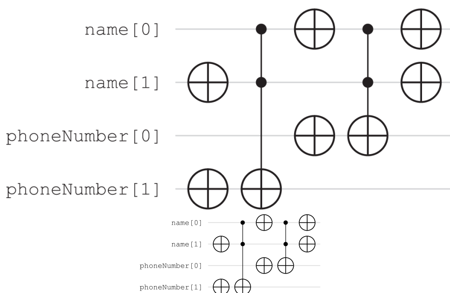
Figure 8.14. A quantum phone book, created using IBM Quantum.
