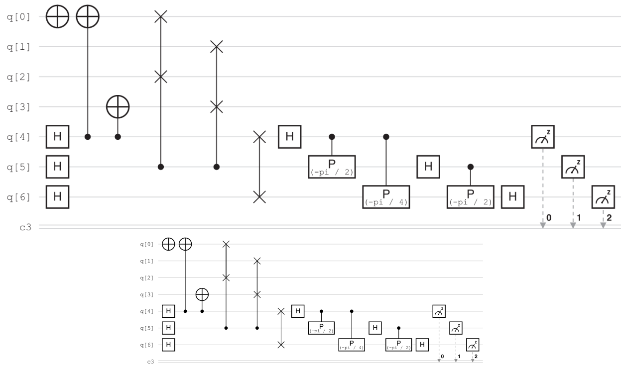
Figure 10.19. The circuit to determine the order of 8 \bmod 15 , created using IBM Quantum. Originally published in Jed Brody and Kristen Gram, “Factoring 15 with a Remote Quantum Computer: A Complete Guide for Beginners,” European Journal of Physics , April 2024, https://iopscience.iop.org/article/10.1088/1361-6404/ad32dc/pdf , under open license CC BY 4.0.
