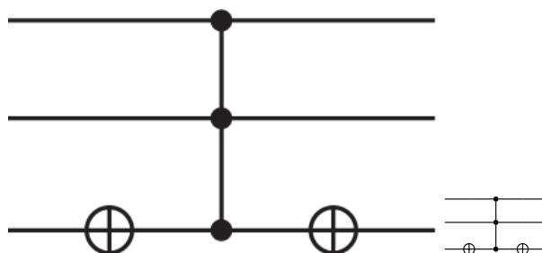
Figure 8.7. A circuit to multiply |011\rangle by -1 , created using the Quantikz LaTeX package.
