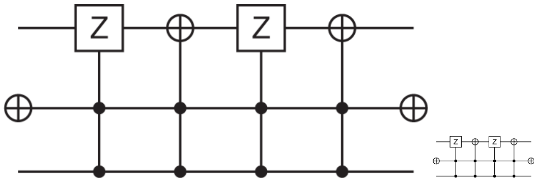
Figure 8.17. The same circuit as Fig. 8.16 , without open-circle controls, created using the Quantikz LaTeX package.
