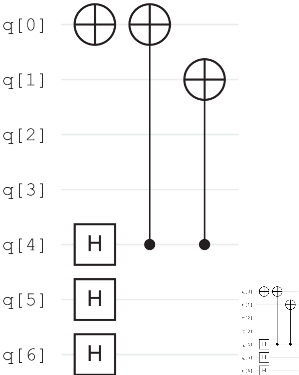
Figure 10.14. The first part of the circuit to determine the order of 2 \bmod 15 , created using IBM Quantum.
