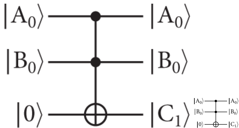
Figure 7.4. A circuit to compute a carry bit, created using the Quantikz LaTeX package.
