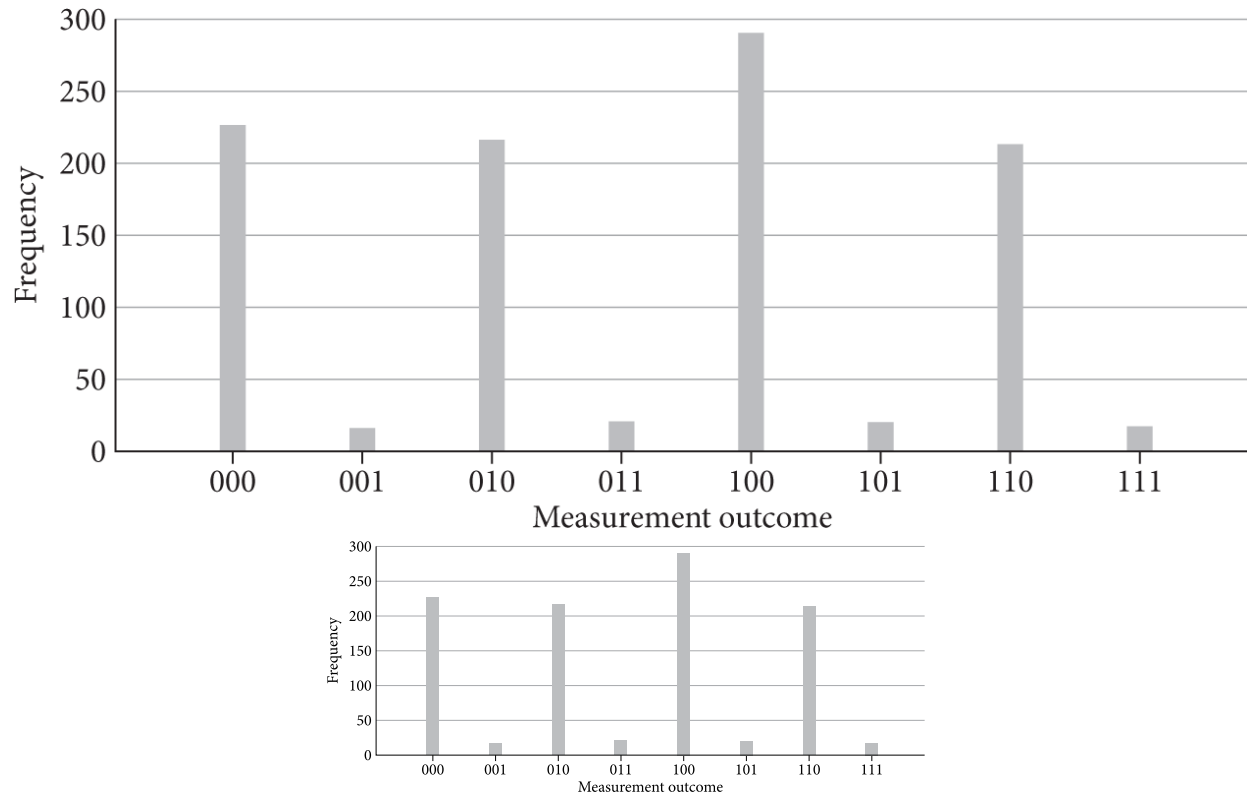
Figure 10.22. Results from the circuit in Fig. 10.16 , created using IBM Quantum.
