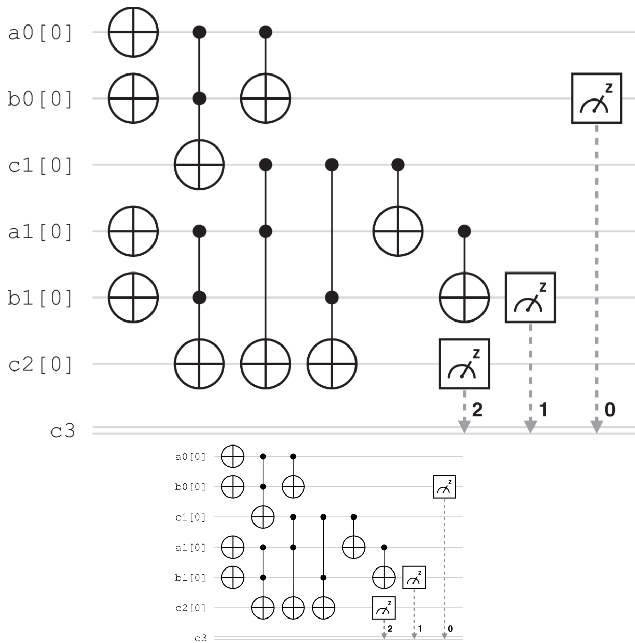
Figure 7.19. A circuit that calculates 3 + 3 , created using IBM Quantum.
