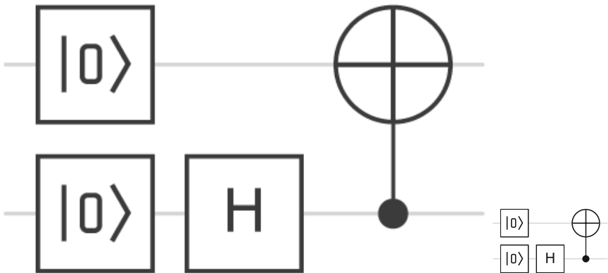
Figure 3.1. A circuit to produce an entangled state, created using IBM Quantum.
