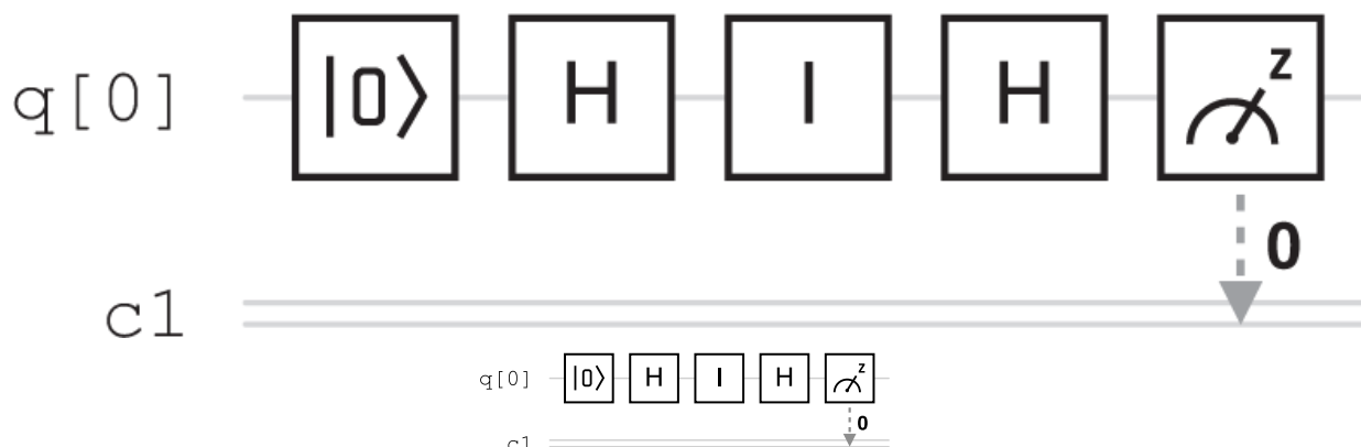
Figure 2.1. Deutsch's algorithm with a phase oracle for a constant function, created using IBM Quantum.
