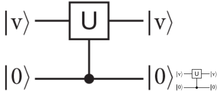
Figure 10.1. A controlled operator that does not act on its eigenvalue because the control is |0\rangle , created using the Quantikz LaTeX package.
