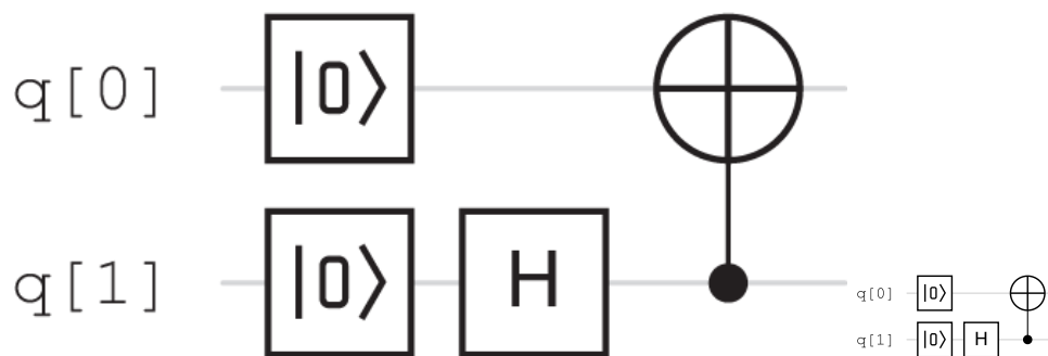
Figure 6.2. A circuit to produce an entangled state, created using IBM Quantum.
