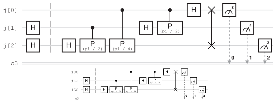
Figure 9.5. The circuit to generate the QFT of \frac{1}{2}|0\rangle + \frac{1}{2}|2\rangle + \frac{1}{2}|4\rangle + \frac{1}{2}|6\rangle , created using IBM Quantum.
