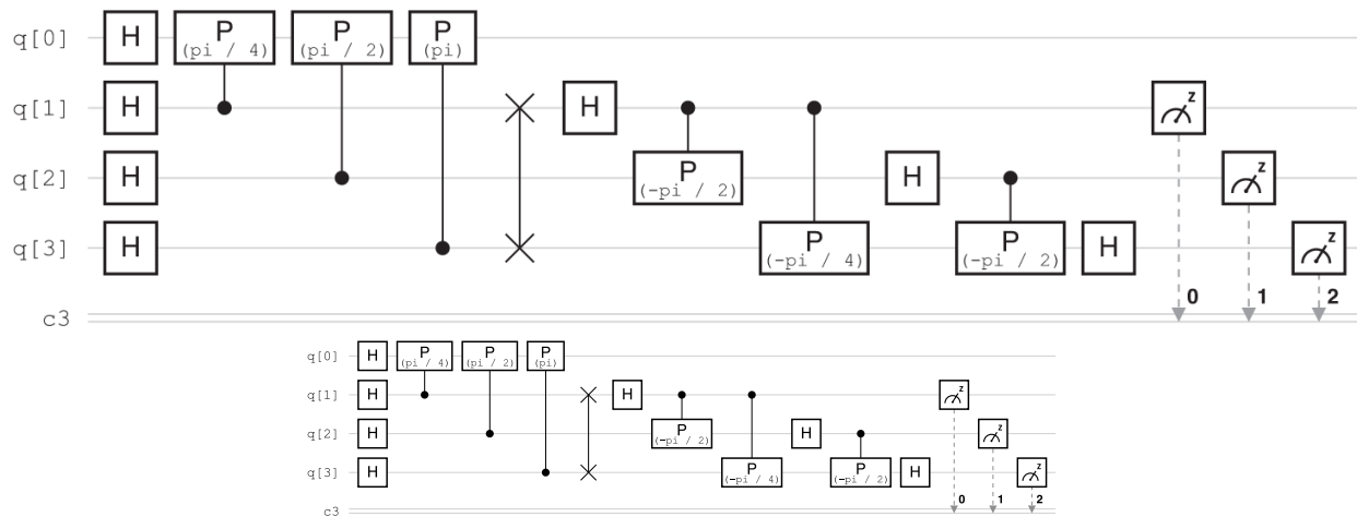
Figure 10.11. Quantum phase estimation to determine both eigenvalues association of P(\pi/4) , created using IBM Quantum.
