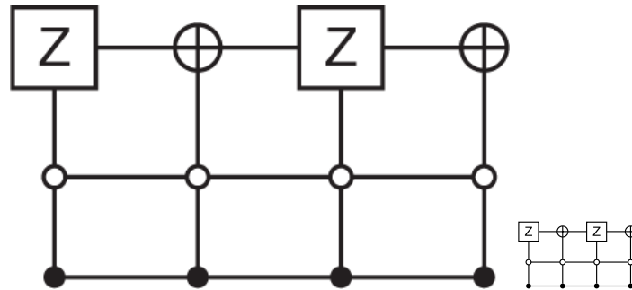
Figure 8.16. Construction of the desired oracle, created using the Quantikz LaTeX package.
