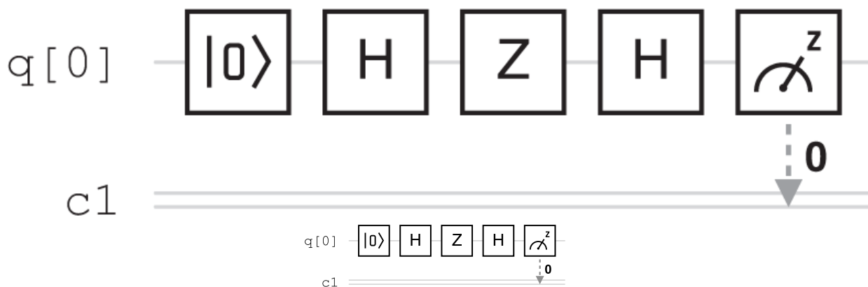
Figure 2.3. Deutsch's algorithm with a phase oracle for a balanced function, created using IBM Quantum.
