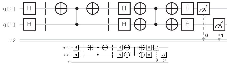
Figure 8.11. Grover’s algorithm for |G\rangle = |2\rangle , created using IBM Quantum.
