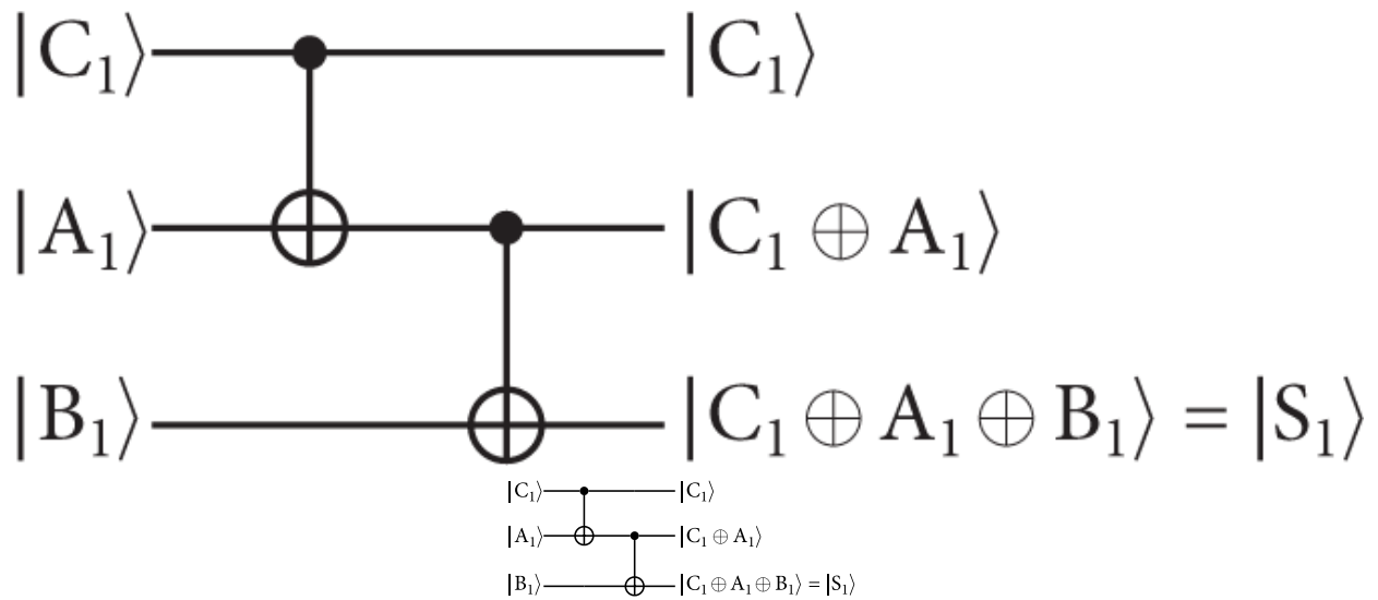
Figure 7.7. A circuit that computes the sum of three bits, created using the Quantikz LaTeX package.
