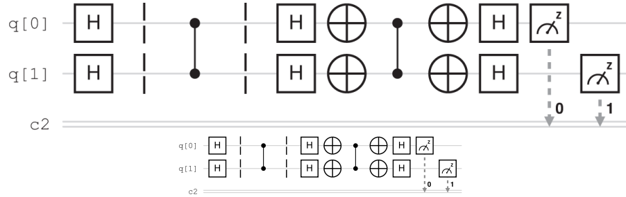
Figure 8.10. Grover's algorithm for |G\rangle = |3\rangle , created using IBM Quantum.
