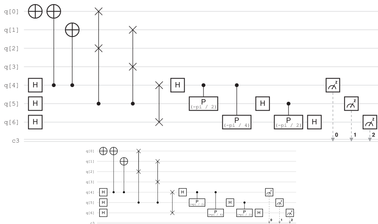
Figure 10.16. The circuit to determine the order of 2 \bmod 15 , created using IBM Quantum. Originally published in Jed Brody and Kristen Gram, “Factoring 15 with a Remote Quantum Computer: A Complete Guide for Beginners,” European Journal of Physics , April 2024, https://iopscience.iop.org/article/10.1088/1361-6404/ad32dc/pdf , under open license CC BY 4.0.
