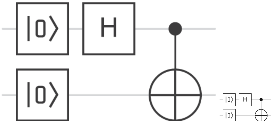
Figure 3.2. A circuit that produces the same entangled state as the one in Fig. 3.1 , created using IBM Quantum.
