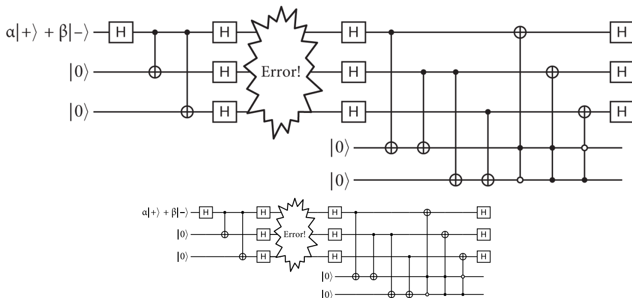
Figure 12.2. Correcting a phase-flip error, created using the Quantikz LaTeX package, including some of the code in the Quantikz tutorial by Alastair Kay ( https://arxiv.org/pdf/1809.03842 ).
