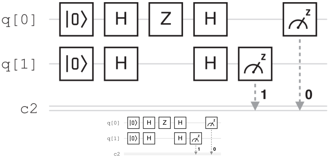
Figure 3.5. The Deutsch-Jozsa algorithm for the function f(x) = x_0 , created using IBM Quantum.
