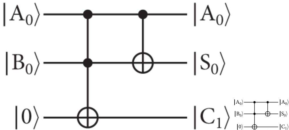
Figure 7.5. A half adder, created using the Quantikz LaTeX package.
