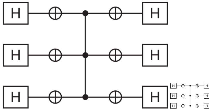
Figure 8.9. Inversion about the mean, created using the Quantikz LaTeX package.
