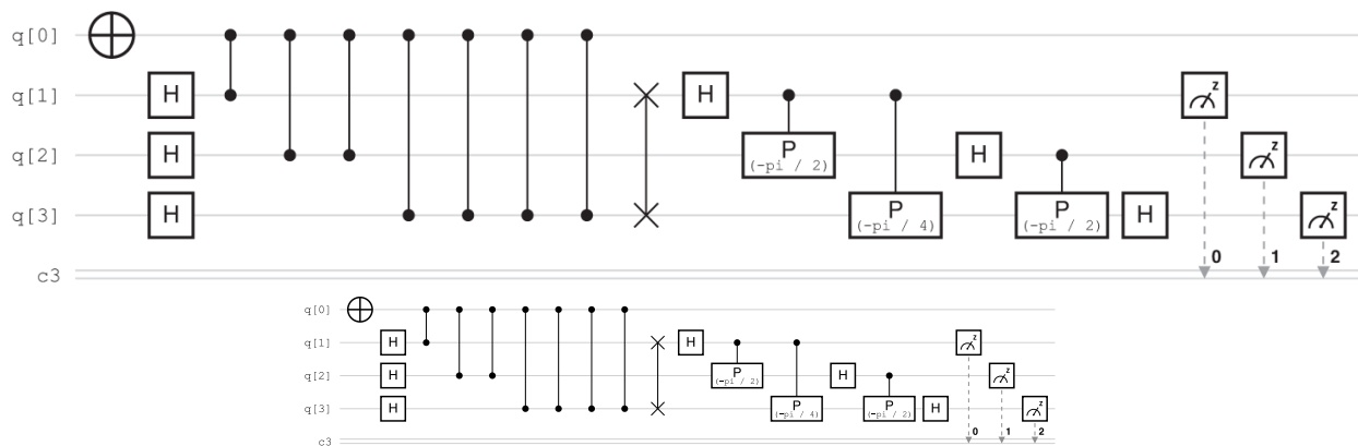
Figure 10.5. Quantum phase estimation to determine the eigenvalue associated with the |1\rangle eigenvector of Z , created using IBM Quantum.
