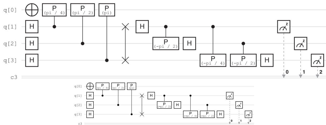
Figure 10.9. Quantum phase estimation to determine the eigenvalue association with the |1\rangle eigenvector of P(\pi/4) , created using IBM Quantum. Originally published in Jed Brody and Kristen Gram, “Factoring 15 with a Remote Quantum Computer: A Complete Guide for Beginners,” European Journal of Physics , April 2024, https://iopscience.iop.org/article/10.1088/1361-6404/ad32dc/pdf , under open license CC BY 4.0.
