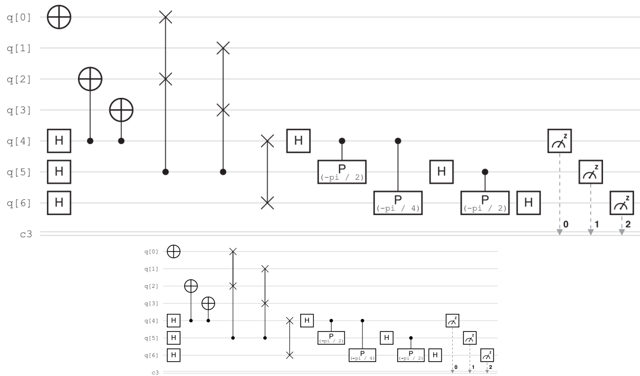
Figure 10.21. The circuit to determine the order of 13 \bmod 15 , created using IBM Quantum. Originally published in Jed Brody and Kristen Gram, “Factoring 15 with a Remote Quantum Computer: A Complete Guide for Beginners,” European Journal of Physics , April 2024, https://iopscience.iop.org/article/10.1088/1361-6404/ad32dc/pdf , under open license CC BY 4.0.
