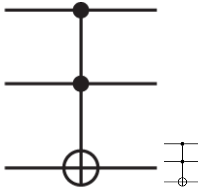
Figure 7.2. The Toffoli gate, created using the Quantikz LaTeX package.
