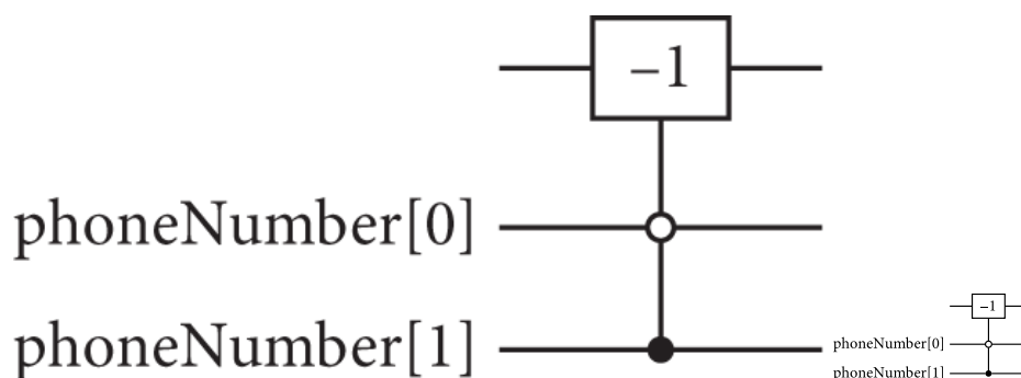
Figure 8.15. The oracle for a desired phone number of 10, created using the Quantikz LaTeX package.
