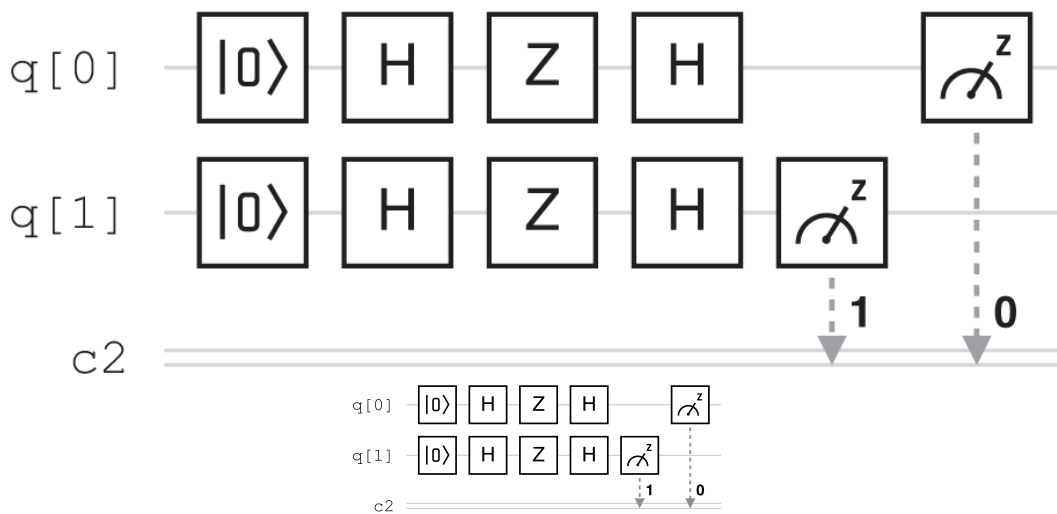
Figure 3.7. The Deutsch-Jozsa algorithm for the function f(x) = 1 if and only if the two bits of x differ, created using IBM Quantum.
