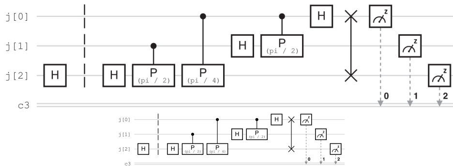
Figure 9.3. The circuit to generate the QFT of \frac{1}{\sqrt{2}}|0\rangle + \frac{1}{\sqrt{2}}|4\rangle , created using IBM Quantum.
