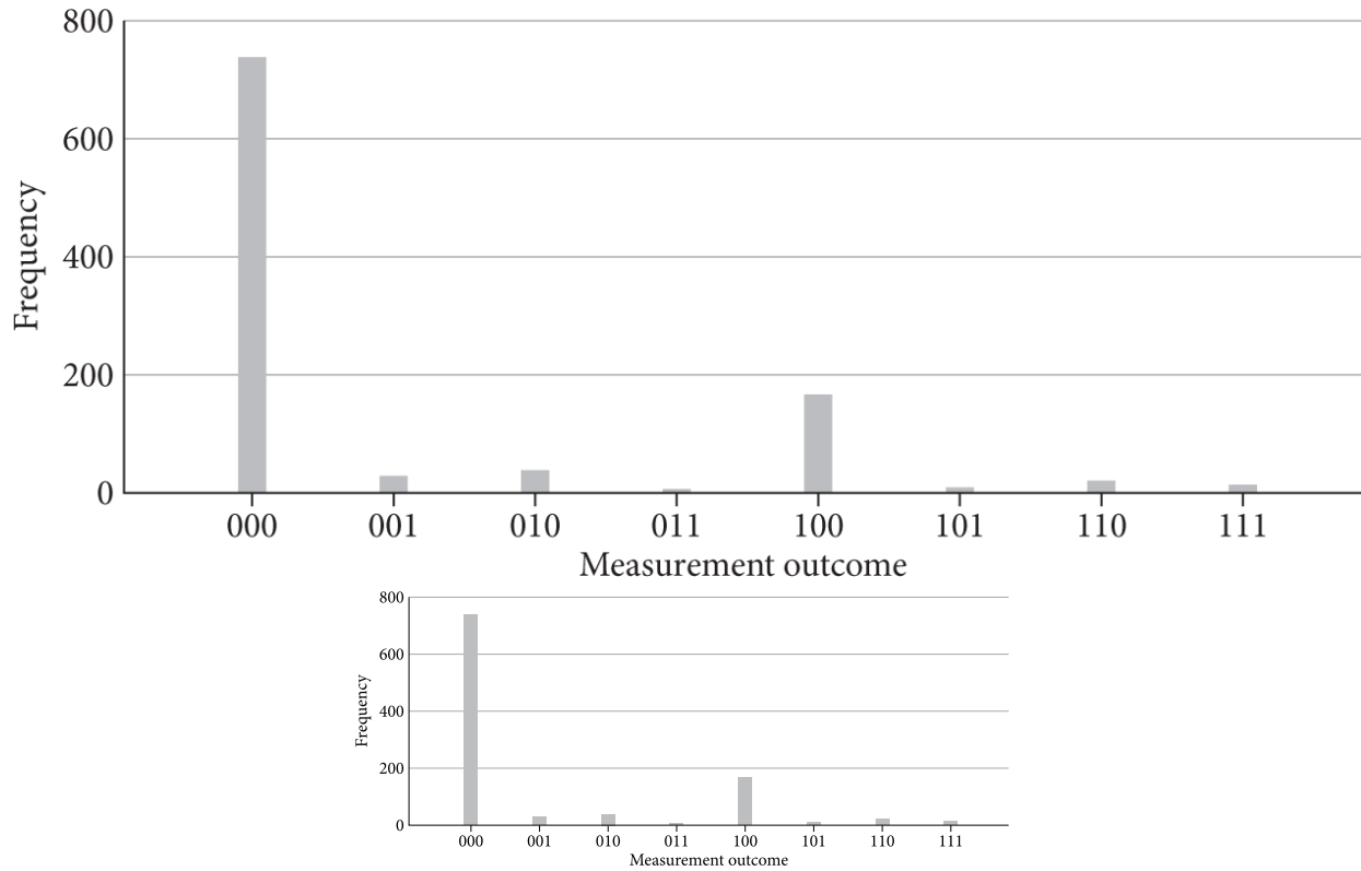
Figure 10.8. Results from the circuit in Fig. 10.7 , created using IBM Quantum.
