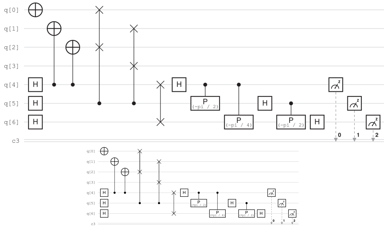
Figure 10.18. The circuit to determine the order of 7 \bmod 15 , created using IBM Quantum. Originally published in Jed Brody and Kristen Gram, “Factoring 15 with a Remote Quantum Computer: A Complete Guide for Beginners,” European Journal of Physics , April 2024, https://iopscience.iop.org/article/10.1088/1361-6404/ad32dc/pdf , under open license CC BY 4.0.
