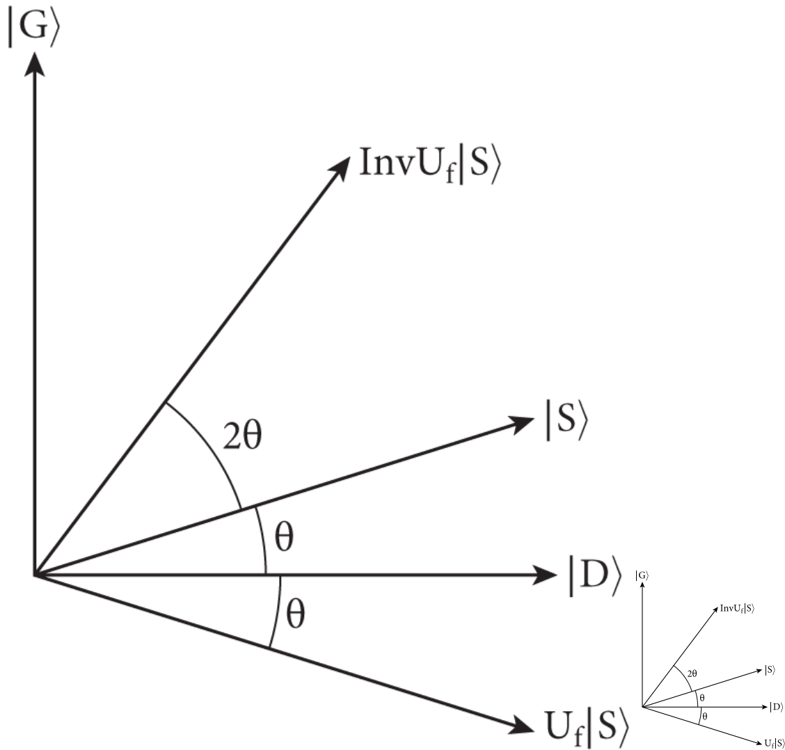
Figure 8.5. The effect of \text{Inv}U_f , a counterclockwise rotation of 2\theta .
