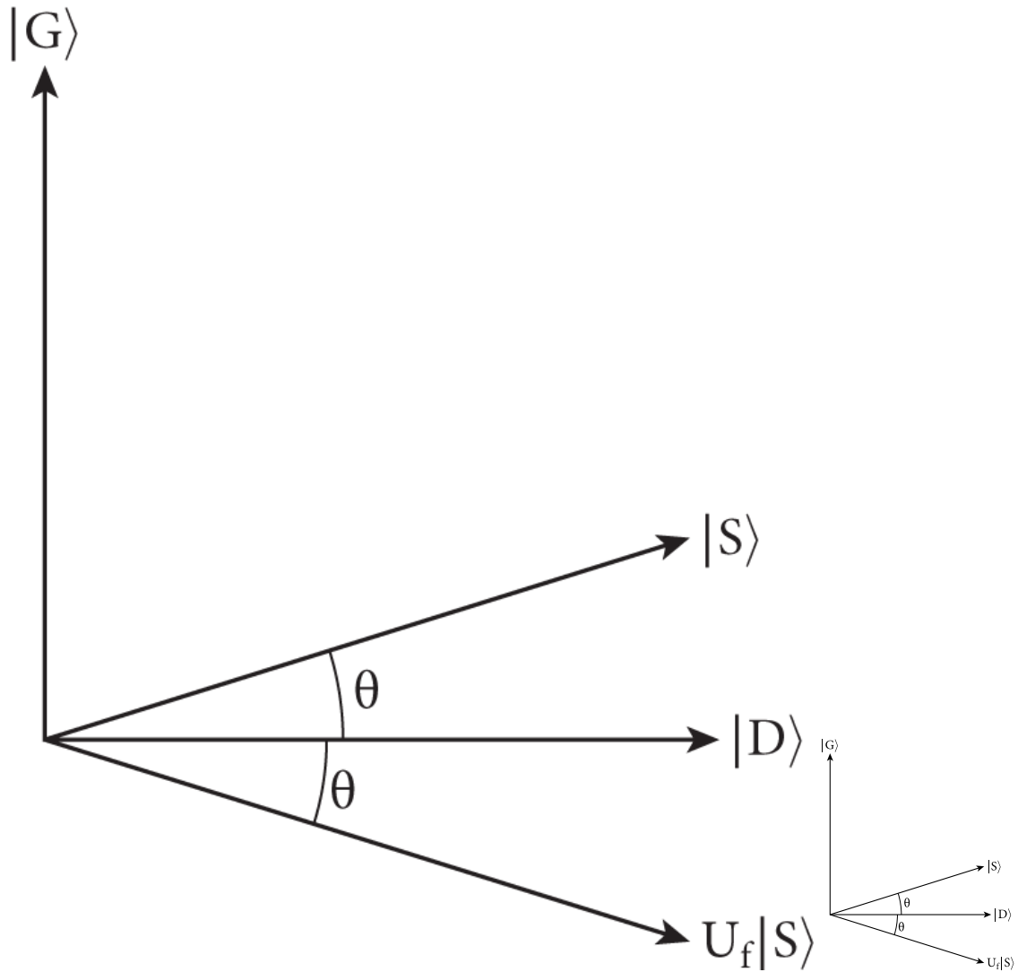
Figure 8.3. U_f acting as a reflection about |D\rangle .
