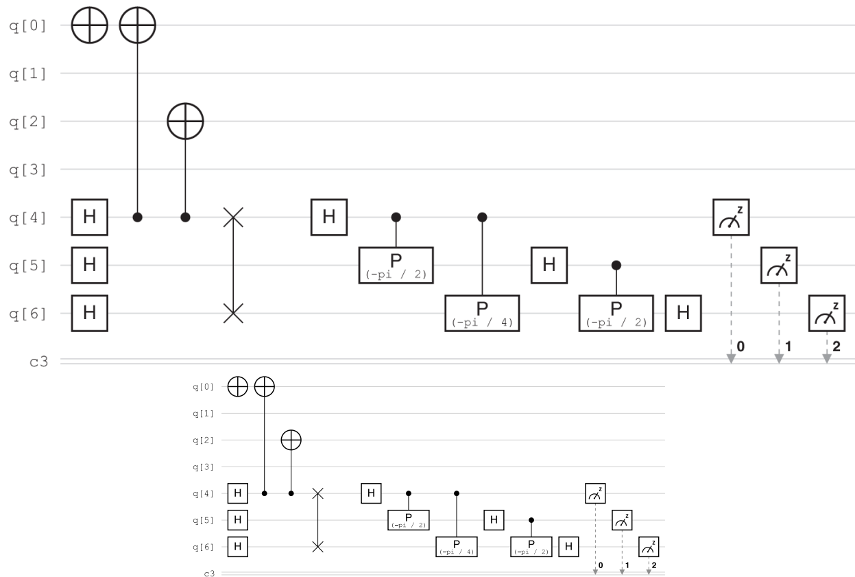
Figure 10.17. The circuit to determine the order of 4 \bmod 15 , created using IBM Quantum. Originally published in Jed Brody and Kristen Gram, “Factoring 15 with a Remote Quantum Computer: A Complete Guide for Beginners,” European Journal of Physics , April 2024, https://iopscience.iop.org/article/10.1088/1361-6404/ad32dc/pdf , under open license CC BY 4.0.
