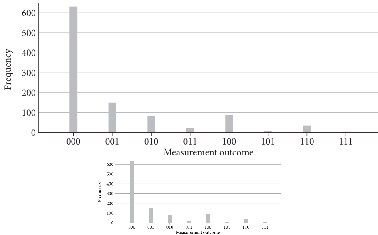
Figure 7.14. Results from the circuit in Fig. 7.13 , created using IBM Quantum.
