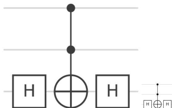
Figure 8.6. Construction of a doubly controlled Z, created using IBM Quantum.
