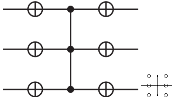
Figure 8.8. A circuit to multiply |000\rangle by -1 , created using the Quantikz LaTeX package.
