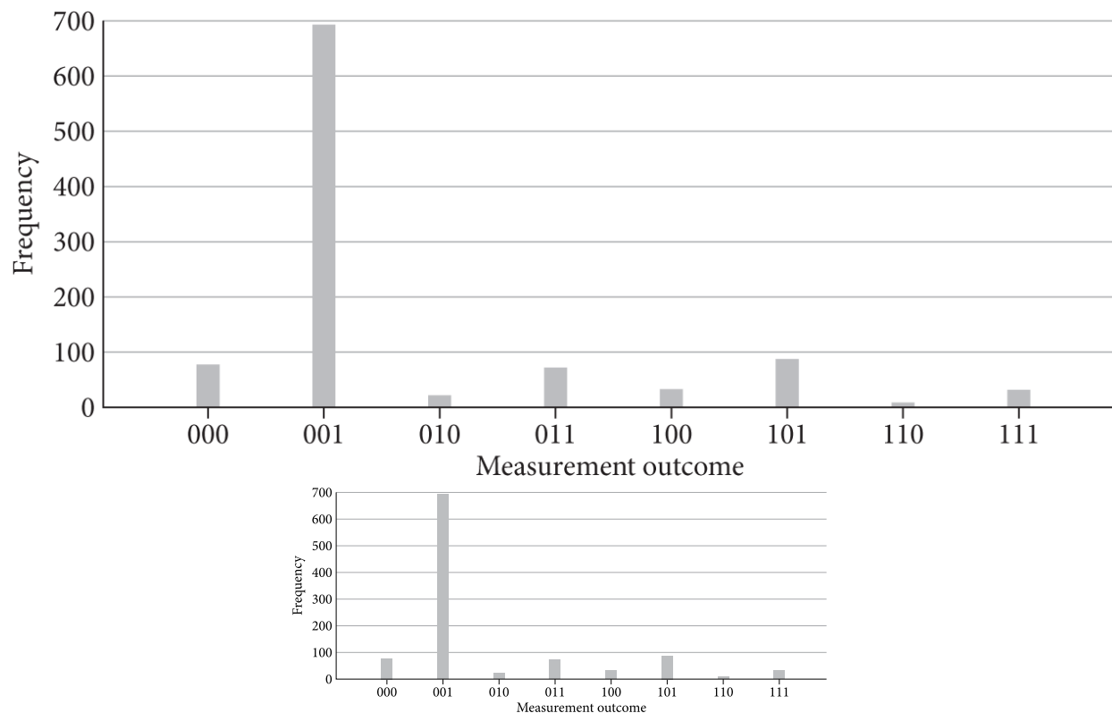
Figure 10.10. Results from the circuit in Fig. 10.9 , created using IBM Quantum.
