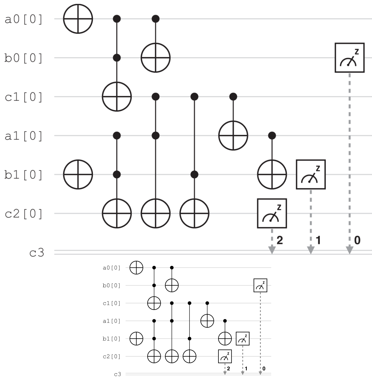
Figure 7.17. A circuit that calculates 1 + 2 , created using IBM Quantum.
