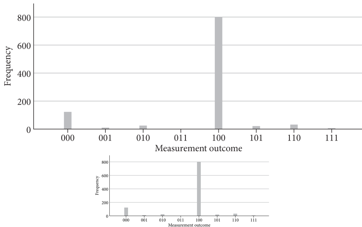
Figure 10.6. Results from the circuit in Fig. 10.5 , created using IBM Quantum.
