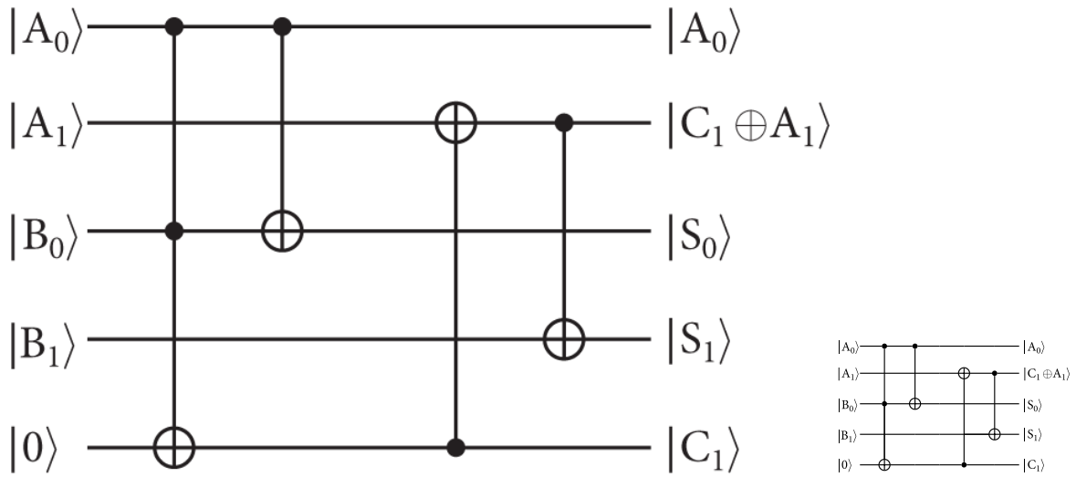
Figure 8.23. A rearrangement of Fig. 8.22 , created using the Quantikz LaTeX package.
