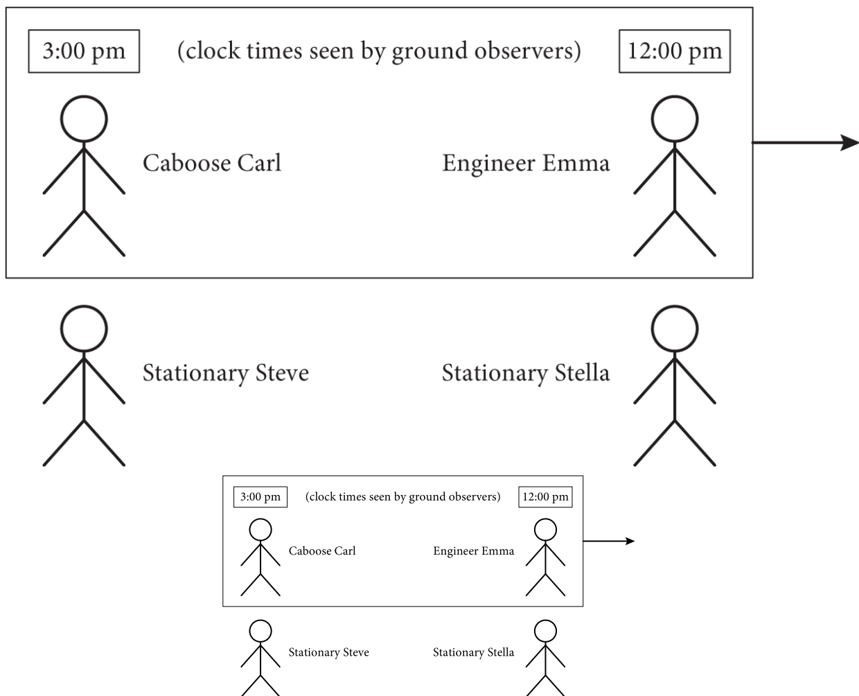
Figure 5.1. A relativistic train as seen by observers on the ground.
