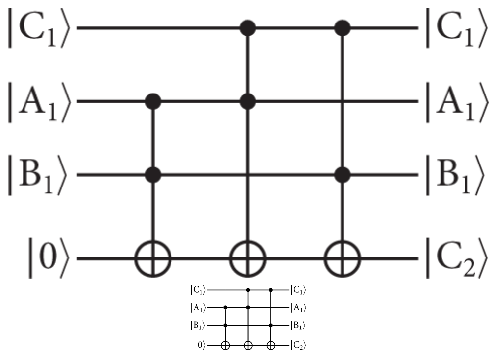
Figure 7.10. A circuit that computes the carry bit from a sum of three bits, created using the Quantikz LaTeX package.
