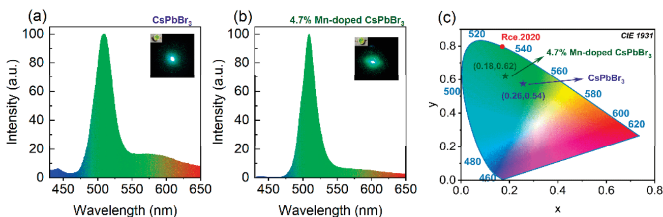
Figure 4. (a,b) Light-emitting diode (LED) emission spectra of the undoped and 4.7% Mn-doped \text{CsPbBr}_3 perovskite QDs. Insets: Optical images corresponding to the LED. (c) Chromaticity coordinates.
