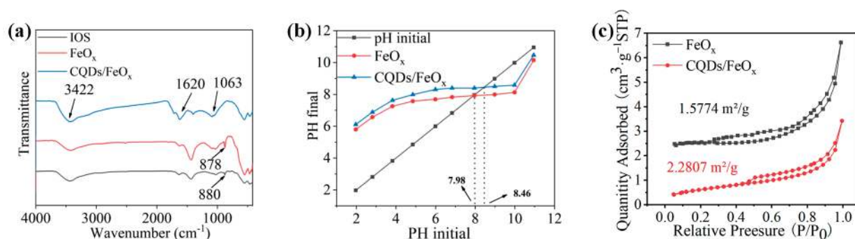
Figure 5. (a) IR spectra of IOS, FeO x powder and CQDs/FeO x composite; (b,c) The PZC value (b) and BET (c) of FeO x powder and CQDs/FeO x composite.
