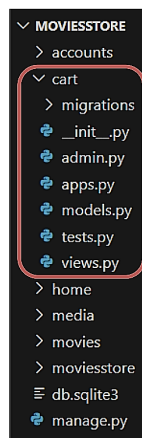
Figure 10.4 – The MOVIESSTORE project structure containing the cart app
