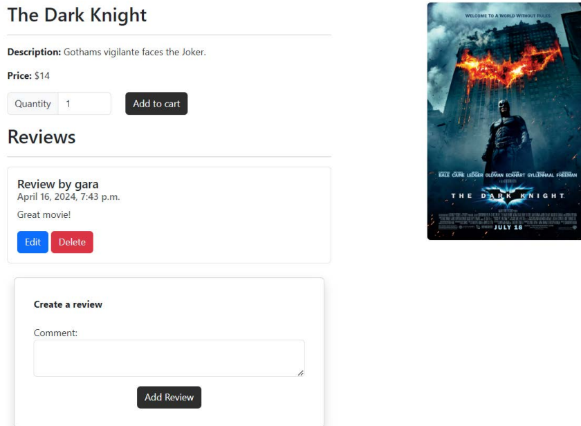
Figure 1.10 – A specific movie page with its reviews
