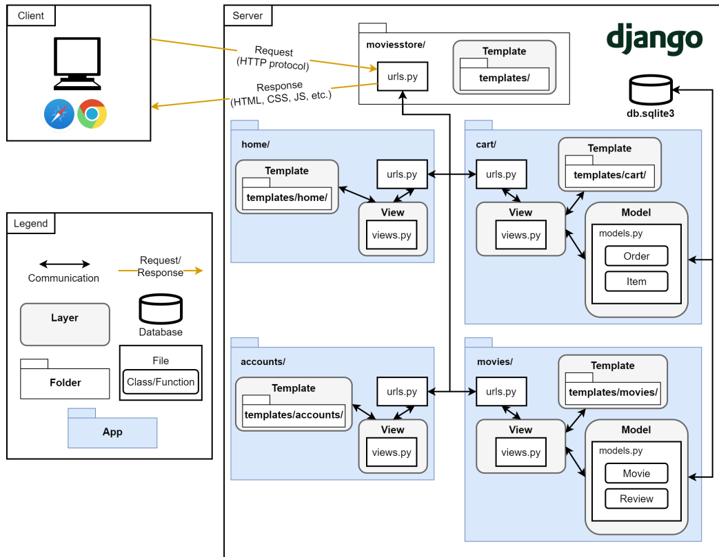
Figure 1.11 – The Movies Store software architecture diagram
