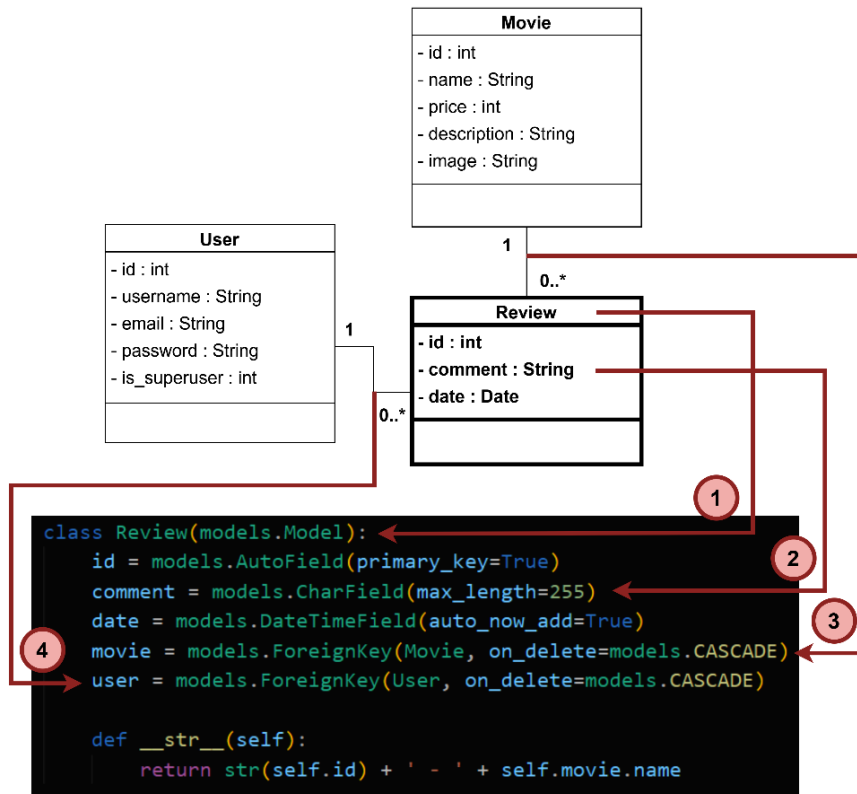
Figure 11.7 – Relationship between a class and a model
