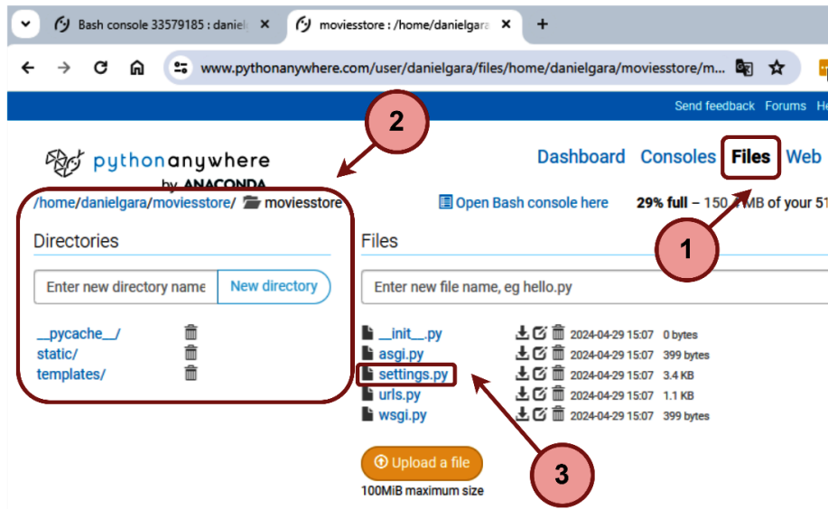
Figure 13.20 – Accessing the settings.py file
