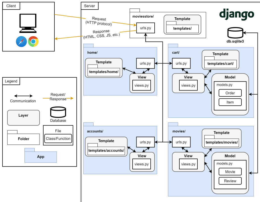
Figure 12.5 – Movies Store architecture
