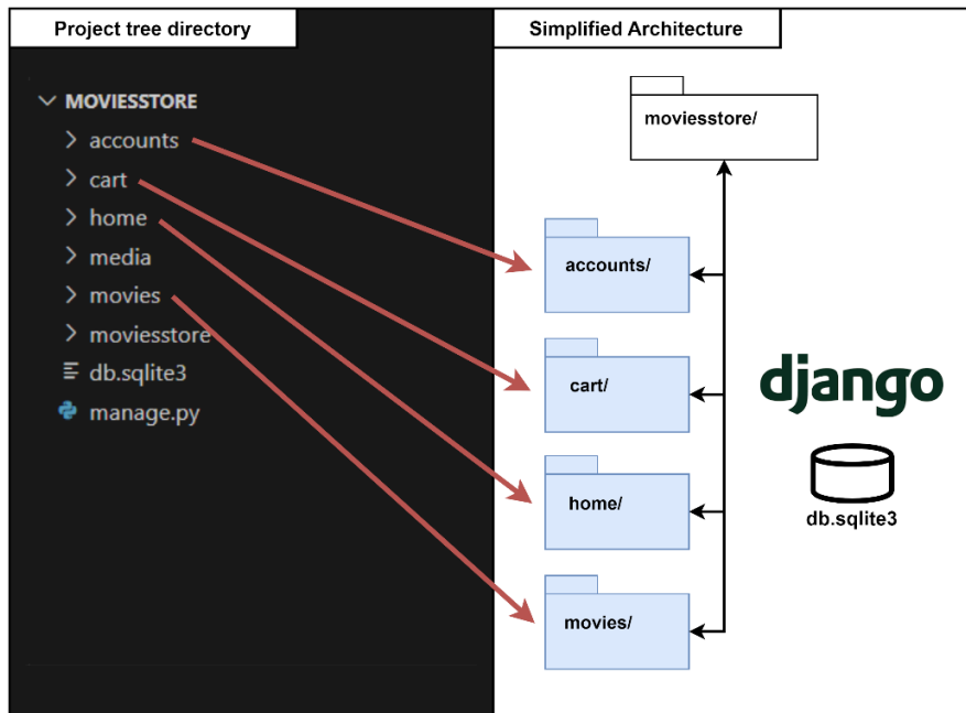
Figure 12.4 – Project tree directory compared with simplified architecture
