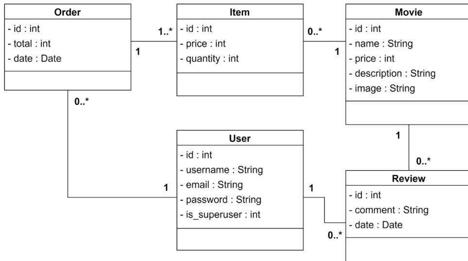
Figure 1.6 – The Movies Store class diagram
