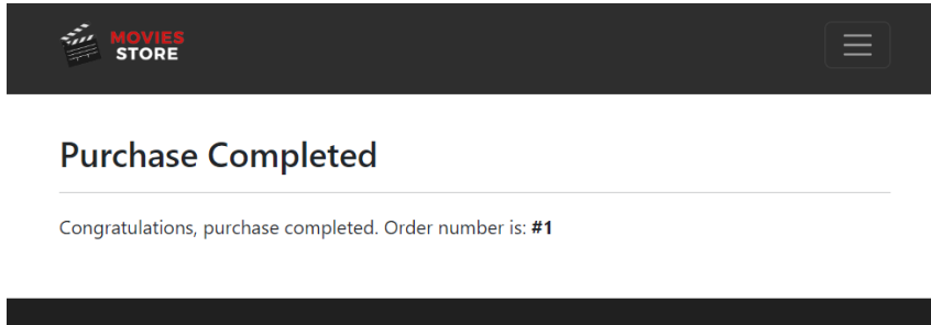
Figure 12.1 – Purchase page
