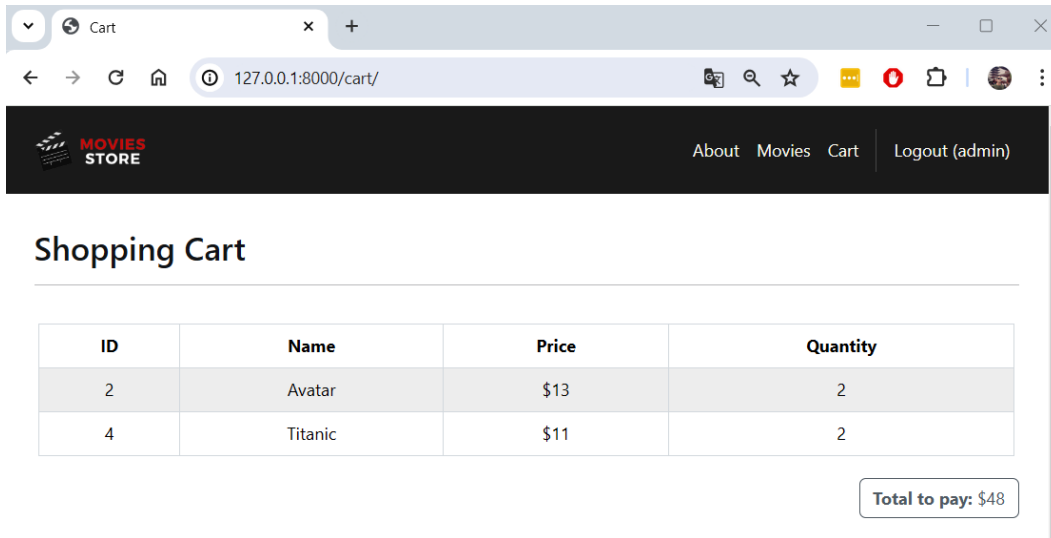
Figure 10.6 – The Cart page
