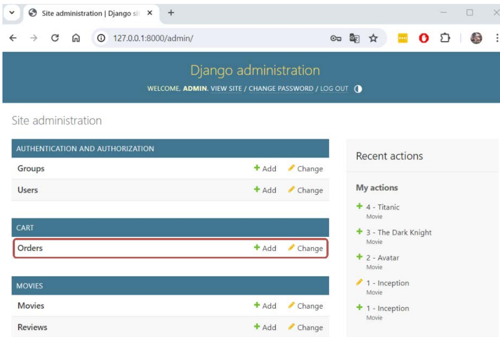
Figure 11.3 – Admin page with orders available
