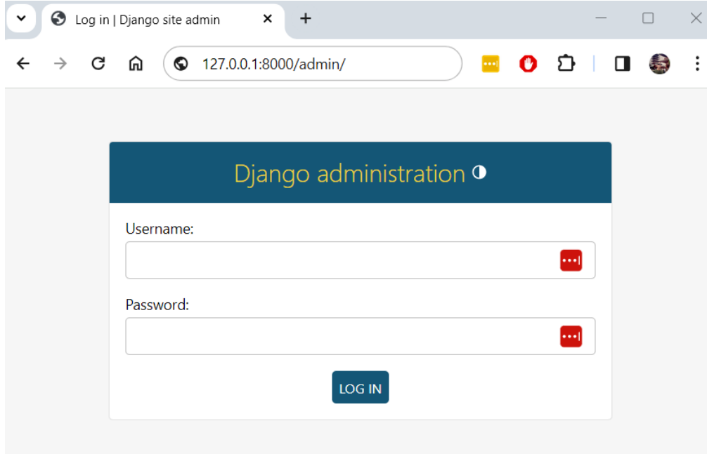
Figure 5.5 – Admin page
