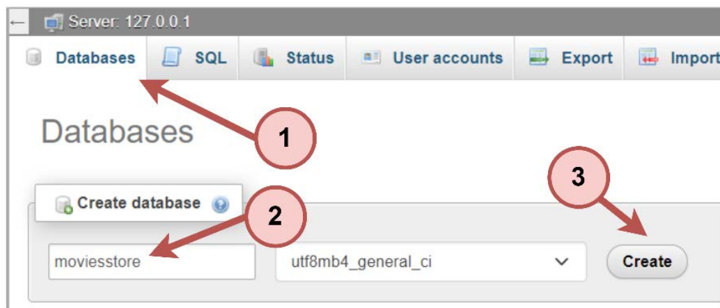
Figure 7.8 – Database creation
