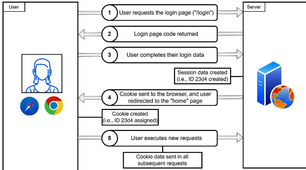
Figure 10.1 – An example of a Django session operation
