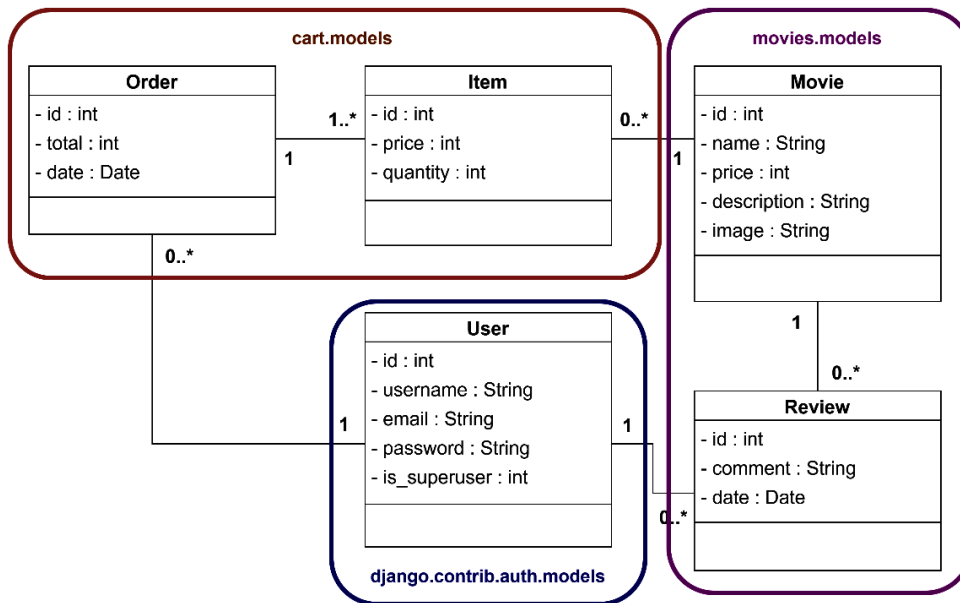
Figure 11.6 – Movies Store class diagram, highlighting model locations
