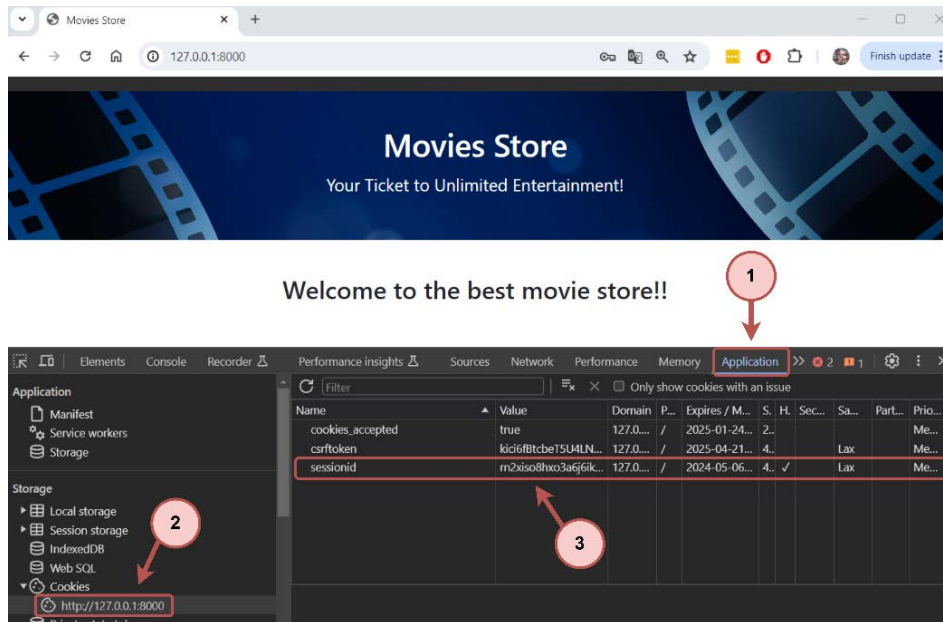
Figure 10.3 – The Movies Store cookie data
