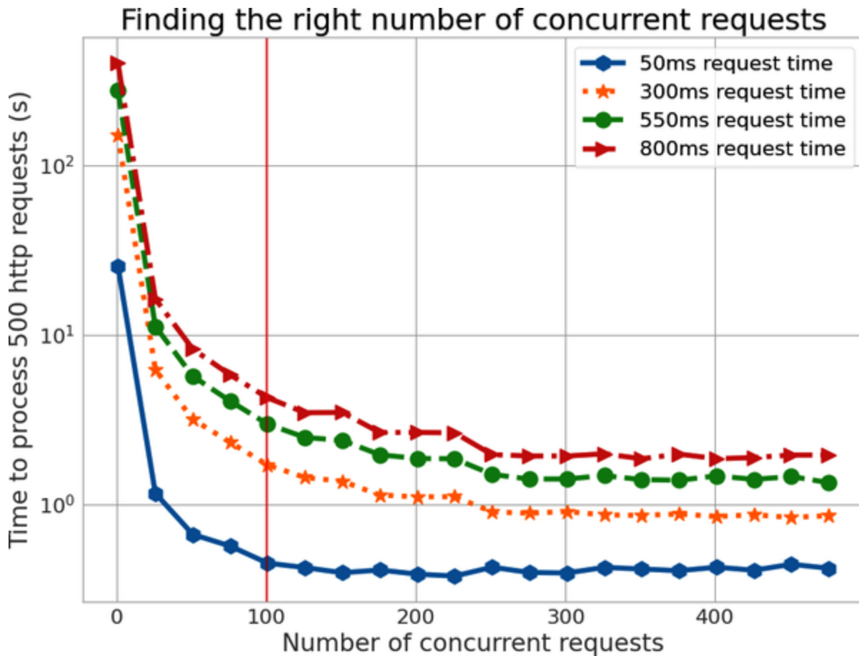
Figure 9-4. Experimenting with different numbers of concurrent requests for various request times
