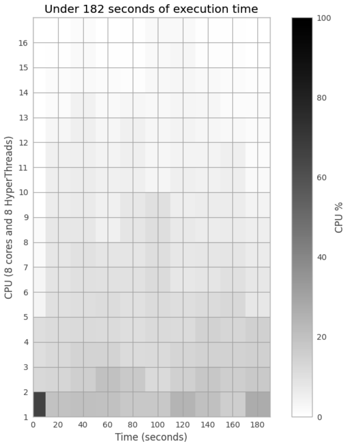
Figure 10-8. Estimating pi using Python objects and eight threads
