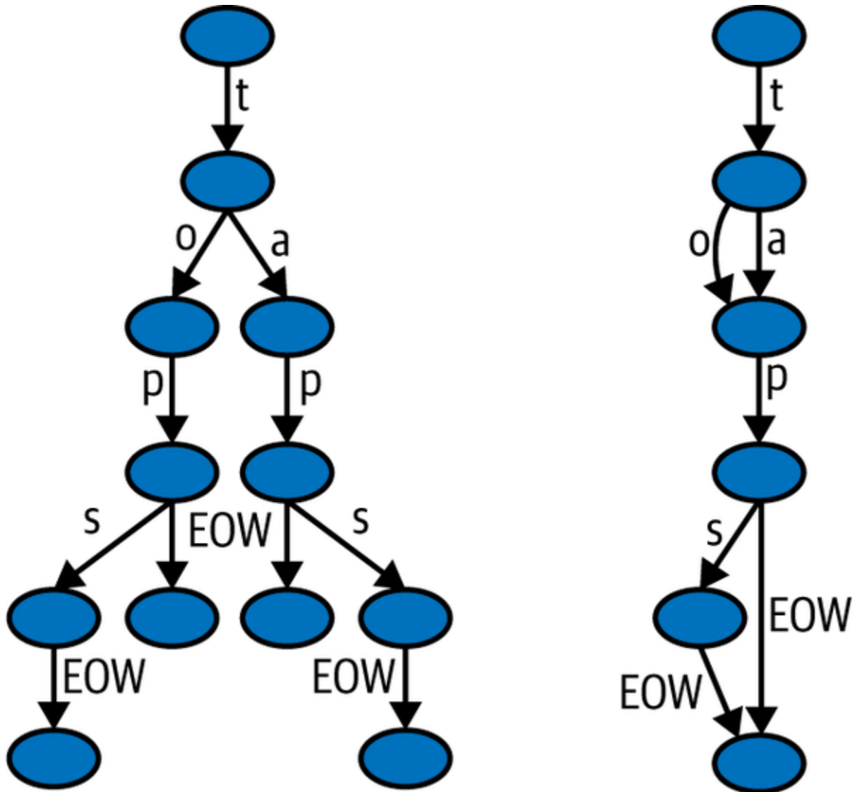
Figure 12-3. Trie and DAWG structures (image by Chkno [CC BY-SA 3.0])
