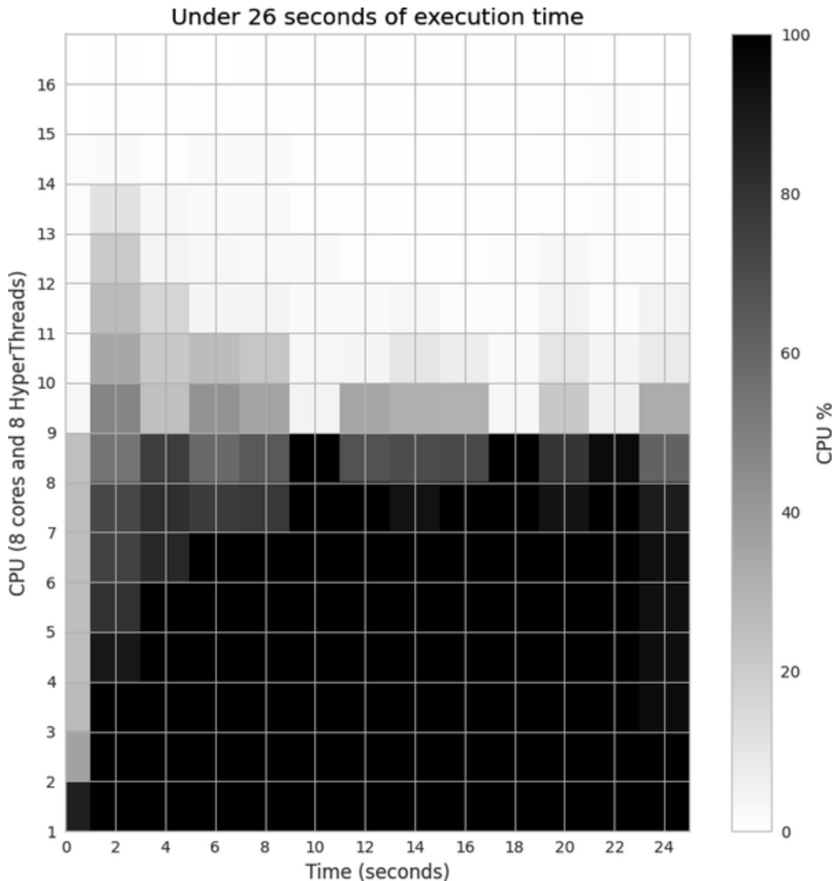
Figure 10-6. Estimating pi using Python objects and eight processes
