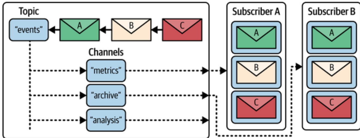
Figure 11-2. Overview of pub/sub-like topology
