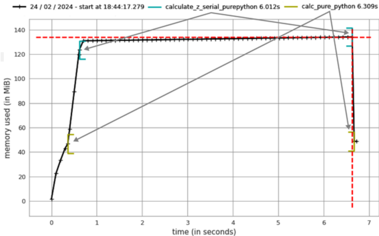
Figure 2-6. memory_profiler report using mprof
