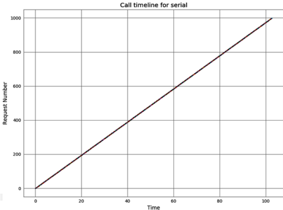
Figure 9-2. Request time for Example 9-4
