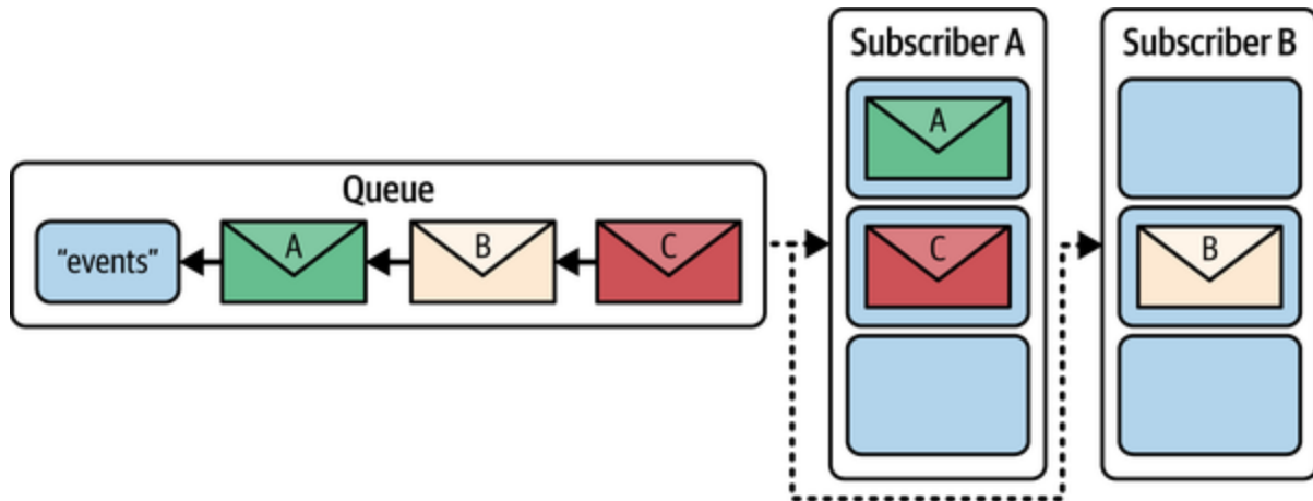
Figure 11-1. Overview of a Queue topology
