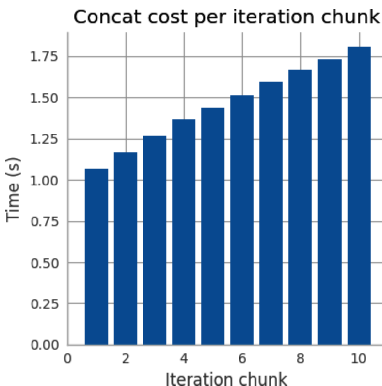
Figure 7-3. Iterative concatenation to a Series becomes increasingly slow
