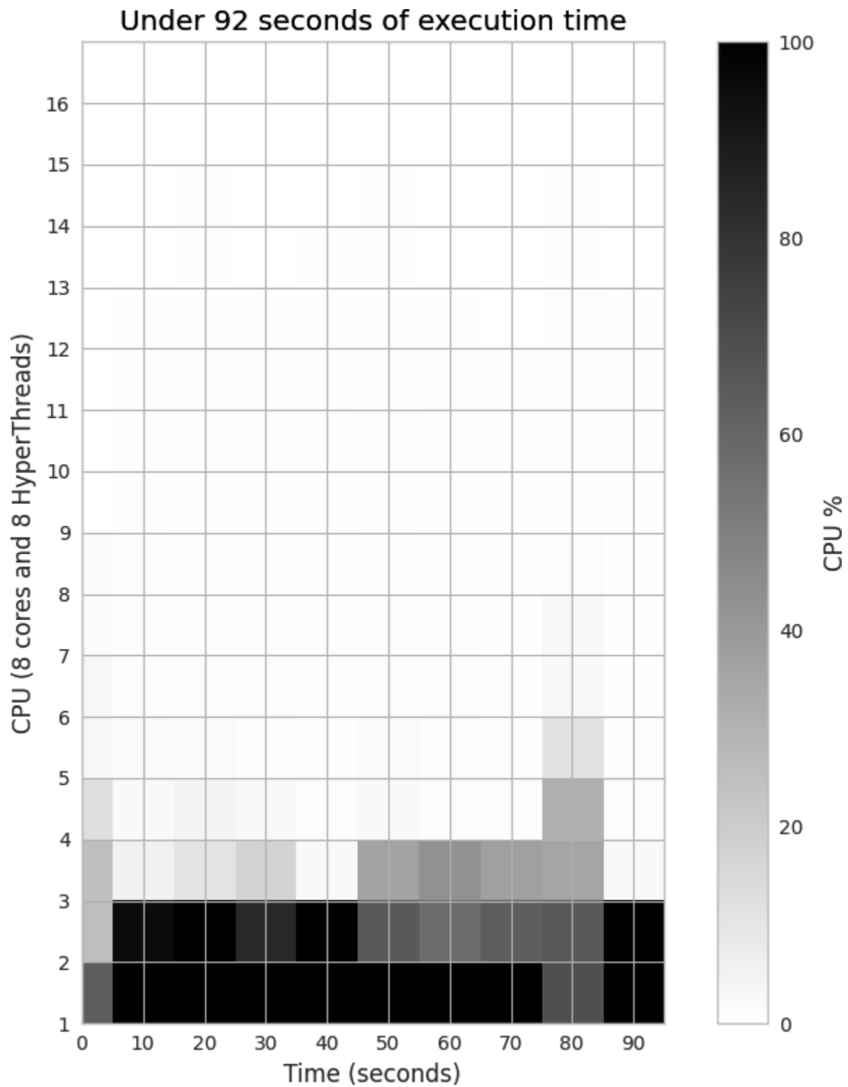
Figure 10-4. Estimating pi using Python objects and two processes
