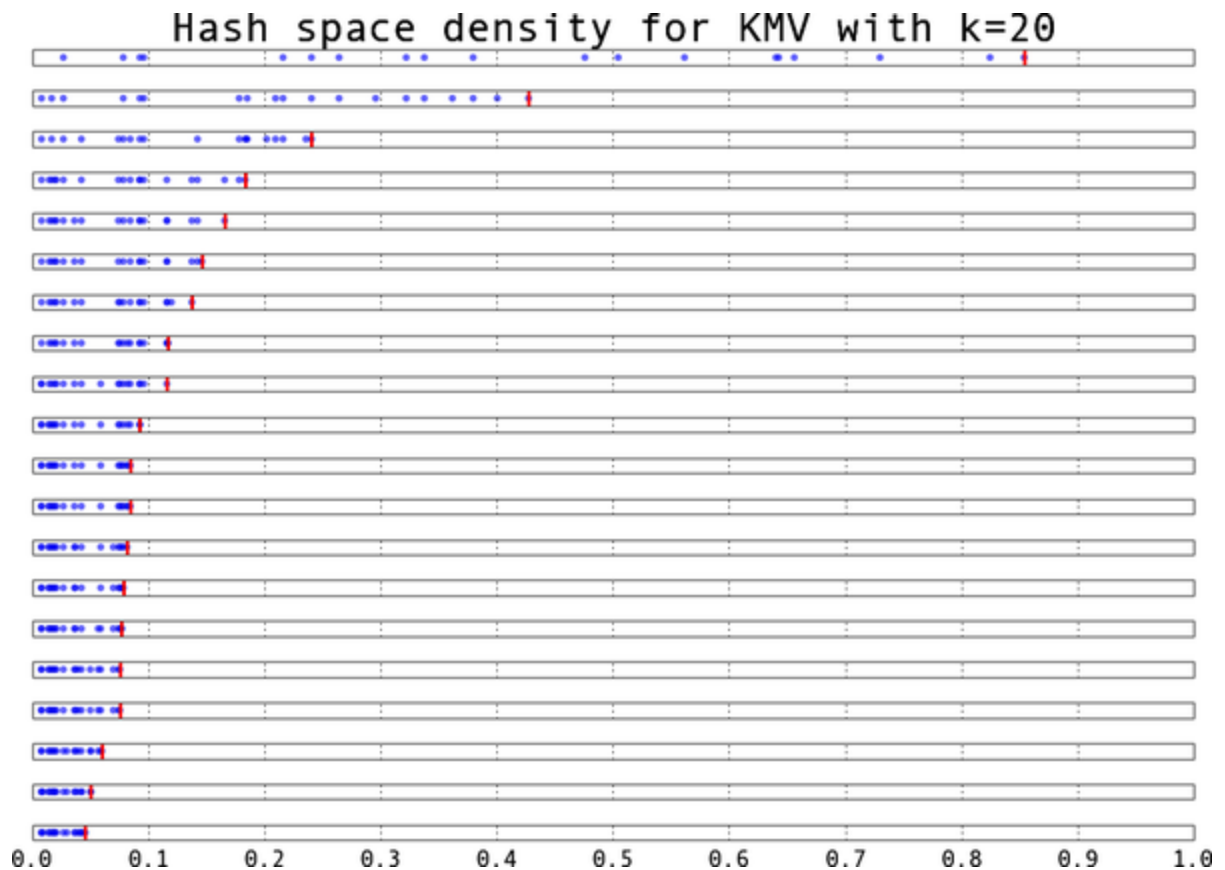
Figure 12-8. The value stores in a KMV as more elements are added
