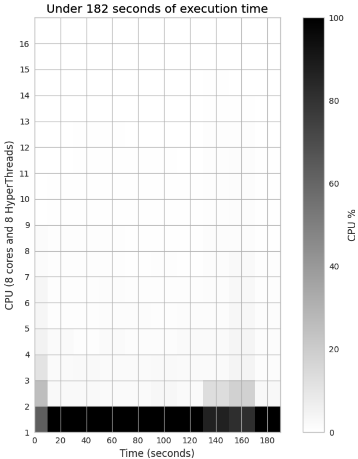
Figure 10-3. Estimating pi using Python objects and one process
