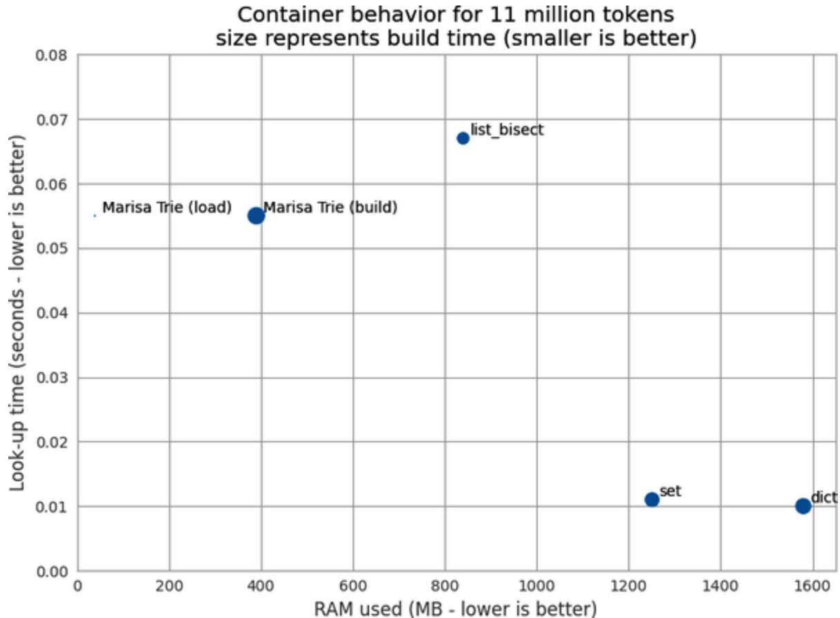
Figure 12-2. Trie versus set , list , and dict containers
