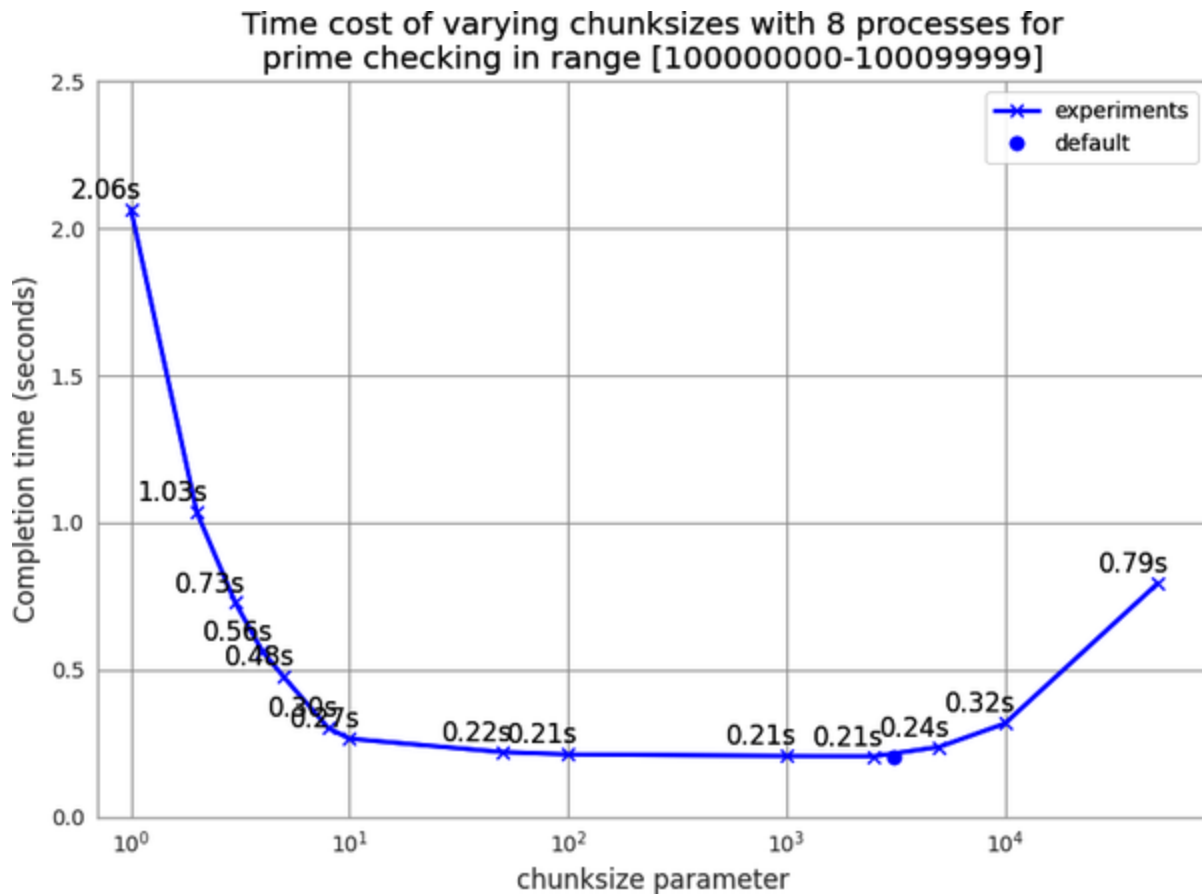
Figure 10-12. Choosing a sensible chunksize value (continued)
