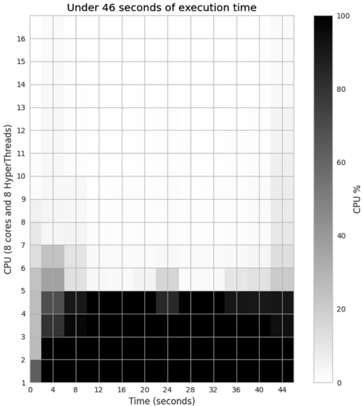
Figure 10-5. Estimating pi using Python objects and four processes
