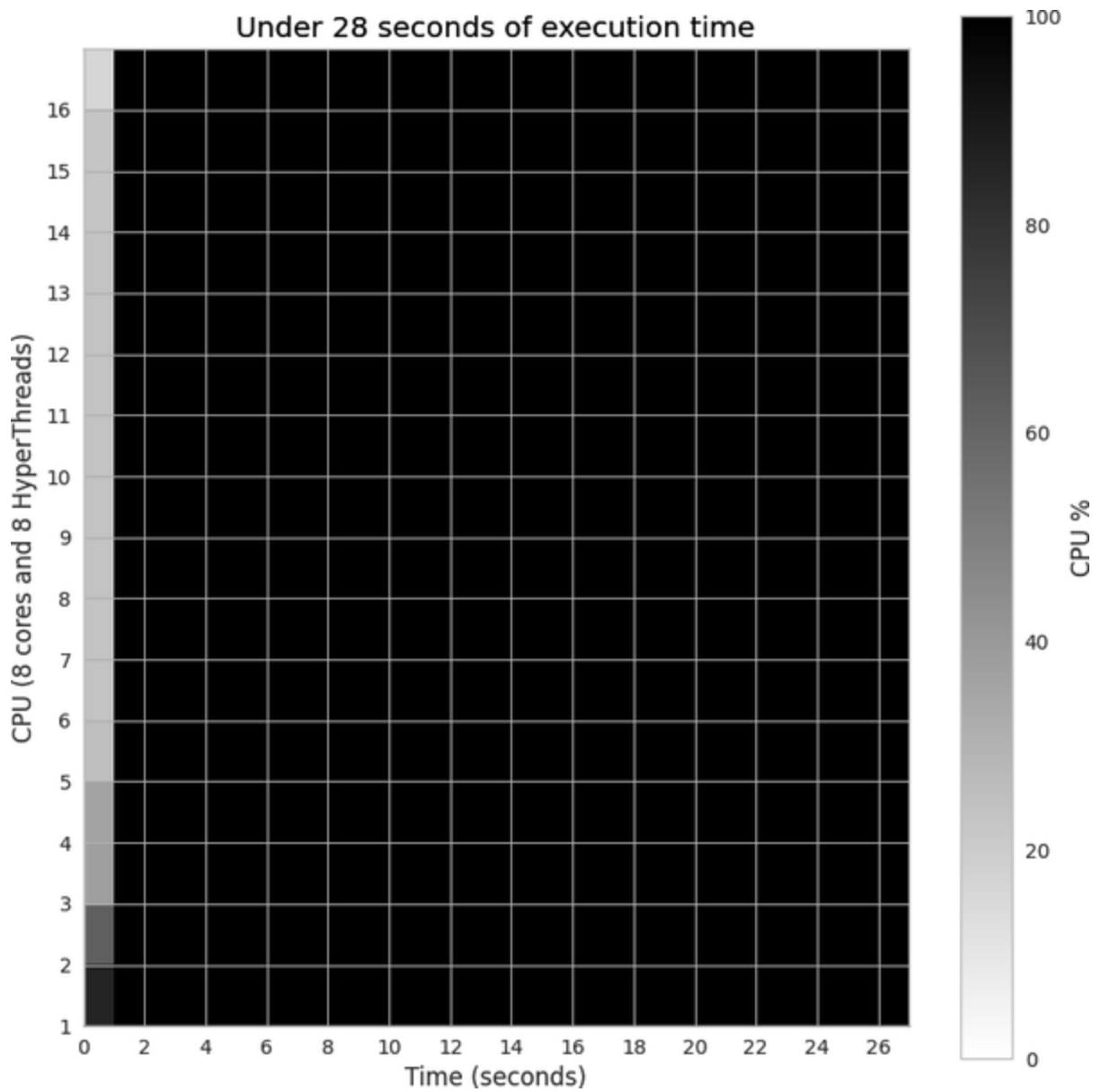
Figure 10-7. Estimating pi using Python objects and sixteen processes, with little additional gain
