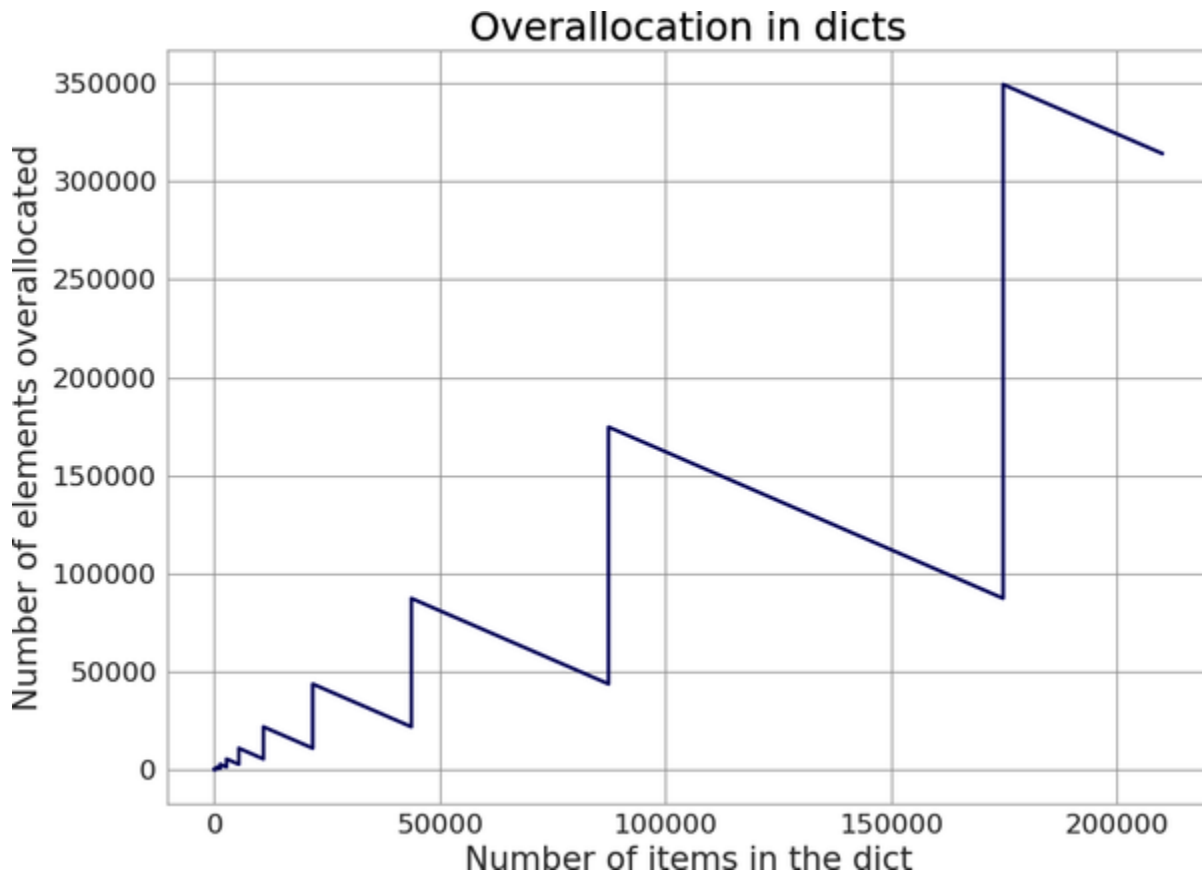
Figure 4-2. Graph showing how many extra elements are being allocated to accommodate a dictionary of a given size. Dictionaries will always be at least one-third empty but will also have even more space allocated to make sure the total size is a power of two. The graph looks similar for sets; however, the rate of increase changes at the 50,000-element mark.
