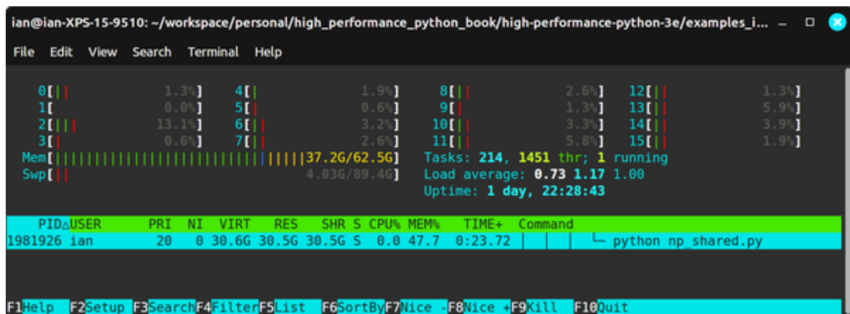
Figure 10-19. htop showing RAM and swap usage
