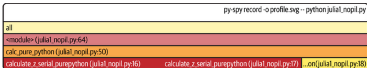
Figure 2-11. Part of a flame chart for PySpy
