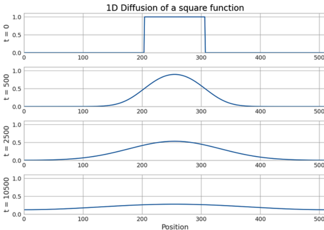
Figure 6-1. Example of 1D diffusion
