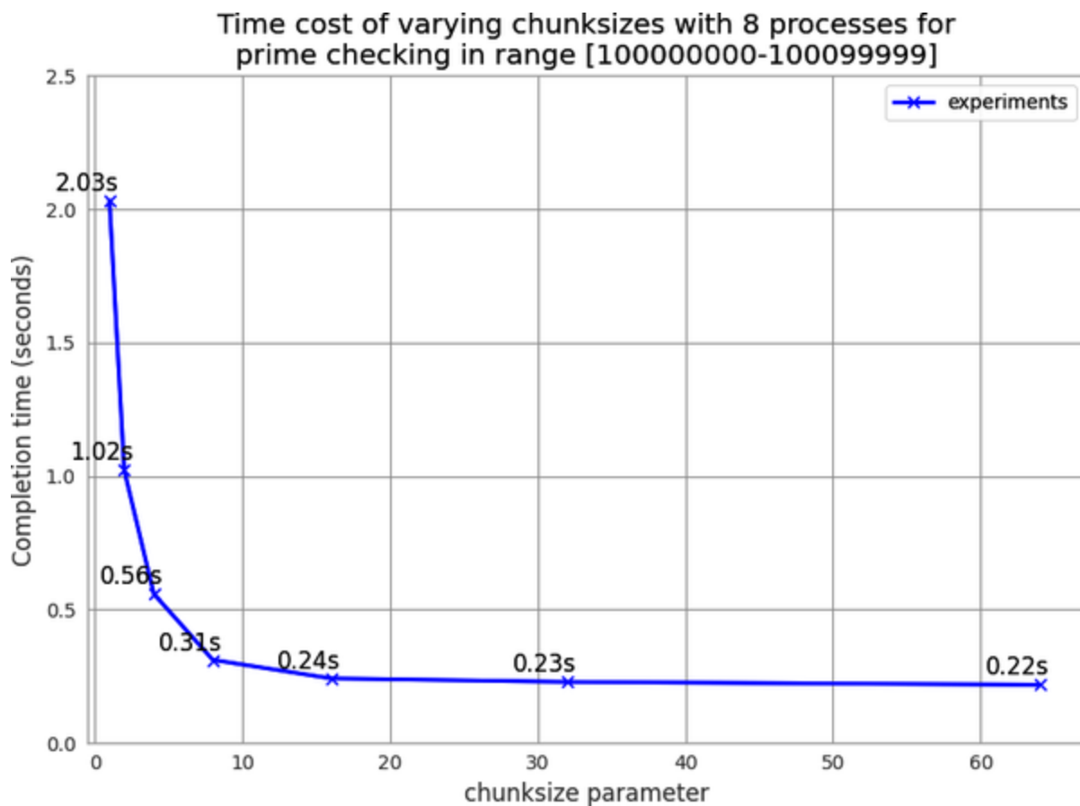
Figure 10-11. Choosing a sensible chunksize value
