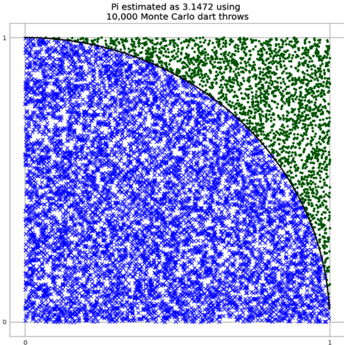
Figure 10-1. Estimating pi using the Monte Carlo method
