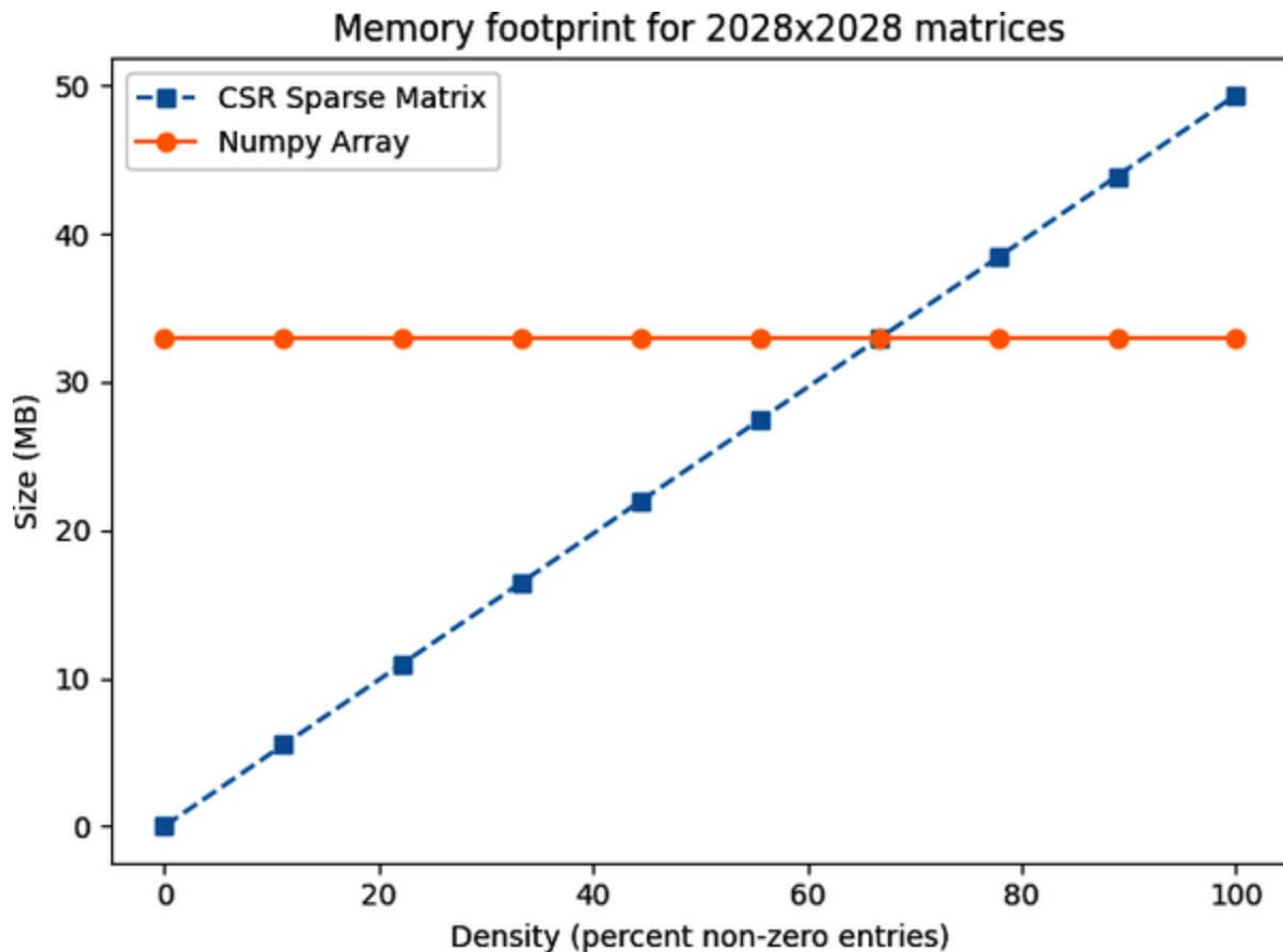
Figure 12-6. Sparse versus dense memory footprint
