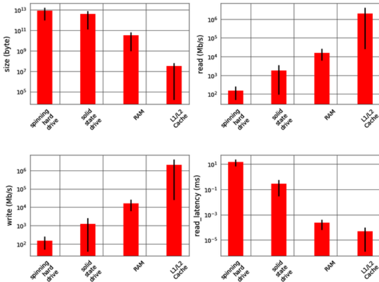
Figure 1-2. Characteristic values for different types of memory units 3
