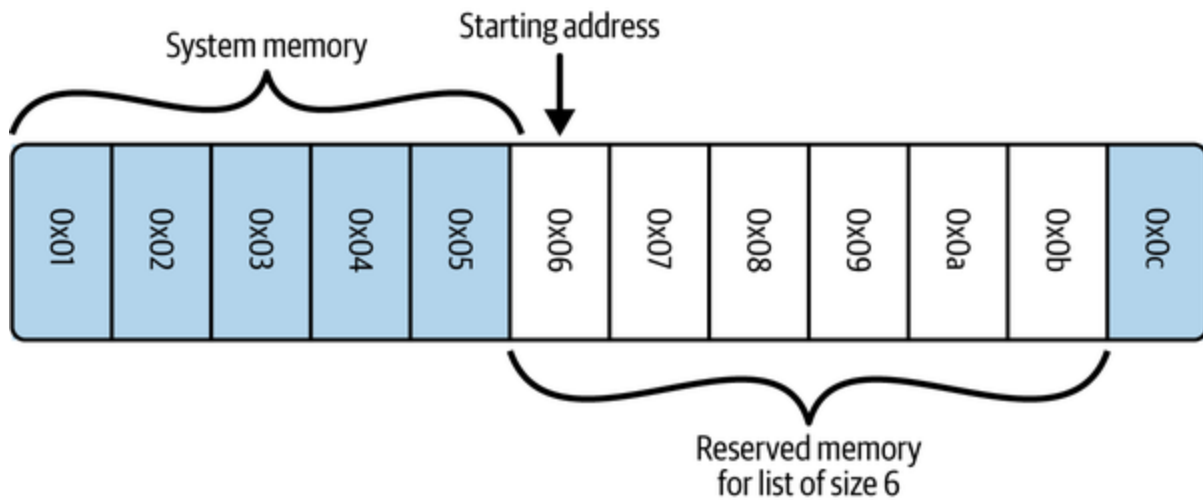
Figure 3-1. Example of system memory layout for an array of size 6
