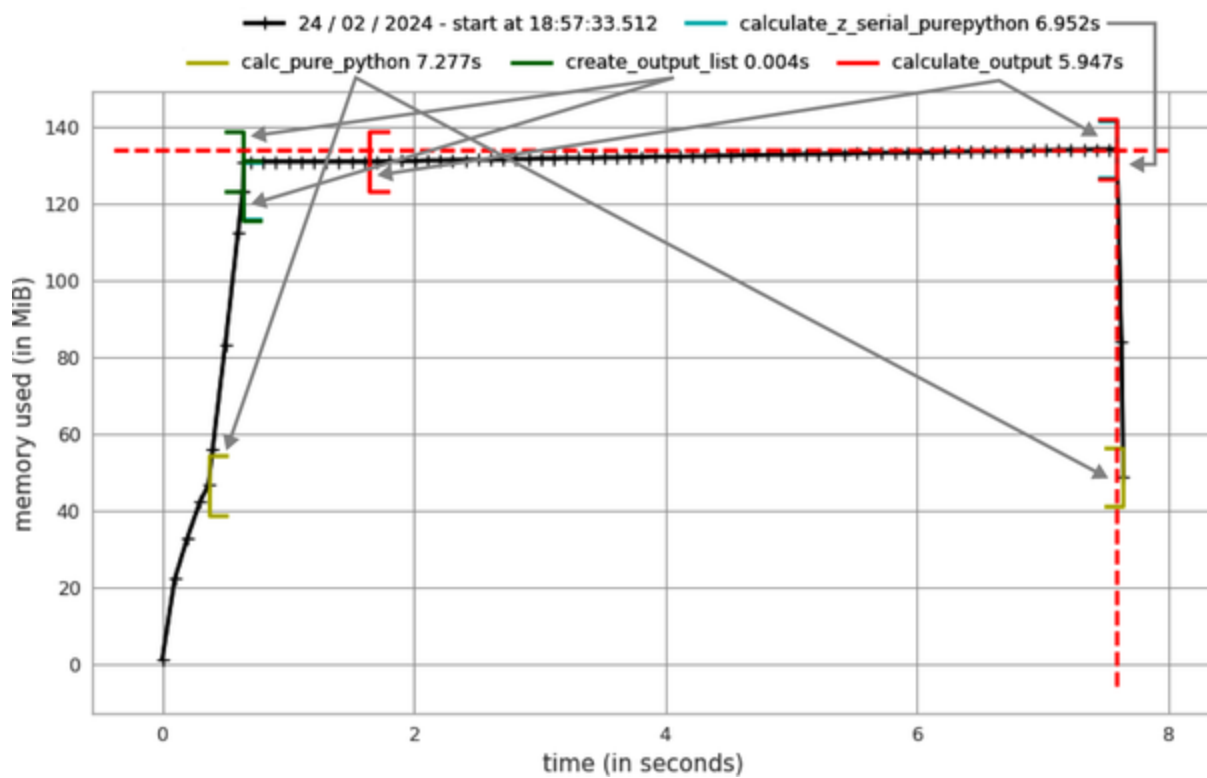
Figure 2-7. memory_profiler report using mprof with labels
