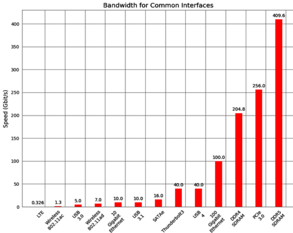
Figure 1-3. Connection speeds of various common interfaces 4
