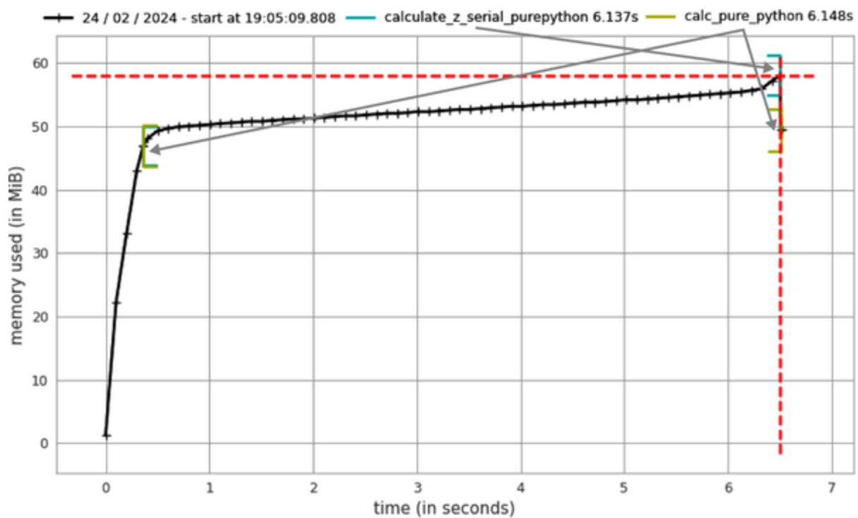
Figure 2-8. memory_profiler after removing two large lists
