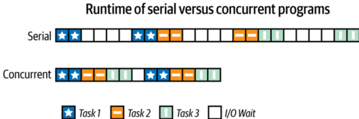
Figure 9-1. Comparison of serial and concurrent programs
