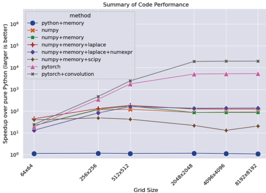
Figure 6-8. Summary of speedups from the methods attempted in this chapter
