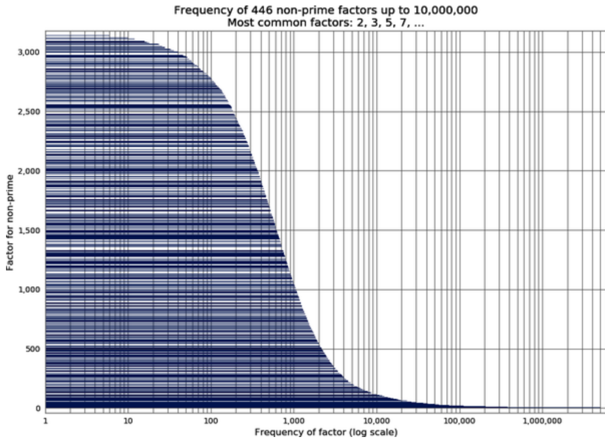
Figure 10-16. The frequency of factors of nonprimes
