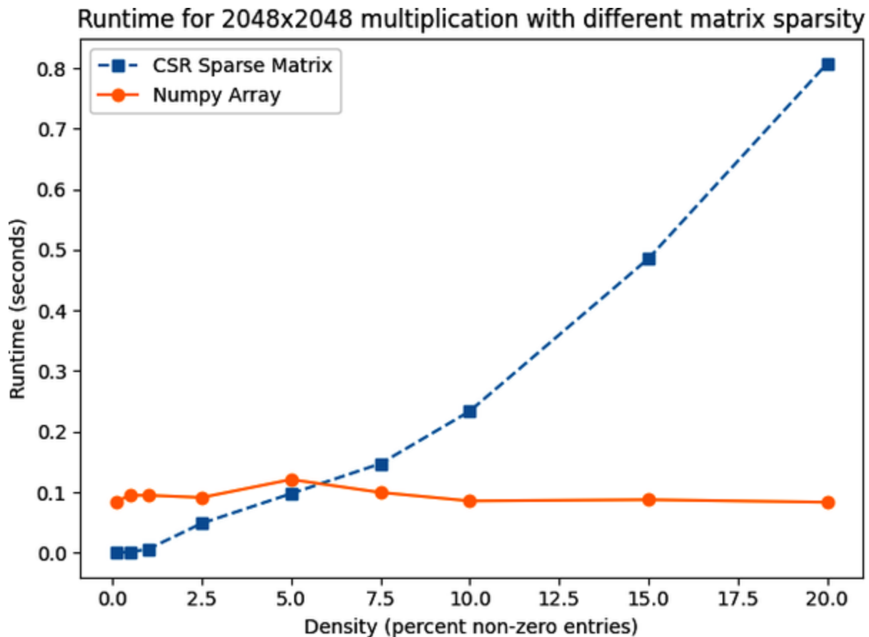
Figure 12-5. Sparse versus dense matrix multiplication
