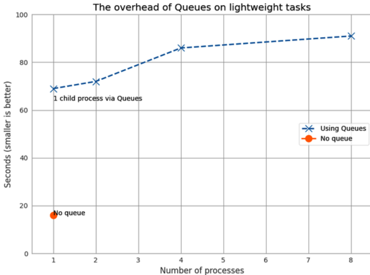
Figure 10-15. Cost of using Queue objects
