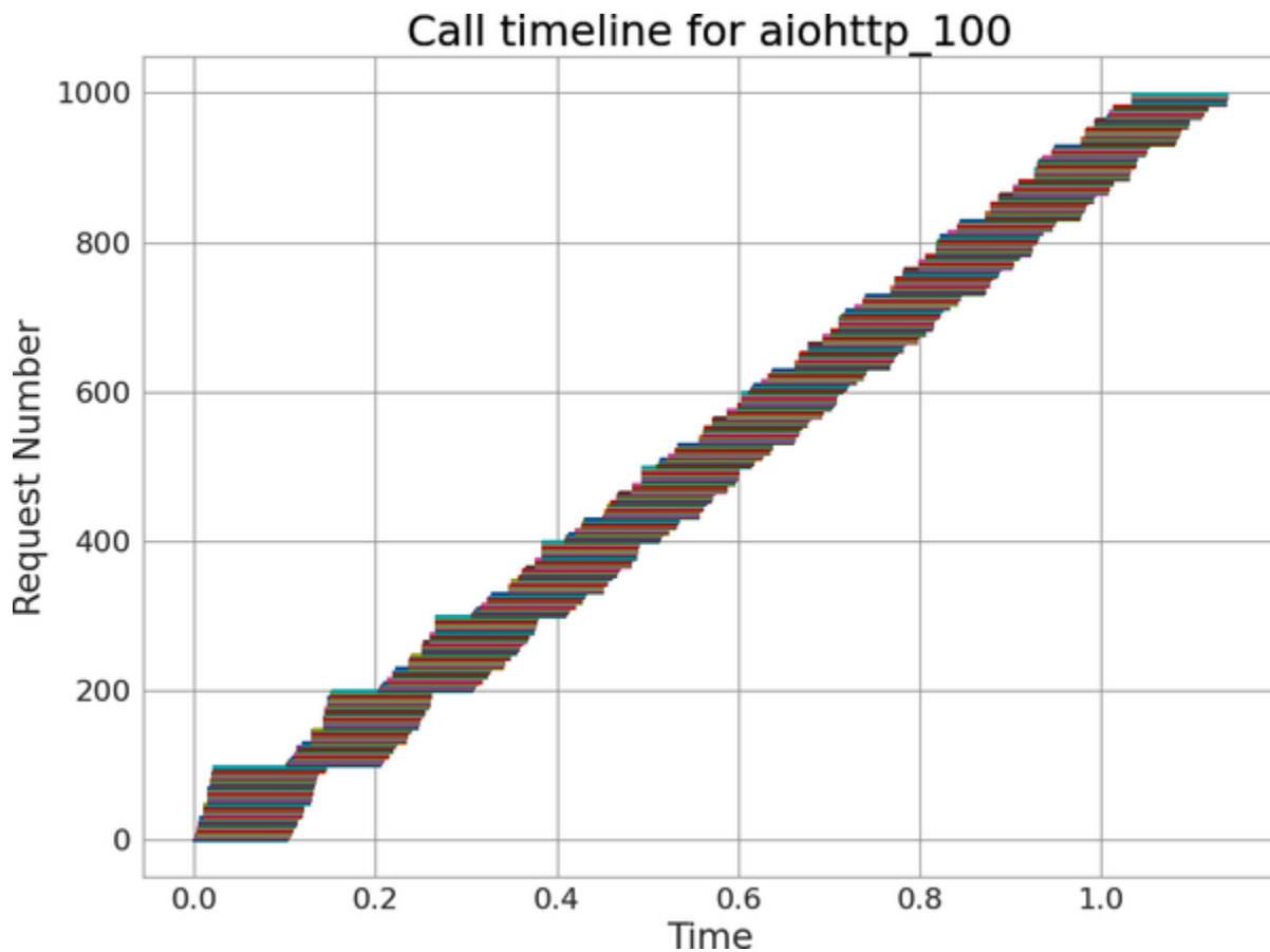
Figure 9-3. Chronology of HTTP requests for Example 9-5
