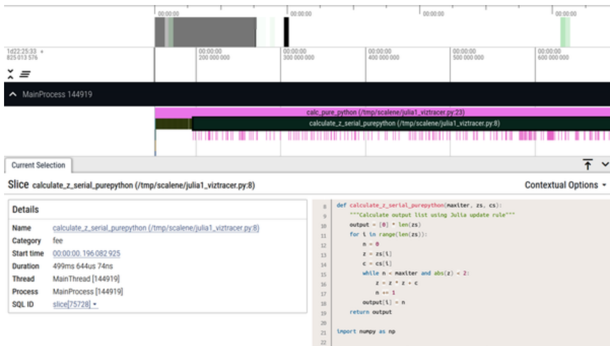
Figure 2-12. Overview of the Julia execution laid out through time
