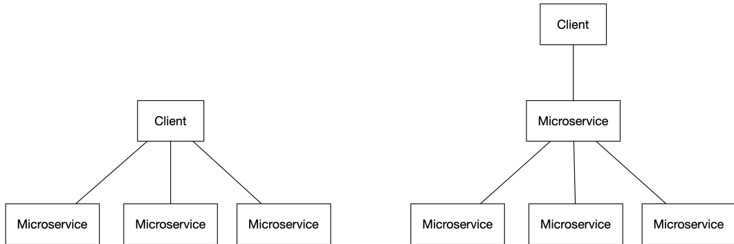
Figure 3.3. Architecture Without and With Service Aggregation
