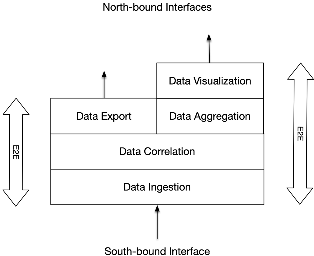
Figure 6.20. Telecom Network Analytics Software System
