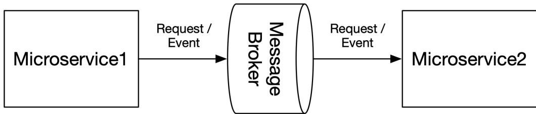
Figure 3.23. Request-Only Asynchronous Communication Method
