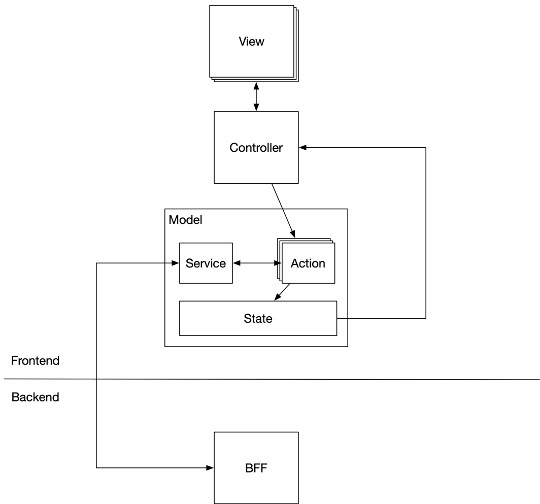
Figure 4.83. Frontend MVC Architecture with Redux
