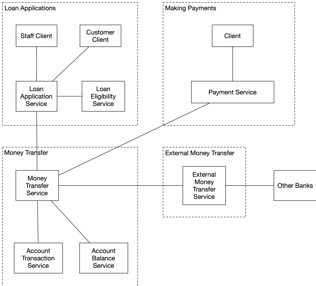
Figure 3.33. Banking Software System Bounded Contexts
