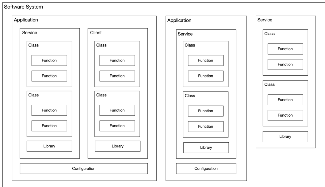
Figure 3.1. Software Hierarchy
