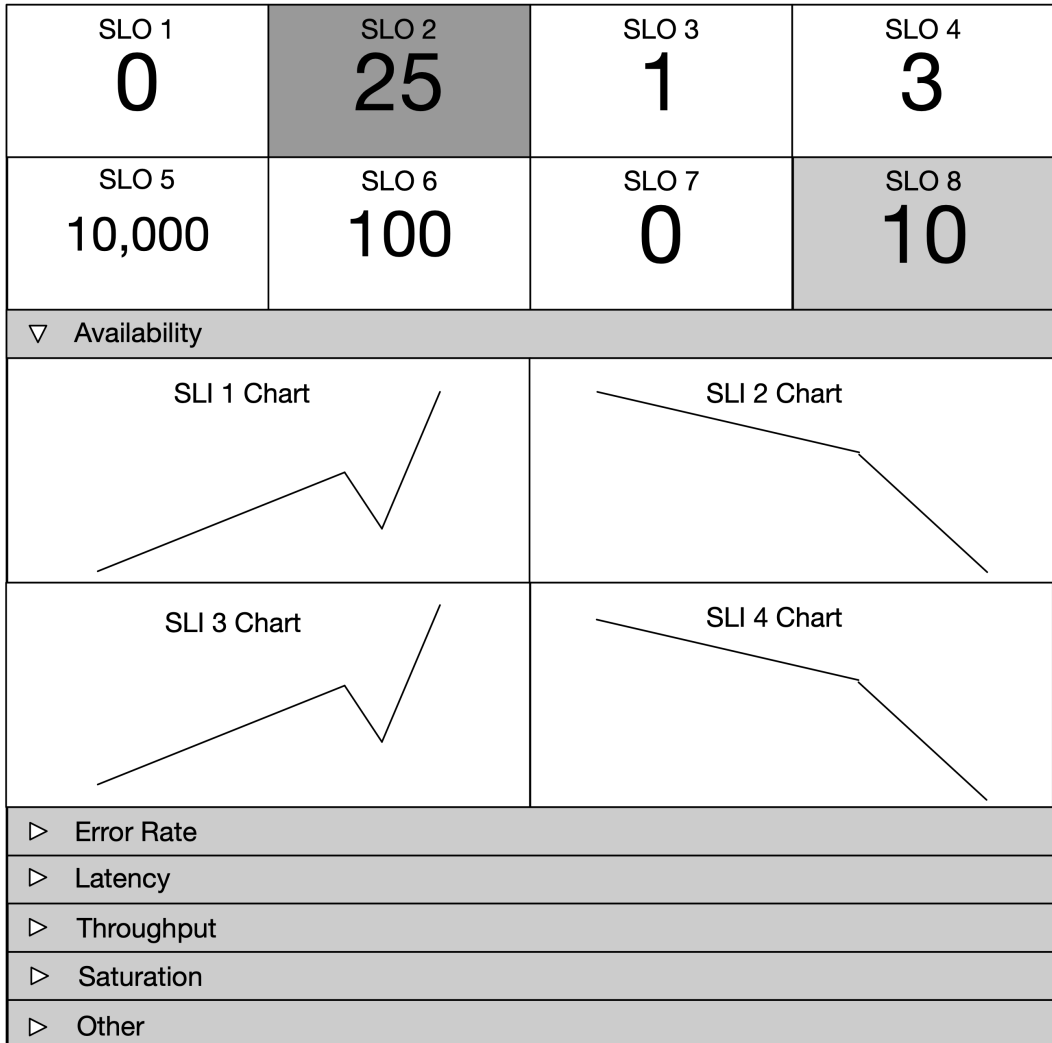
Figure 12.3. DevSecOps Diagram
