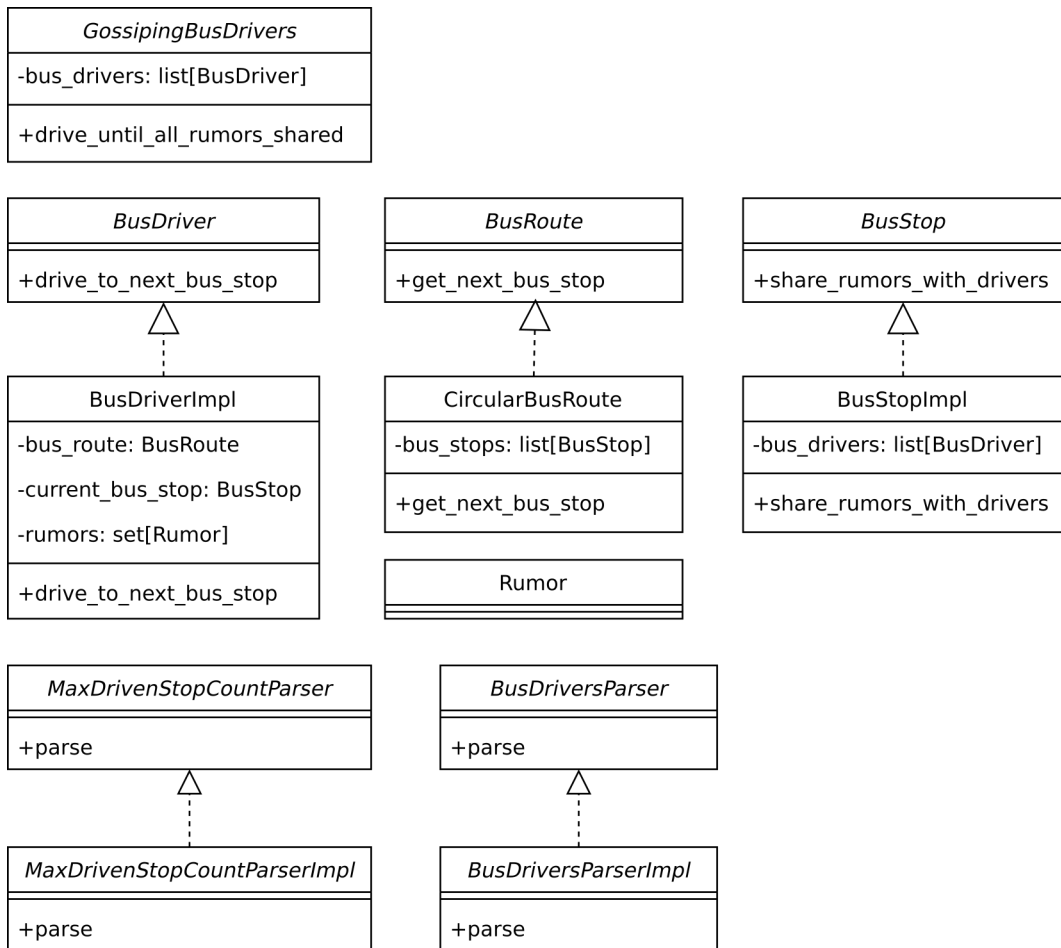
Figure 6.8. Class diagram with interfaces
