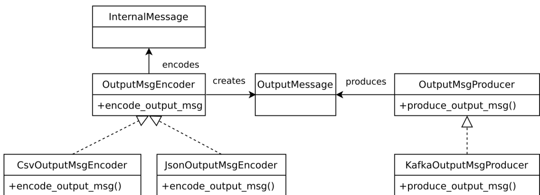
Figure 4.25. Output Subdomain Class Diagram
