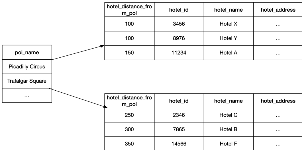
Figure 9.9. hotels_by_poi Table
