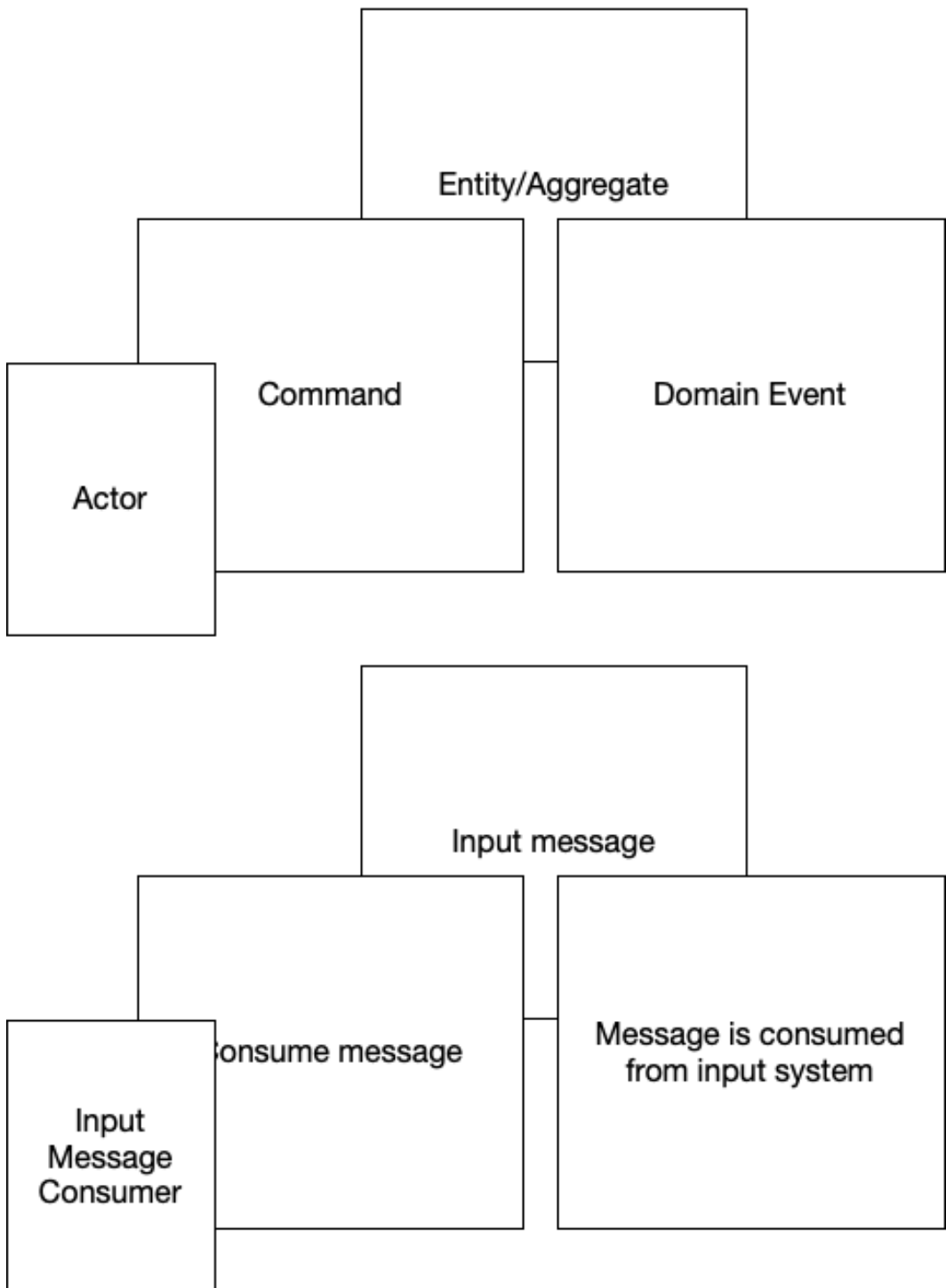
Figure 4.19. Event Storming
