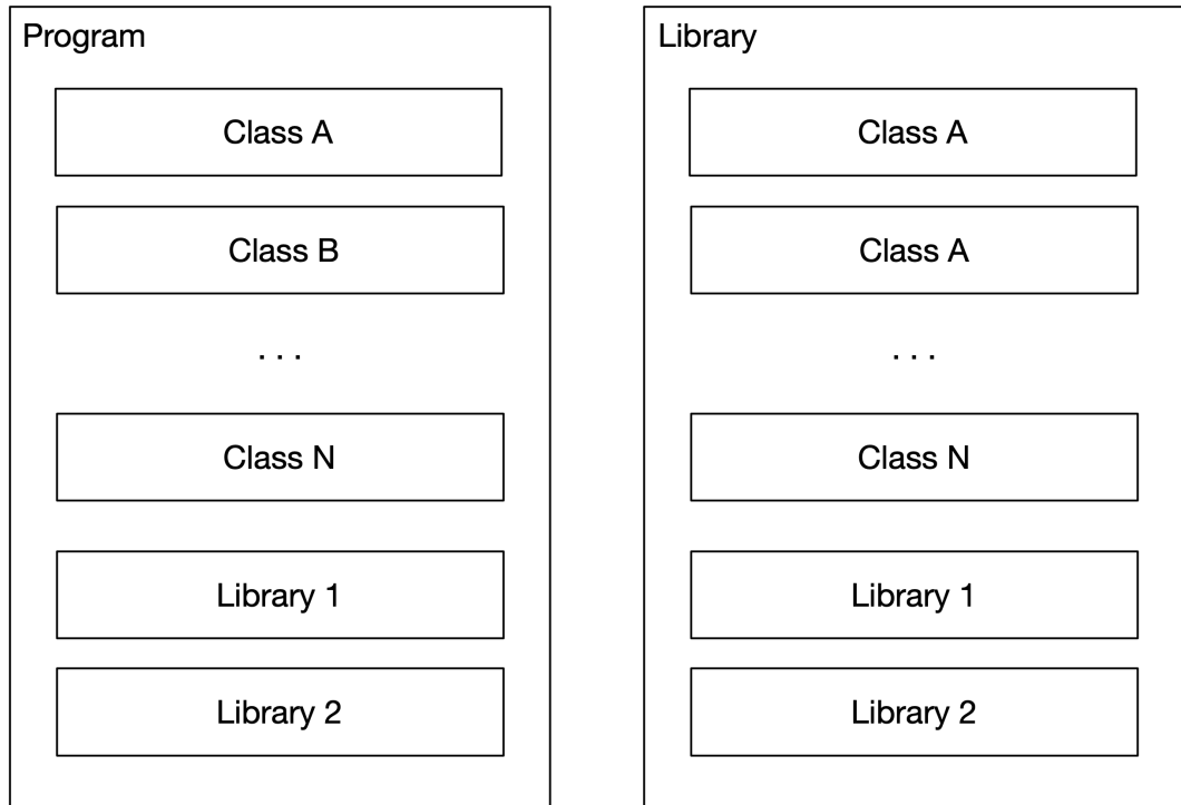
Figure 3.2. Software Components
