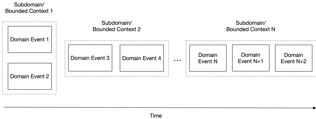
Figure 3.30. Event storming
