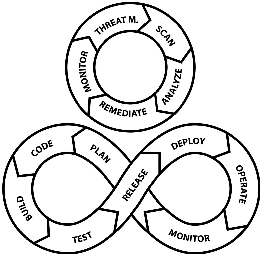
Figure 12.1. DevSecOps Diagram
