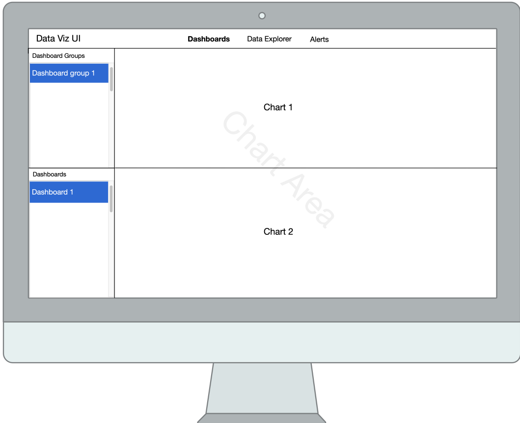
Figure 5.1. Dashboards Page
