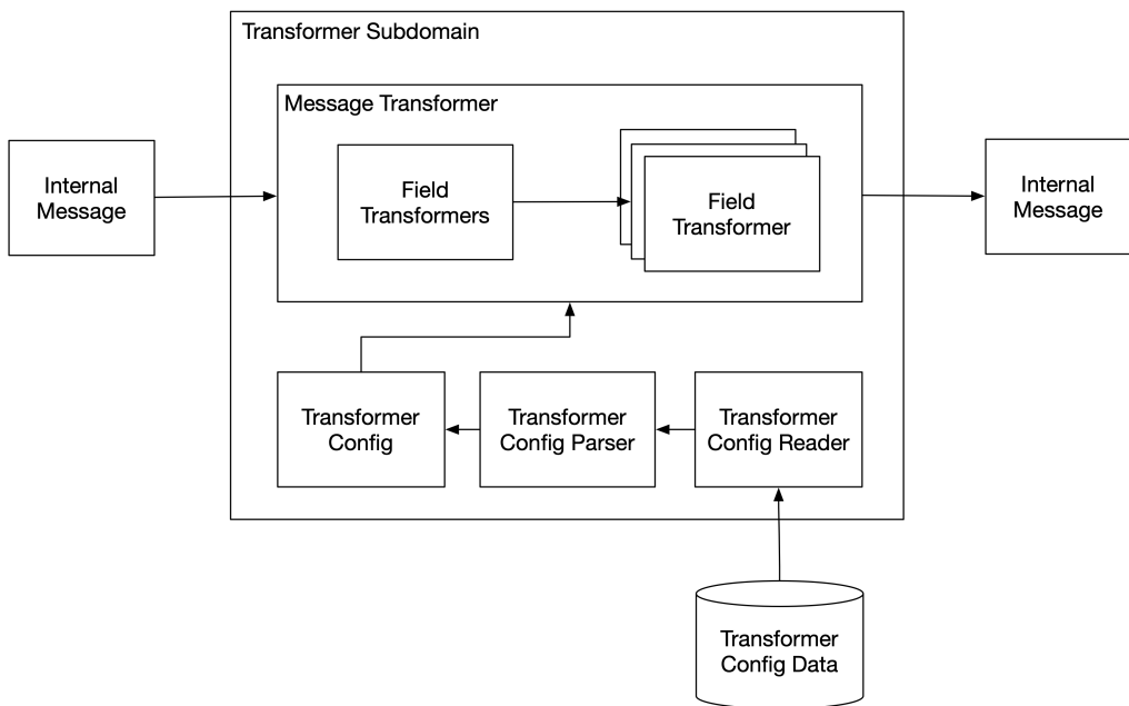
Figure 4.22. Transform Subdomain
