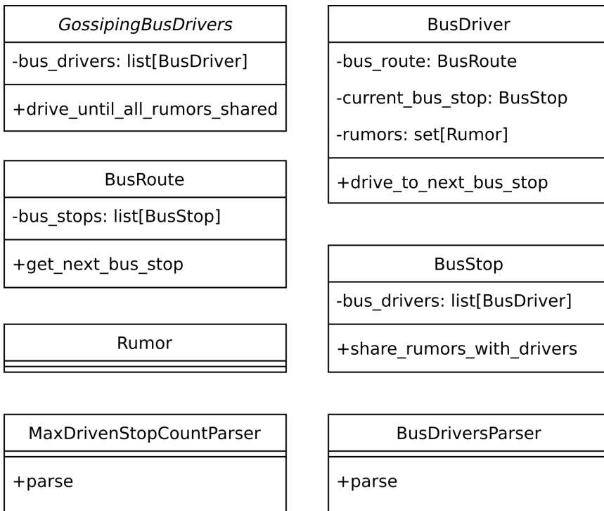
Figure 6.7. Class diagram
