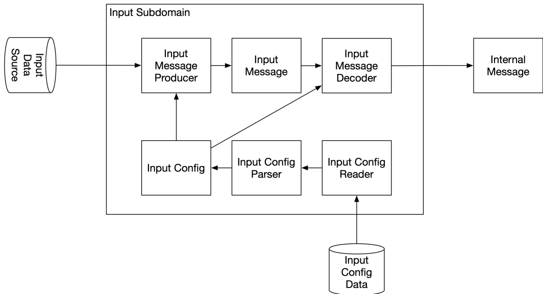
Figure 4.20. Input Subdomain
