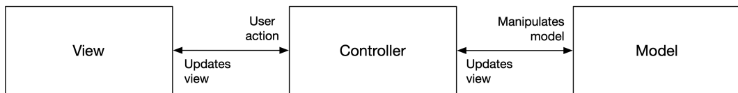
Figure 4.46. Model-View-Controller
