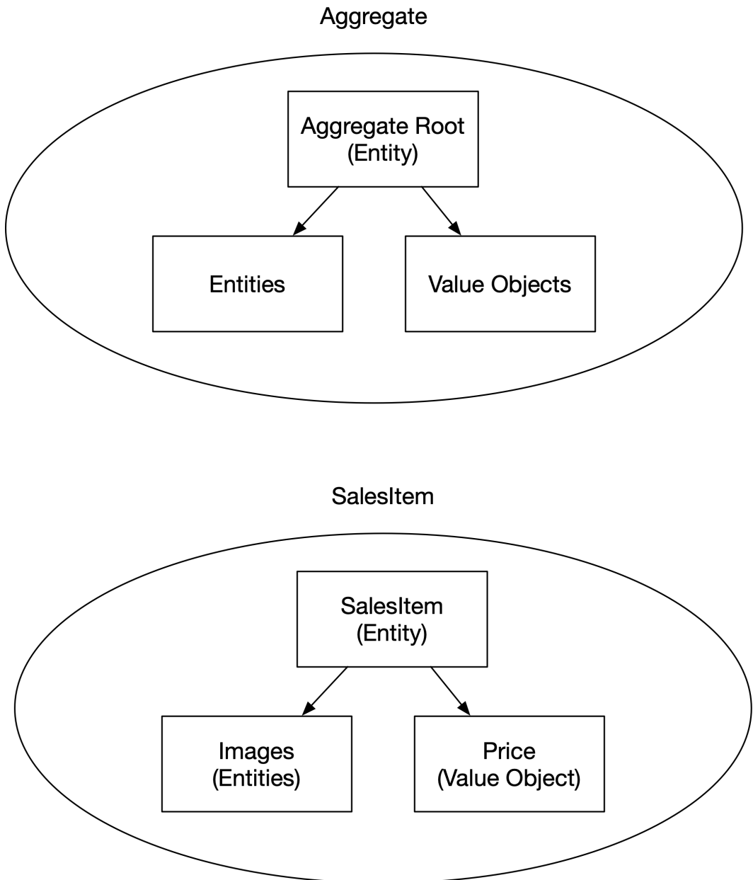
Figure 4.17. Aggregate Example
