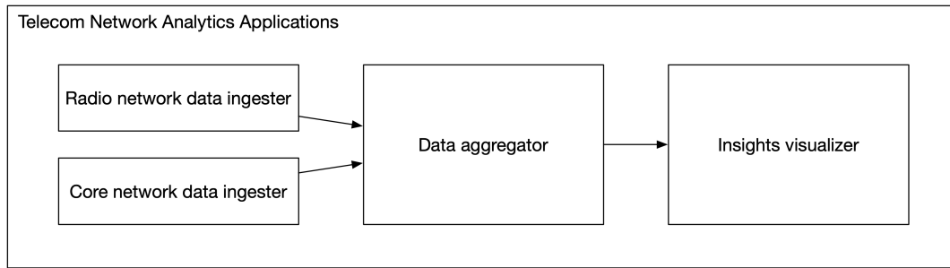
Figure 3.27. Applications
