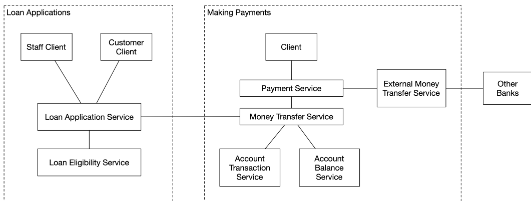
Figure 3.32. Banking Software System Bounded Contexts
