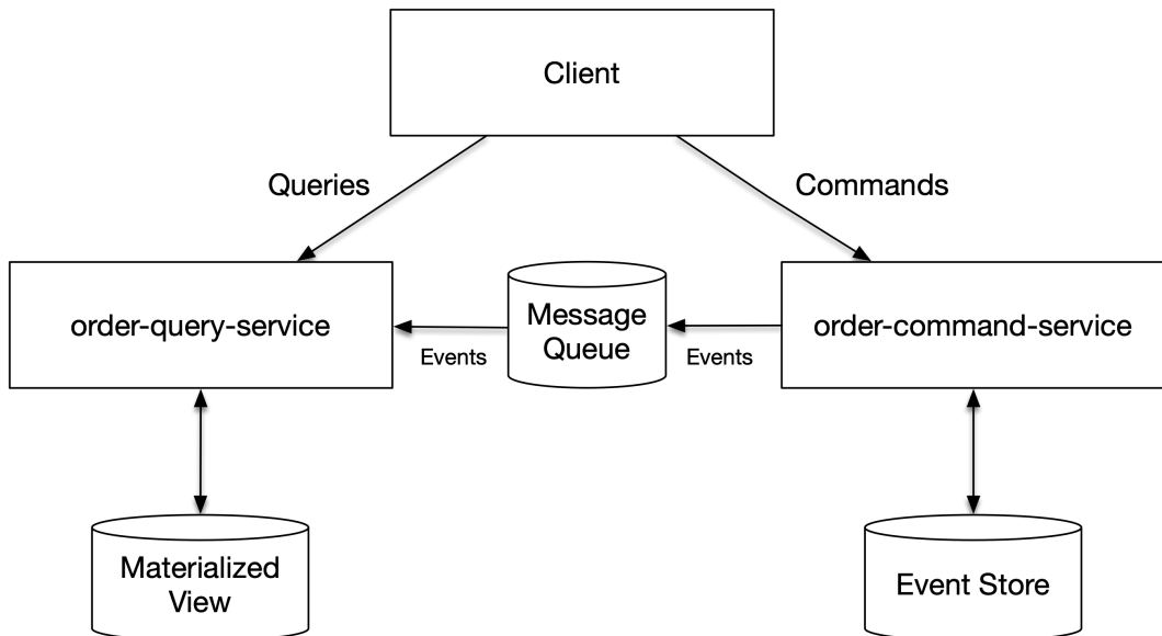
Figure 3.38. Order Services using CQRS
