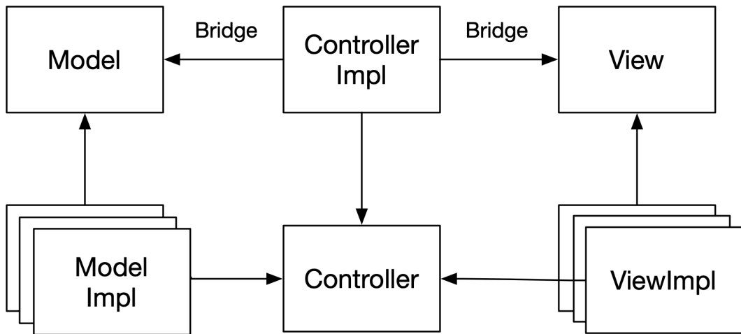
Figure 4.47. Dependencies in MVC pattern
