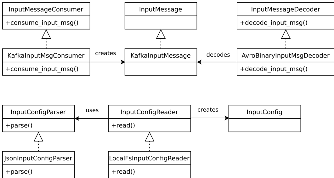
Figure 4.21. Input Subdomain Class Diagram
