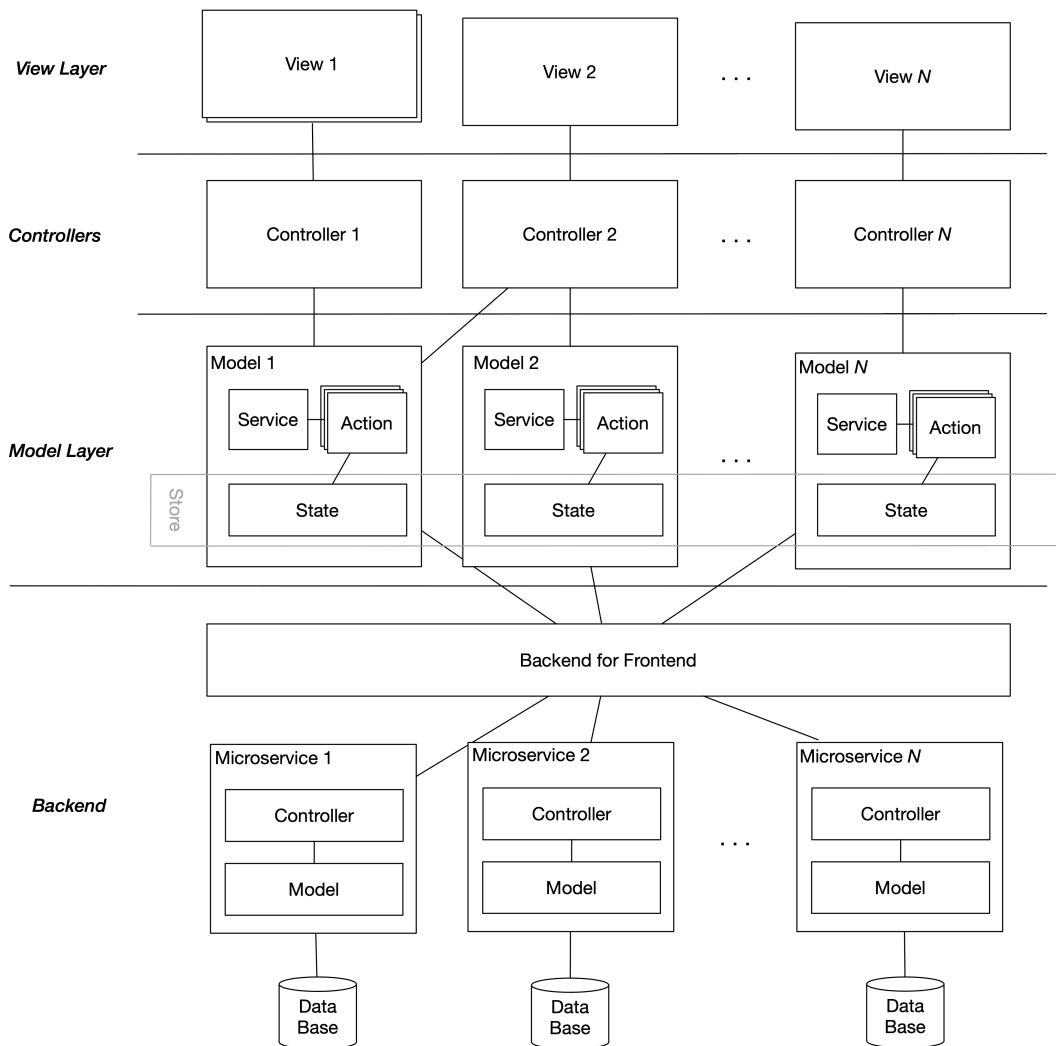
Figure 4.84. Frontend MVC Architecture with Redux + Backend
