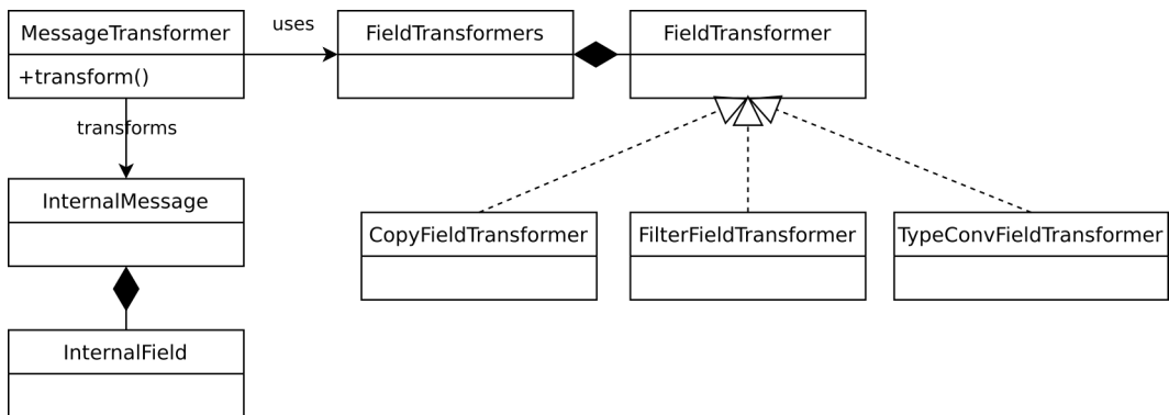
Figure 4.23. Transform Subdomain Class Diagram
