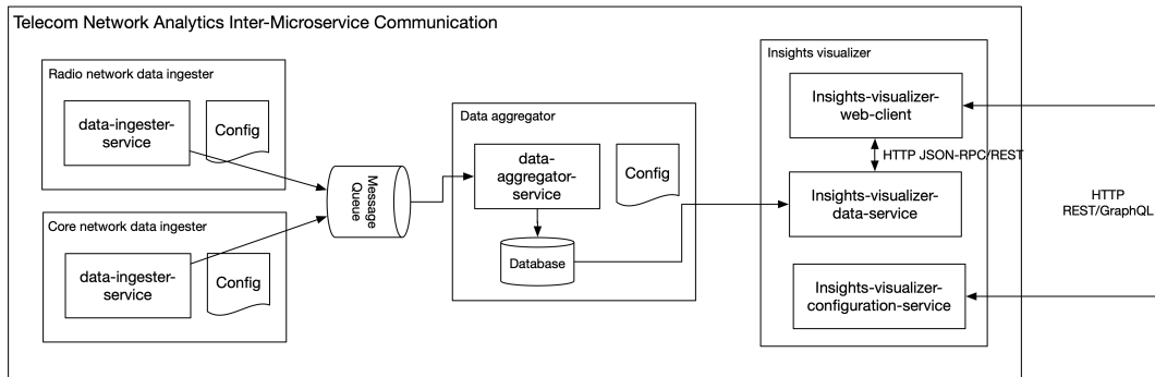
Figure 3.29. Inter-Microservice Communication
