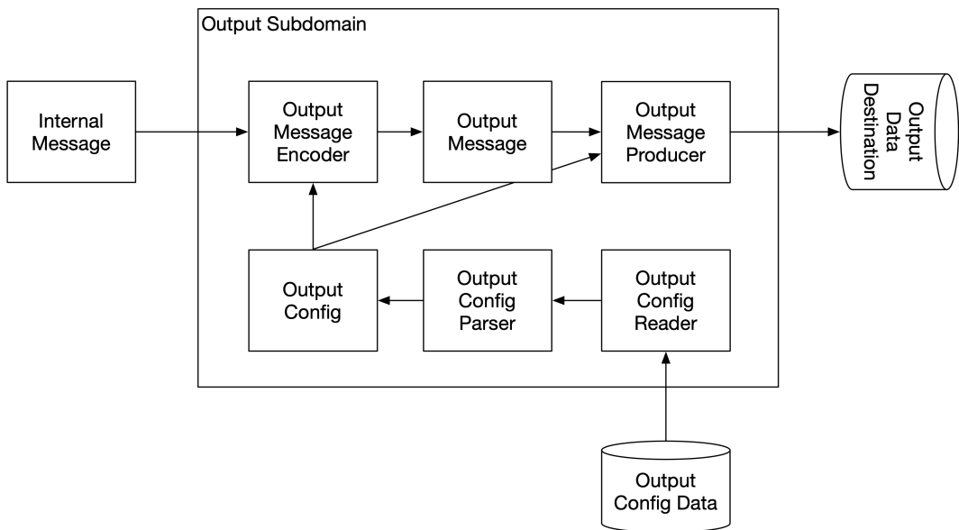
Figure 4.24. Output Subdomain
