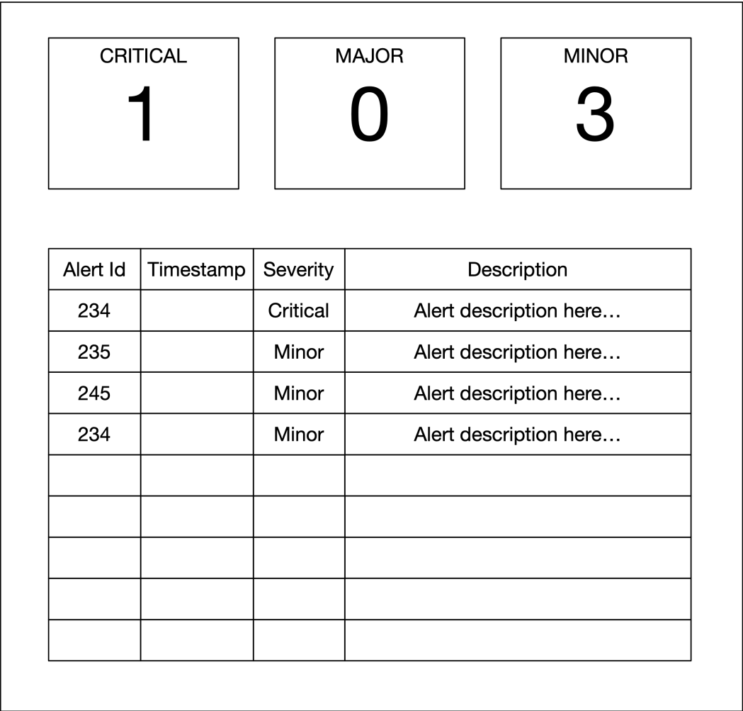
Figure 12.2. DevSecOps Diagram
