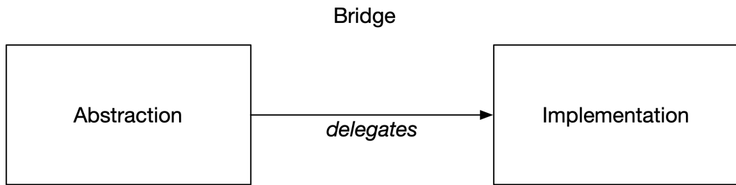
Figure 4.29. Bridge Pattern
