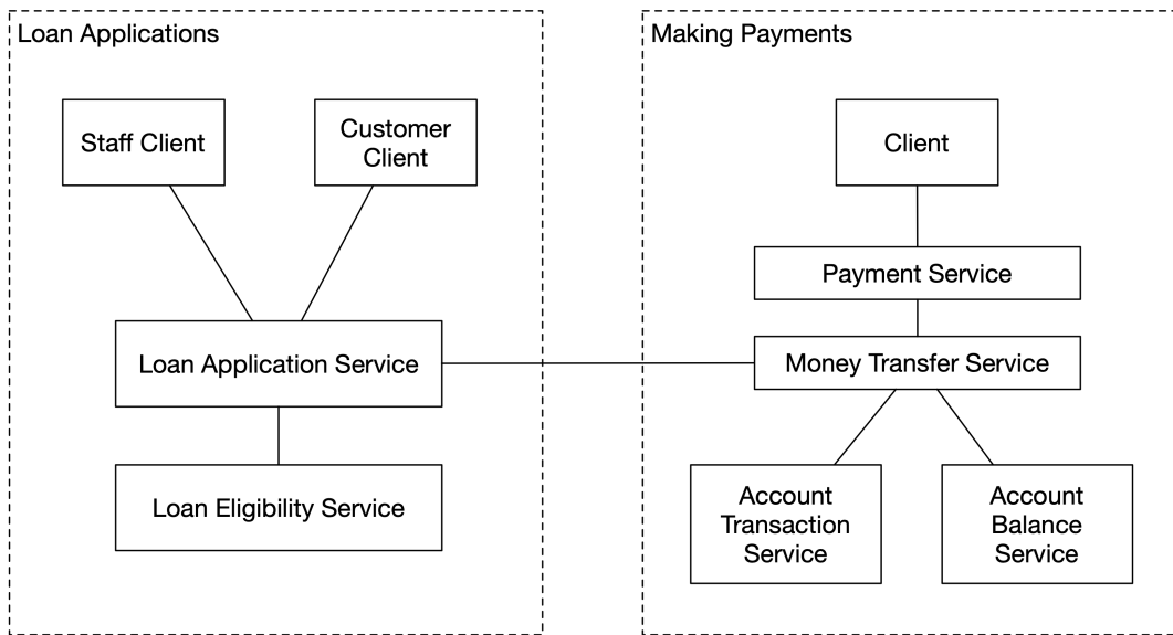
Figure 3.31. Banking Software System Bounded Contexts
