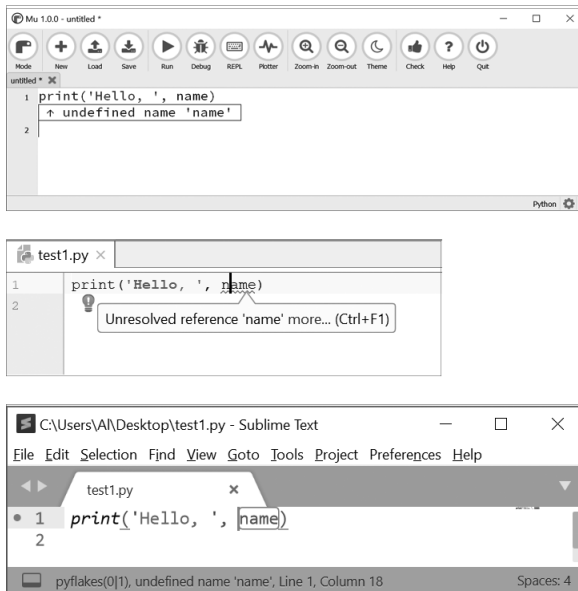
Figure 1-2: A linter points out an undefined variable in Mu (top), PyCharm (middle), and Sublime Text (bottom).
