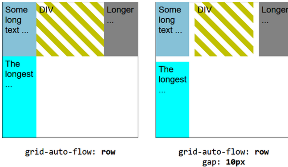
Figure 18-29. The grid item spacing set to 10 pixels with the gap property
