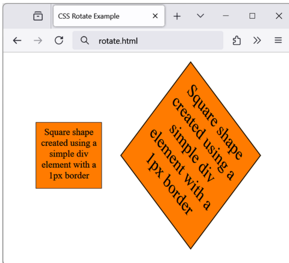
Figure 18-14. An object before and after transformation
