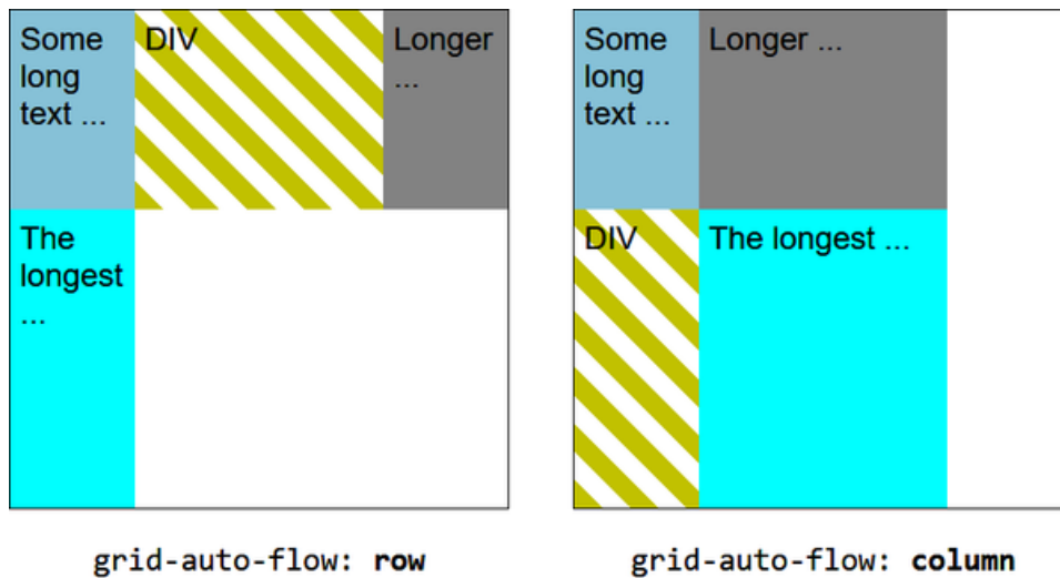
Figure 18-27. Setting the flow direction of the grid with the grid-auto-flow property
