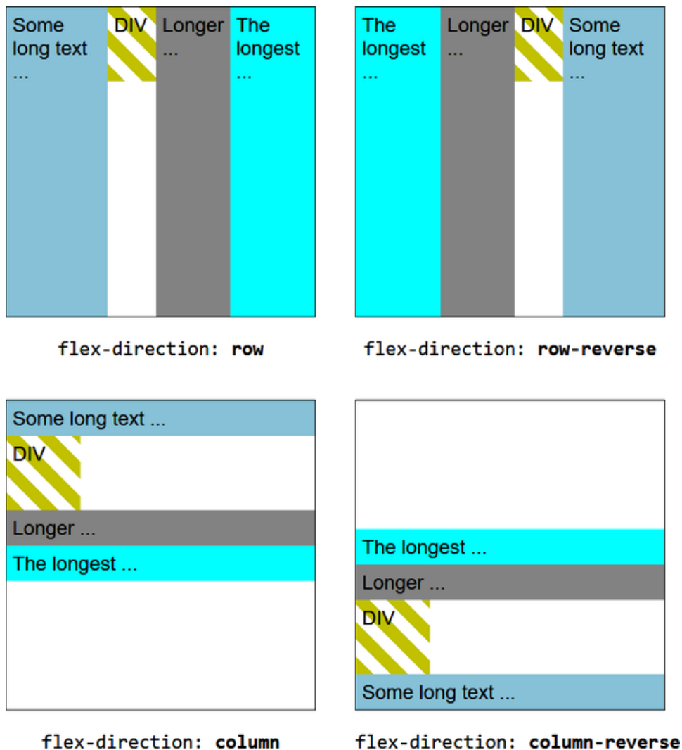
Figure 18-19. The flex-direction property
