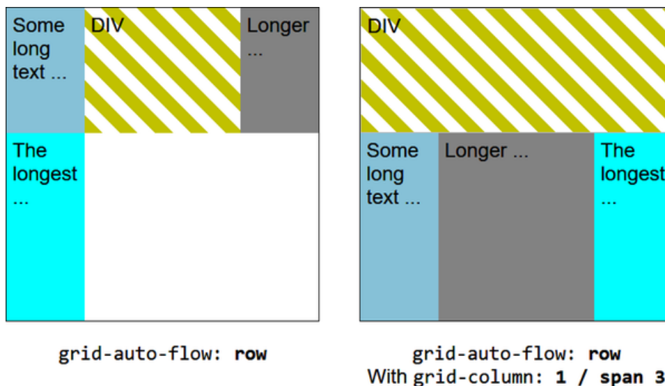
Figure 18-28. Placing the DIV into the first column, spanning all three, using the grid-column property
