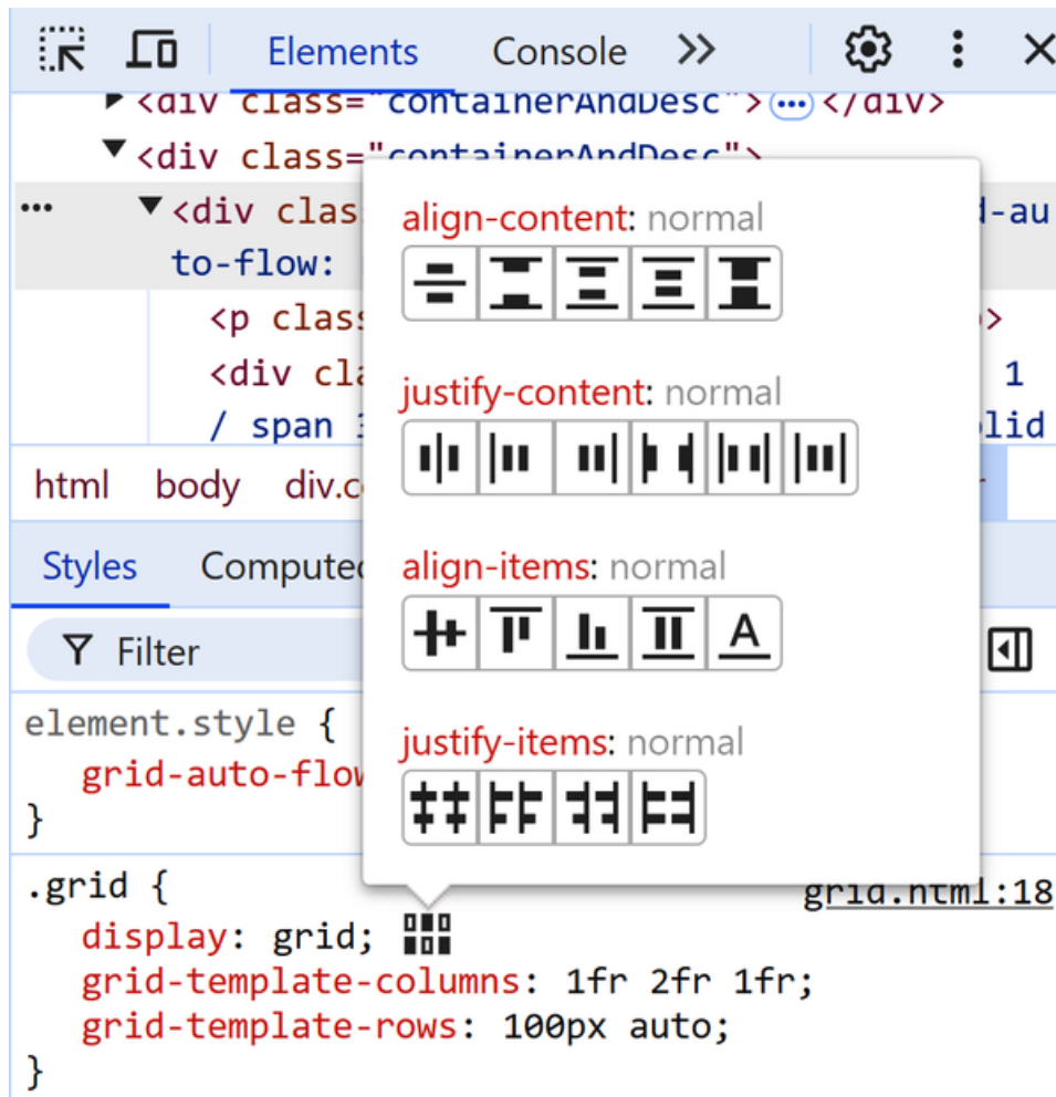
Figure 18-25. Grid editor in Chrome developer tools
