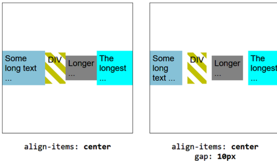
Figure 18-24. Defining the spacing between items with the gap property
