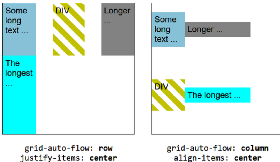
Figure 18-30. The grid items aligned with the justify-items and align-items properties
