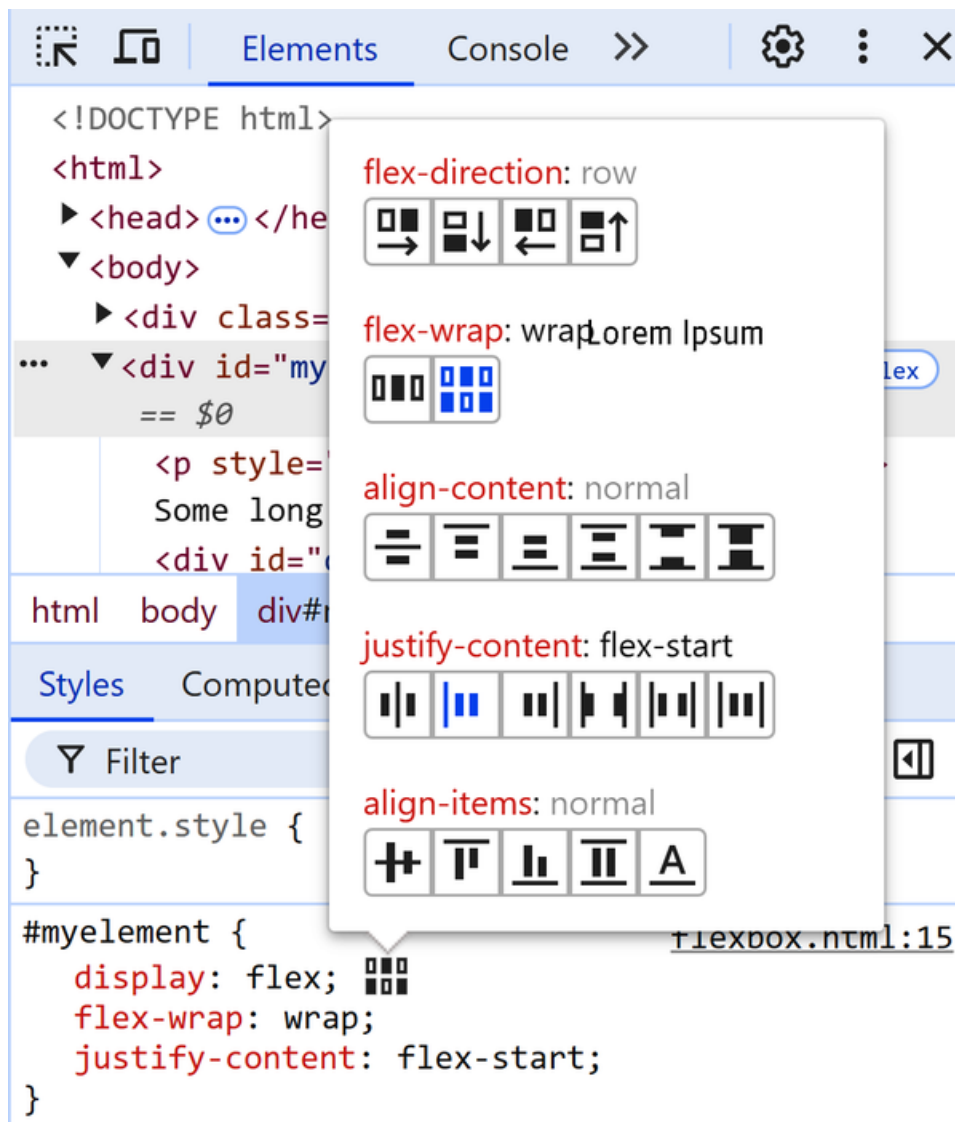
Figure 18-18. Flexbox editor in Chrome developer tools
