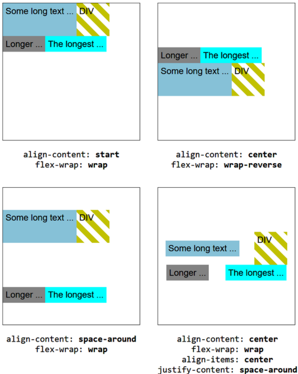
Figure 18-22. Various values of the align-content property with flex-wrap applied
