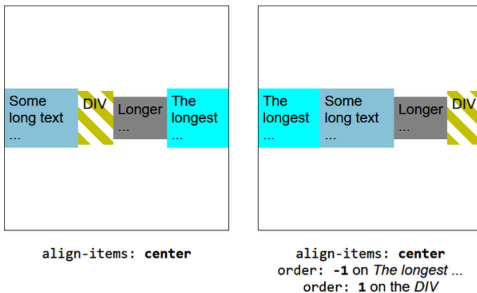
Figure 18-23. Reordered elements using the order CSS property
