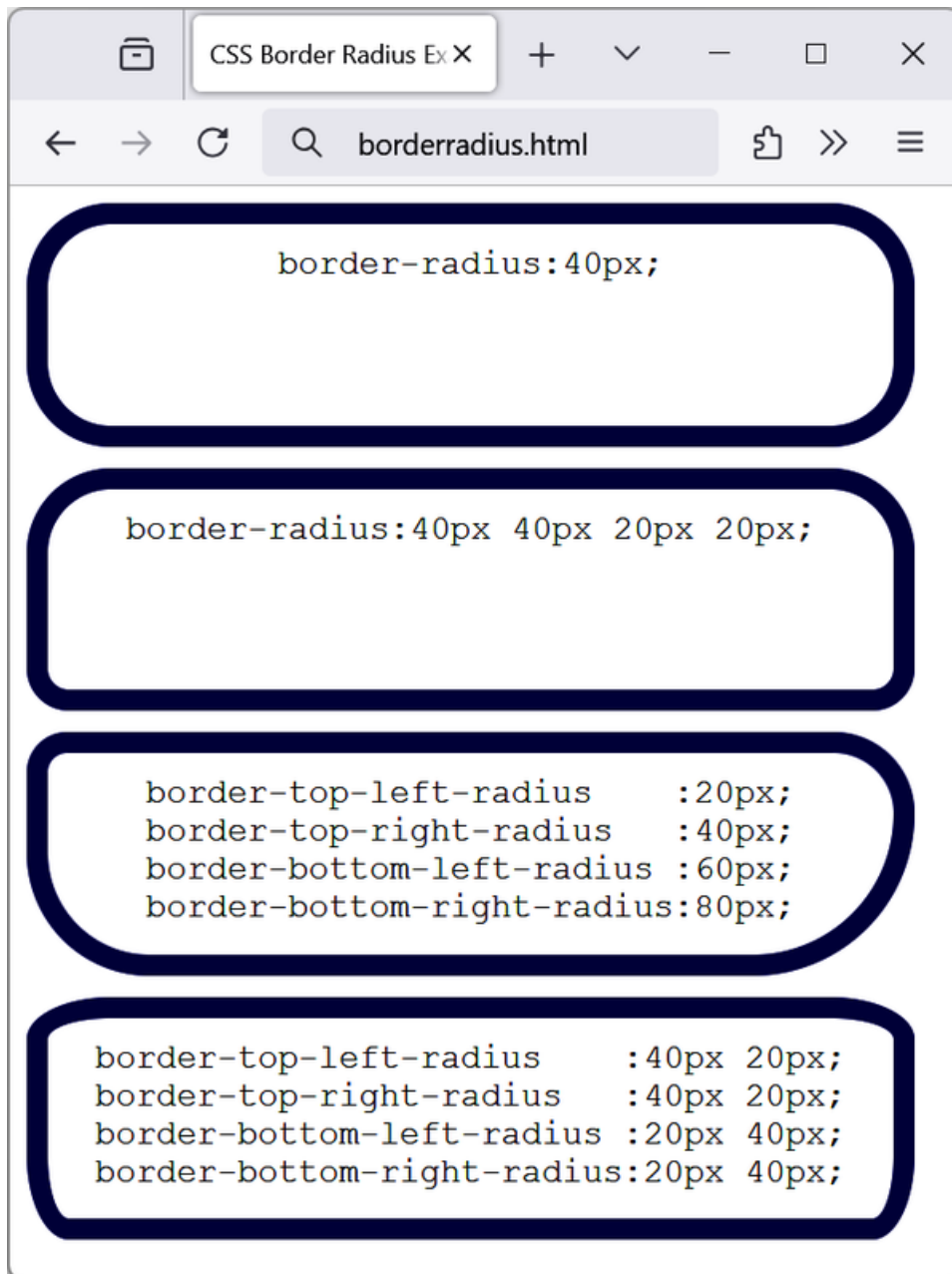
Figure 18-4. Mixing and matching various border radius properties
