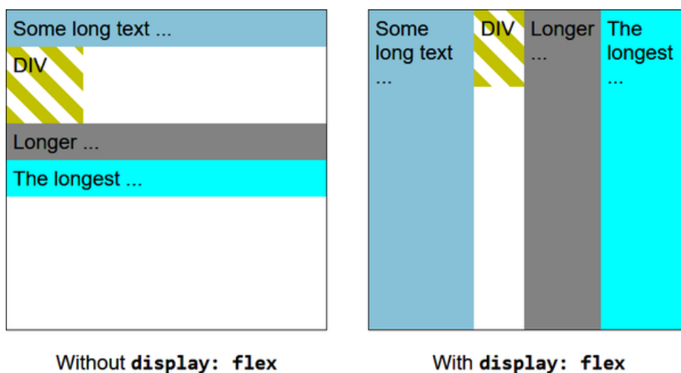
Figure 18-17. Enabling flexbox
