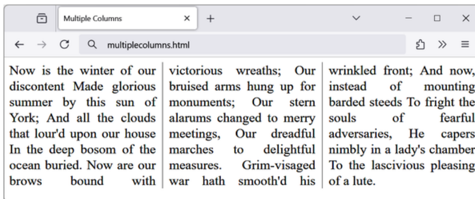
Figure 18-6. Flowing text in multiple columns
