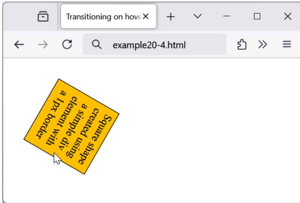
Figure 18-16. The object rotates and changes color when hovered over
