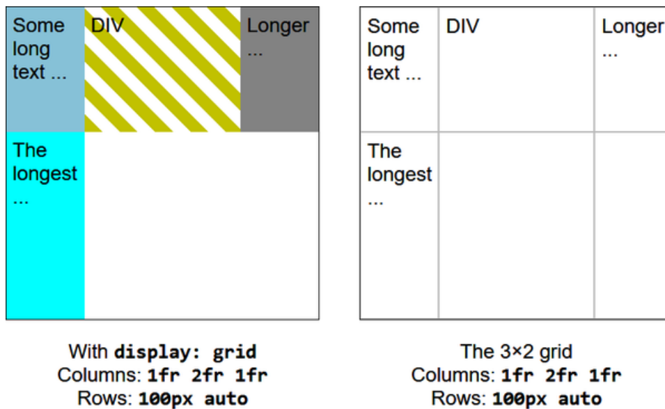
Figure 18-26. Creating a grid with the grid-template-column and grid-template-rows properties
