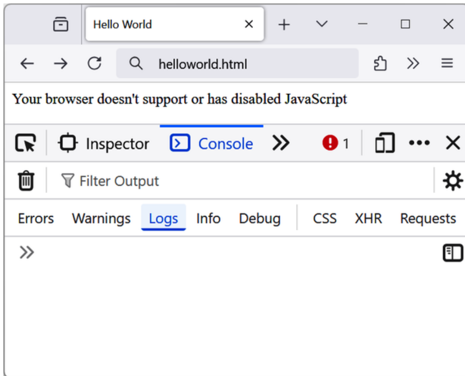
Figure 13-2. JavaScript, disabled
