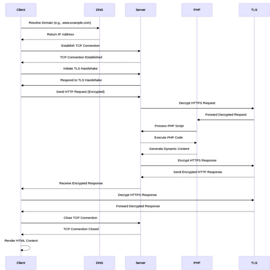
Figure 6-2. Https Connection workflow lifecycle
