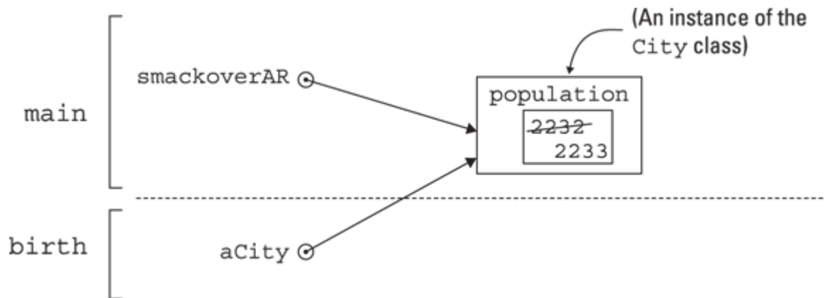
FIGURE 7-16: Pass by reference, under the hood.
