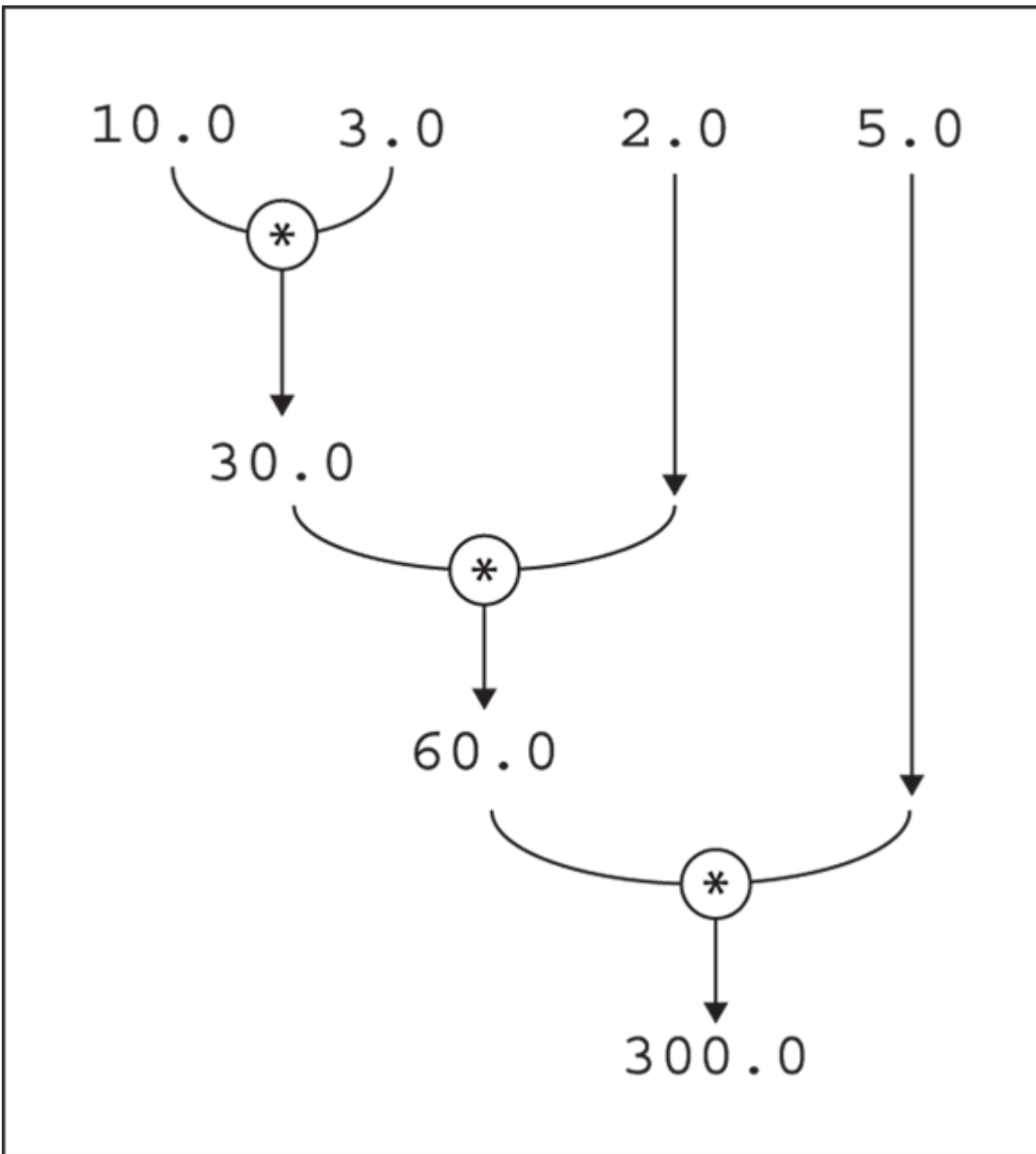
FIGURE 12-17: The reduce method multiplies values from an incoming stream.
