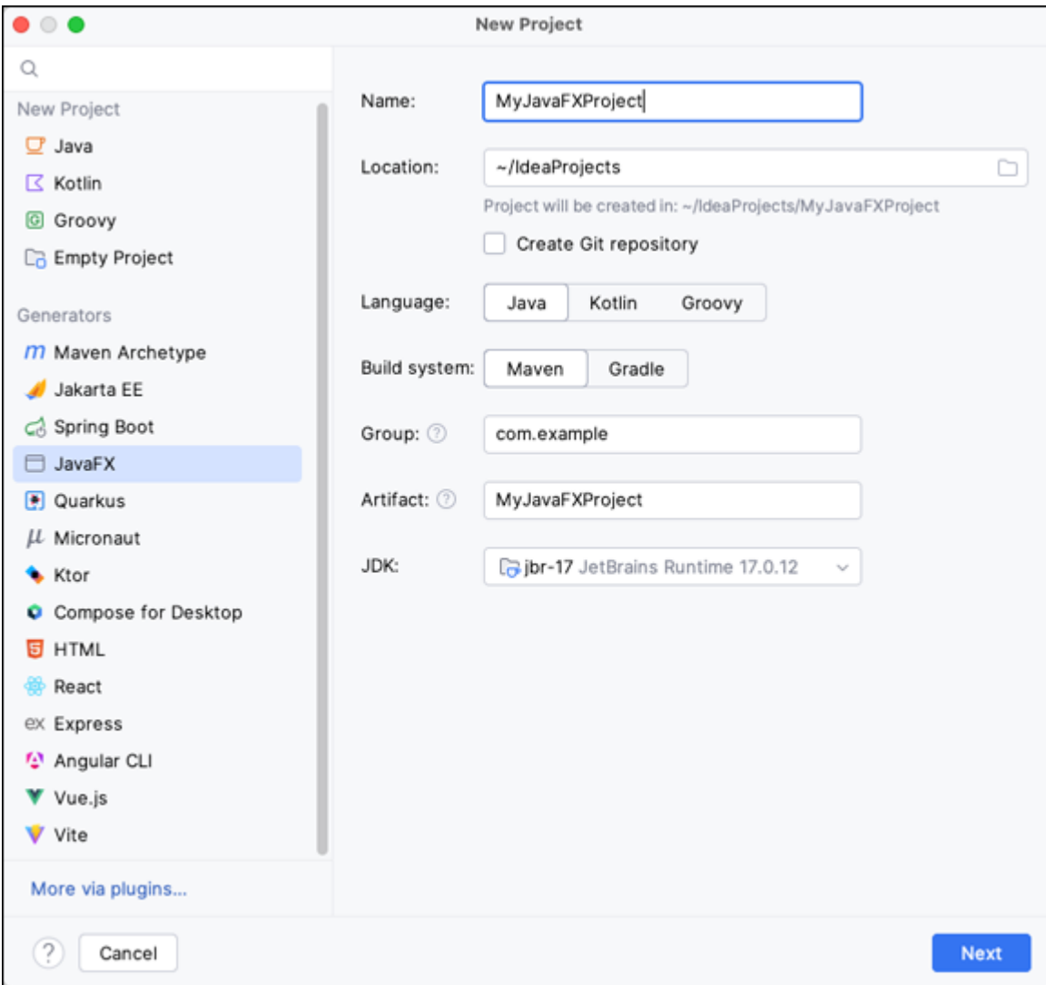
FIGURE 16-2: The New Project dialog box.
