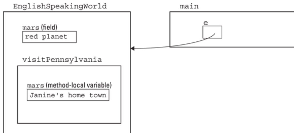
FIGURE 7-12: The structure of the code in Listings 7-12 and 7-13 .
