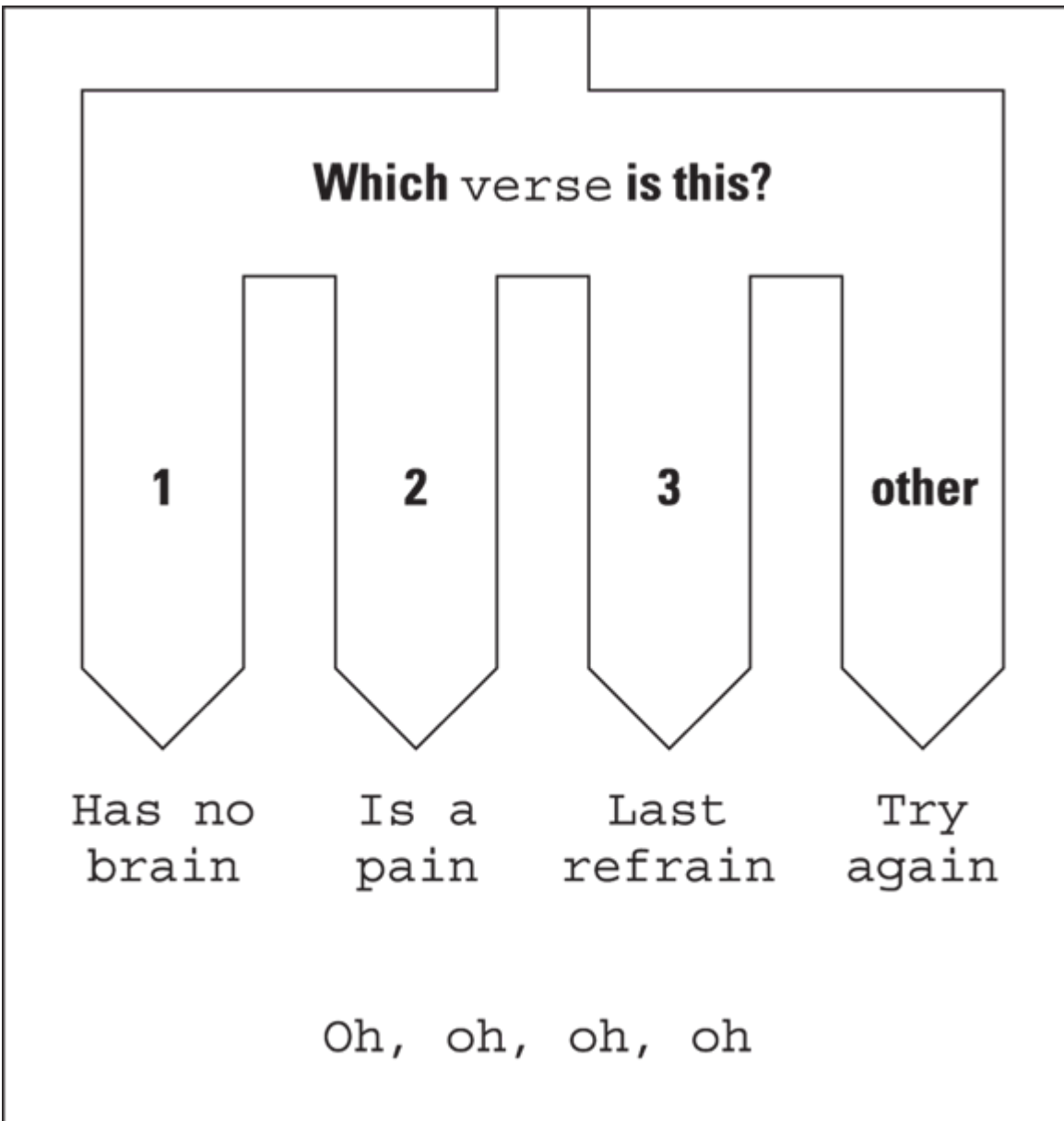
FIGURE 5-12: The big fork in the code of Listing 5-6 .
