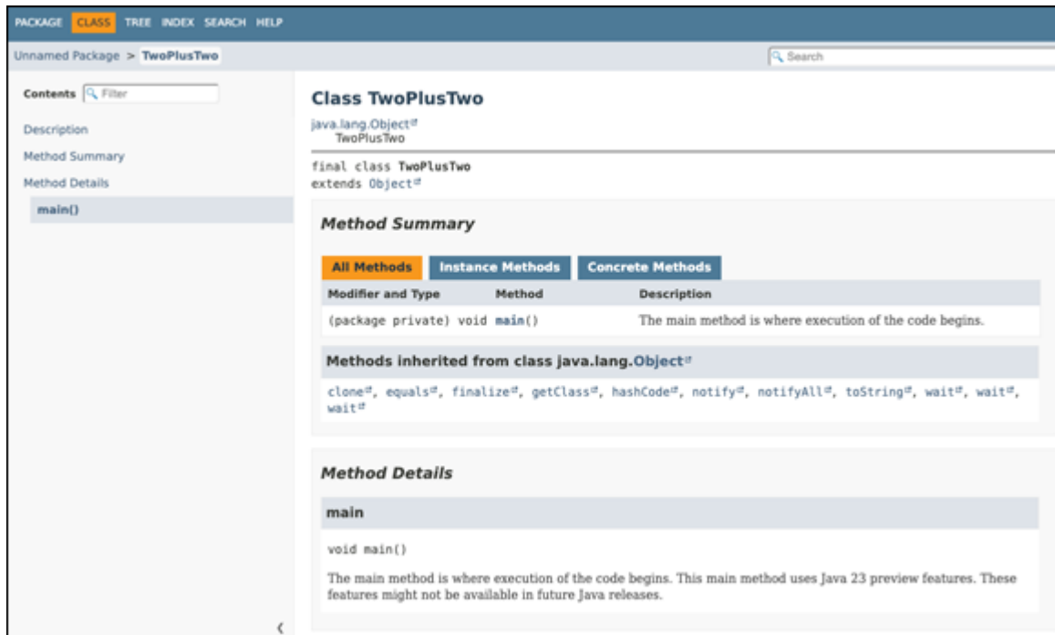
FIGURE 3-7: The Javadoc page generated from the code in Listing 3-5 .
