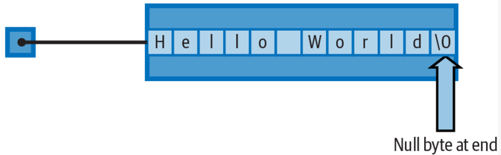
Figure 3-1. String, StringBuilder, and C-language strings
