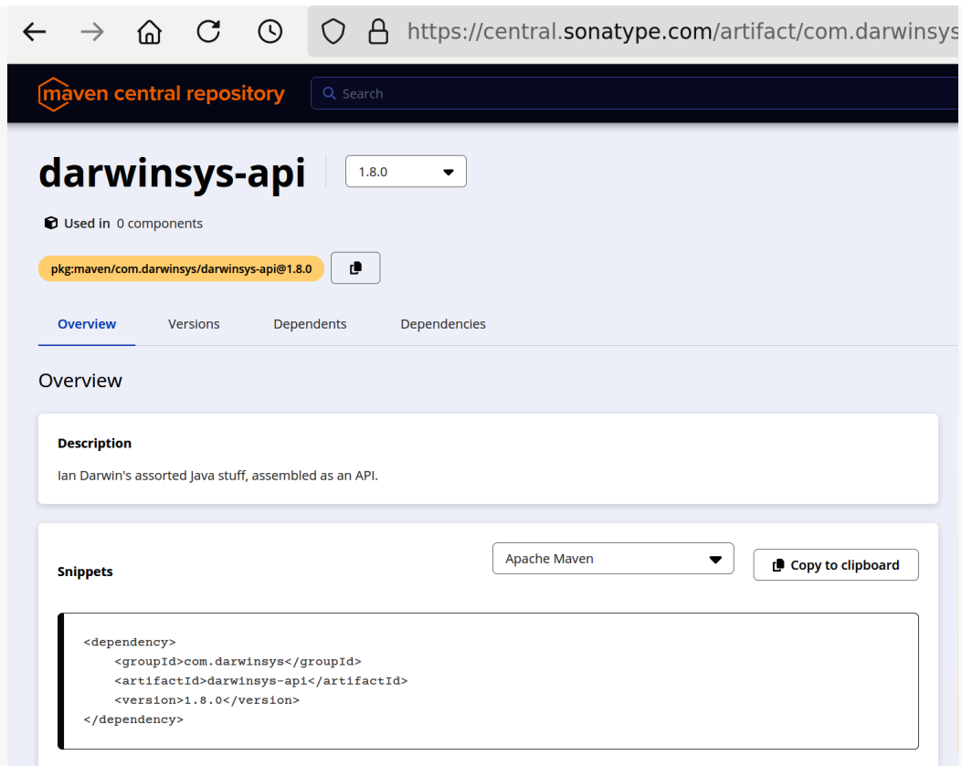
Figure 2-1. Maven Central search results
