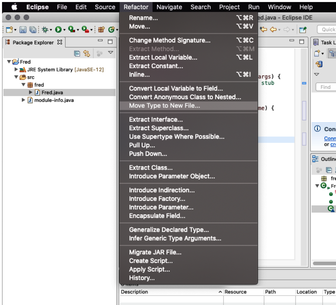
Figure 1-3. Refactoring in Eclipse
