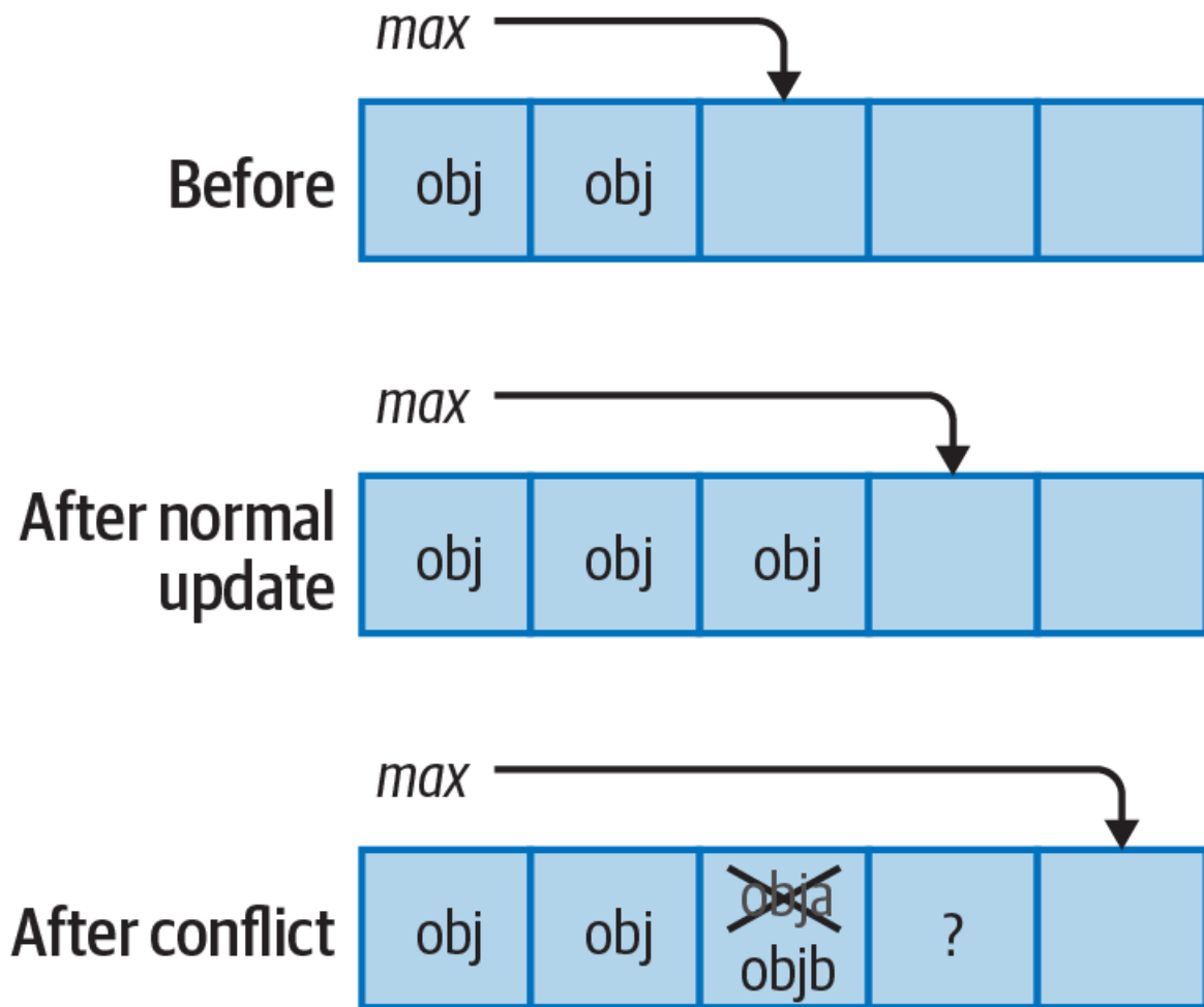
Figure 11-1. Non-thread-safe add method in operation: normal and failed updates
