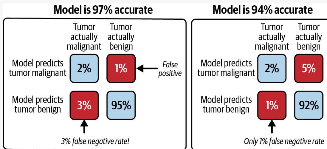
Figure 13-2. More accuracy isn't always the best indicator
