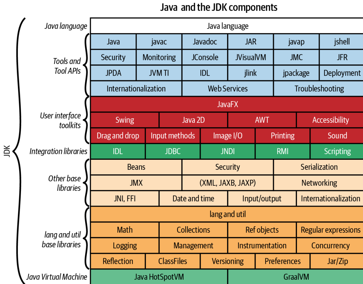
Figure P-1. Java conceptual diagram
