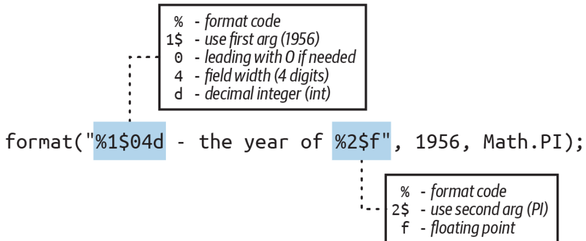
Figure 3-2. Formatter codes examined
