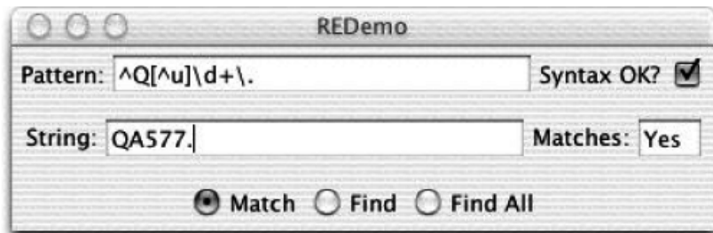
Figure 4-2. REDemo with “Q not followed by u” example
