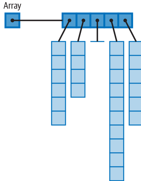
Figure 7-3. Multidimensional arrays
