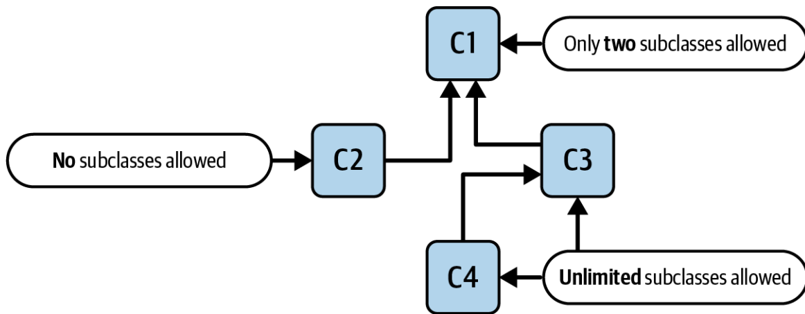
Figure 8-2. Sealed types inheritance
