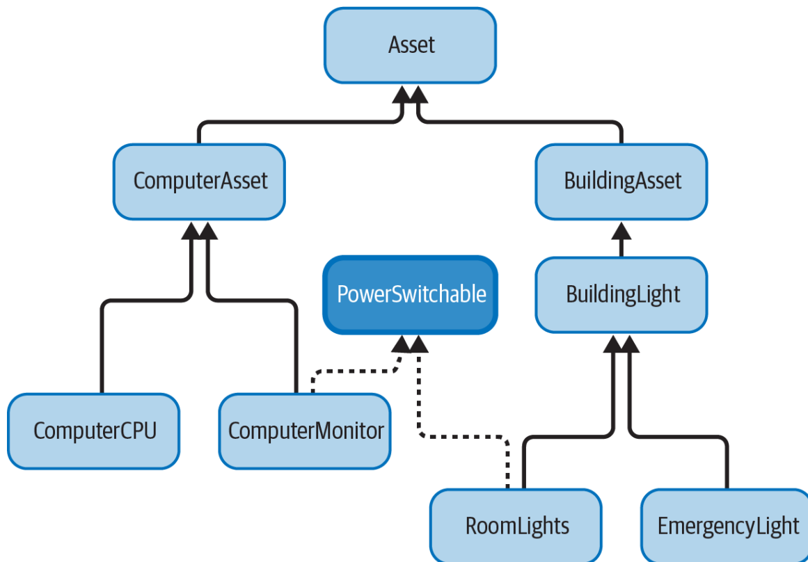
Figure 8-1. Classes for a building management system
