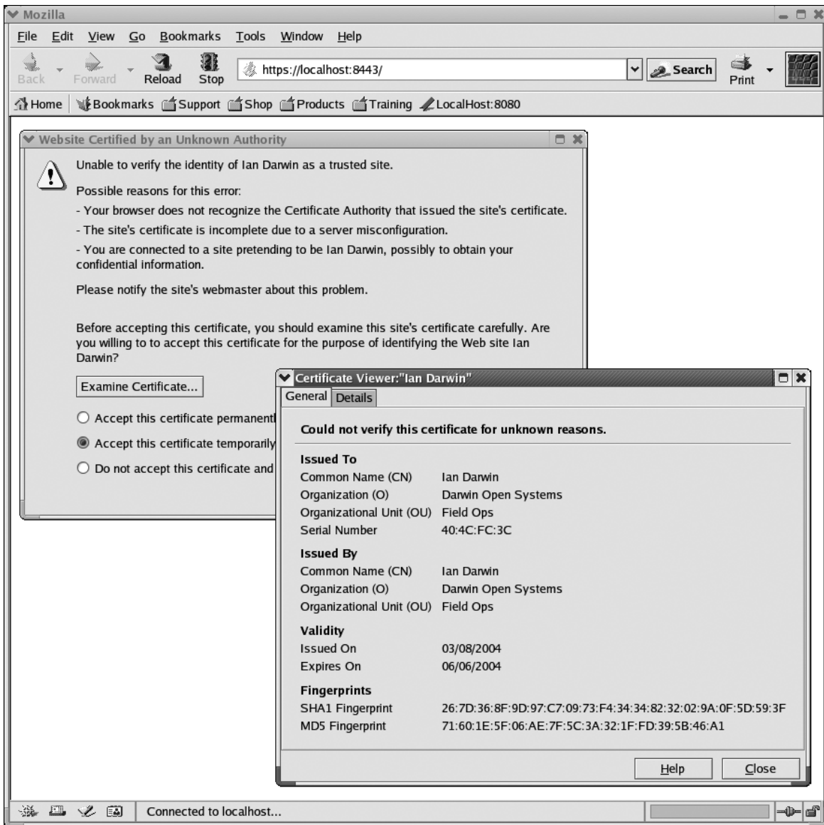
Figure 15-2. Browser caution
