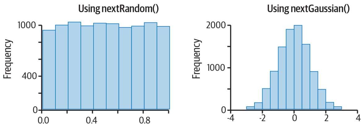
Figure 12-1. Flat (left) and Gaussian (right) distributions
