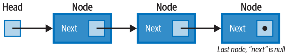
Figure 7-2. Linked list structure
