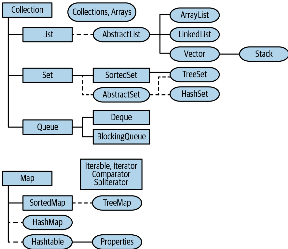
Figure 7-1. The Collections Framework
