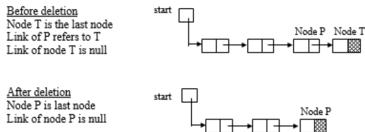
Figure 3.14 Deletion at the end of the list
