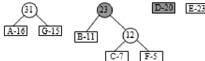
Figure 6.186 Trees weighted 16 and 15 are combined
