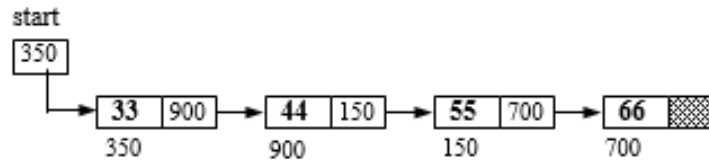
Figure 3.2 Single linked list
