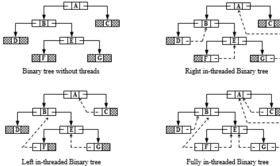
Figure 6.45 Threaded binary tree
