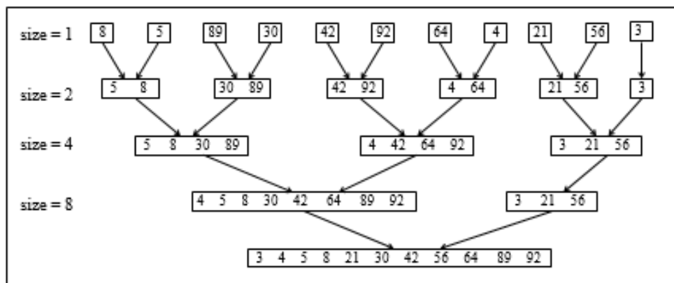
Figure 8.16 Bottom up merge sort
