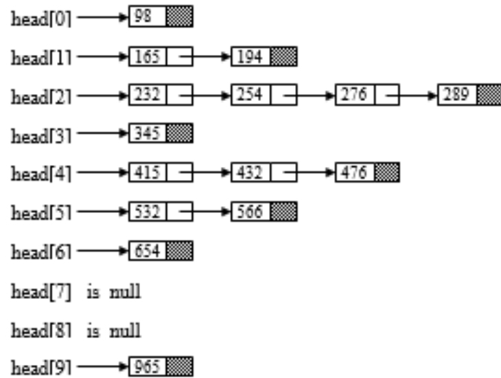
Figure 8.34 Linked lists for f(x) values
