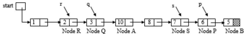
Figure 3.47 Selection sort by rearranging links - 2
