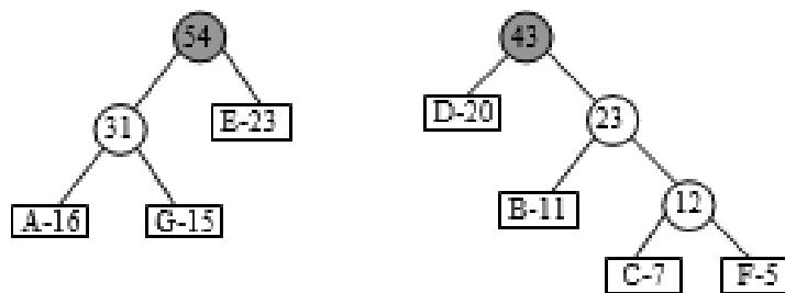
Figure 6.188 Trees weighted 31 and 23 are combined
