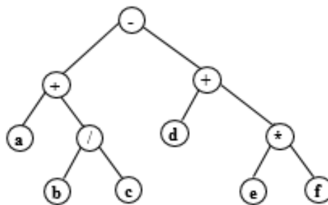
Figure 11.33 Expression tree from algebraic expression
