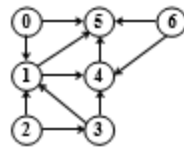
Figure 7.139 Directed graph for topological sorting
