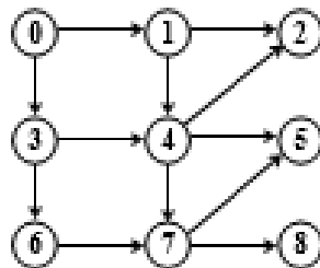
Figure 7.71 Graph for depth first search traversal
