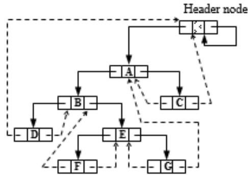
Figure 6.52 Threaded tree with header node
