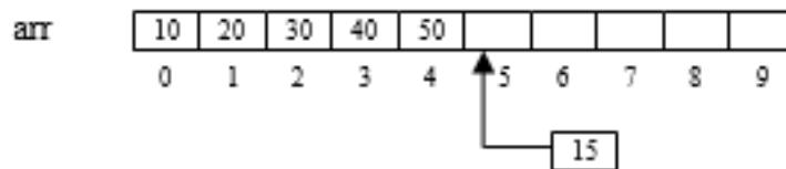
Figure 2.4 Insertion at the end
