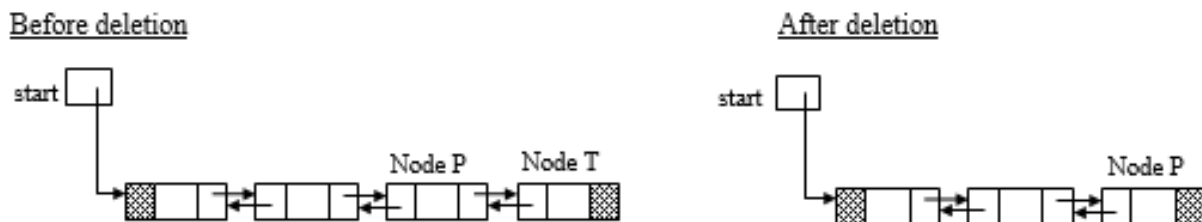
Figure 3.26 Deletion at the end of the list
