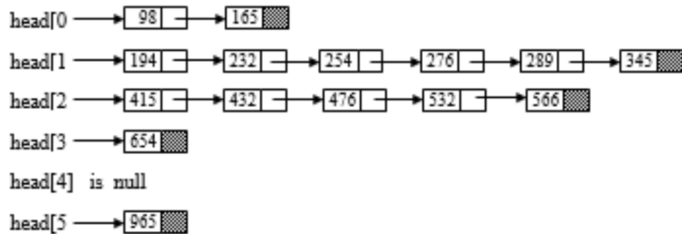
Figure 8.35 Linked lists for h(x) values
