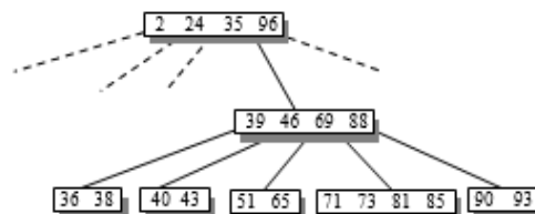
Figure 6.250 B-tree example for inserting 80
