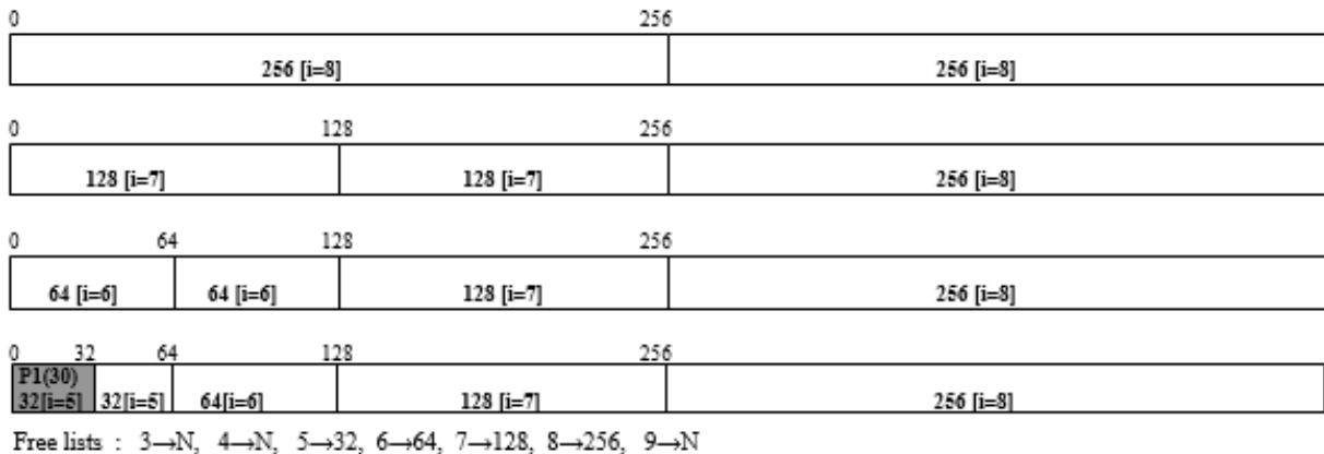
Figure 10.19 Allocate 30K for P1
