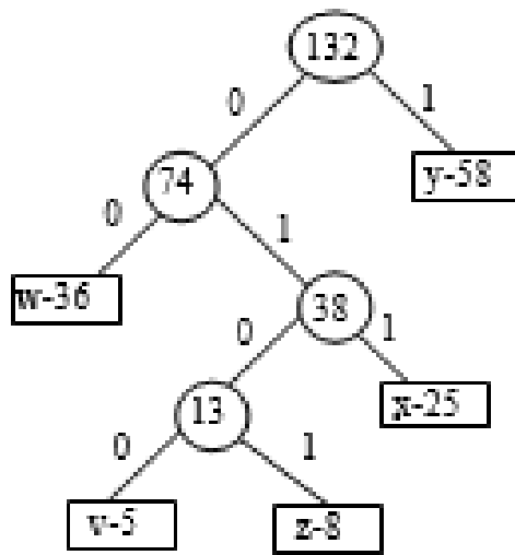
Figure 6.193 Bit values assigned to branches of huffman tree
