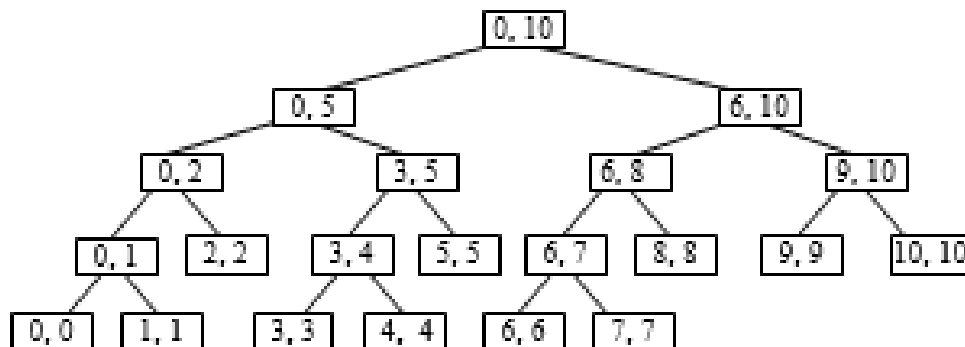
Figure 8.15 Merge sort recursive calls with low and up values
