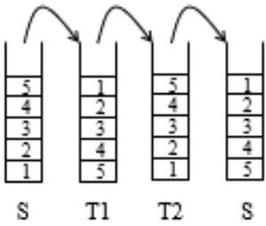
Figure 11.14 Reversing a stack using two stacks
