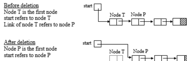
Figure 3.11 Deletion of first node
