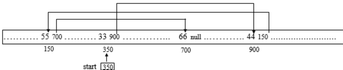
Figure 3.3 Single linked list in memory
