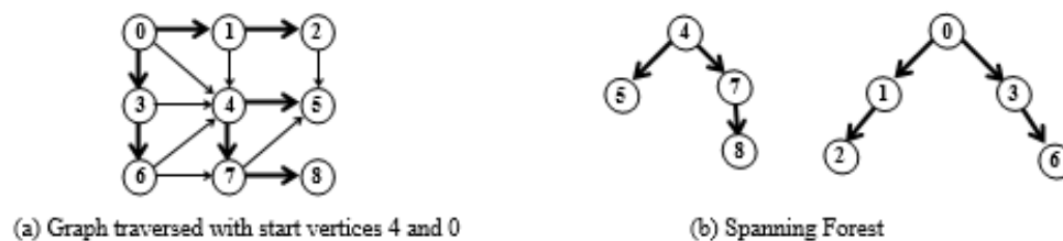
Figure 7.67 Breadth first search spanning forest
