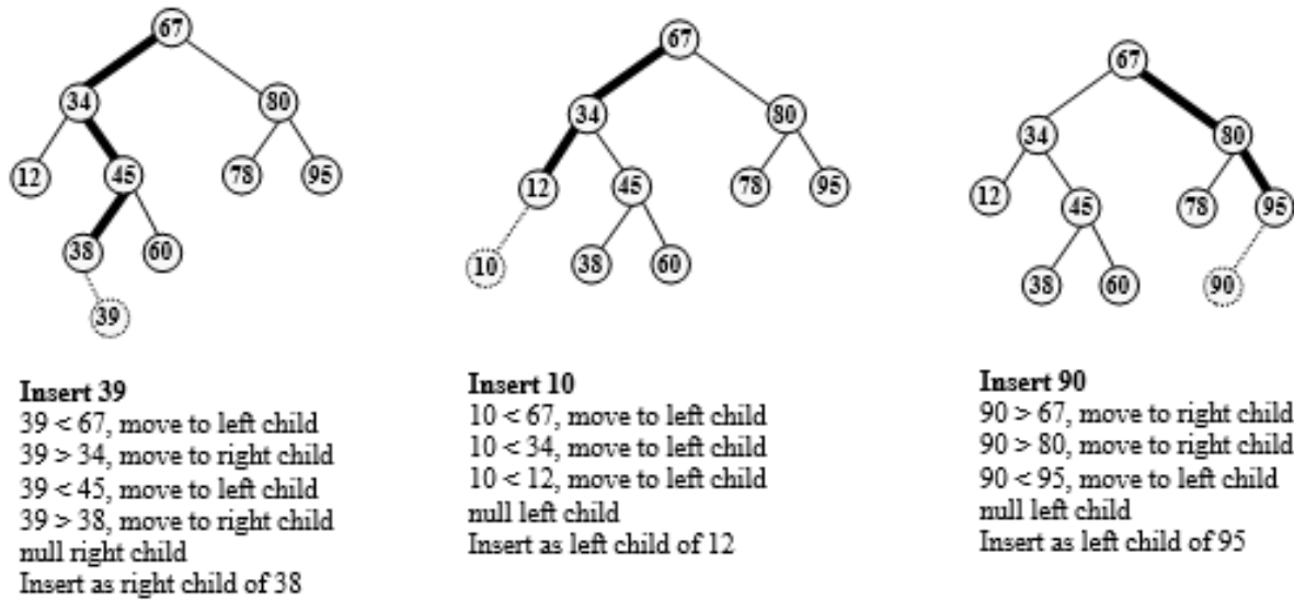
Figure 6.35 Insertion in a binary search tree
