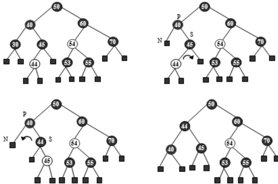
Figure 6.165 Delete 30
