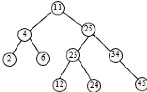
Figure 11.35 AVL tree
