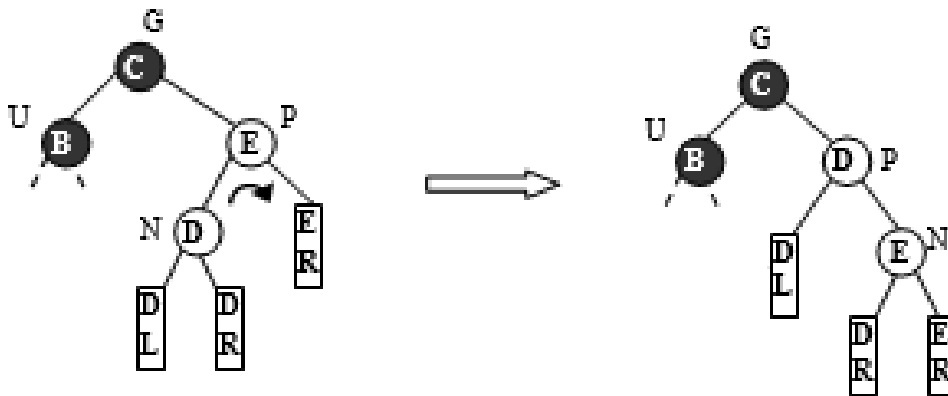
Figure 6.136 Case R_2a
