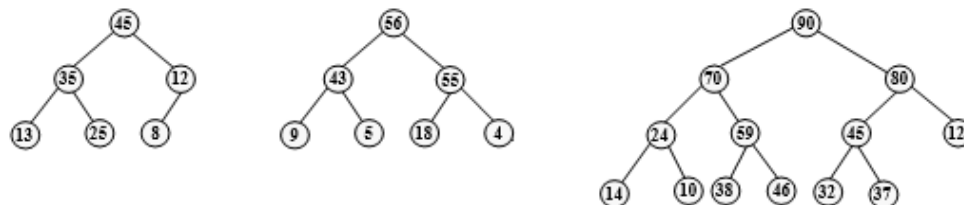
Figure 6.168 Max heaps
