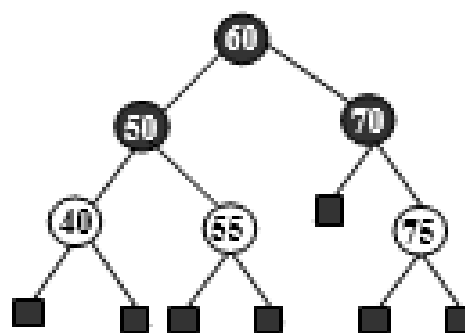
Figure 6.142 Insert 55, 75
