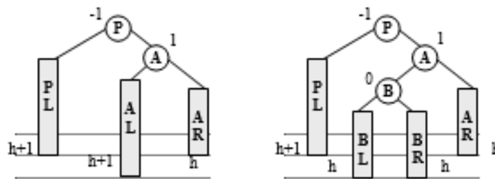
Figure 6.110 Case L_C3
