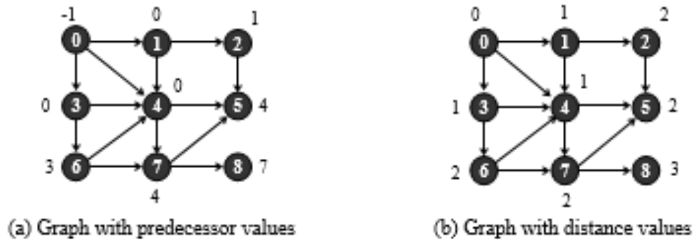
Figure 7.65 Graph with predecessor and distance values
