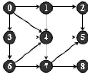
Figure 7.54 Visit 8
