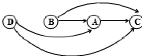
Figure 7.135 Another topological order of the previous graph
