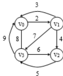
(a) Weighted Directed Graph
