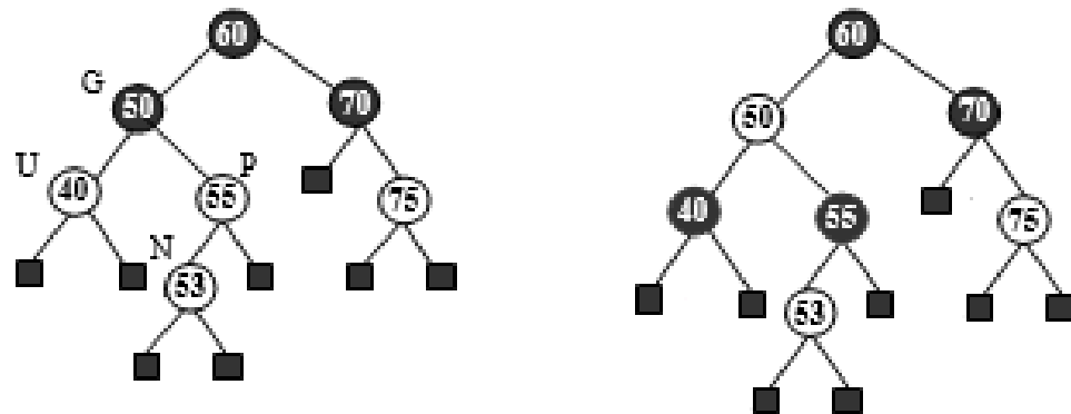
Figure 6.143 Insert 53
