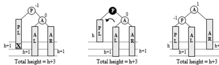
Figure 6.108 Case L_C1
