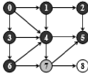
Figure 7.62 Visit 5
