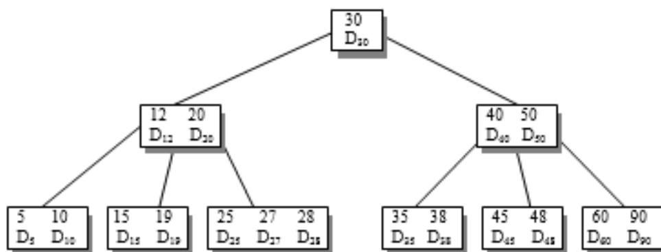
Figure 6.268 B-tree example
