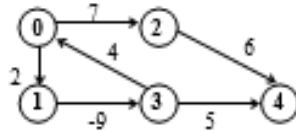
Figure 7.104 Graph with negative cycle
