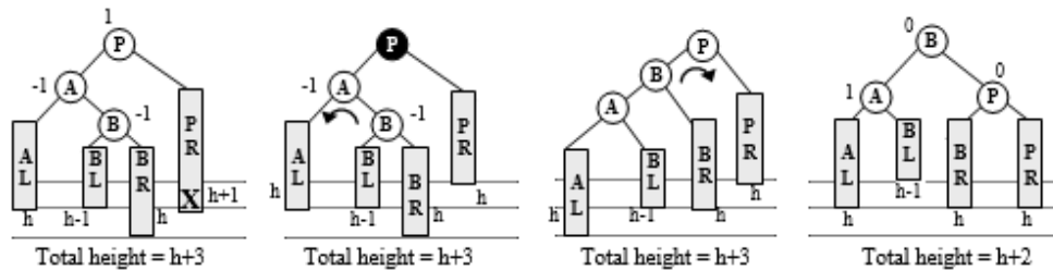
Figure 6.120 Case R_C3c
