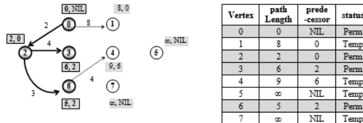
Figure 7.92 Make vertex 3 permanent
