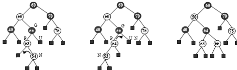
Figure 6.144 Insert 54
