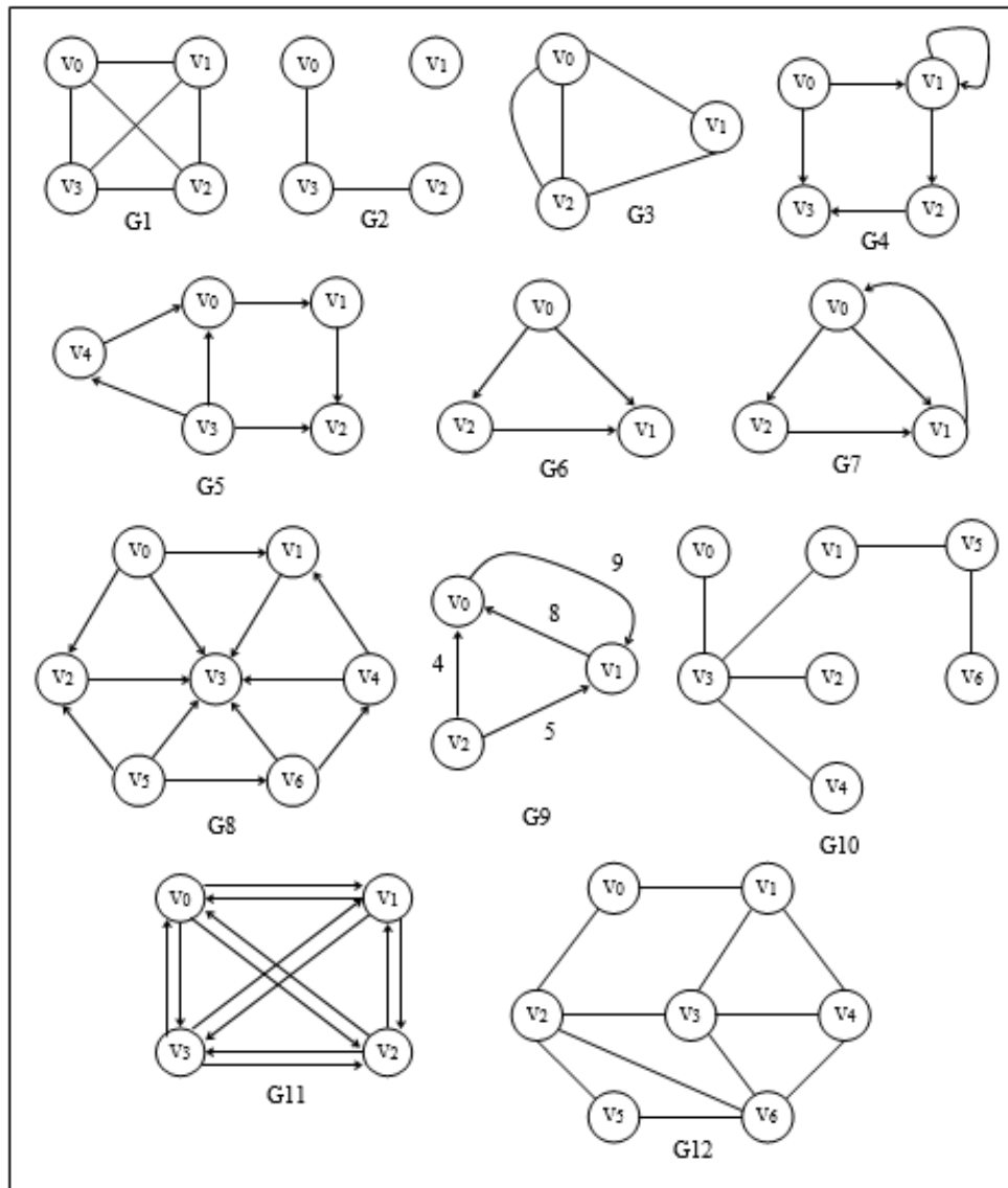
Figure 7.3 Graphs examples
