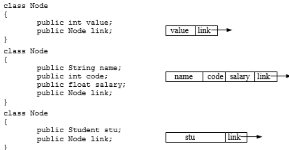
Figure 3.5 Node examples
