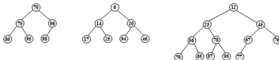
Figure 6.169 Min heaps
