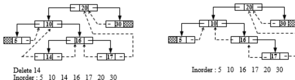
Figure 6.48 Deletion of 14
