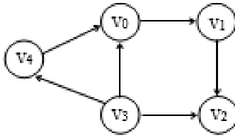
Figure 7.2 Directed graph
