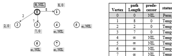
Figure 7.89 Make vertex 0 permanent
