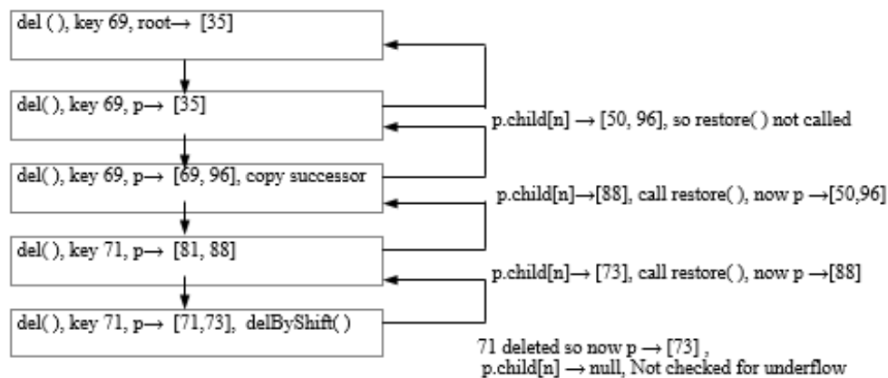
Figure 6.261 Deletion of 69
