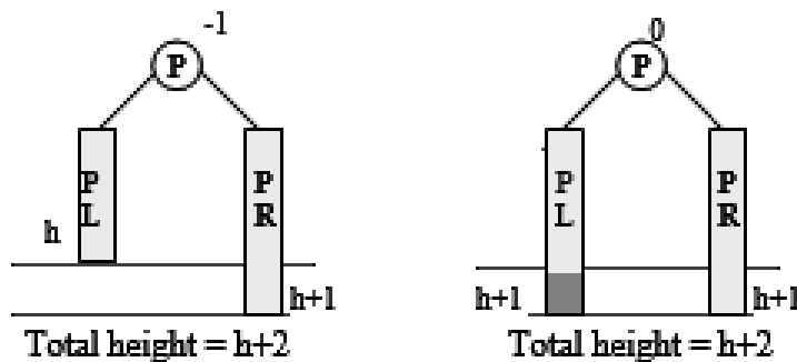
Figure 6.71 Case L_B
