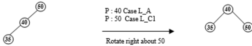
Figure 6.97 Insert 35
