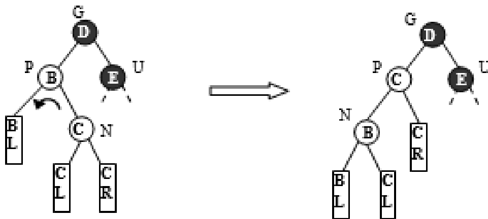
Figure 6.133 Case L_2a
