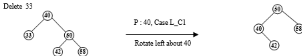
Figure 6.127 Delete 33
