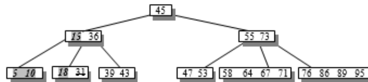
Figure 6.231 Delete 31
