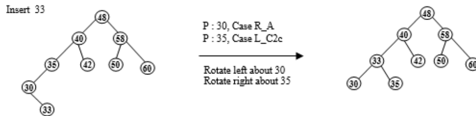
Figure 6.103 Insert 33
