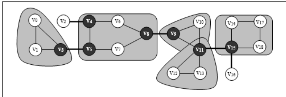
Figure 7.11 Biconnected components
