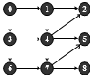
Figure 7.75 Visit vertex 3, 6
