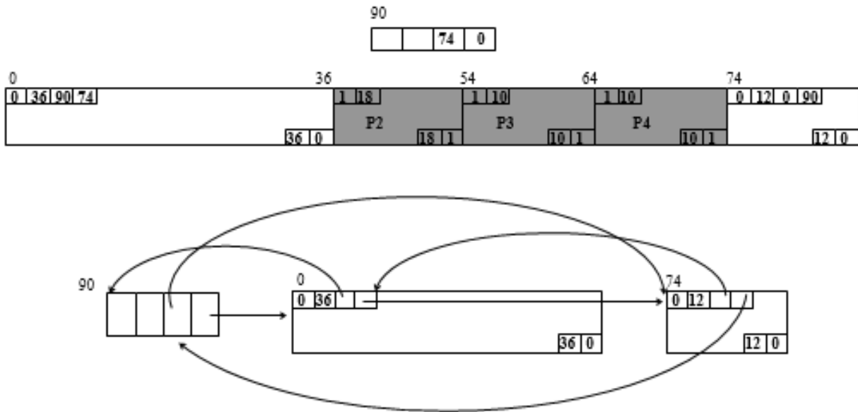
Figure 10.17 Free P1
