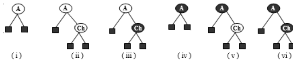
Figure 6.148 Deletion cases
