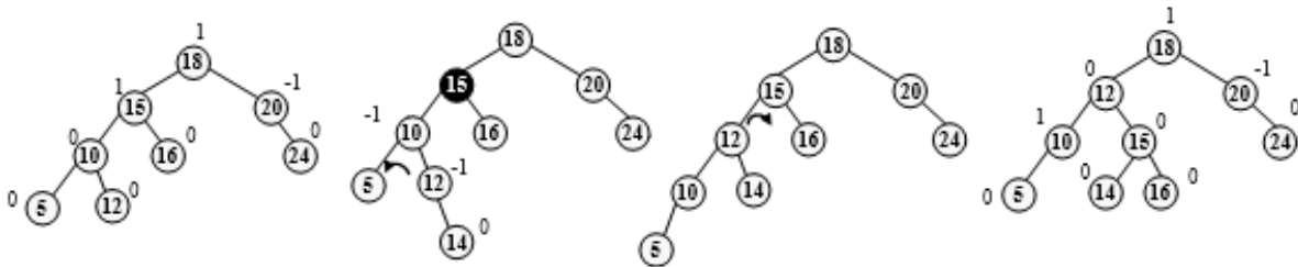
Figure 6.83 Insertion of 14
