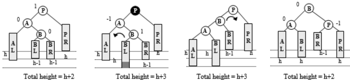
Figure 6.80 Case L_C2b
