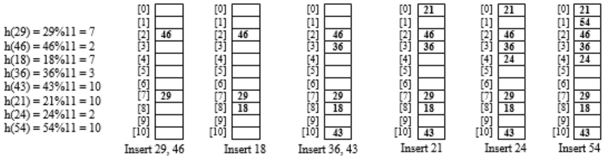
Figure 9.9 Linear probing
