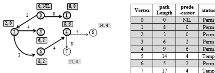
Figure 7.94 Make vertex 4 permanent
