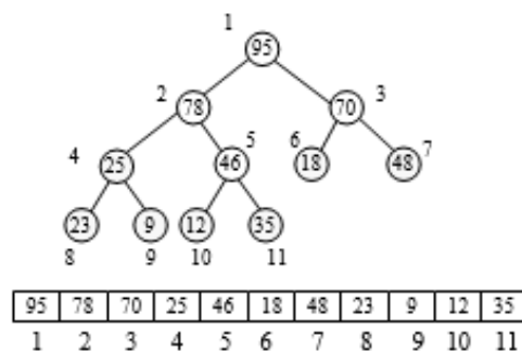
Figure 8.27 Heap tree
