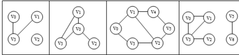
Figure 7.17 Graphs which are not trees
