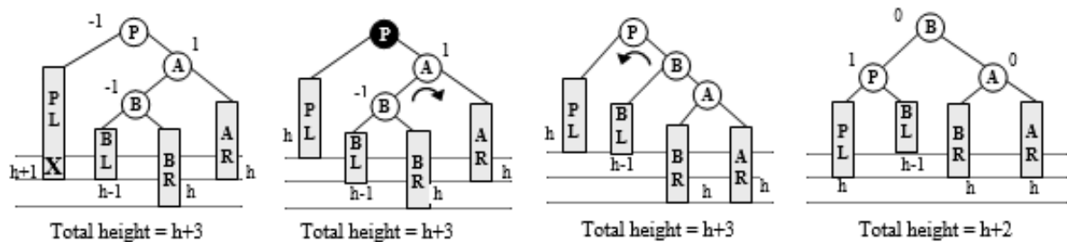
Figure 6.113 Case L_C3c
