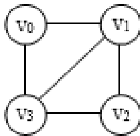
Figure 7.1 Undirected graph
