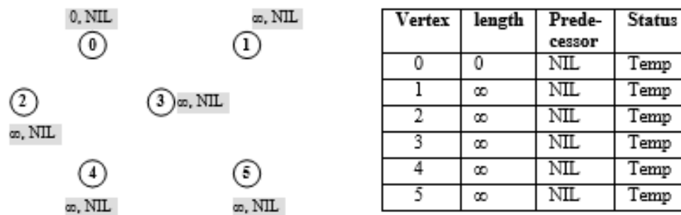
Figure 7.120 Initial tree and table for length, predecessor, status of vertex
