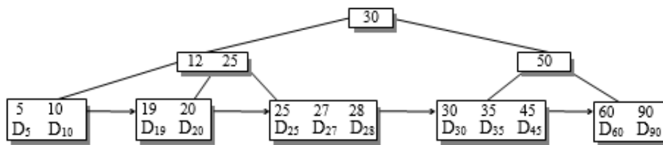
Figure 6.273 Deletion of 48
