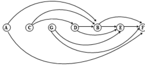
Figure 7.138 Topological order of the graph
