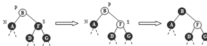
Figure 6.151 Case L_2a
