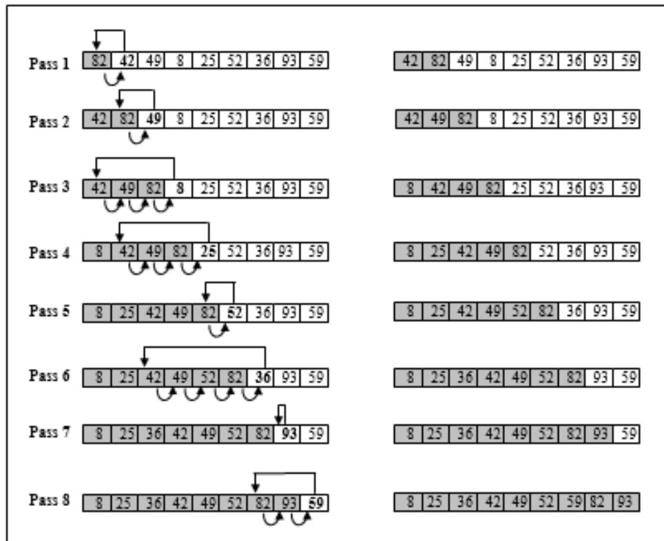
Figure 8.9 Insertion sort
