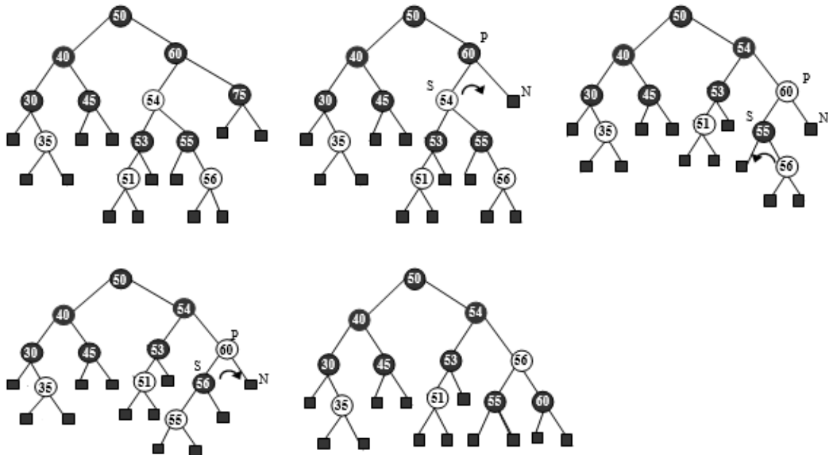
Figure 6.166 Delete 75
