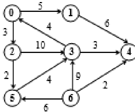
Figure 7.85 Weighted directed graph
