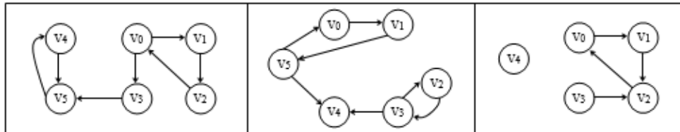
Figure 7.13 Graphs which are not strongly connected
