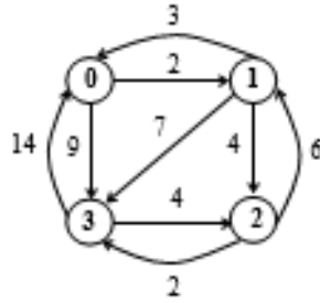
Figure 7.111 Graph for finding shortest path
