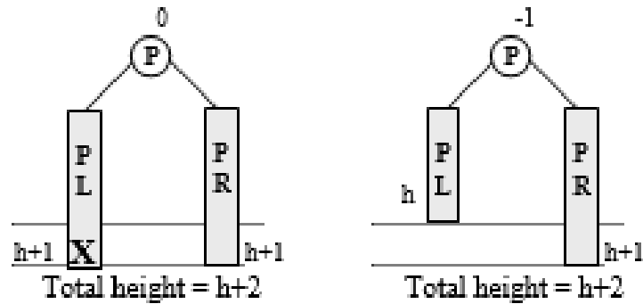
Figure 6.105 Case L_A
