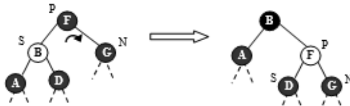
Figure 6.155 Case R_1
