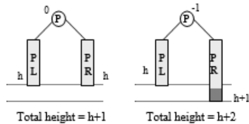
Figure 6.85 Case R_A
