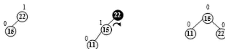
Figure 6.76 Insertion of 11
