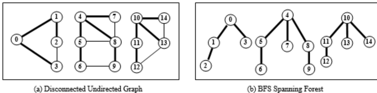
Figure 7.69 BFS spanning forest for disconnected undirected graph
