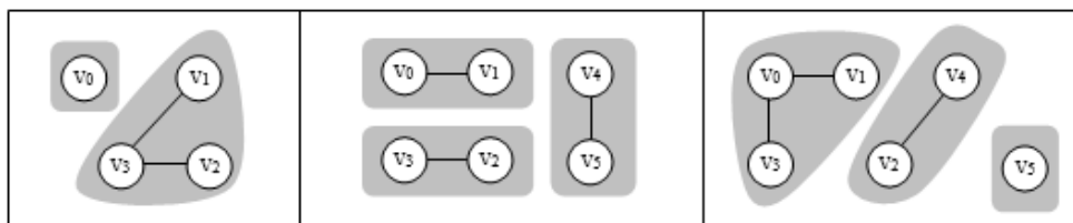
Figure 7.6 Connected components
