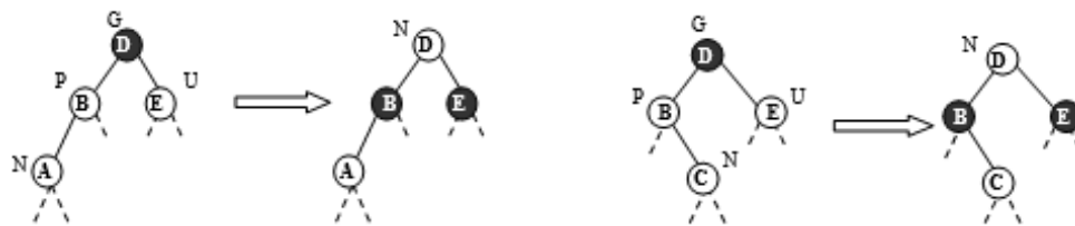
Figure 6.132 Case L_1
