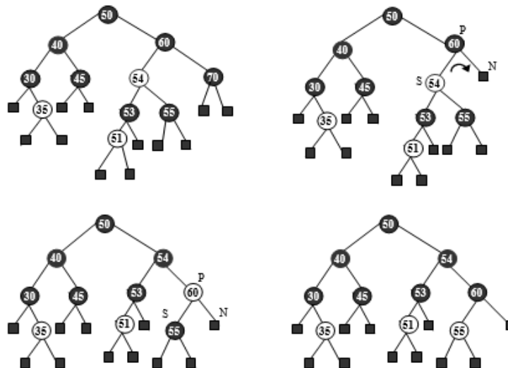
Figure 6.162 Delete 70
