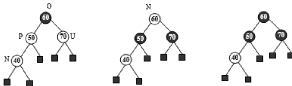
Figure 6.141 Insert 40
