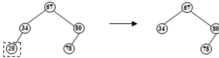
Figure 6.37 Deletion of 20
