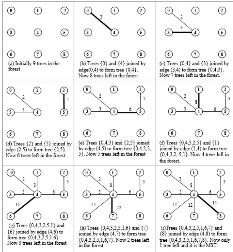
Figure 7.131 Kruskal's algorithm procedure to create a minimum spanning tree
