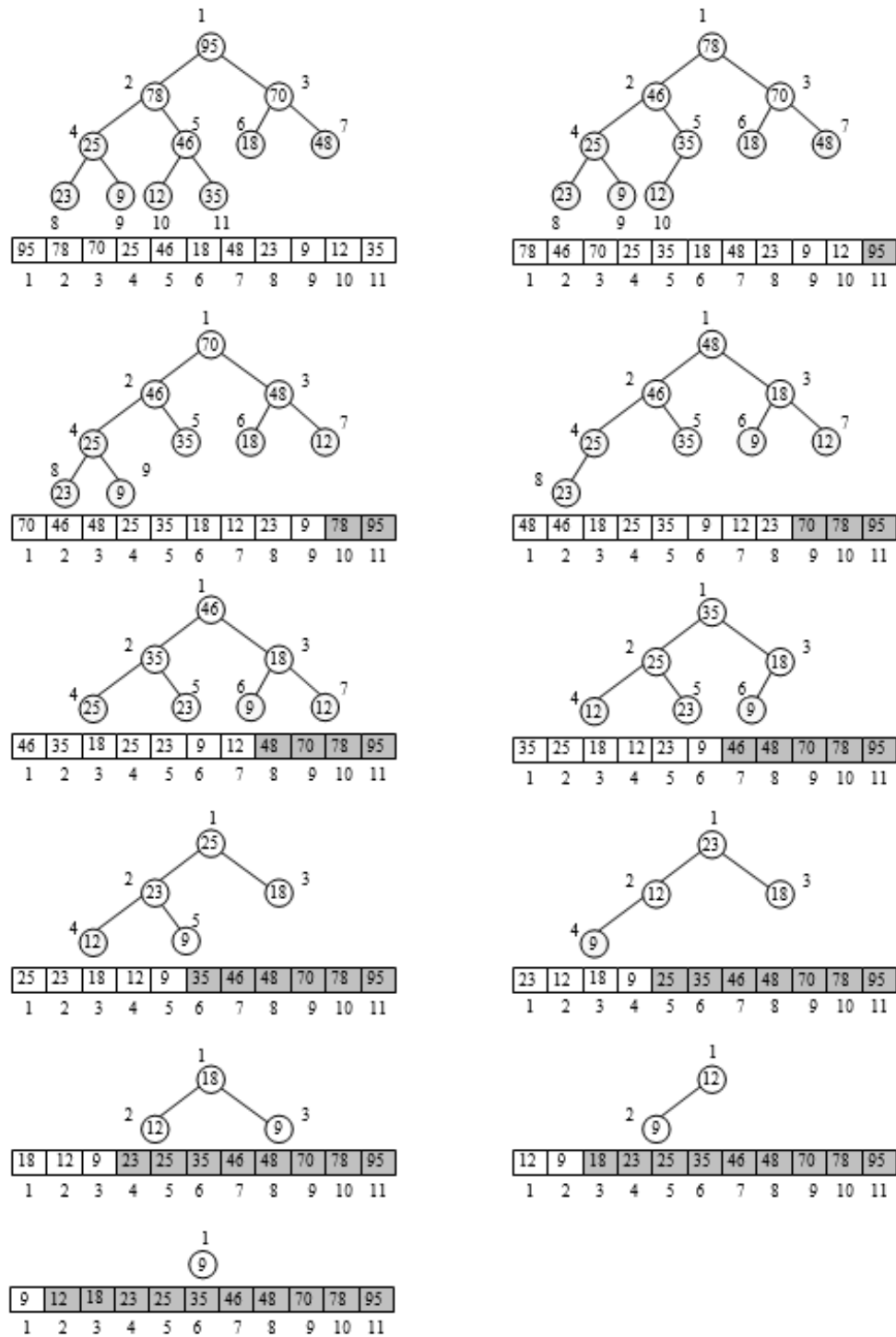
Figure 8.28 Heap sort
