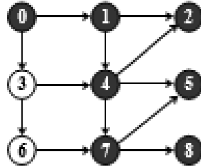
Figure 7.74 Visit vertex 7, 8
