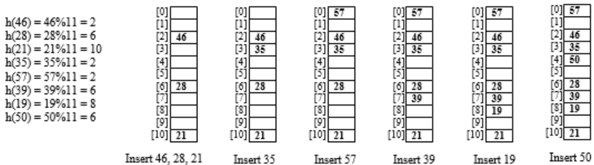
Figure 9.10 Quadratic probing
