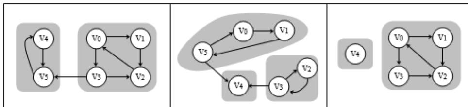
Figure 7.14 Strongly connected components
