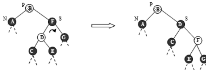
Figure 6.153 Case L_3a
