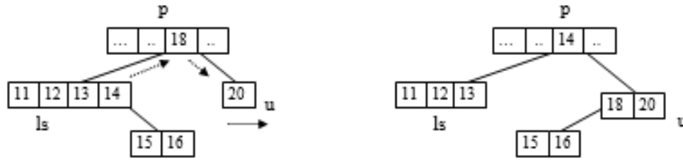
Figure 6.265 Borrow left
