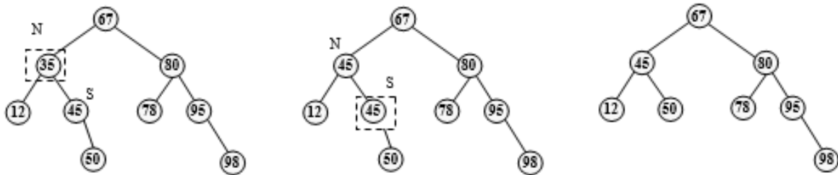
Figure 6.44 Deletion of 35
