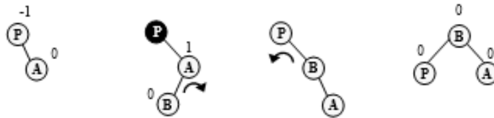
Figure 6.93 Case R_C2c
