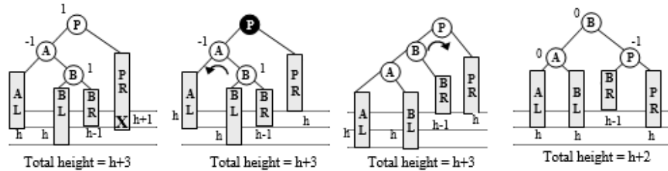
Figure 6.119 Case R_C3b
