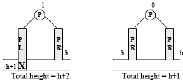
Figure 6.106 Case L_B
