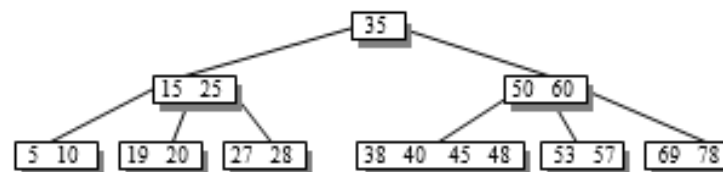
Figure 6.240 B-tree after deletion of 30
