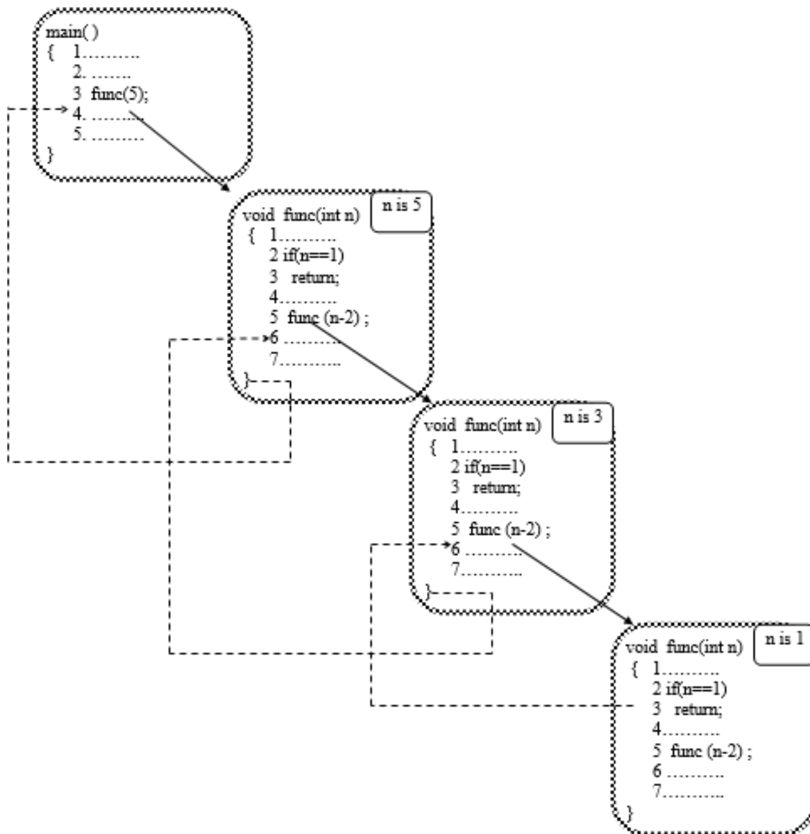
Figure 5.2 Flow of control in recursive method calls
