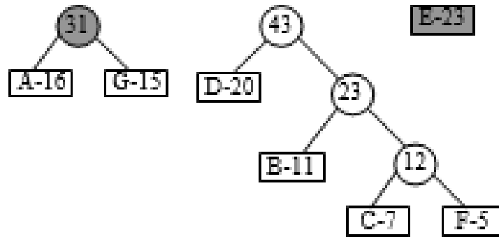
Figure 6.187 Trees weighted 20 and 23 are combined
