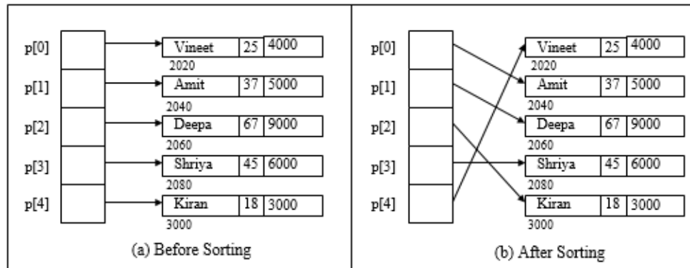
Figure 8.5 Sorting by rearranging references
