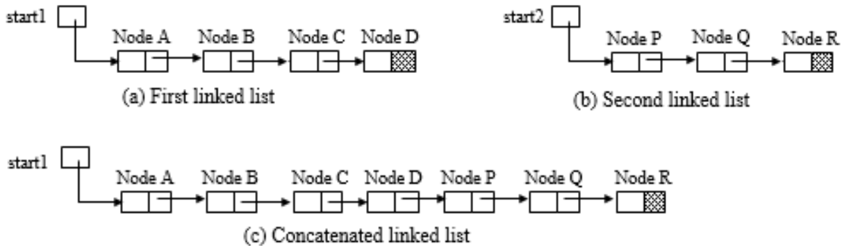
Figure 3.53 Concatenation of two linked lists
