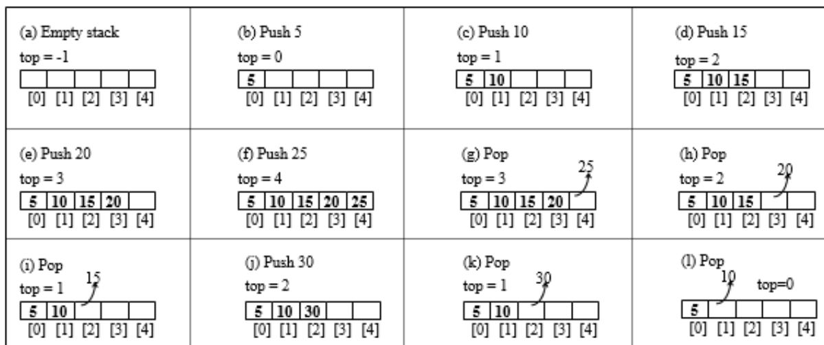
Figure 4.3 Array implementation of stack
