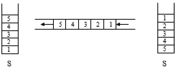
Figure 11.15 Reversing a stack using a queue
