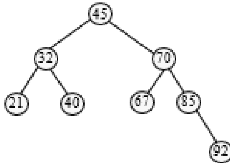
Figure 11.23 Binary search tree
