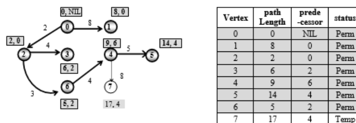
Figure 7.95 Make vertex 5 permanent
