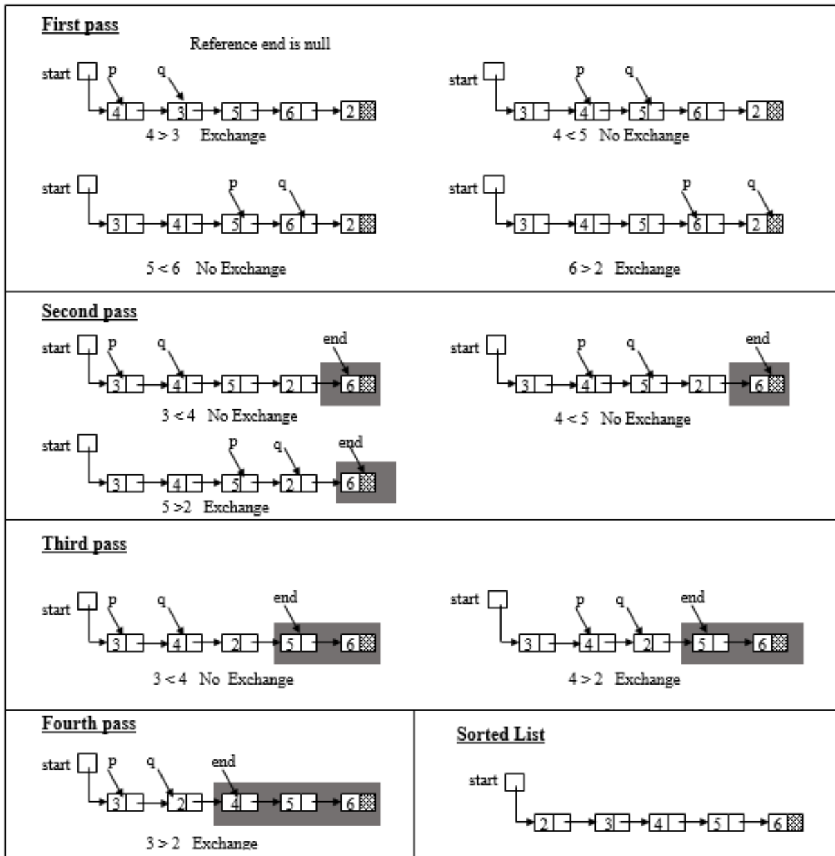
Figure 3.45 Bubble sort by exchanging data
