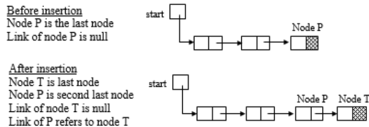
Figure 3.9 Insertion at the end of the list
