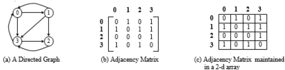
Figure 7.26 Adjacency matrix of a graph maintained in a 2-d array
