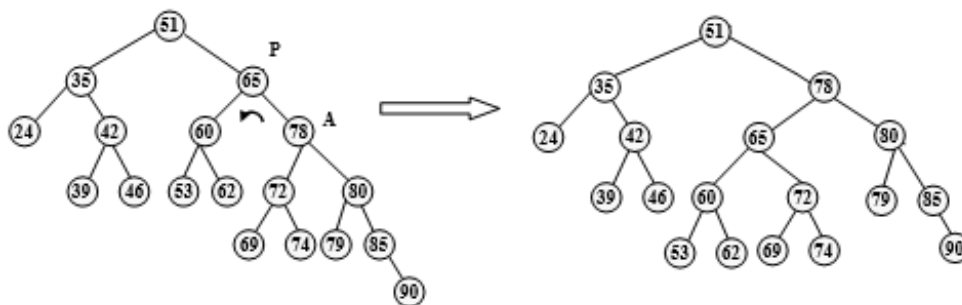
Figure 6.65 Left rotation about node 65
