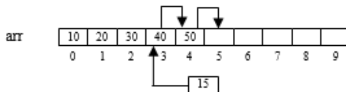
Figure 2.5 Insertion in between
