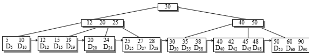
Figure 6.270 B+ tree after insertion of 42, 24
