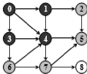
Figure 7.59 Visit 4, insert 5, 7 into the queue
