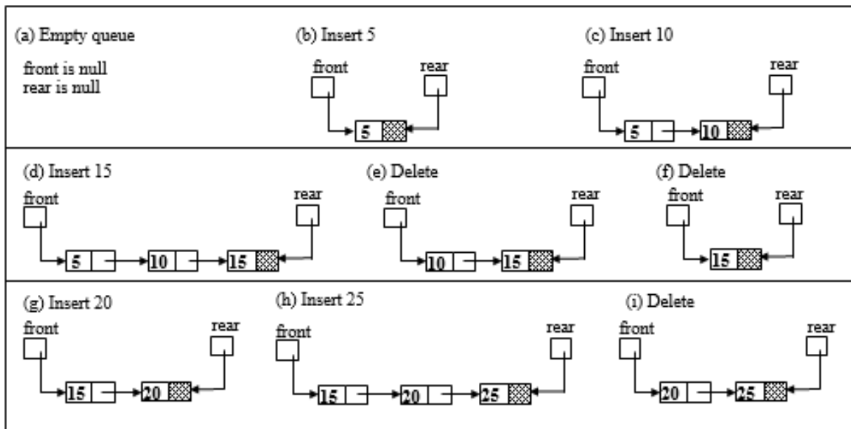
Figure 4.9 Linked list implementation of queue
