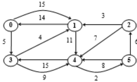
Figure 7.152 Graph to find shortest path using dijkstra's algorithm
