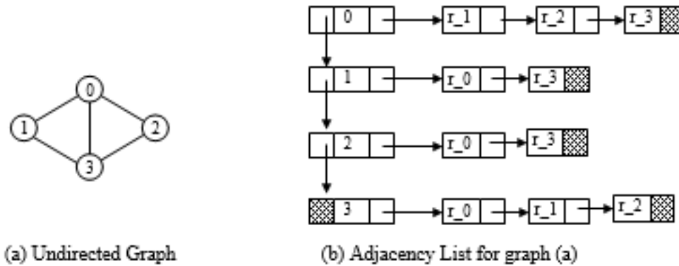
Figure 7.30 Adjacency list for an undirected graph
