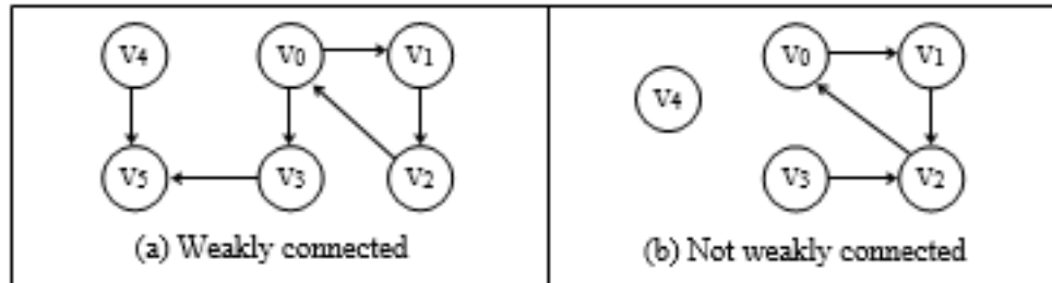
Figure 7.15 Weakly connected and not weakly connected graph
