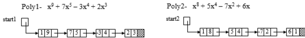
Figure 3.60 Two polynomial expressions for addition
