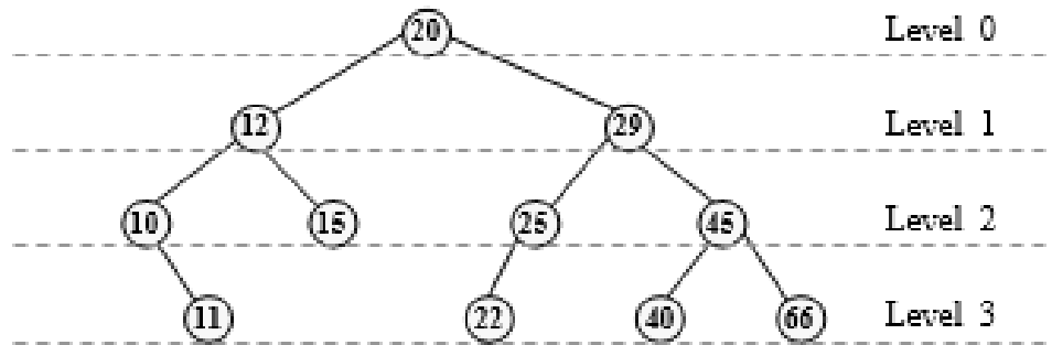
Figure 6.20 Level Order Traversal
