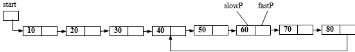
Figure 3.56 Cycle detection in a single linked list
