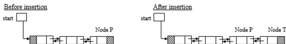
Figure 3.21 Insertion at the end of the list
