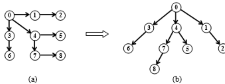
Figure 7.66 Breadth first search spanning tree
