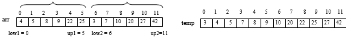
Figure 8.12 Merging of two sorted lists in same array
