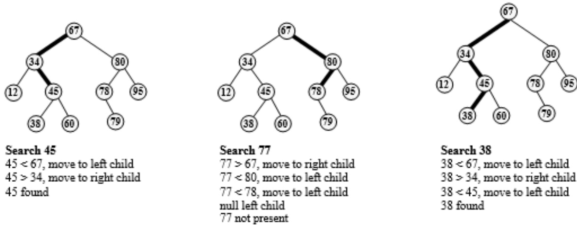
Figure 6.34 Searching in a binary search tree
