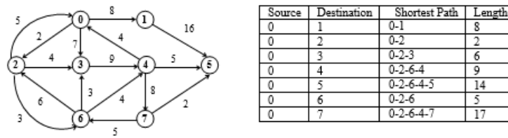
Figure 7.86 Shortest path from vertex 0 to others vertices for the graph
