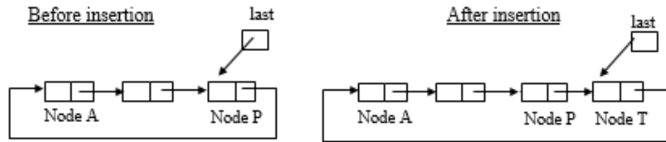
Figure 3.33 Insertion at the end of the list
