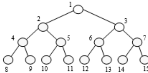
Figure 6.8 Full binary tree nodes numbered
