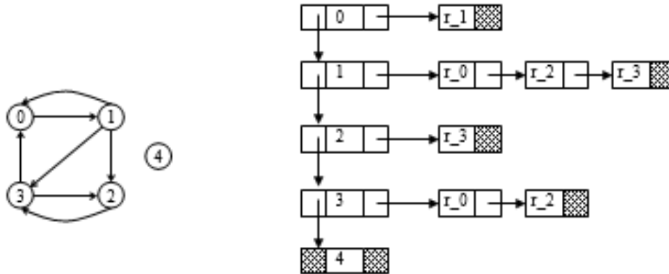
Figure 7.31 Insertion of a vertex
