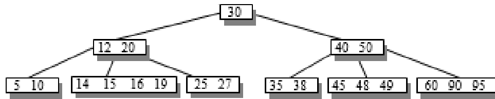
Figure 6.248 B-tree after insertion of 95
