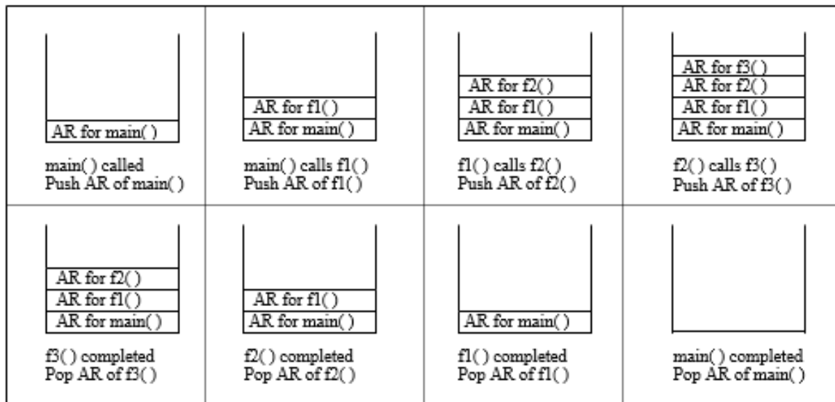
Figure 4.19 Stack for method calls
