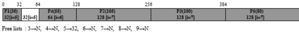
Figure 10.23 Allocate 80K for P5
