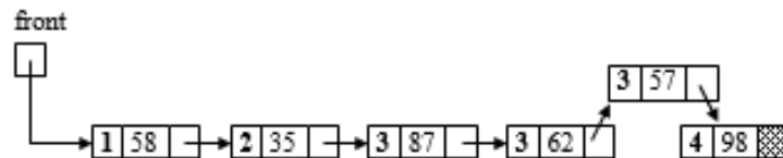
Figure 4.16 Insertion in priority queue
