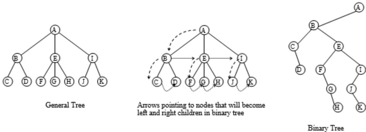
Figure 6.194 Example of general tree to binary tree
