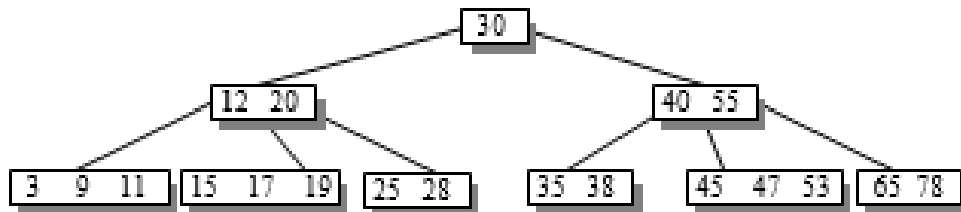
Figure 6.256 B-tree example for deleting 19
