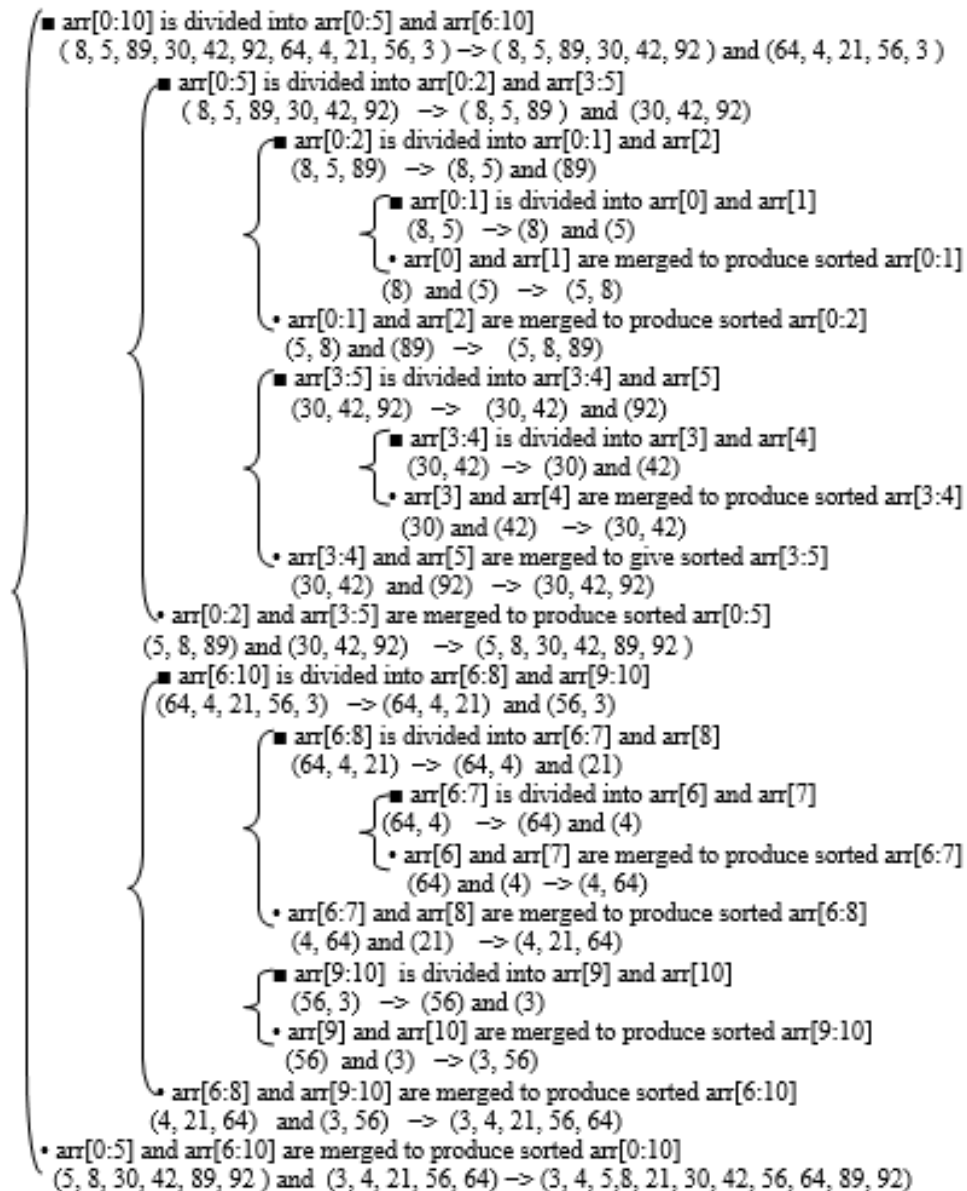
Figure 8.14 Top-down merge sort process
