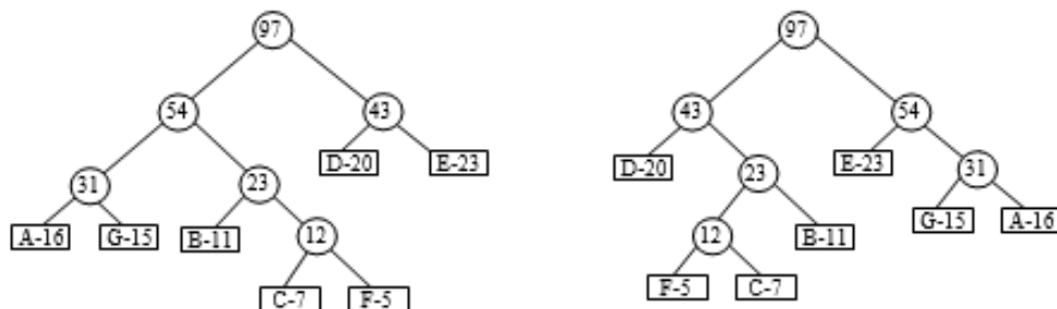
Figure 6.190 Huffman trees for same set of wiights
