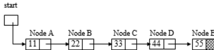
Figure 3.6 Single linked list example
