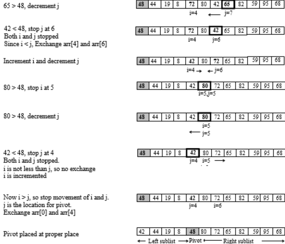
Figure 8.20 Partition process continued
