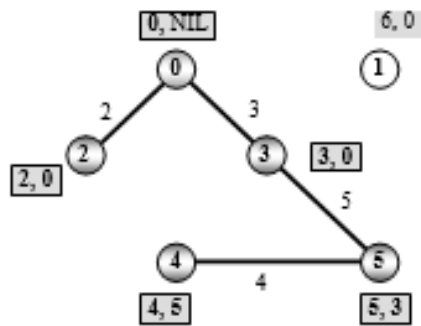
Figure 7.126 Make vertex 4 permanent
