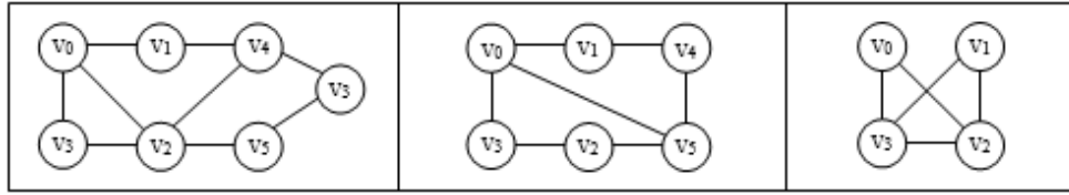
Figure 7.10 Biconnected graphs examples
