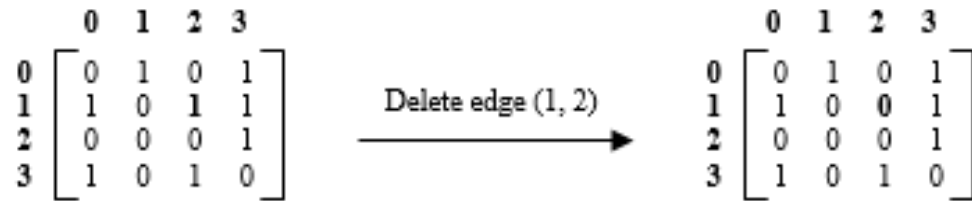
Figure 7.28 Deletion of an edge
