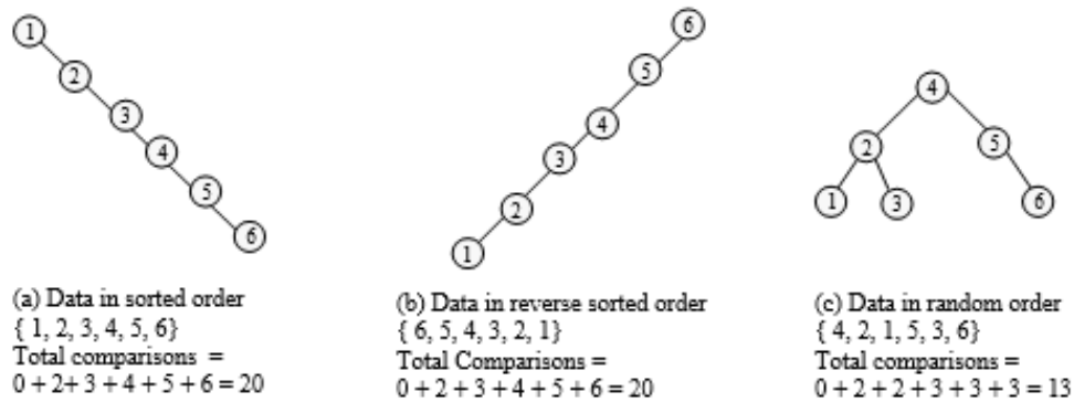
Figure 8.25 Binary search trees by inserting numbers in different order
