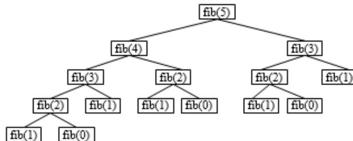
Figure 5.12 Recursive calls of method fib(5)
