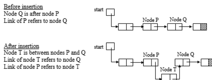
Figure 3.10 Insertion in between the list nodes
