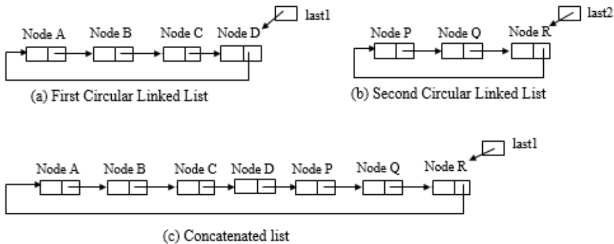
Figure 3.54 Concatenation of two circular linked lists
