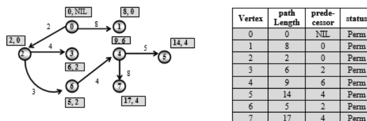
Figure 7.96 Make vertex 7 permanent
