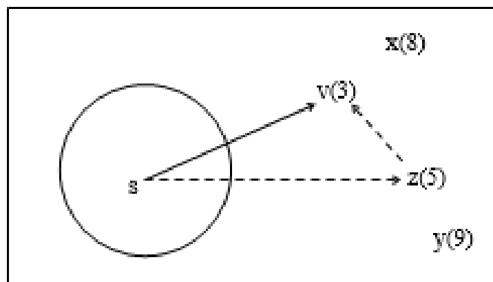
Figure 7.99 Shortest distance from s to v
