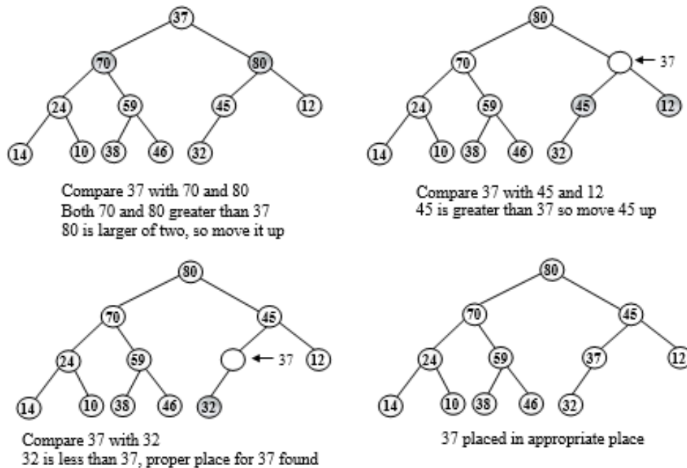
Figure 6.177 Placing key 37 at appropriate place
