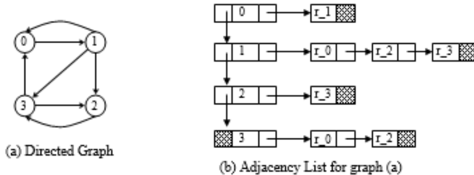
Figure 7.29 Adjacency list for a directed graph
