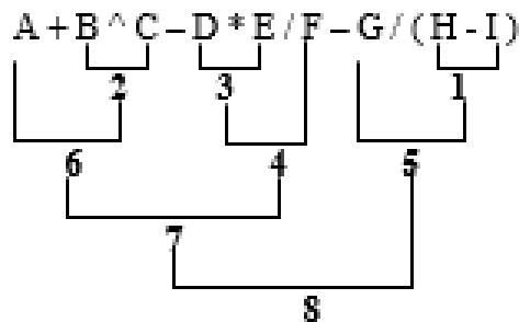
Figure 4.22 Arithmetic expression with parentheses evaluation
