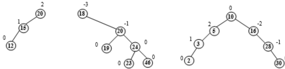
Figure 6.58 Binary search trees (Non-AVL trees) with balance factor
