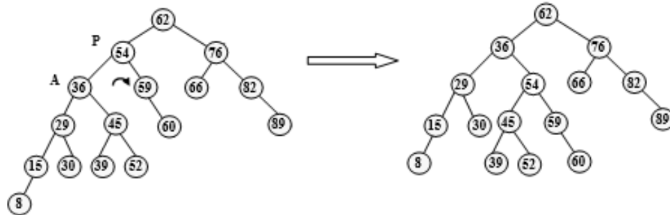
Figure 6.61 Right rotation about node 54
