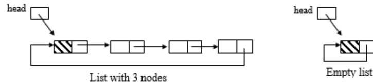
Figure 3.39 Circular single linked list with header
