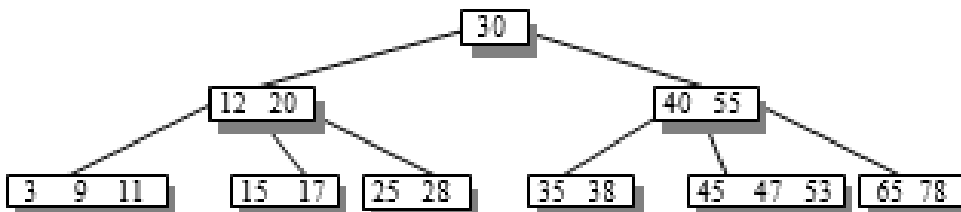
Figure 6.257 B-tree after deletion of 19
