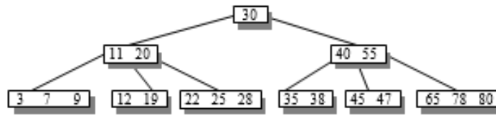
Figure 6.217 B-tree after deletion of 15
