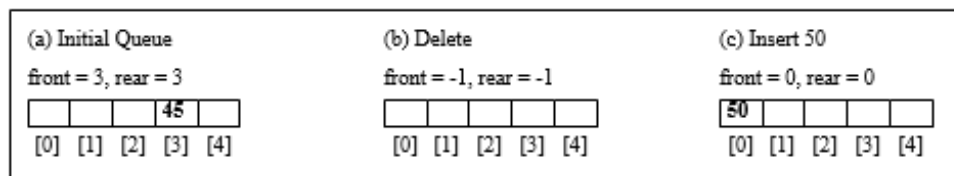
Figure 4.13 Circular queue operations example
