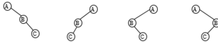
Figure 11.29 Binary trees with same preorder and postorder traversals
