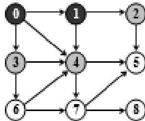
Figure 7.57 Visit 1, insert 2 into the queue
