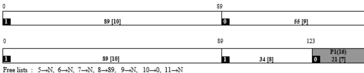
Figure 10.33 Allocate 16K for P1
