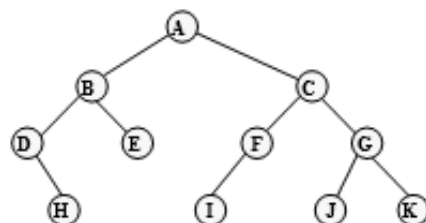
Figure 6.18 Binary tree traversals
