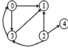
Figure 11.37 Graph from adjacency tree
