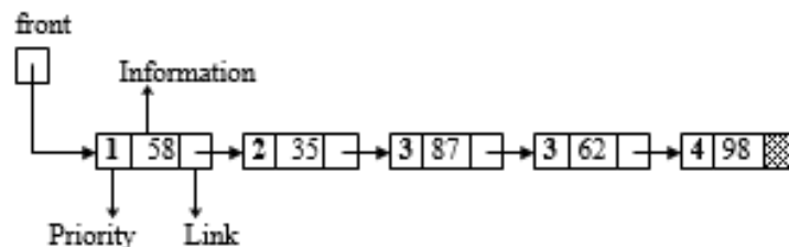
Figure 4.15 Priority queue example
