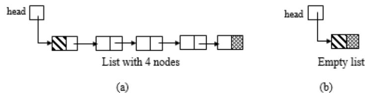
Figure 3.38 Single linked list with header node
