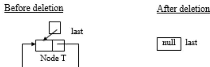
Figure 3.35 Deletion of the only node
