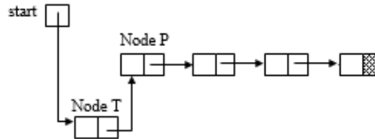
Figure 3.7 Insertion at the beginning of the list
