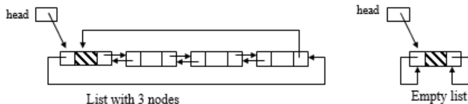
Figure 3.41 Doubly linked circular list with header
