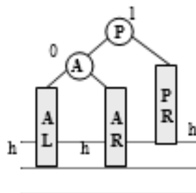
Figure 6.73 Root A for subtree PL
