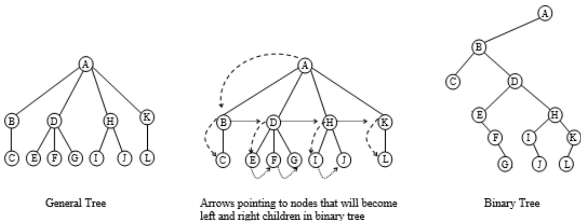
Figure 6.195 Another example of general tree to binary tree
