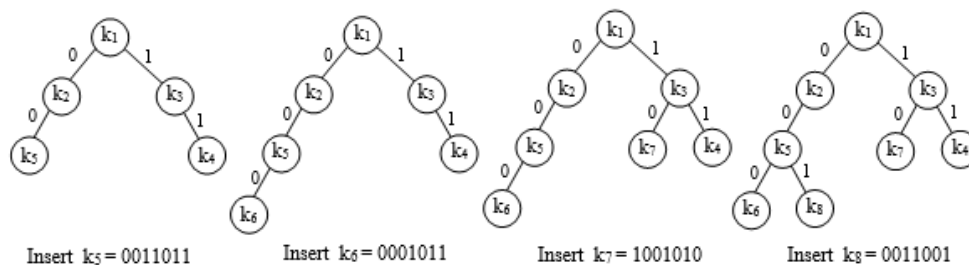
Figure 6.276 Inserting keys into digital search tree continued
