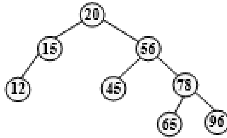
Figure 6.55 Binary search tree
