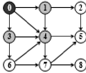
Figure 7.56 Visit 0, insert 1, 3, 4 into the queue
