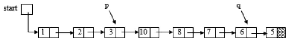
Figure 3.48 Selection sort by rearranging links - 3
