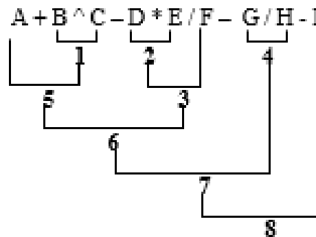
Figure 4.21 Arithmetic expression evaluation
