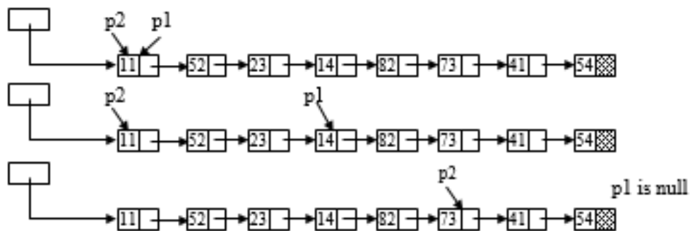
Figure 11.5 Getting n^{\text{th}} node from end of a single linked list
