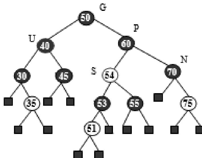
Figure 6.131 Relatives of node 70
