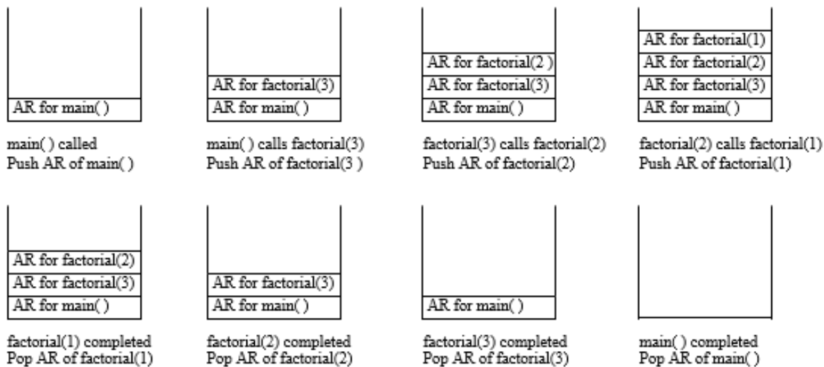
Figure 5.18 Recursive method factorial(3) evaluation in stack
