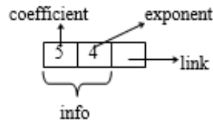
Figure 3.58 Node in polynomial expression
