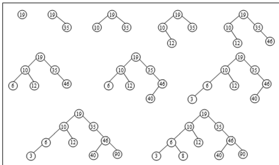
Figure 8.23 Binary tree sort
