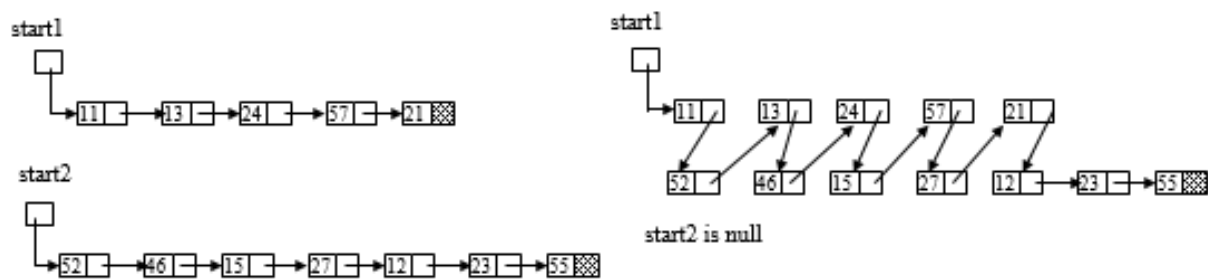
Figure 11.7 Combining alternate nodes of two lists
