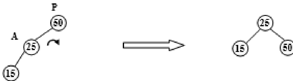
Figure 6.62 Right rotation about node 50
