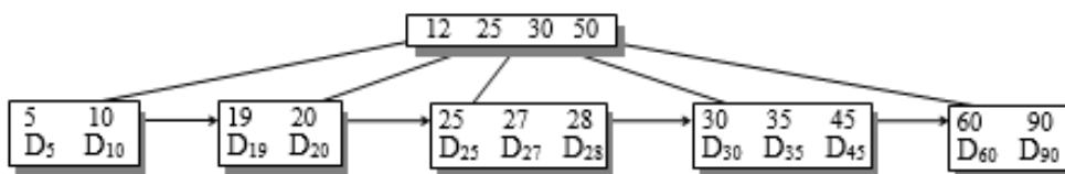
Figure 6.274 B+ tree after deletion of 48
