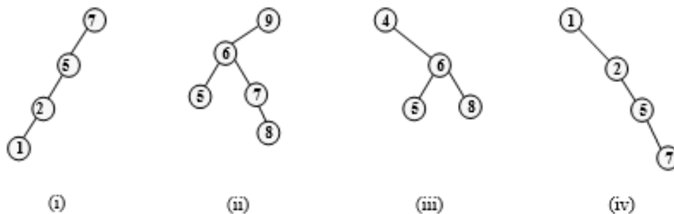
Figure 6.279 Binary search trees
