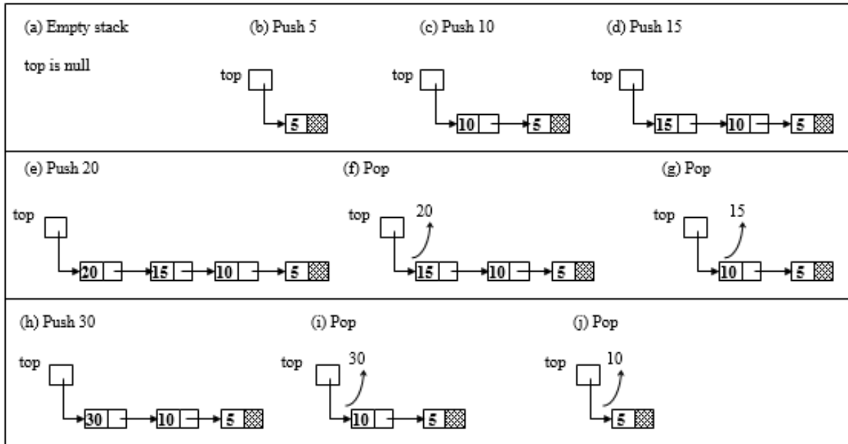
Figure 4.4 Linked list implementation of stack
