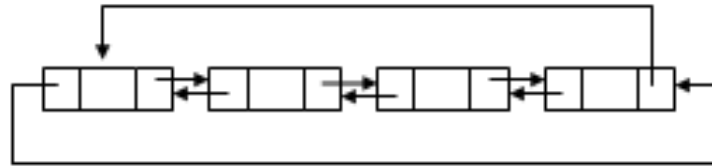
Figure 3.37 Circular doubly linked list
