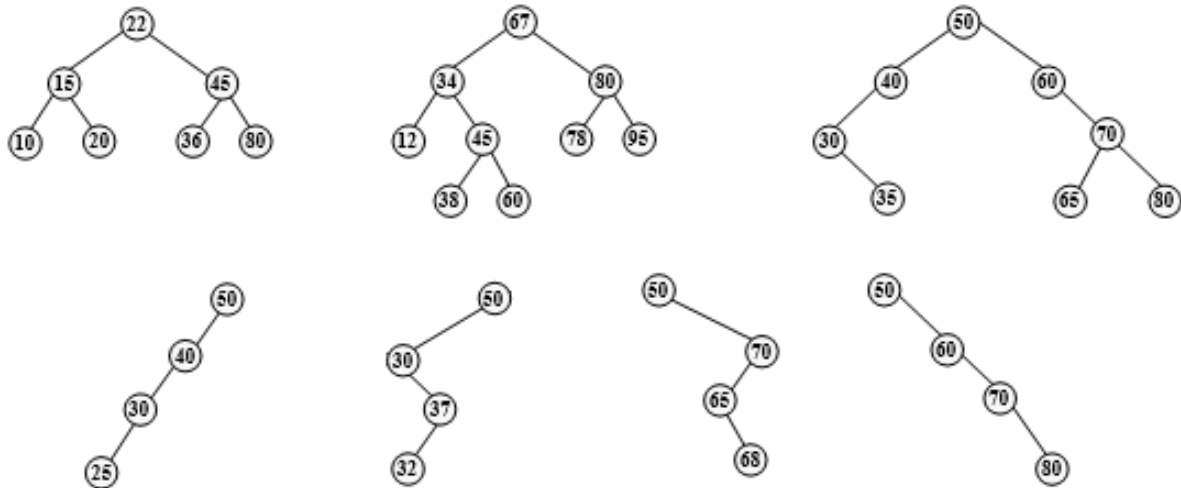
Figure 6.32 Binary search tree examples
