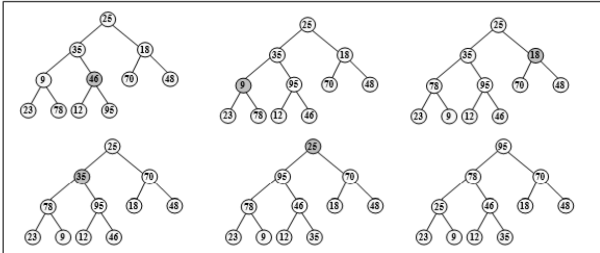
Figure 6.181 Building heap using bottom up approach
