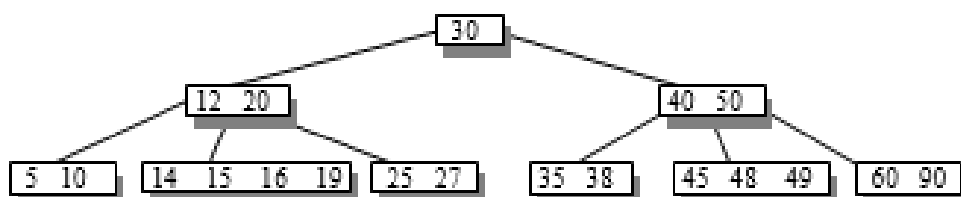
Figure 6.244 B-tree example for inserting 17
