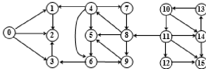
Figure 7.79 Directed graph for DFS
