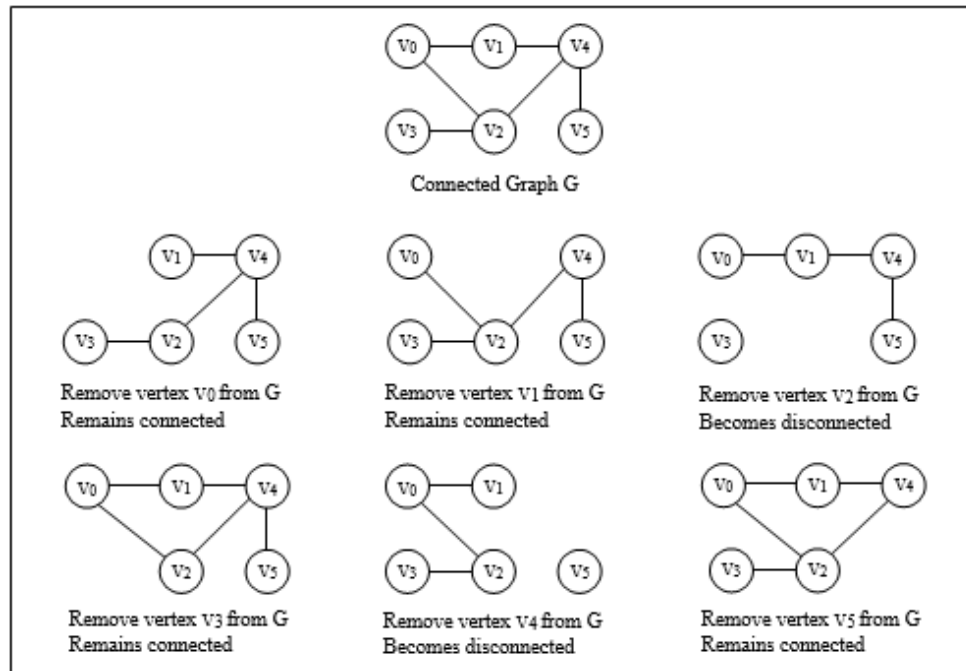
Figure 7.8 Graphs examples to find articulation points
