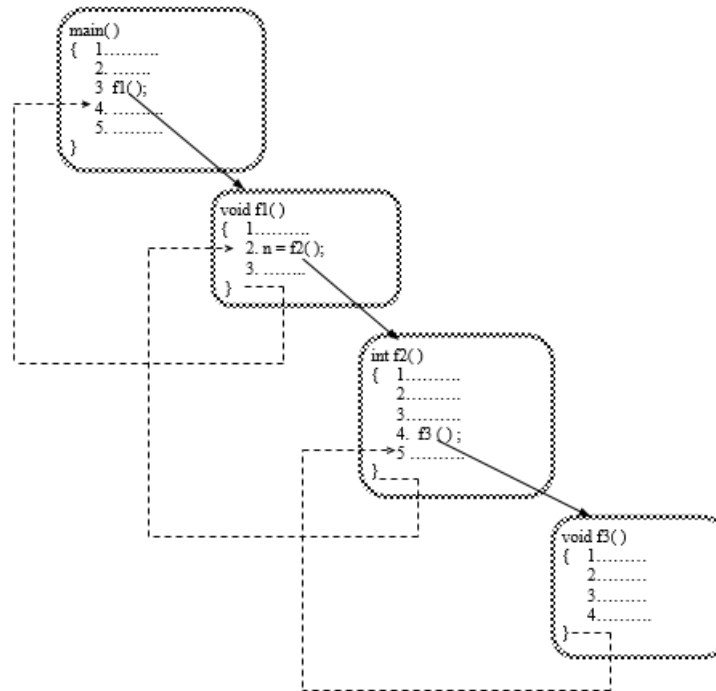
Figure 5.1 Flow of control in normal method calls
