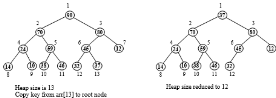
Figure 6.176 Deleting root key from a heap
