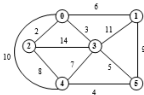
Figure 7.119 Weighted undirected connected graph
