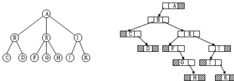
Figure 6.196 Linked representation of a general tree
