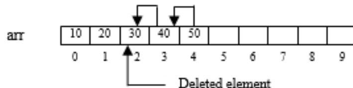
Figure 2.7 Deletion in between
