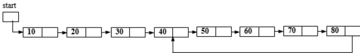
Figure 3.55 Single linked list with cycle
