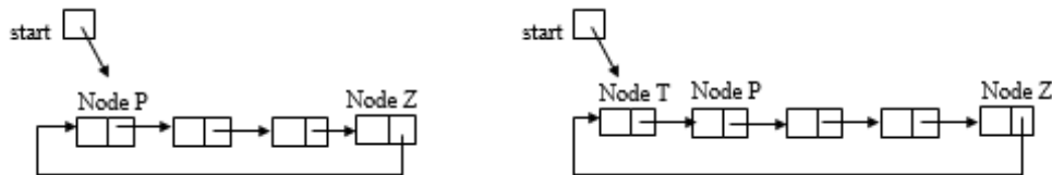
Figure 3.30 Circular list with a reference referring to first node
