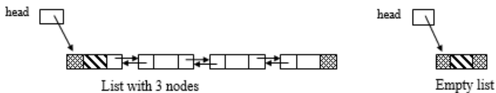
Figure 3.40 Doubly linked list with header
