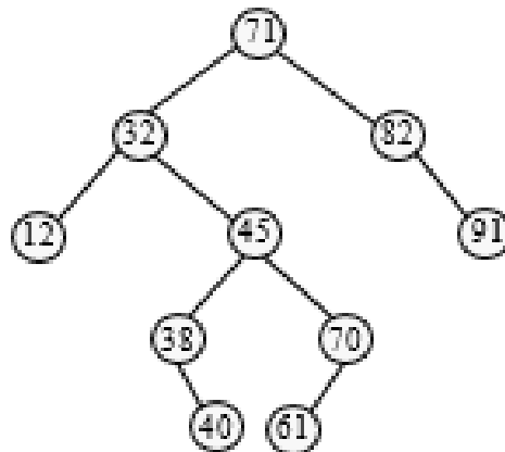
Figure 11.24 Binary search tree
