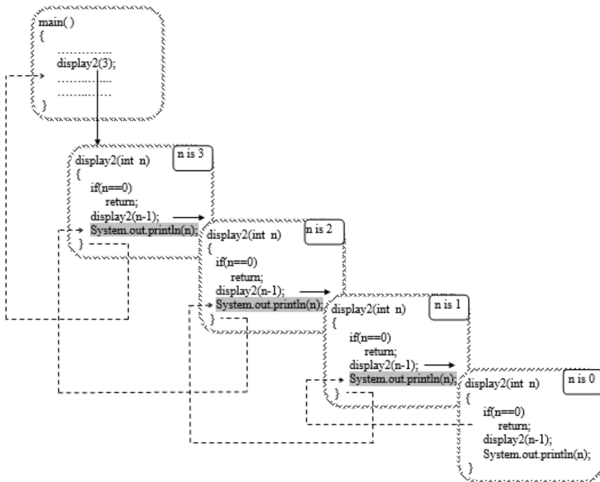
Figure 5.8 Displaying numbers from 1 to n
