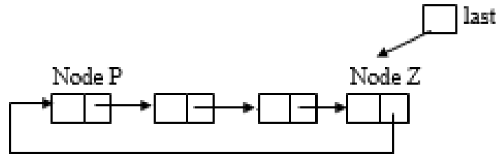
Figure 3.29 Circular list with a reference referring to last node
