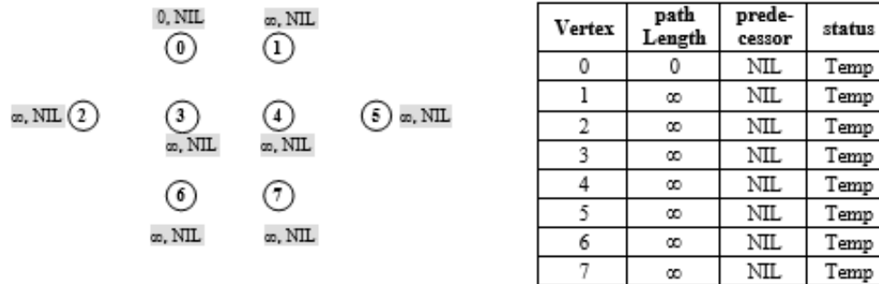
Figure 7.88 Initial graph and table for path length, predecessor, status of vertex
