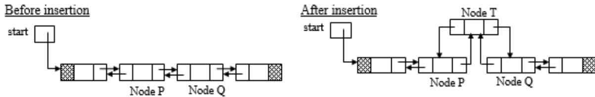
Figure 3.22 Insertion in between the nodes
