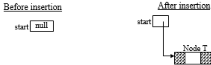
Figure 3.20 Insertion in an empty list
