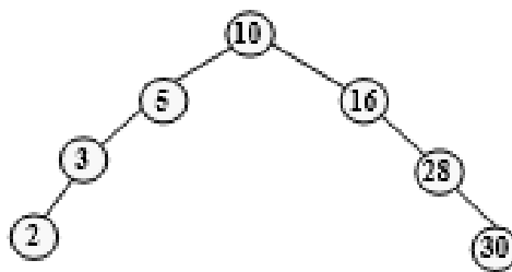
Figure 6.56 Binary search tree
