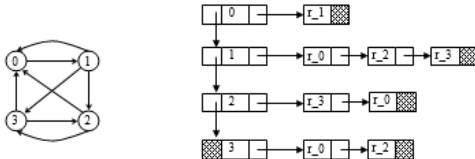
Figure 7.32 Insertion of an edge
