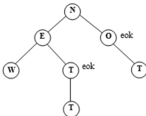
Figure 6.278 Keys in trie
