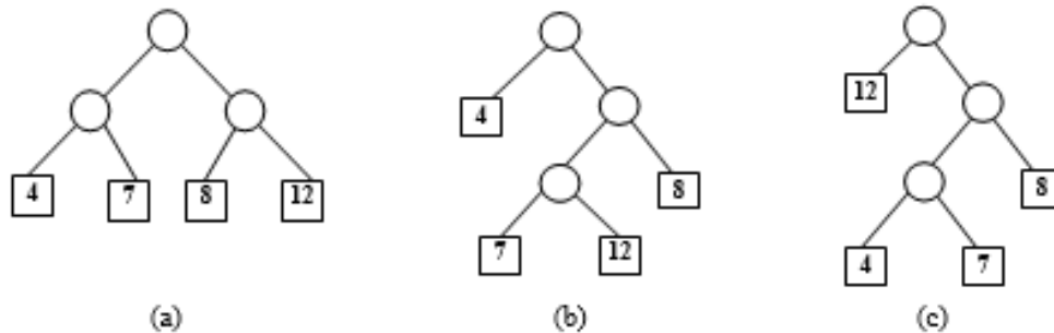
Figure 6.182 Extended binary trees with weights
