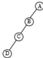
Figure 11.26 Binary tree with same inorder and postorder traversals
