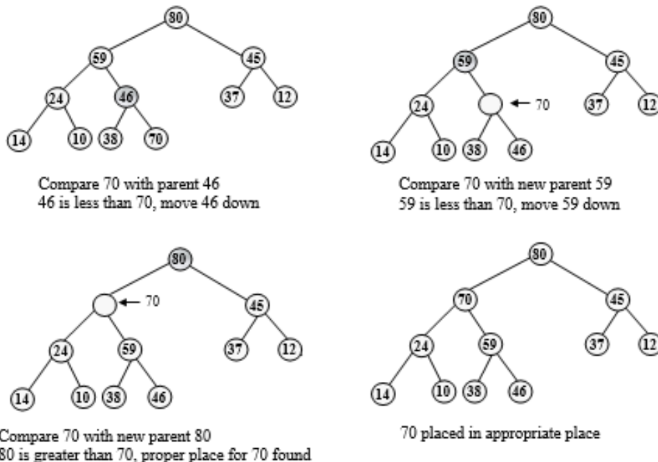
Figure 6.172 Placing 70 at appropriate place
