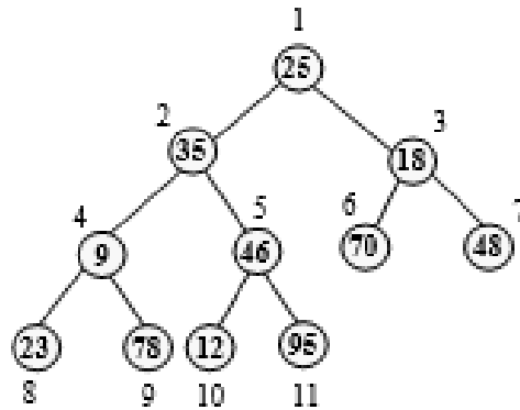
Figure 6.180 Array representing a complete binary tree
