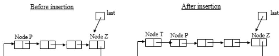
Figure 3.31 Insertion at the beginning of the list
