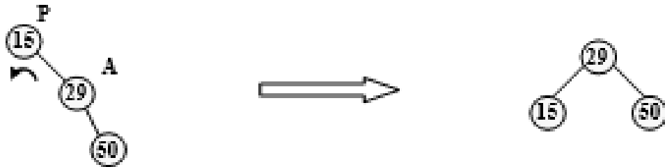
Figure 6.66 Left rotation about node 15
