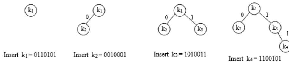
Figure 6.275 Inserting keys into digital search tree
