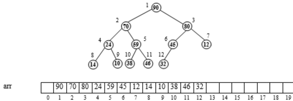
Figure 6.170 Array representation of a heap
