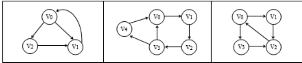
Figure 7.12 Strongly connected graphs
