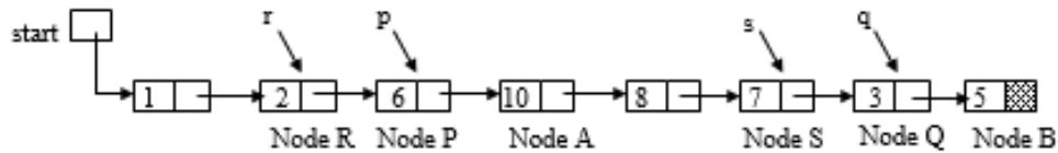
Figure 3.46 Selection sort by rearranging links - 1
