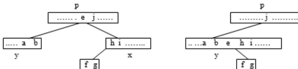
Figure 6.267 Combining two nodes
