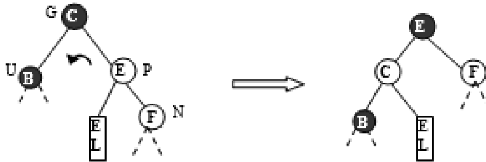
Figure 6.137 Case R 2b
