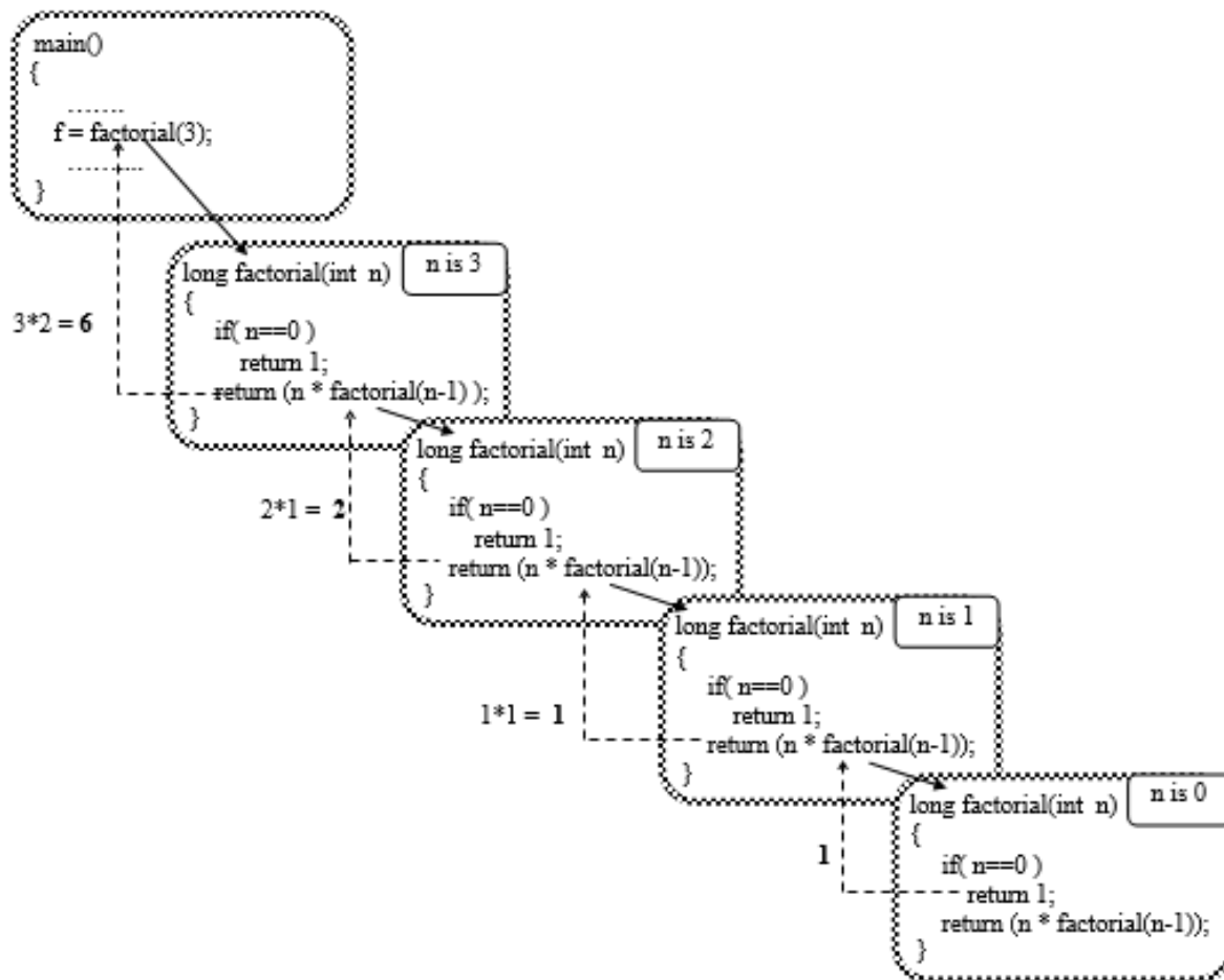
Figure 5.4 Finding factorial of a number recursively
