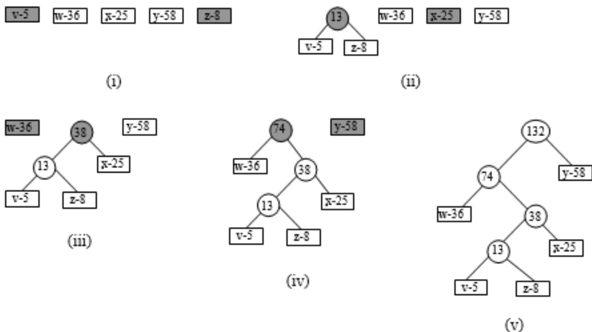
Figure 6.192 Creation of huffman tree
