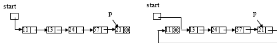
Figure 11.1 Removing first node and inserting at end
