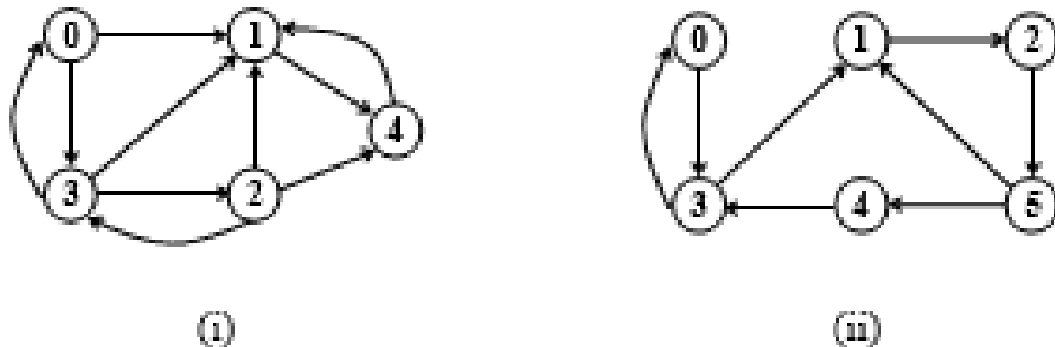
Figure 7.150 Graphs to check if it is strongly connected
