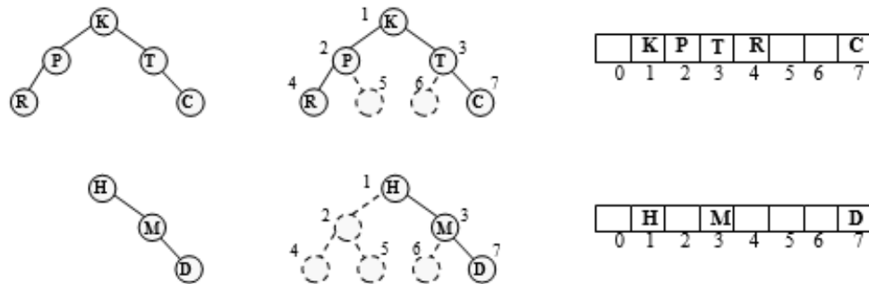
Figure 6.12 Binary trees array representation
