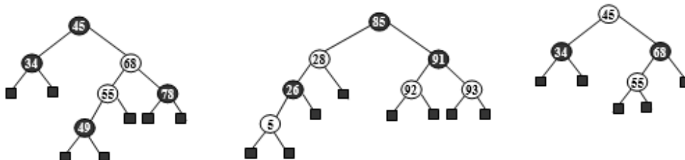
Figure 6.130 Trees violating red black tree properties
