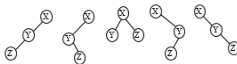
Figure 11.21 Binary trees of 3 nodes having preorder XYZ
