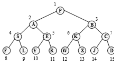
Figure 6.10 Numbering for full binary tree
