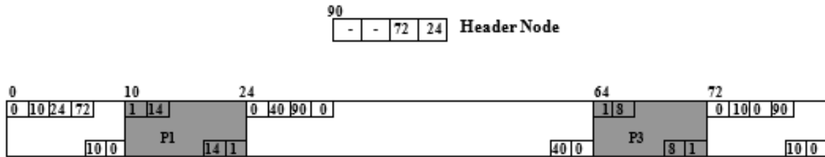
Figure 11.45 Deallocated the memory block P2 using Boundary tag method
