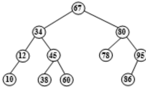
Figure 6.33 Binary search tree
