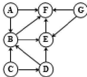
Figure 7.137 Directed graph representing the table
