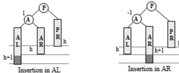
Figure 6.74 Two cases of insertion
