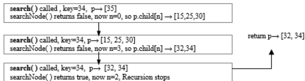
Figure 6.242 Search 34
