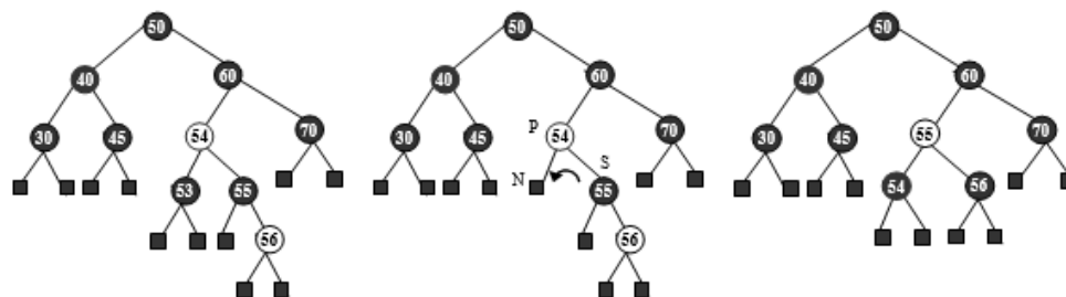
Figure 6.164 Delete 53
