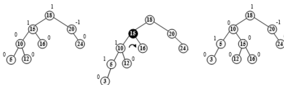
Figure 6.77 Insertion of 3
