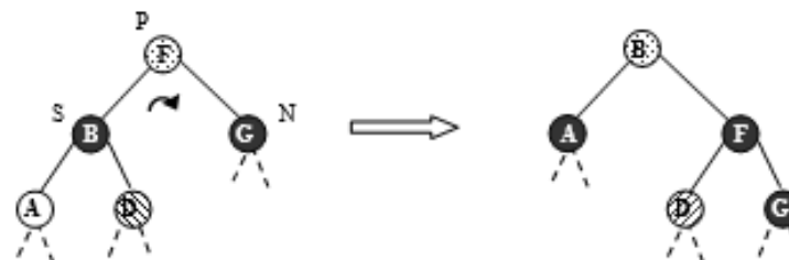
Figure 6.159 Case R_3b
