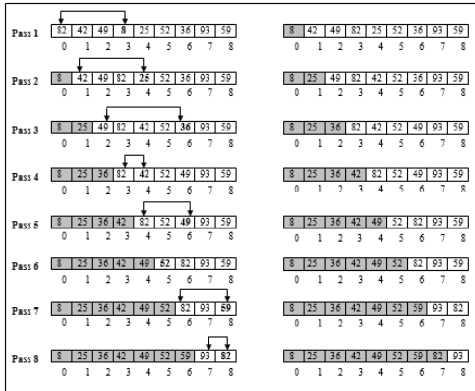
Figure 8.6 Selection sort
