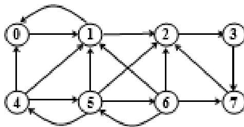
Figure 7.151 Graph to find strongly connected components
