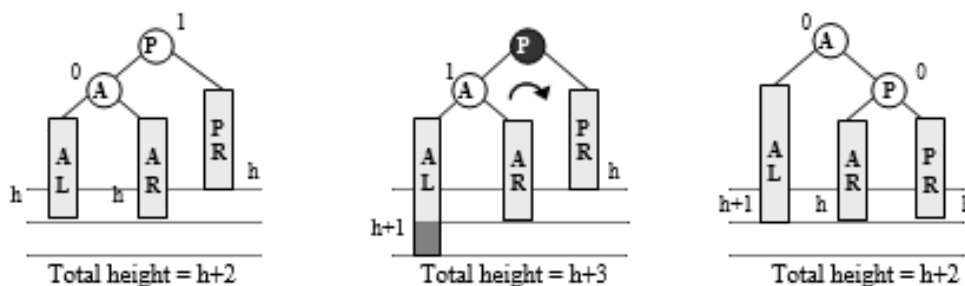
Figure 6.75 Case L_C1
