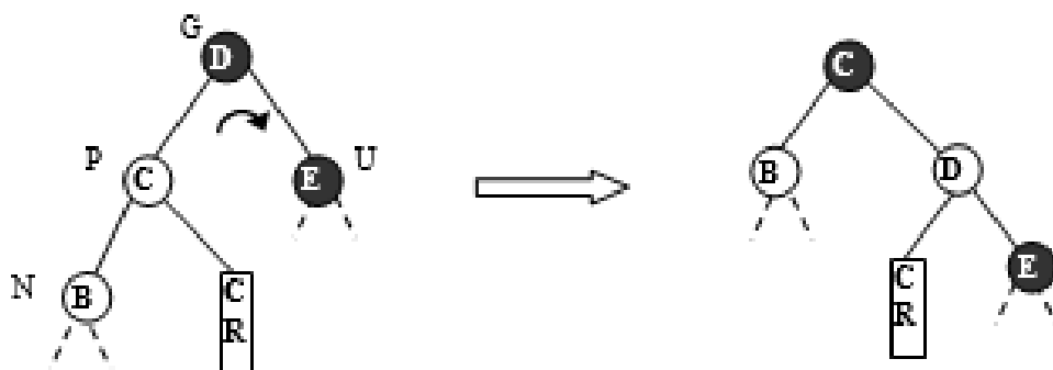
Figure 6.134 Case L_2b
