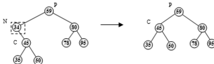
Figure 6.40 Deletion of 34
