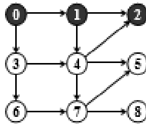
Figure 7.72 Visit vertex 0, 1, 2
