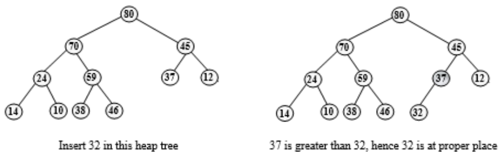
Figure 6.174 Insert 32
