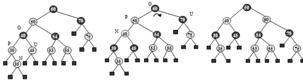
Figure 6.146 Insert 35
