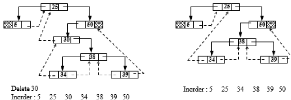
Figure 6.51 Deletion of 30
