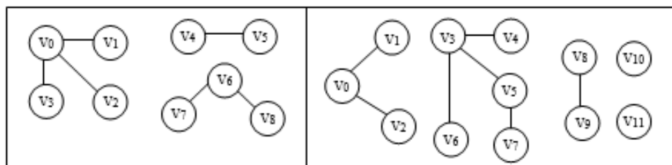
Figure 7.18 Forest
