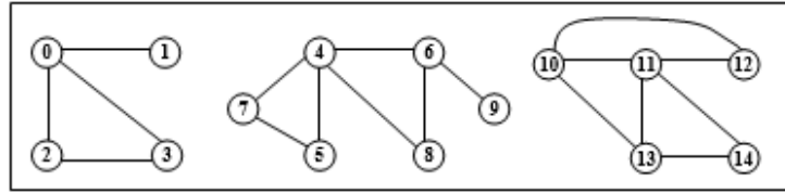
Figure 7.81 Undirected graph for DFS
