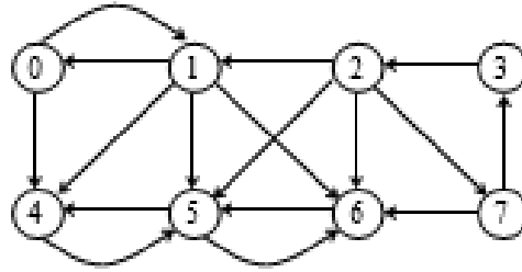
Figure 11.41 Reverse graph
