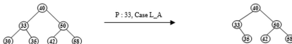
Figure 6.125 Delete 30
