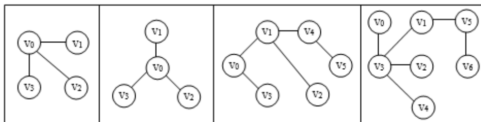
Figure 7.16 Examples of trees
