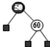
Figure 6.139 Insert 60
