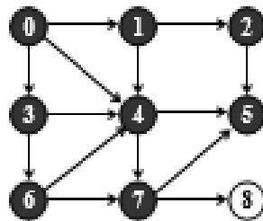
Figure 7.53 Visit 2, 6, 5, 7
