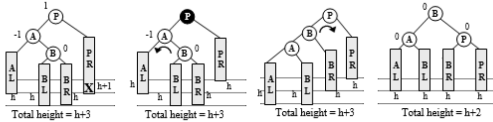
Figure 6.118 Case R_C3a
