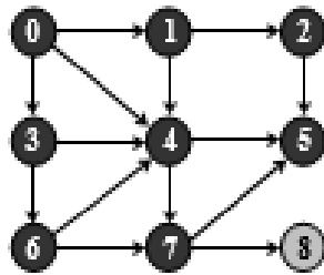
Figure 7.63 Visit 7, insert 8 into the queue
