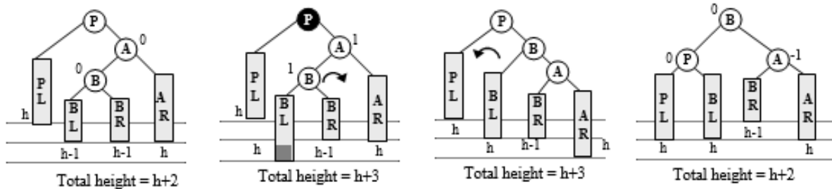
Figure 6.92 Case R_C2b
