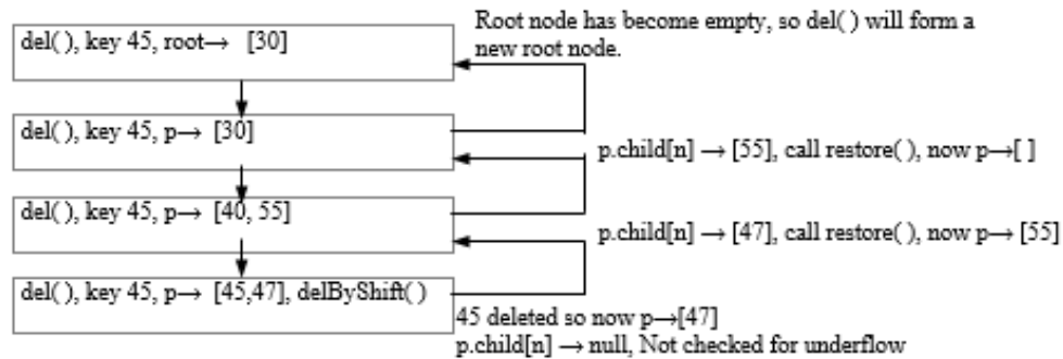
Figure 6.264 Deletion of 45
