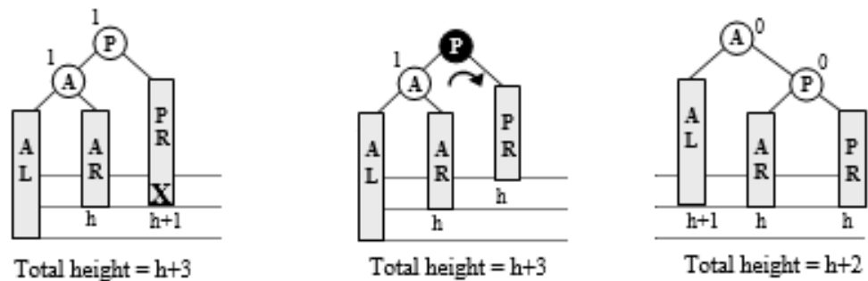
Figure 6.117 Case R_C2
