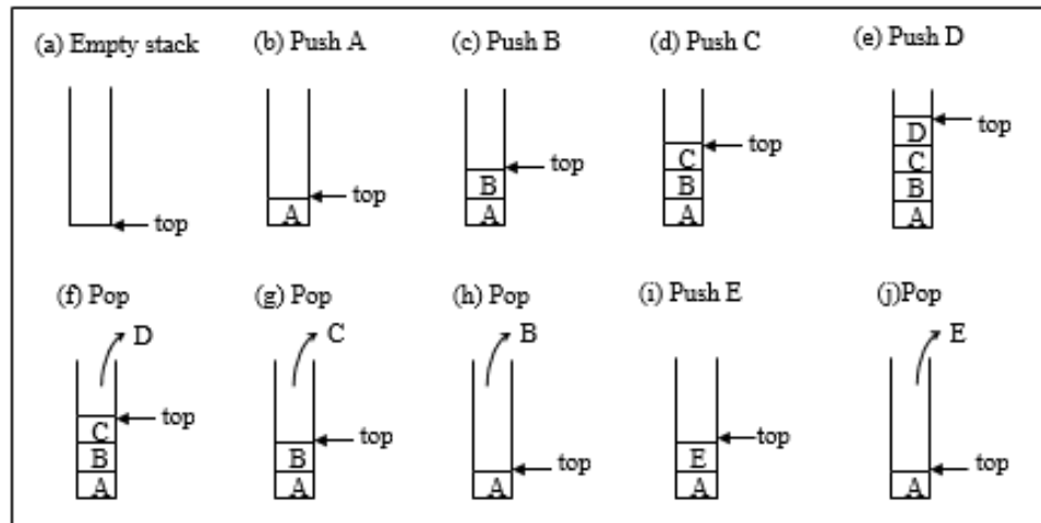
Figure 4.2 Stack operations
