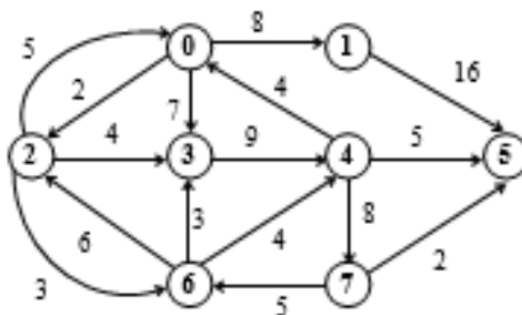
Figure 7.87 Graph for finding shortest paths
