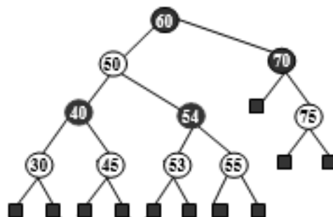
Figure 6.145 Insert 30, 45
