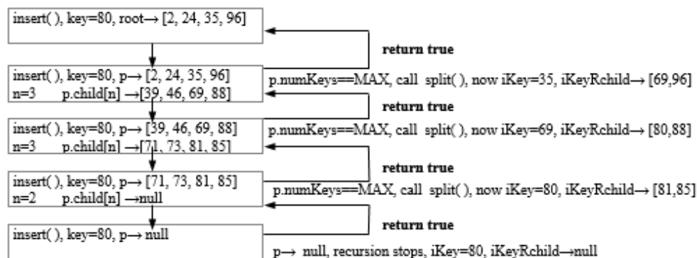
Figure 6.252 Insertion of 80
