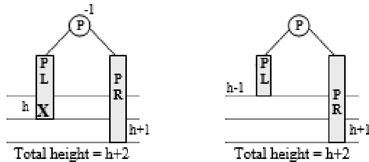
Figure 6.107 Case L_C
