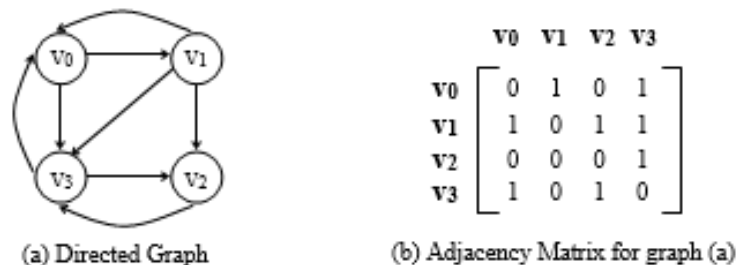
Figure 7.22 Adjacency matrix for a directed graph
