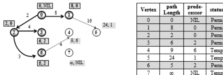
Figure 7.93 Make vertex 1 permanent
