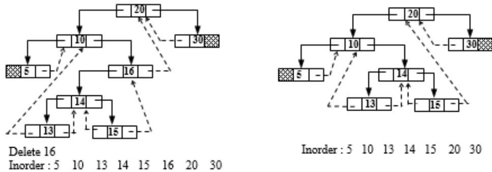
Figure 6.50 Deletion of 16
