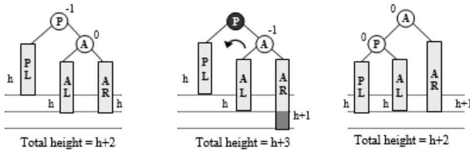
Figure 6.87 Case R_C1
