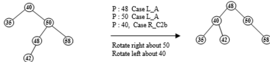
Figure 6.100 Insert 42
