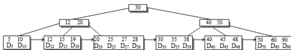
Figure 6.269 B+ tree example
