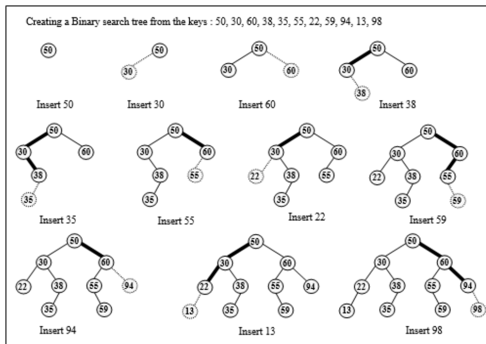
Figure 6.36 Creation of binary search tree
