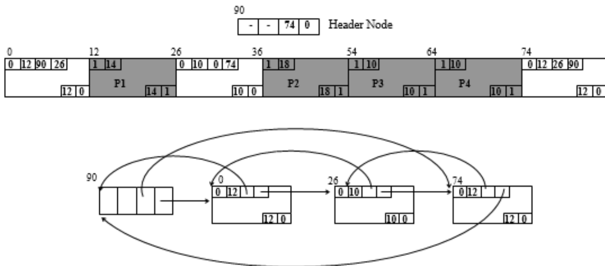
Figure 10.13 Program allocation in memory and free list
