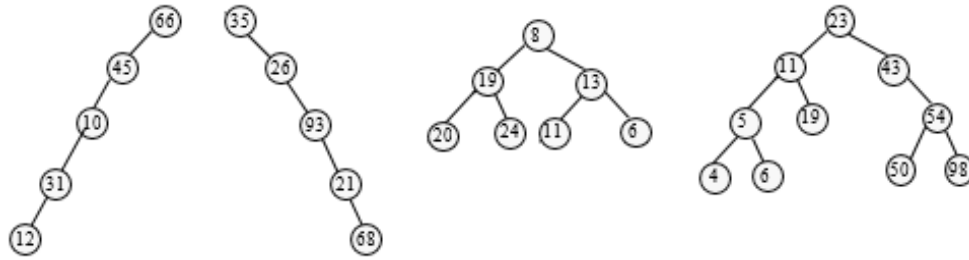
Figure 11.28 Binary trees from inorder and postorder traversals
