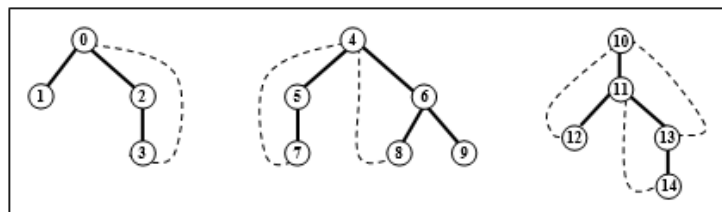
Figure 7.83 Tree edges and back edges for the undirected graph
