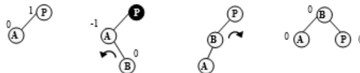
Figure 6.81 Case L_C2c
