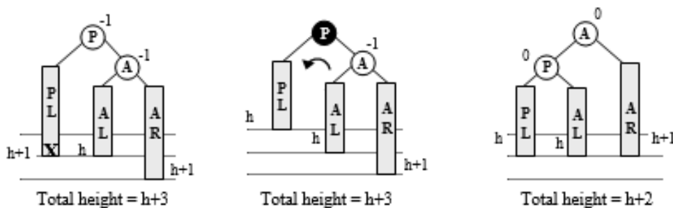
Figure 6.109 Case L_C2
