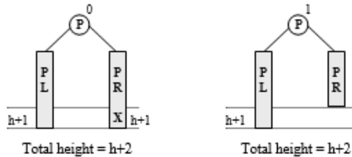
Figure 6.114 Case R_A
