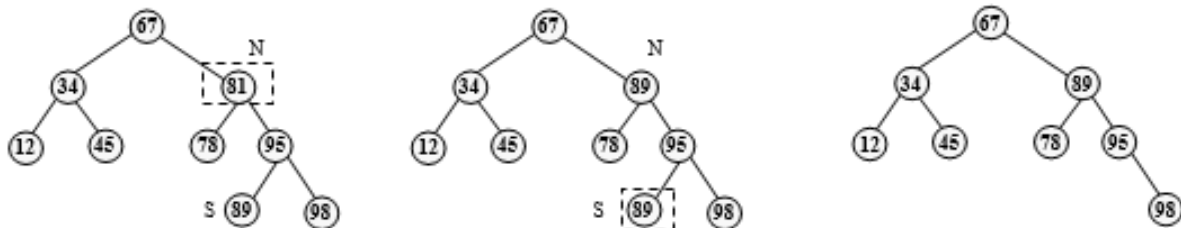
Figure 6.42 Deletion of 81
