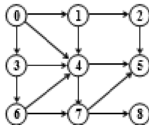
Figure 7.51 Graph for breadth first search traversal
