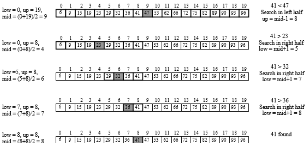
Figure 9.3 Search 41
