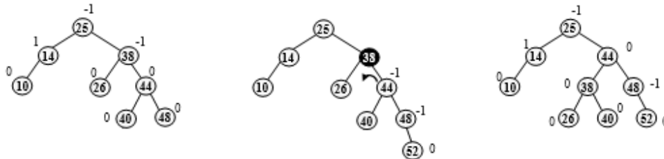
Figure 6.89 Insertion of 52
