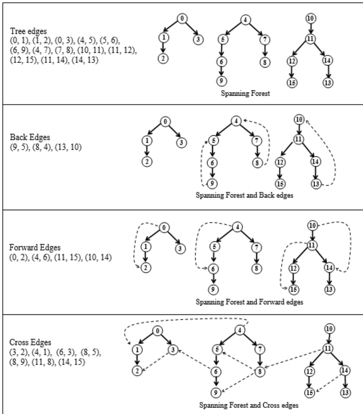
Figure 7.80 DFS spanning forest and different types of edges
