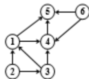
Figure 7.140 Delete the vertex 0 and edges going from vertex 0
