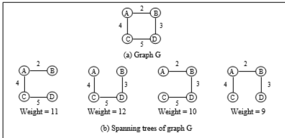
Figure 7.118 Graph and its spanning trees
