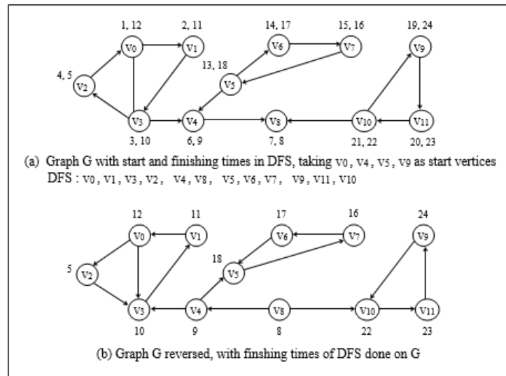
Figure 7.84 Finding strongly connected graph and strongly connected components
