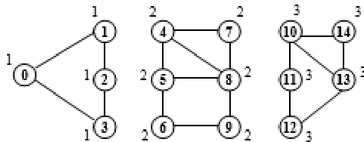
Figure 7.70 Connected components with label
