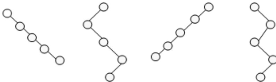
Figure 6.4 Skew trees
