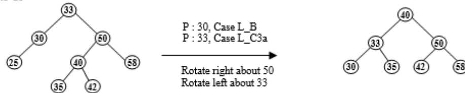
Figure 6.124 Delete 25
