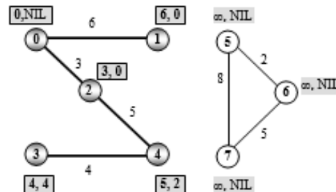
Figure 7.129 Vertex 5, 6, 7 are left temporary
