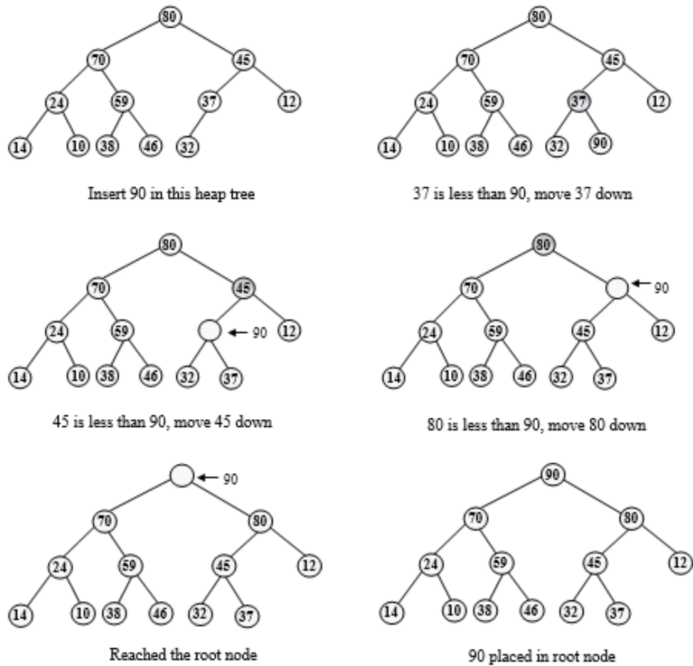
Figure 6.173 Insert 90
