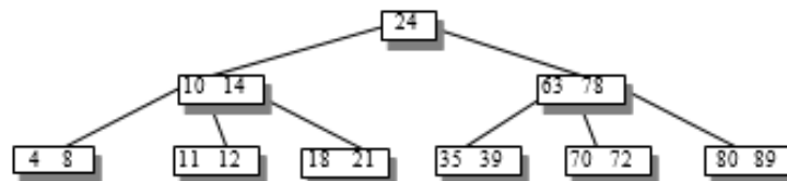
Figure 11.36 B-tree
