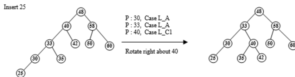
Figure 6.104 Insert 25
