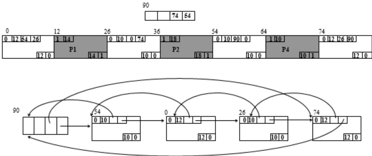
Figure 10.14 Free P3
