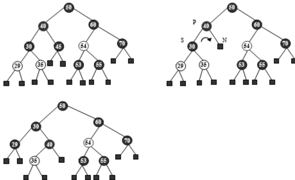
Figure 6.163 Delete 45
