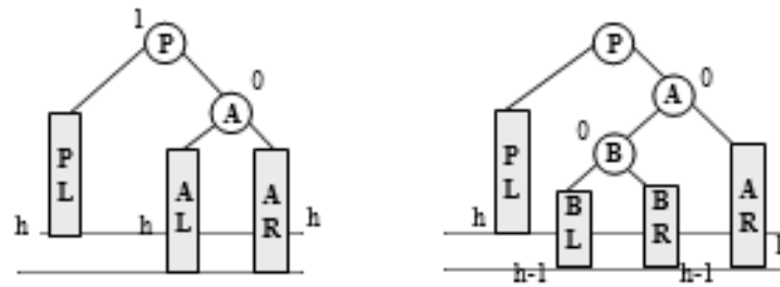
Figure 6.90 Case R_C2
