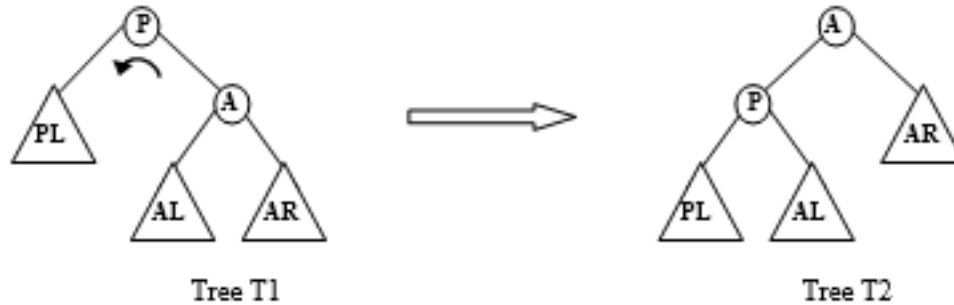
Figure 6.63 Left rotation
