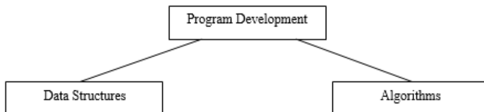
Figure 1.1 Program development
