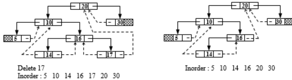
Figure 6.49 Deletion of 17
