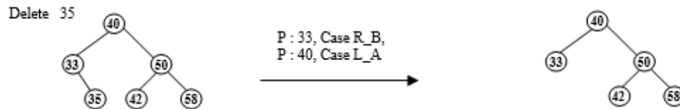
Figure 6.126 Delete 35
