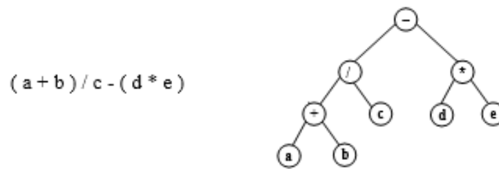
Figure 6.29 Expression tree
