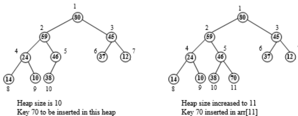
Figure 6.171 Insert 70
