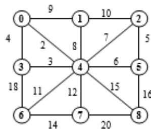
Figure 7.130 Weighted undirected connected graph
