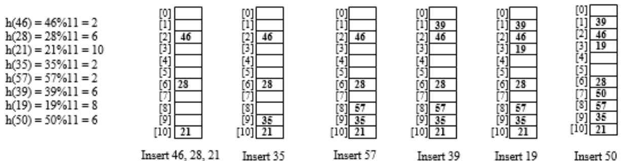
Figure 9.11 Double hashing
