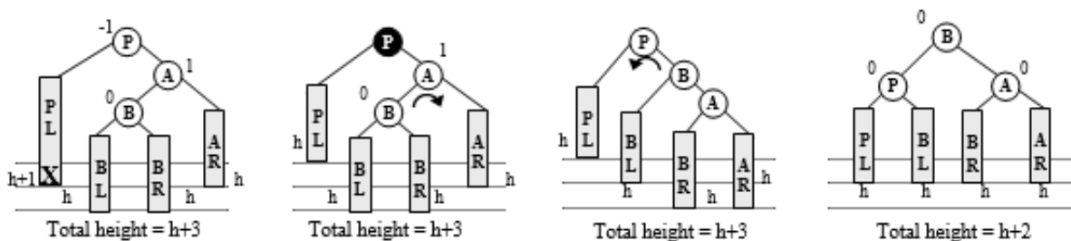
Figure 6.111 Case L_C3a
