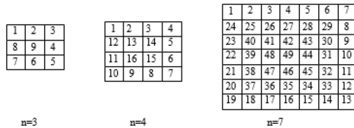
Figure 2.16 Spiral matrix
