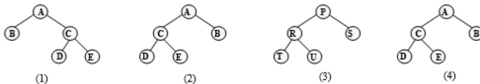
Figure 6.3 Binary trees
