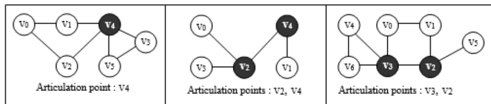
Figure 7.9 More examples of graphs with articulation points
