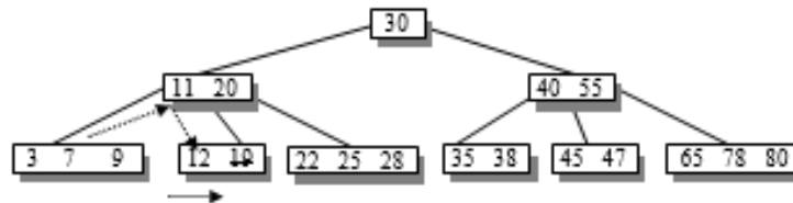
Figure 6.218 Delete 19
