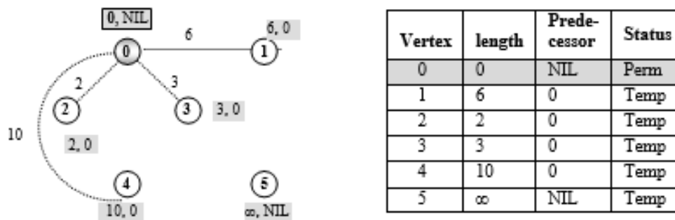
Figure 7.122 Relabel 1, 2, 3, 4
