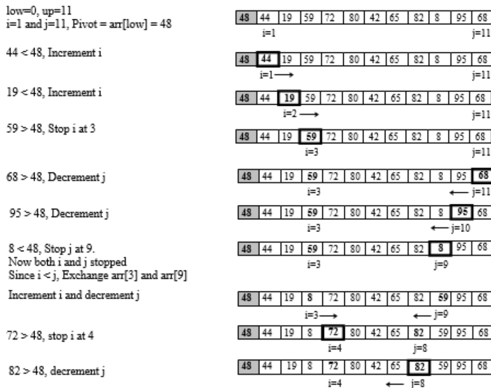
Figure 8.19 Partition process
