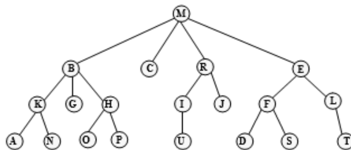
Figure 6.1 Tree
