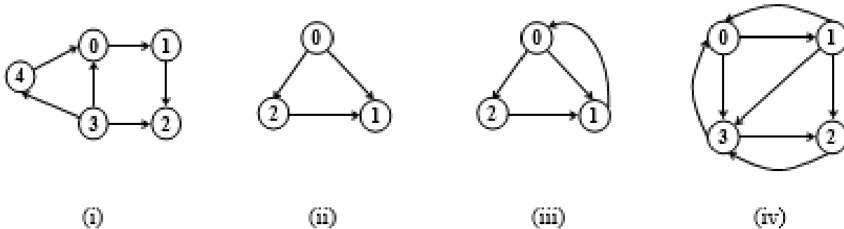
Figure 7.148 Directed graphs
