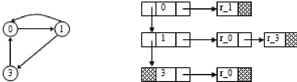
Figure 7.34 Deletion of a vertex
