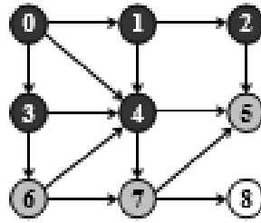
Figure 7.60 Visit 2
