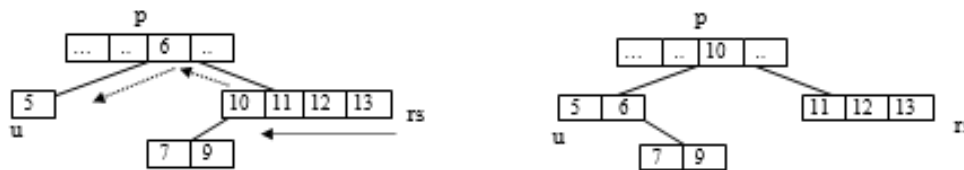
Figure 6.266 Borrow right
