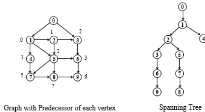
Figure 7.77 Graph with predecessor of each vertex and spanning tree
