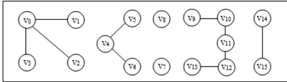
(b) A Spanning forest of Graph shown in (a)
