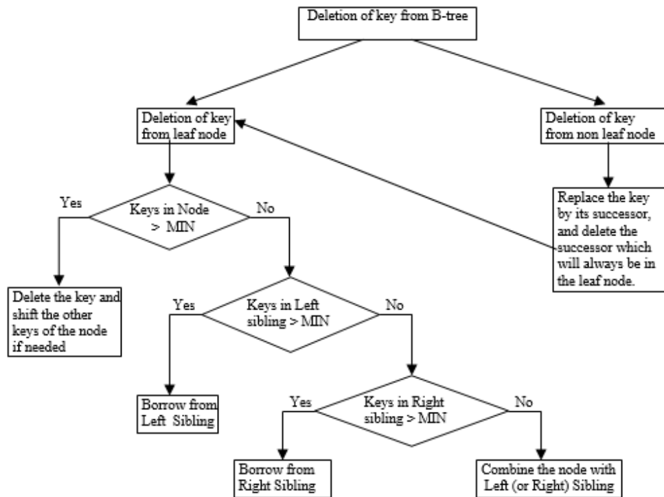
Figure 6.213 Deletion in B-tree
