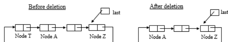
Figure 3.34 Deletion of the first node
