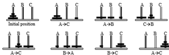
Figure 5.15 Tower of hanoi for 3 disks
