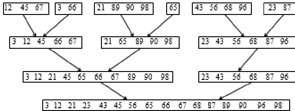
Figure 8.17 Natural merge sort
