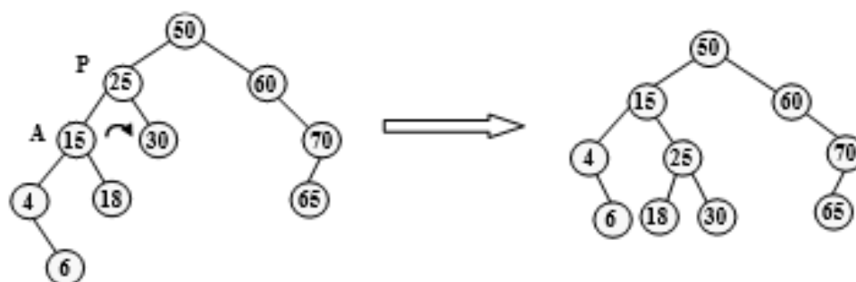
Figure 6.60 Right rotation about node 25
