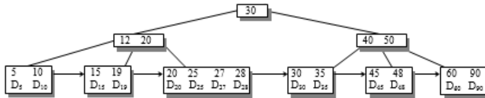
Figure 6.271 B+ tree after deletion of 12, 38, 40, 50
