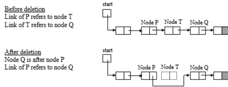
Figure 3.13 Deletion in between the list nodes
