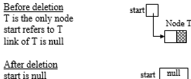
Figure 3.12 Deletion of the only node
