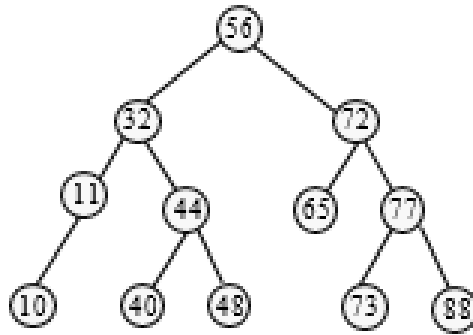
Figure 11.31 Binary search tree from postorder traversal
