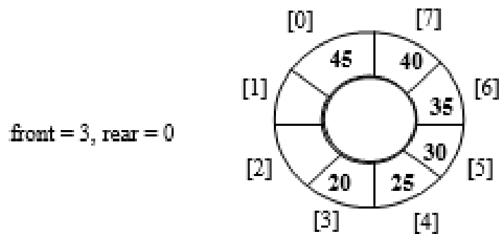
Figure 4.11 Insertion in circular queue
