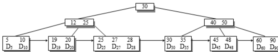
Figure 6.272 B+ tree after deletion of 15
