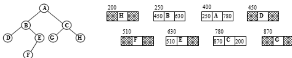
Figure 6.13 Binary tree and its nodes in memory
