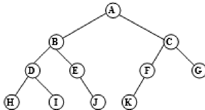
Figure 6.26 Binary tree from inorder and postorder traversal
