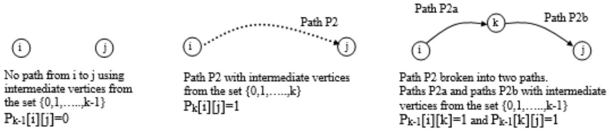
Figure 7.44 Finding path matrix values
