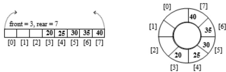
Figure 4.10 Circular queue example
