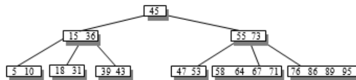
Figure 6.230 B-tree after deletion of 22, 24
