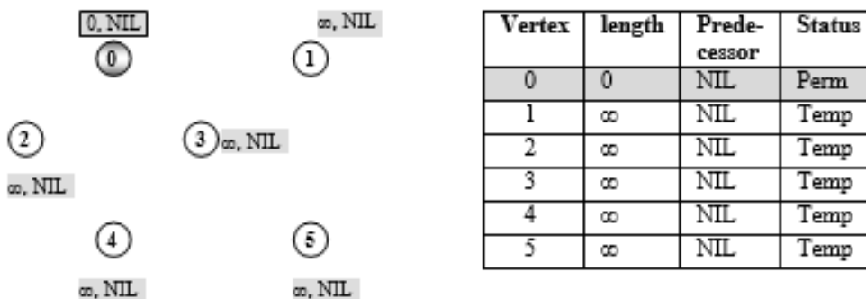
Figure 7.121 Make vertex 0 permanent
