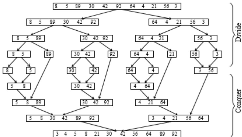
Figure 8.13 Top-down merge sort
