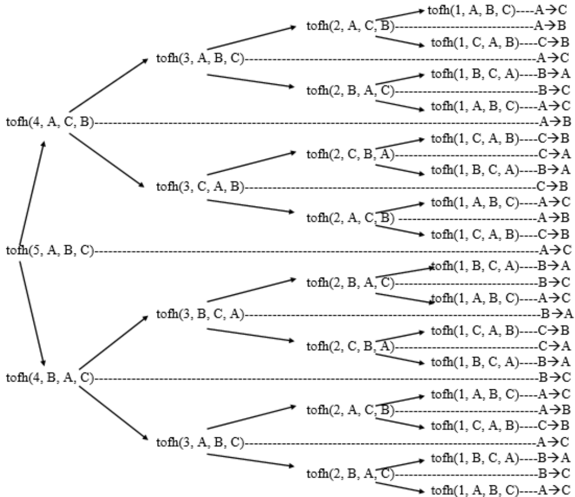
Figure 5.16 Tower of Hanoi for 5 disks
