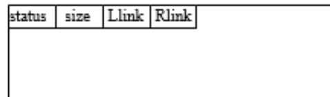
Figure 10.31 Structure of block for buddy system
