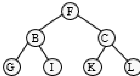
Figure 11.32 Full binary tree from preorder traversal
