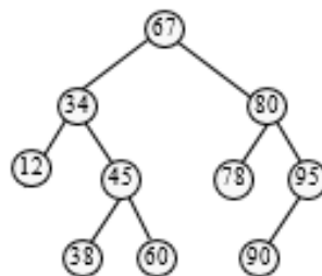
Figure 11.30 Binary search tree from preorder traversal
