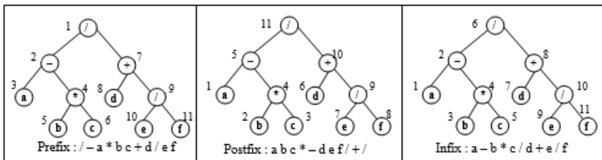
Figure 6.30 Expression tree traversals
