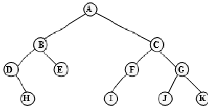
Figure 6.23 Binary tree from inorder and preorder traversal
