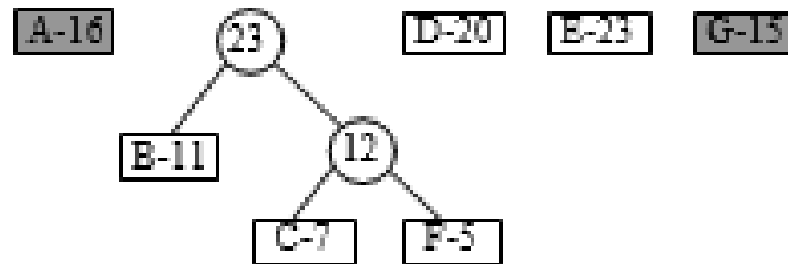
Figure 6.185 Trees weighted 11 and 12 are combined
