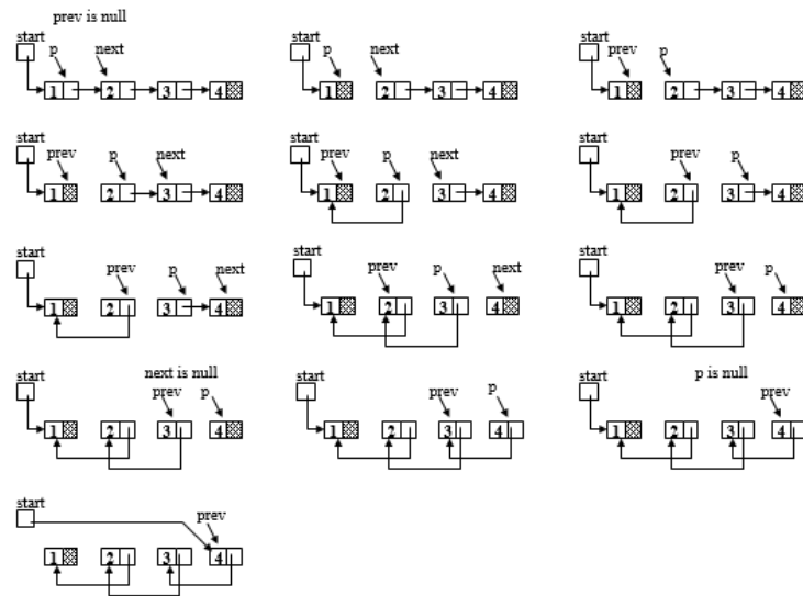
Figure 3.17 Steps of reversing a single linked list
