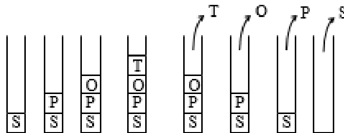
Figure 4.17 Reversal of string
