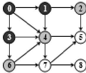
Figure 7.58 Visit 3, insert 6 into the queue
