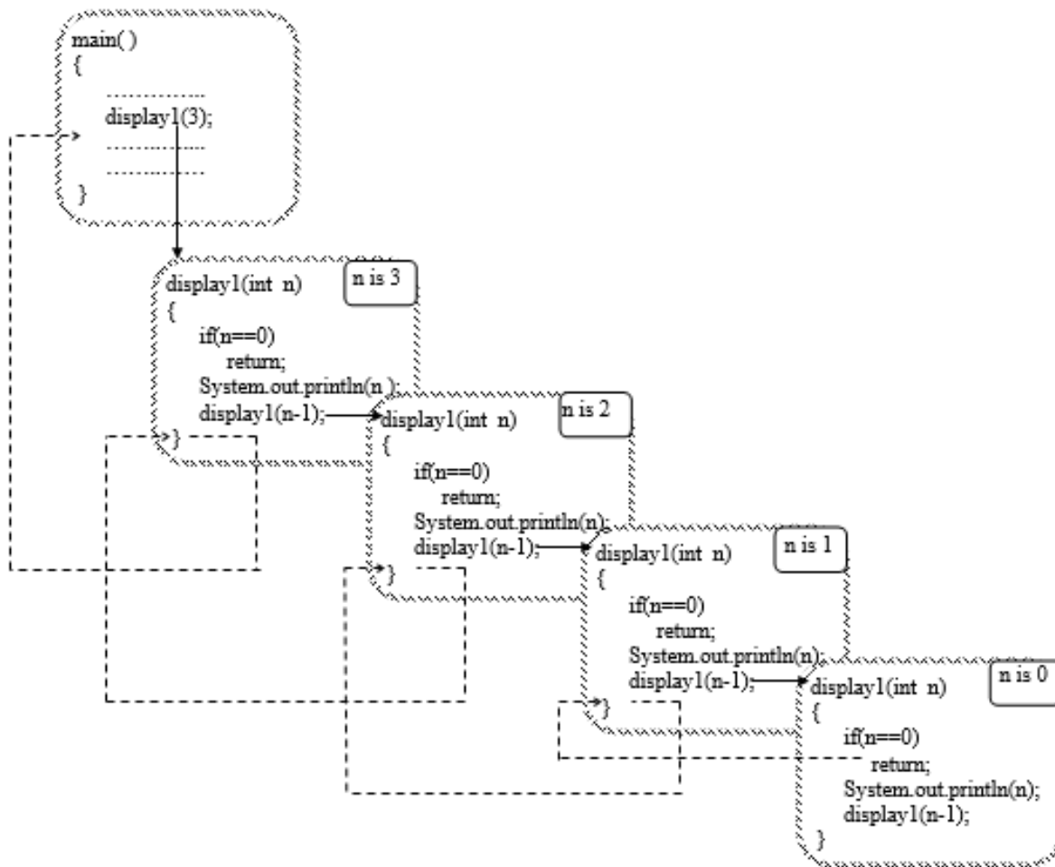
Figure 5.7 Displaying numbers from n to 1
