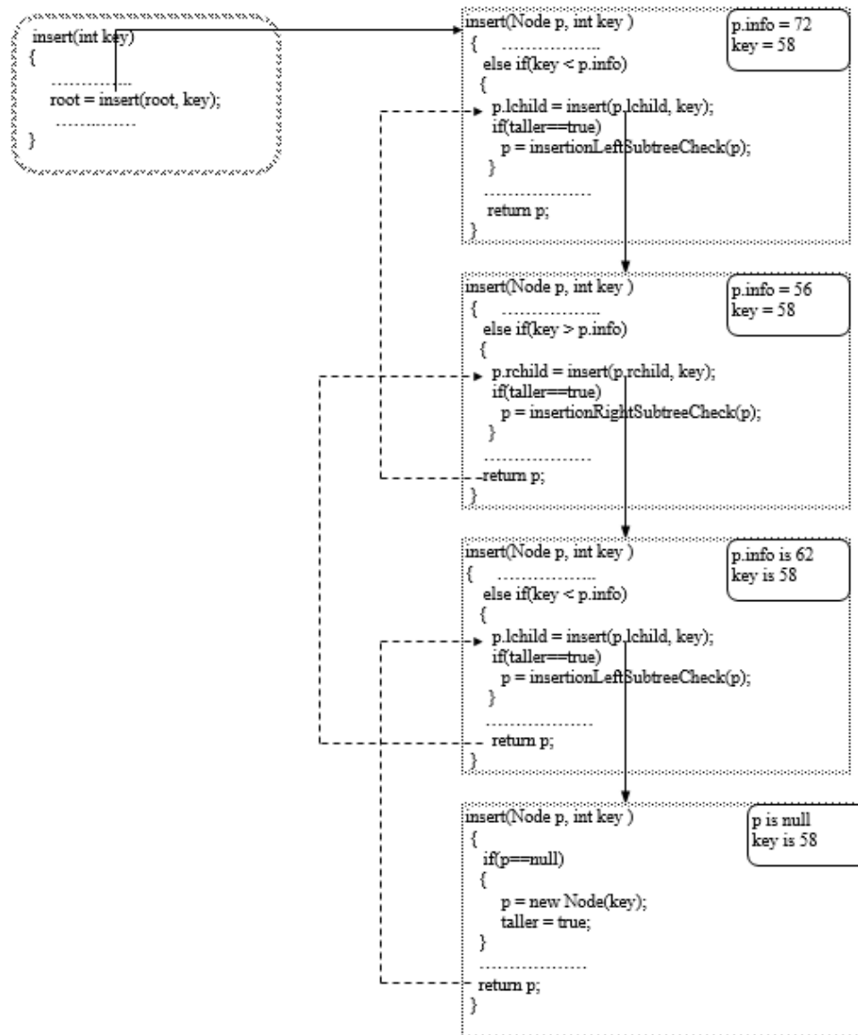
Figure 6.69 Recursive calls for inserting 58
