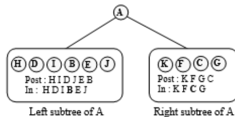
Figure 6.24 Left and right subtree of root A
