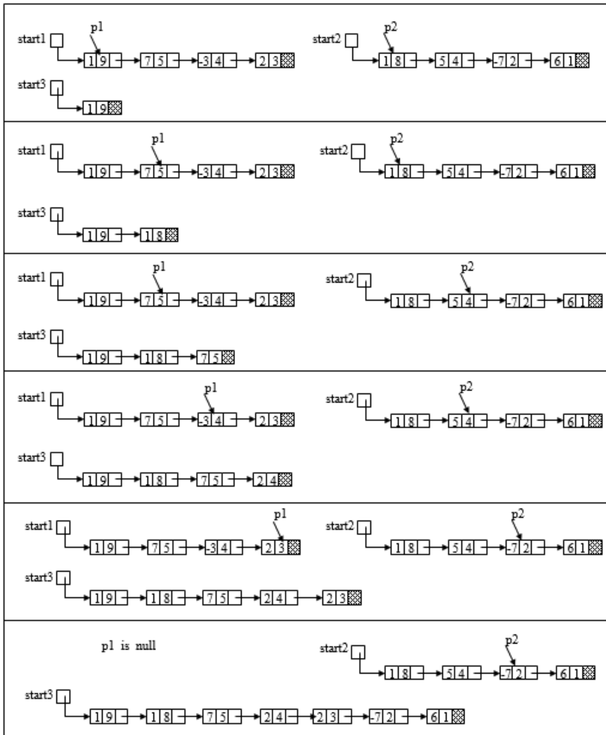
Figure 3.61 Addition of two polynomial expressions
