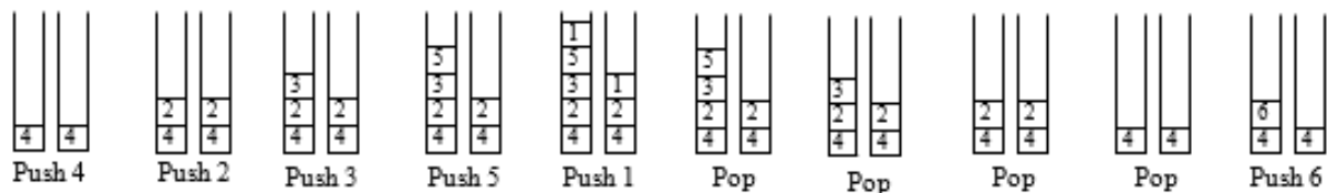
Figure 11.18 Getting minimum element from stack
