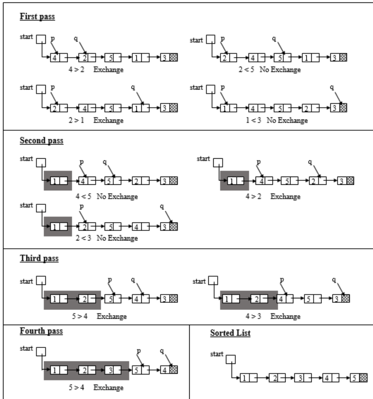
Figure 3.44 Selection sort by exchanging data
