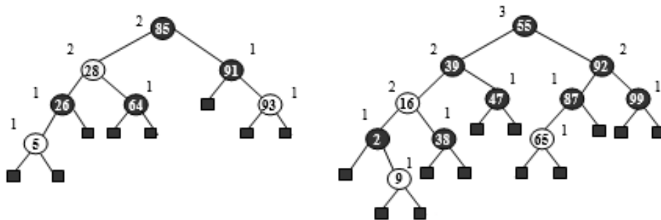
Figure 6.129 Red black trees
