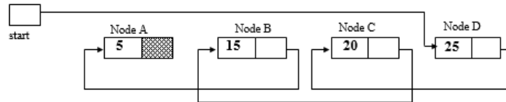
Figure 3.16 Reversed single linked list
