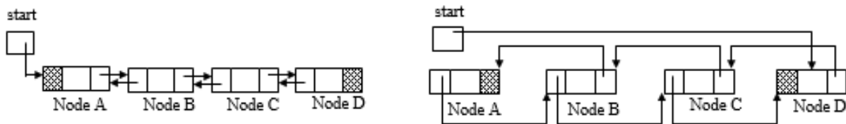
Figure 3.27 Reversing a doubly linked list
