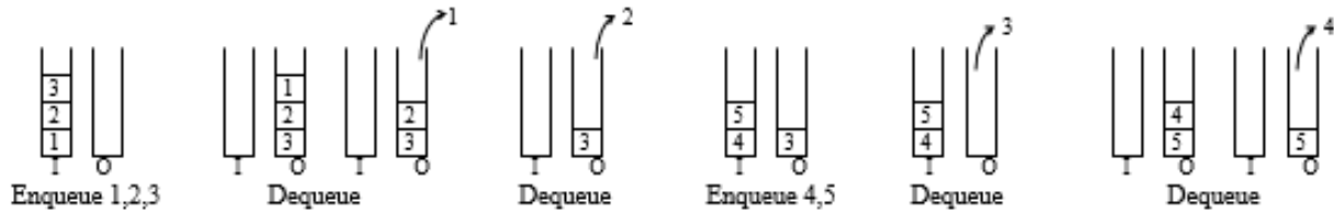
Figure 11.13 Queue using two stacks
