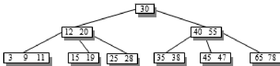
Figure 6.262 B-tree example for deleting 45
