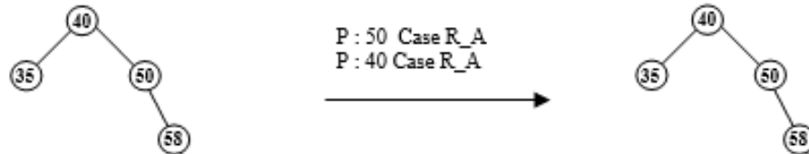
Figure 6.98 Insert 58
