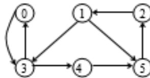
Figure 11.40 Reverse graph
