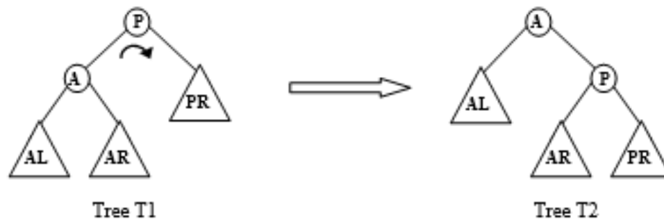
Figure 6.59 Right rotation
