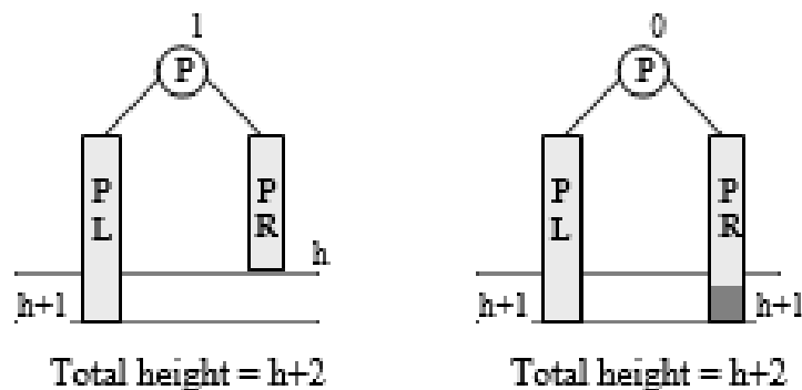
Figure 6.86 Case R_B
