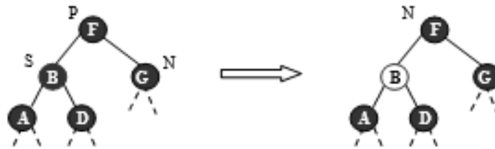
Figure 6.157 Case R_2b
