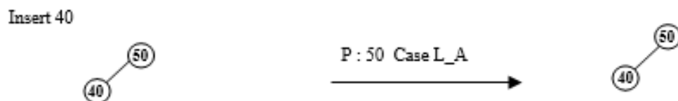
Figure 6.96 Insert 40
