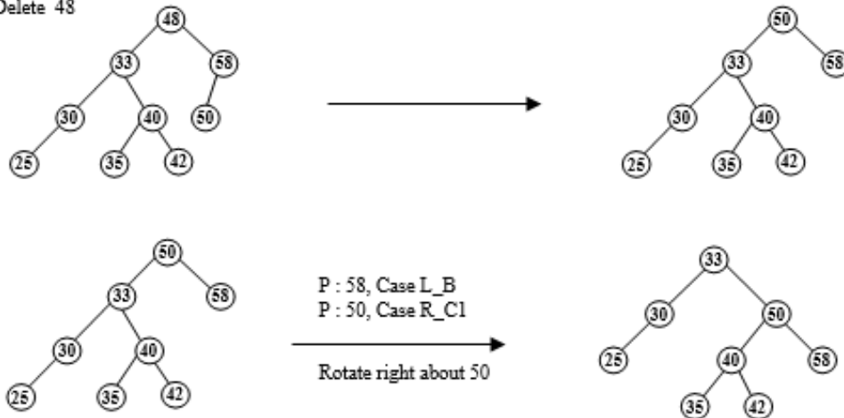
Figure 6.123 Delete 48
