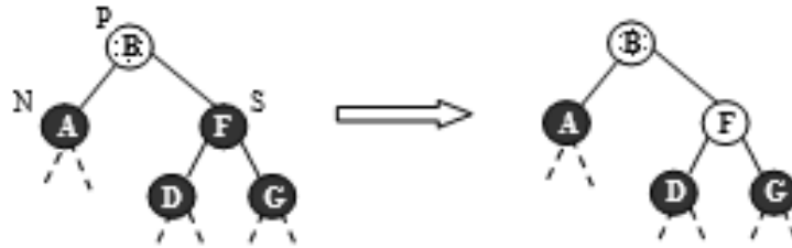
Figure 6.150 Case L_2
