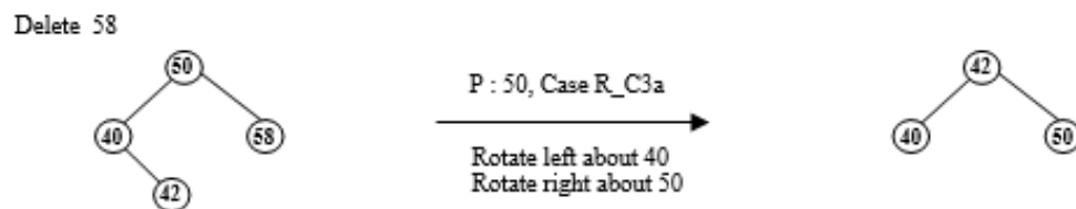
Figure 6.128 Delete 58
