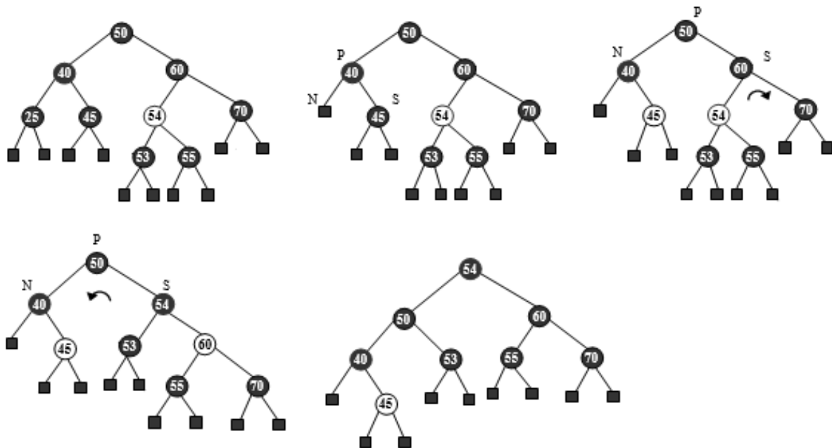
Figure 6.167 Delete 25
