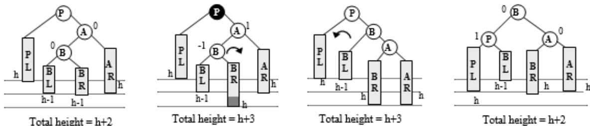
Figure 6.91 Case R_C2a
