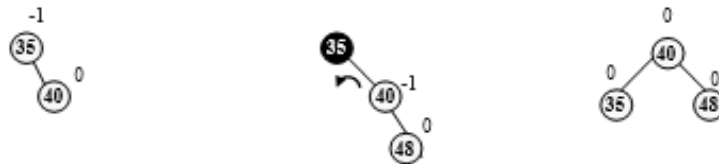
Figure 6.88 Insertion of 48
