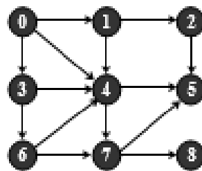
Figure 7.64 Visit 8
