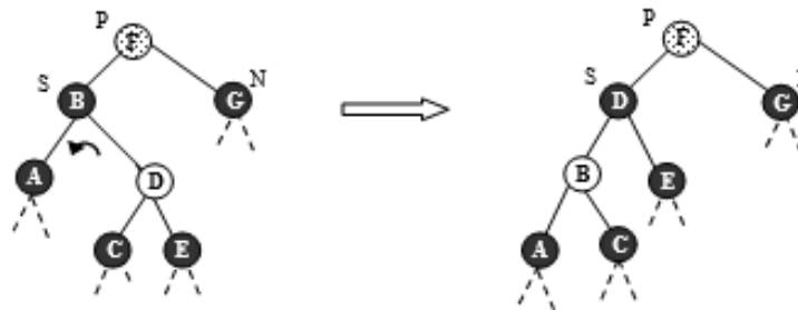
Figure 6.158 Case R_3a
