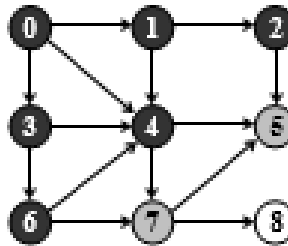
Figure 7.61 Visit 6
