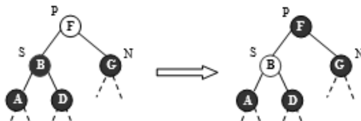
Figure 6.156 Case R_2a
