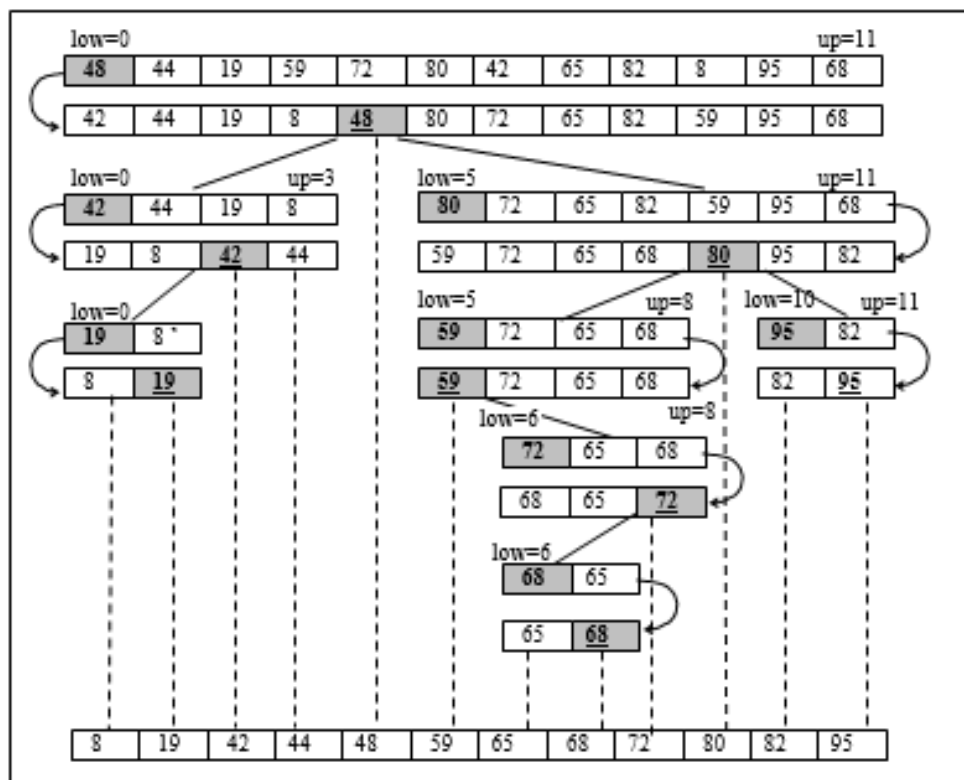
Figure 8.18 Quick sort
