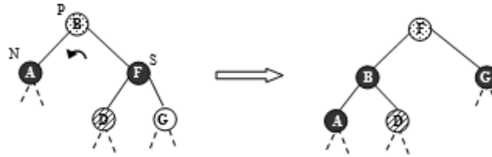
Figure 6.154 Case L_3b
