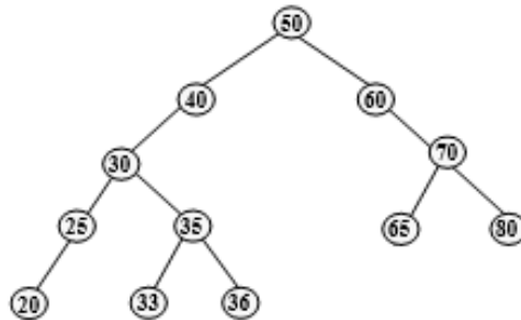
Figure 6.19 Binary tree
