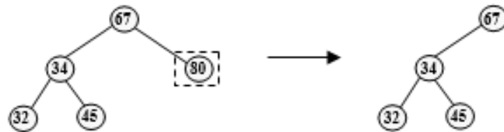
Figure 6.38 Deletion of 80
