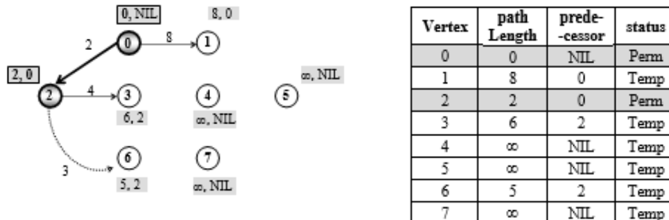
Figure 7.90 Make vertex 2 permanent
