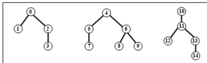
Figure 7.82 Spanning forest for undirected graph
