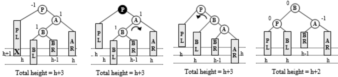
Figure 6.112 Case L_C3b
