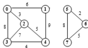
Figure 7.128 Not connected graph
