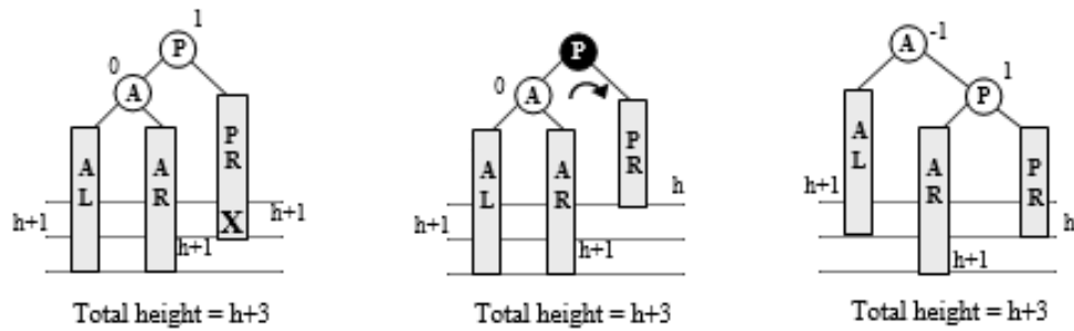
Figure 6.116 Case R_C1
