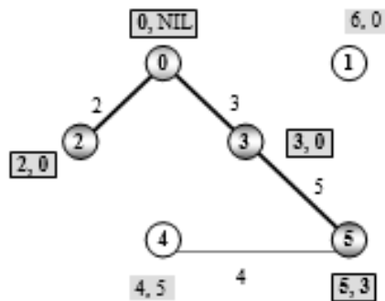
Figure 7.125 Make vertex 5 permanent, relabel 4
