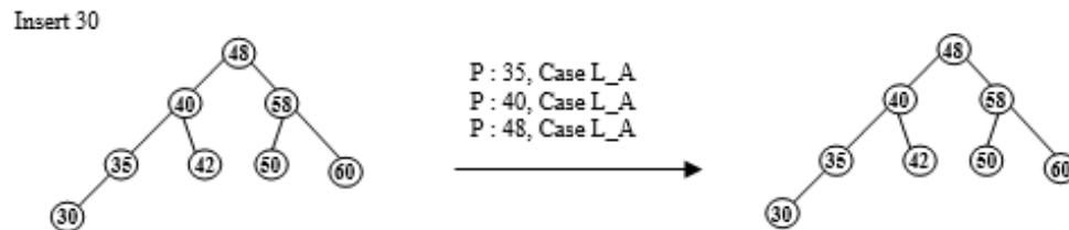
Figure 6.102 Insert 30
