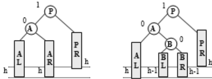
Figure 6.78 Case L_C2
