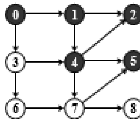
Figure 7.73 Visit vertex 4, 5
