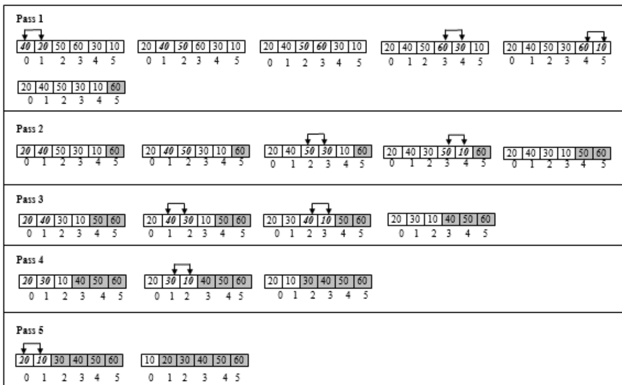
Figure 8.7 Bubble sort
