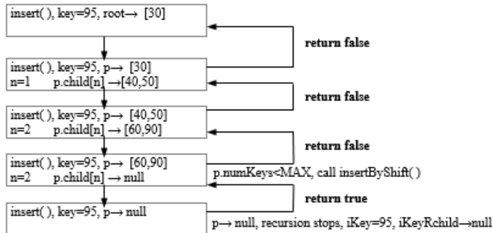
Figure 6.249 Insertion of 95
