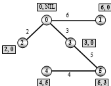
Figure 7.127 Make vertex 1 permanent
