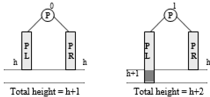
Figure 6.70 Case L_A
