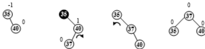
Figure 6.94 Insertion of 37
