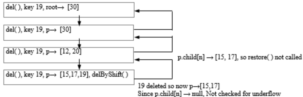
Figure 6.258 Deletion of 19
