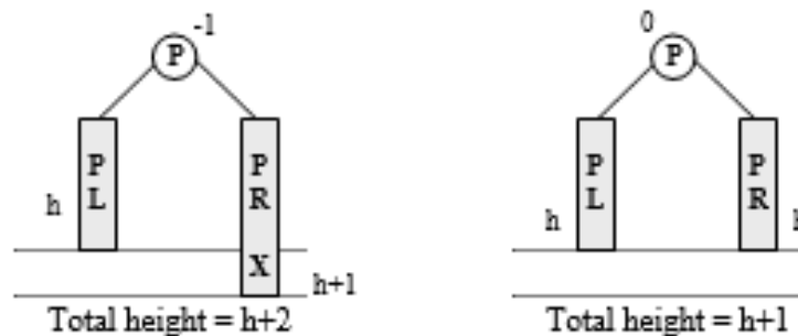
Figure 6.115 Case R_B
