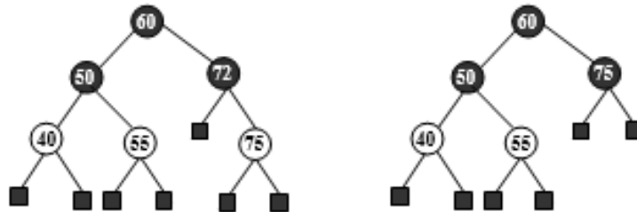
Figure 6.161 Delete 72
