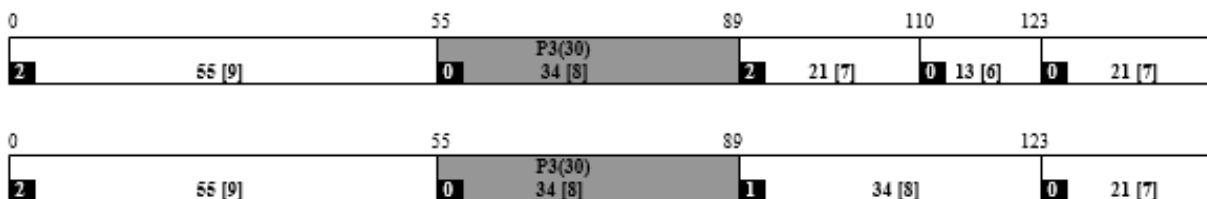
Figure 10.45 Free P6
