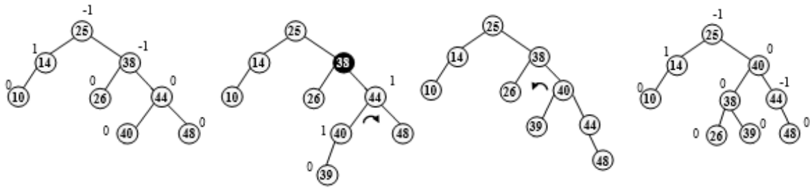
Figure 6.95 Insertion of 39
