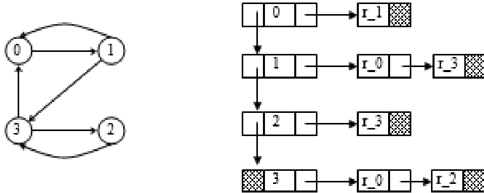
Figure 7.33 Deletion of an edge
