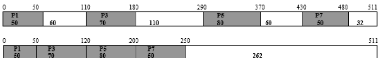
Figure 10.49 Compaction
