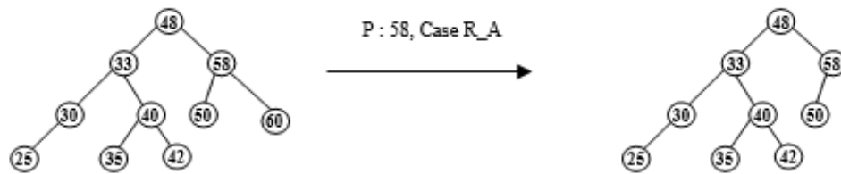
Figure 6.122 Delete 60
