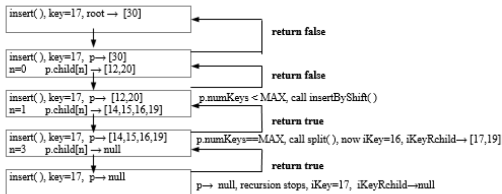
Figure 6.246 Insertion of 17
