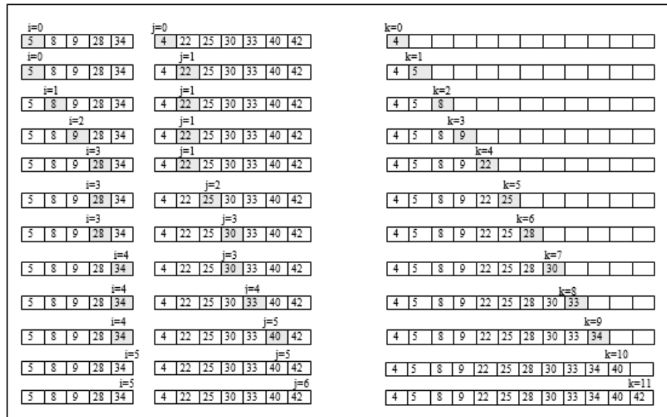
Figure 8.11 Merging
