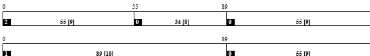
Figure 10.47 Free P3
