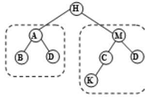
Figure 6.28 Binary tree
