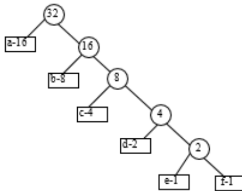
Figure 11.34 Huffman tree
