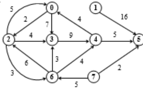
Figure 7.97 Graph with some vertices not reachable
