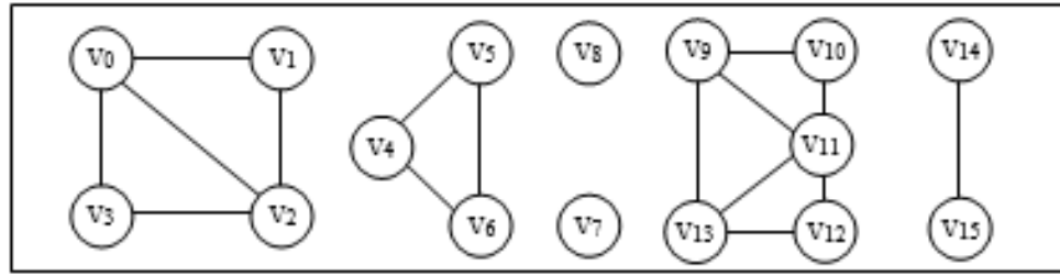
(a) A disconnected Graph
