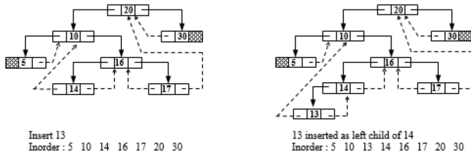
Figure 6.46 Insertion of 13
