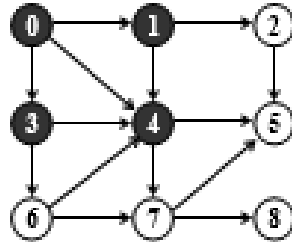
Figure 7.52 Visit start vertex 0, then visit 1, 3, 4
