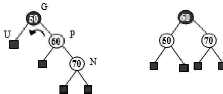
Figure 6.140 Insert 70
