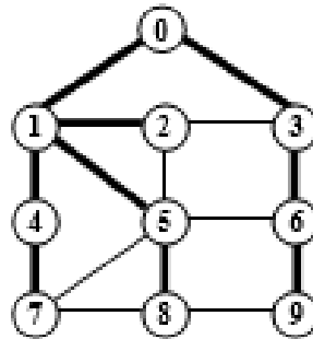
Figure 7.68 Undirected graph, traversed with start vertex 0
