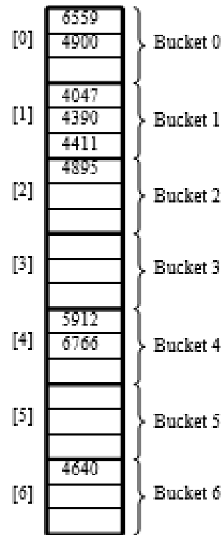
Figure 9.13 Bucket hashing
