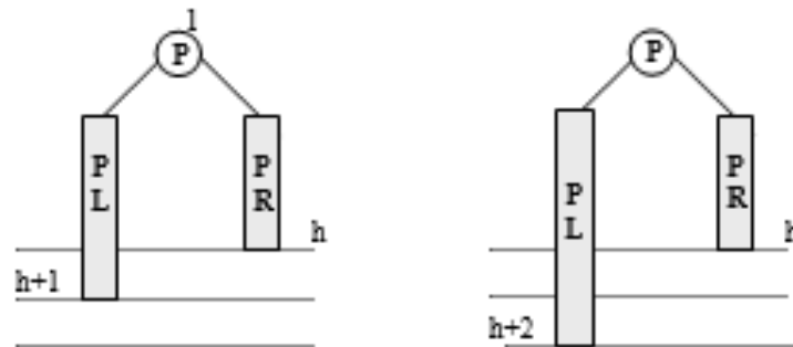
Figure 6.72 Case L_C
