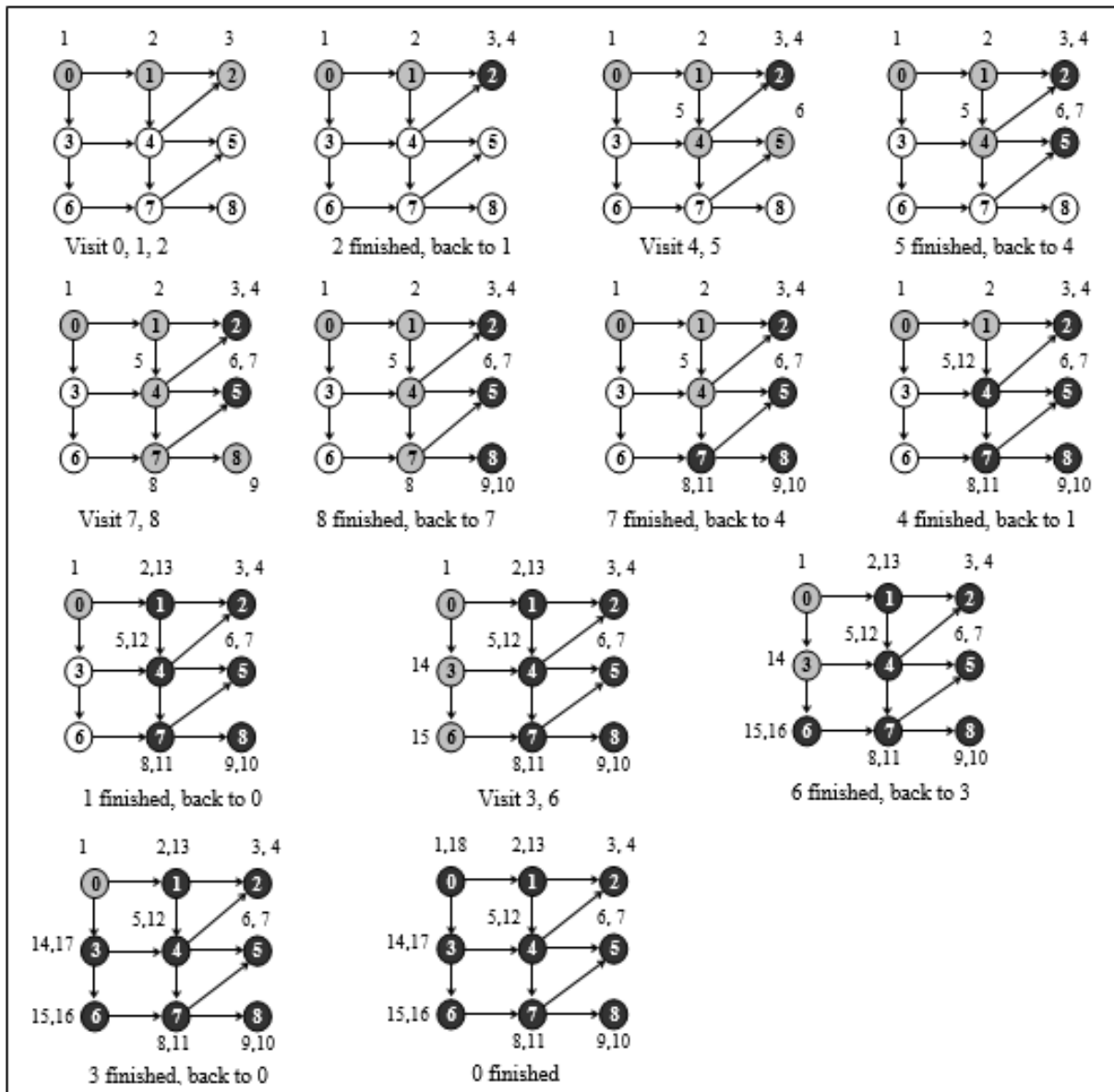
Figure 7.78 Recursive DFS showing discovery time and finishing time
