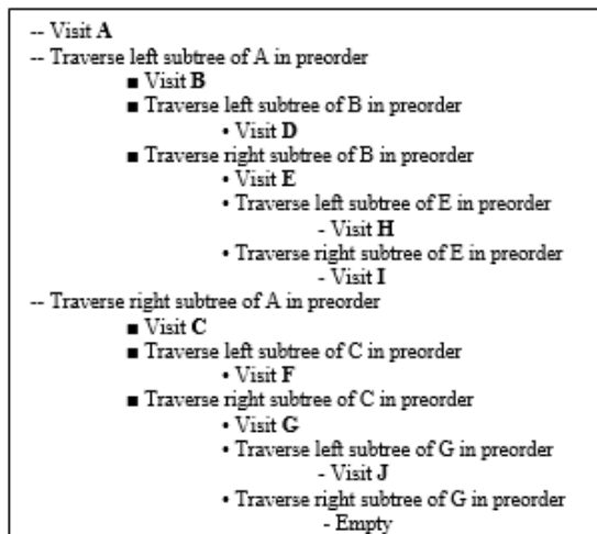
Figure 6.15 Preorder traversal
