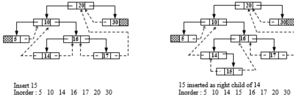
Figure 6.47 Insertion of 15
