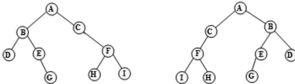
Figure 6.281 Mirror image
