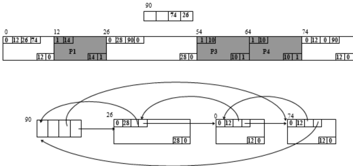
Figure 10.16 Free P2
