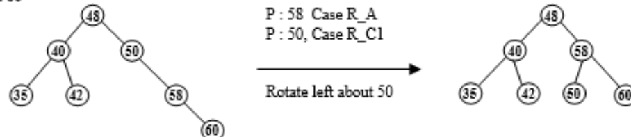
Figure 6.101 Insert 60
