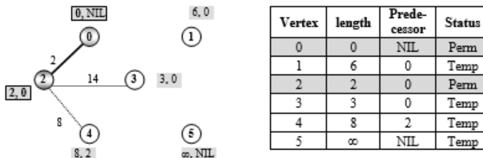
Figure 7.123 Make vertex 2 permanent, relabel 4
