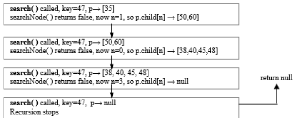
Figure 6.243 Search 47
