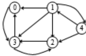
Figure 11.39 Reverse graph
