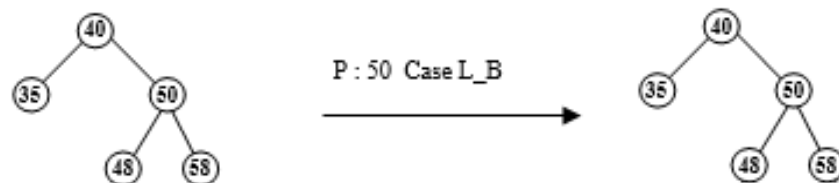
Figure 6.99 Insert 48
