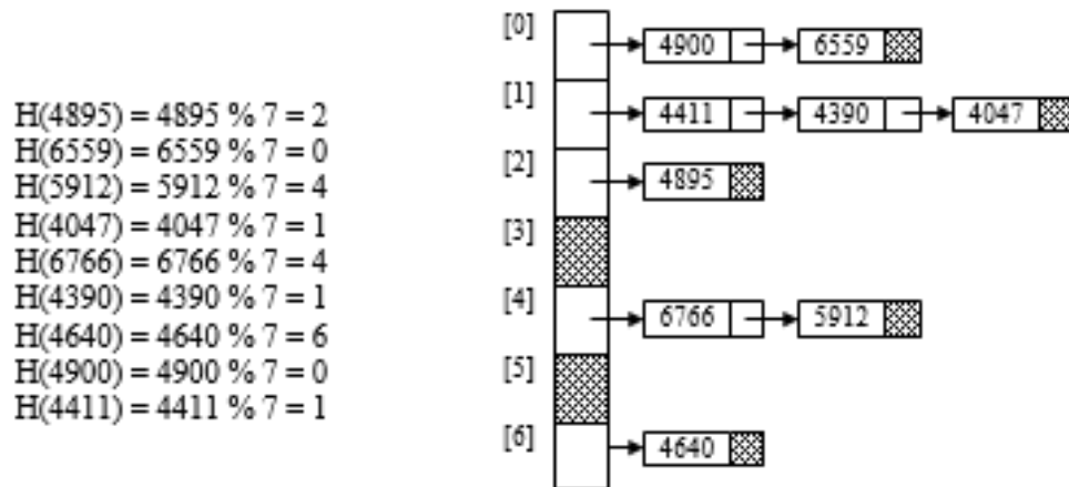
Figure 9.12 Separate chaining
