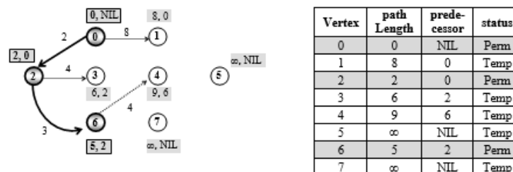
Figure 7.91 Make vertex 6 permanent
