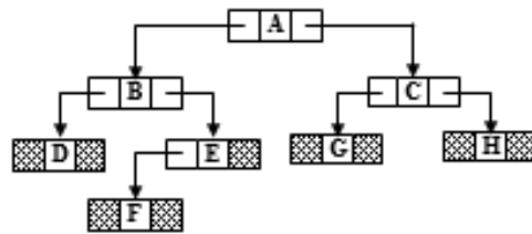
Figure 6.14 Binary tree linked representation
