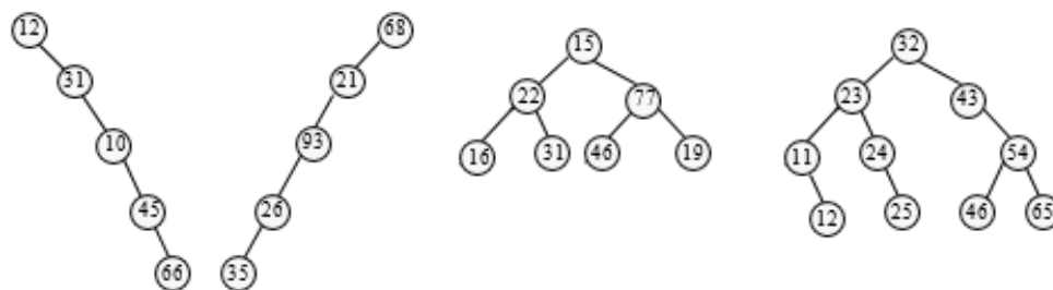
Figure 11.27 Binary trees from inorder and preorder traversals
