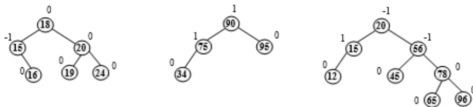
Figure 6.57 AVL trees with balance factor
