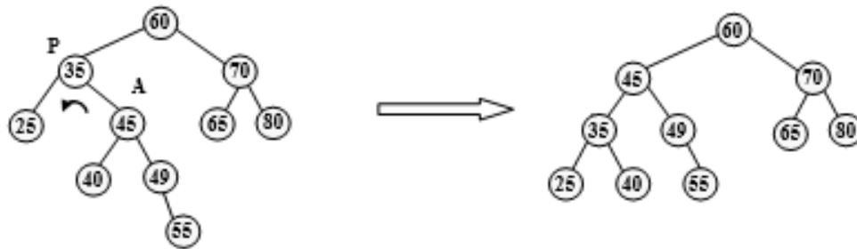
Figure 6.64 Left rotation about node 35
