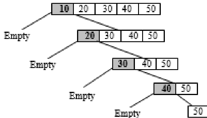
Figure 8.21 Quick sort for already sorted list
