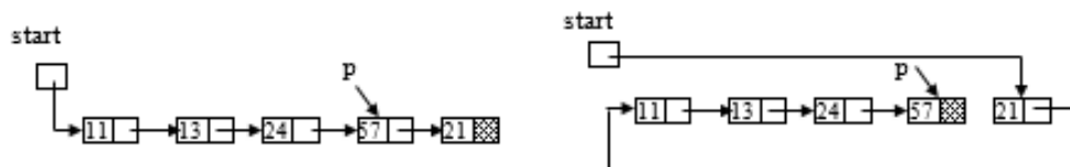
Figure 11.2 Removing last node and inserting at beginning
