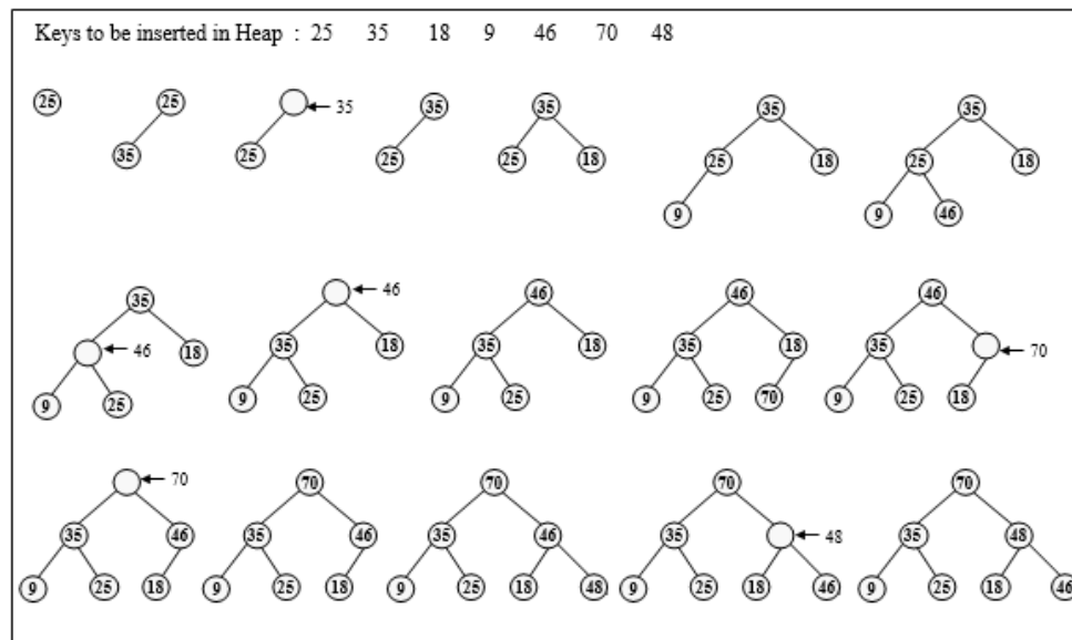
Figure 6.175 Inserting keys in heap tree
