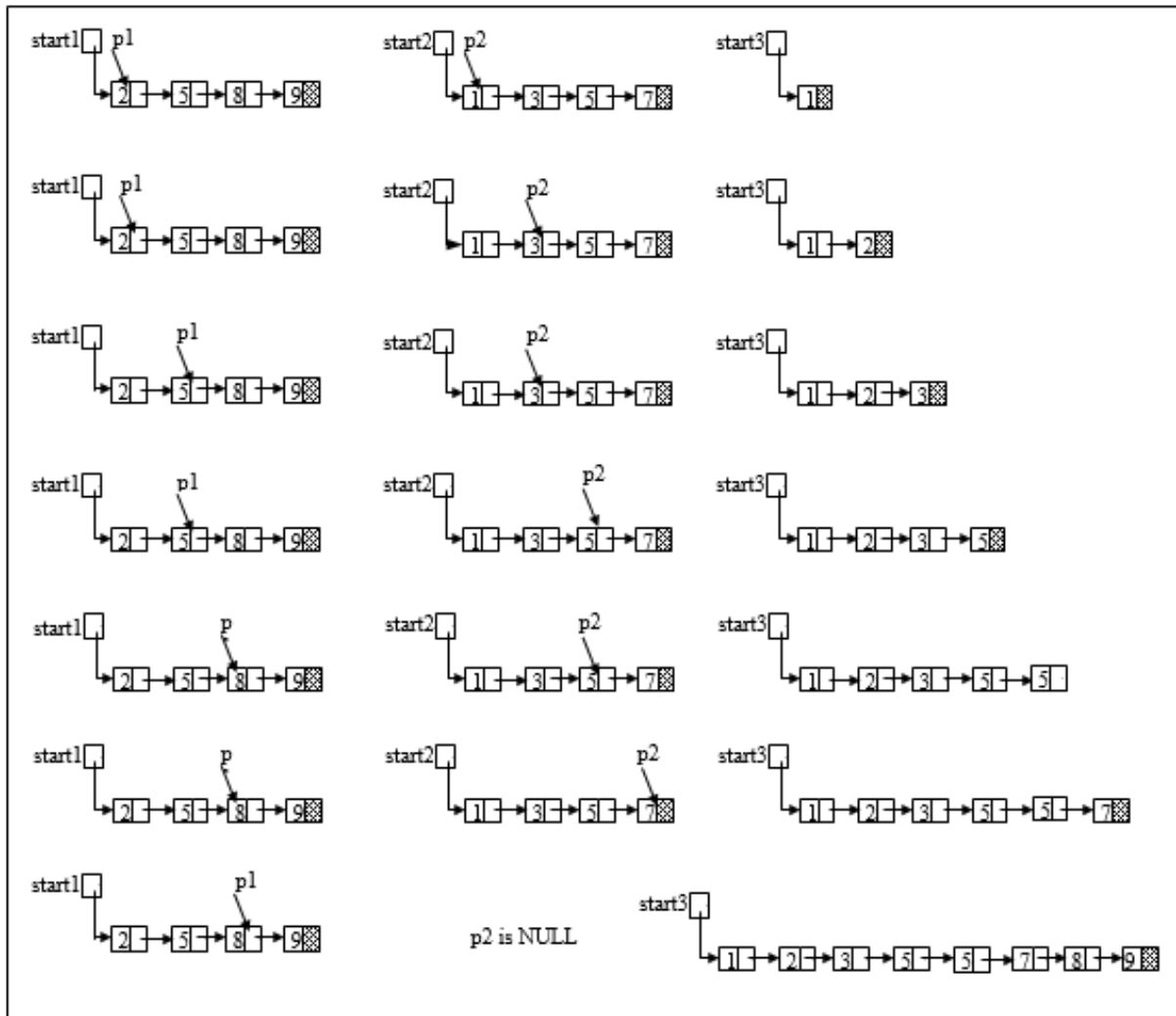
Figure 3.52 Merging of two sorted linked lists
