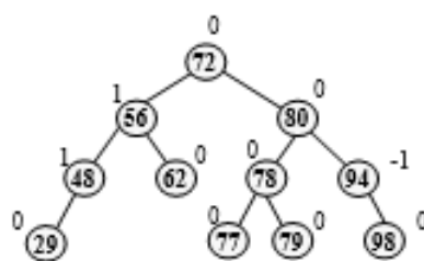
(i) 77 inserted in T
