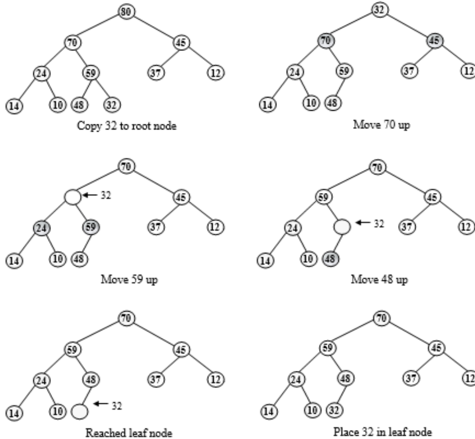
Figure 6.178 Example of deletion of root from the heap
