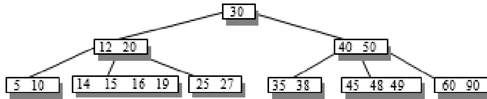
Figure 6.247 B-tree example for inserting 95
