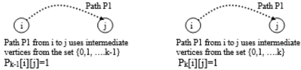
Figure 7.43 Finding P_{k-1}[i][j] and P_k[i][j] values
