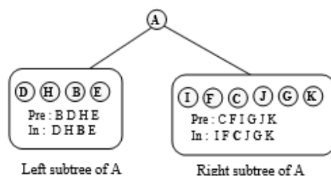
Figure 6.21 Left and right subtree of root A
