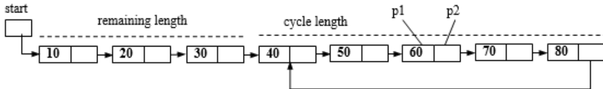
Figure 3.57 Removal of cycle in a single linked list
