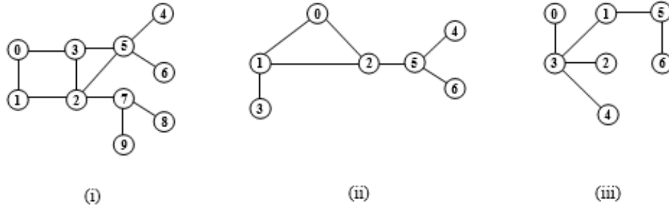
Figure 7.149 Graphs to find articulation point
