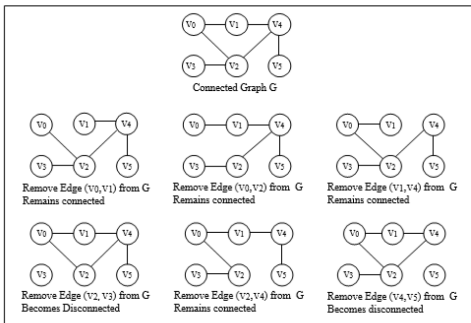
Figure 7.7 Graphs examples to find bridge
