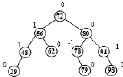
Figure 6.67 AVL tree (T)
