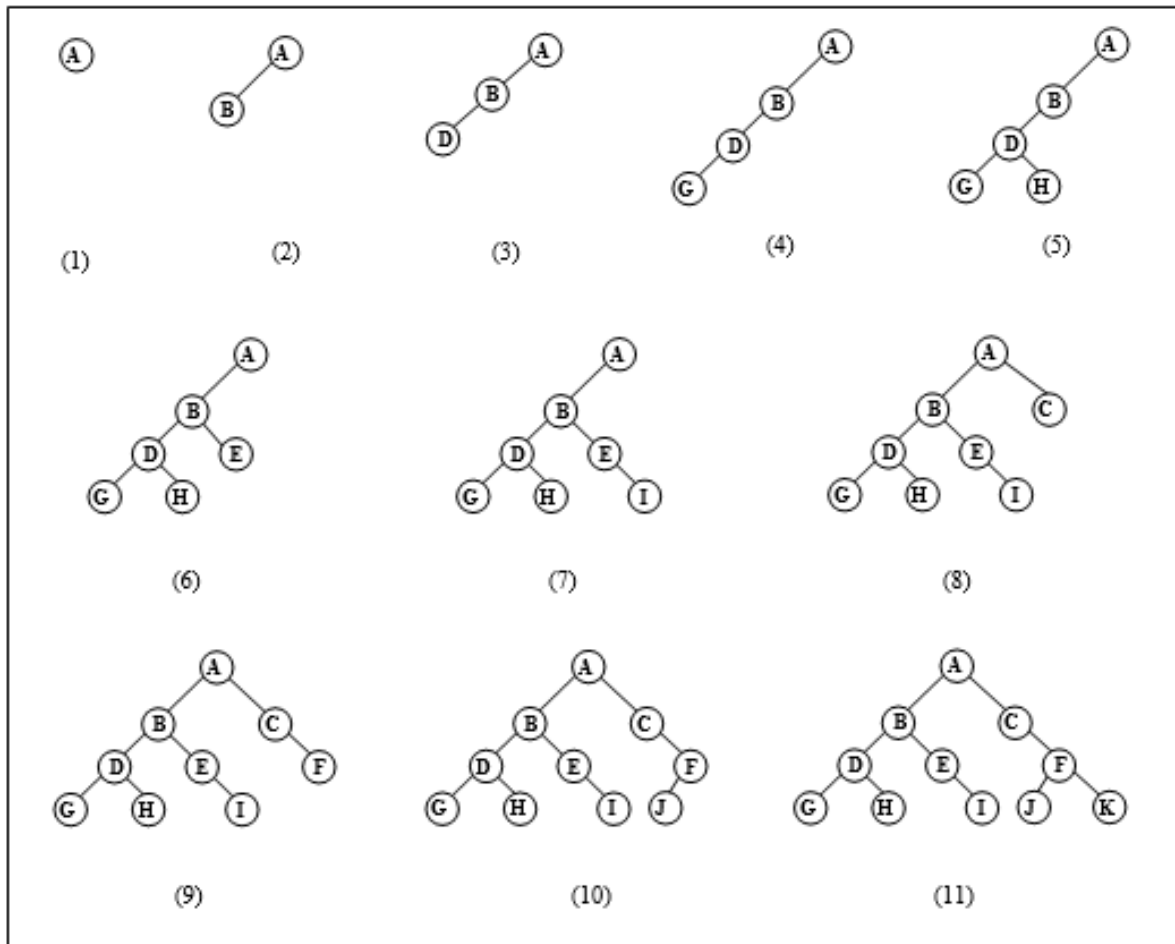
Figure 6.27 Binary tree construction from preorder and inorder traversal
