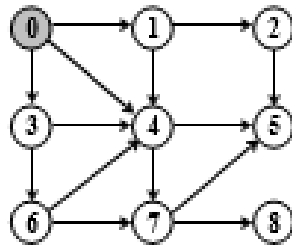
Figure 7.55 Insert 0 into the queue
