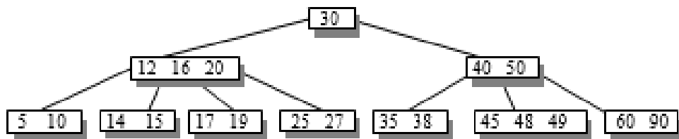
Figure 6.245 B-tree after insertion of 17
