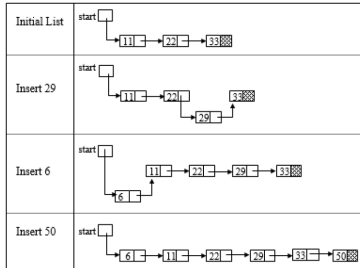
Figure 3.42 Insertion in a sorted linked list
