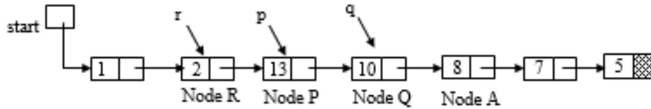
Figure 3.50 Bubble sort by rearranging links
