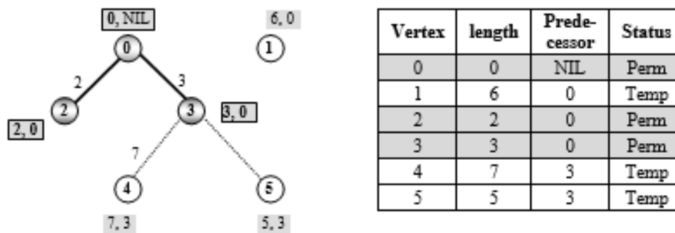
Figure 7.124 Make vertex 3 permanent, relabel 4, 5
