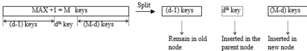
Figure 6.255 Split the keys
