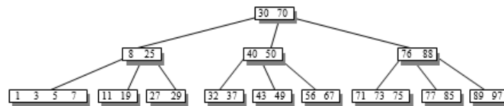
Figure 6.200 B-tree of order 5
