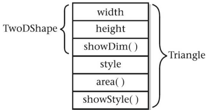
Figure 7-1 A conceptual depiction of the Triangle class
