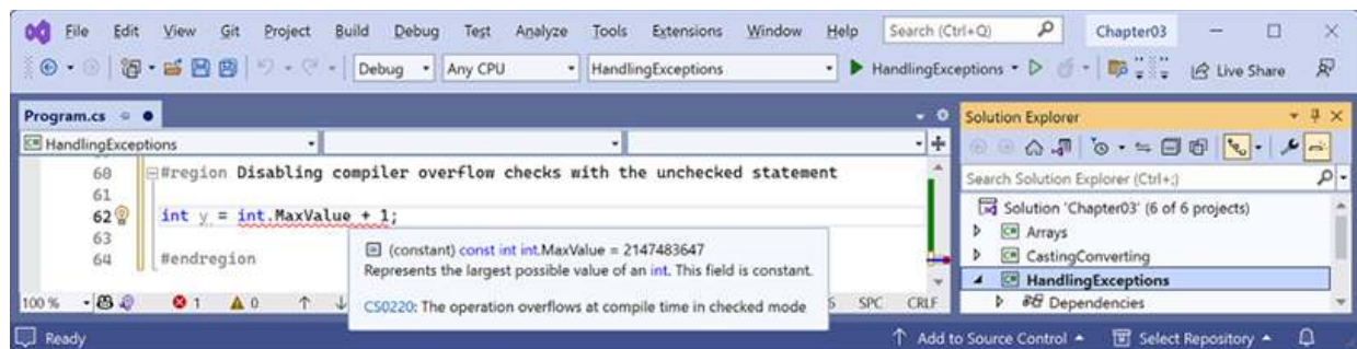
Figure 3.4: A compile-time check for integer overflow
