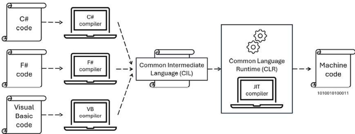
Figure 1.5: How C# and other languages are related to .NET
