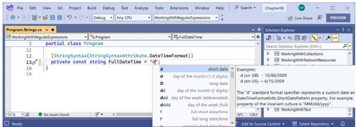
Figure 8.2: IntelliSense activated due to the StringSyntax attribute
