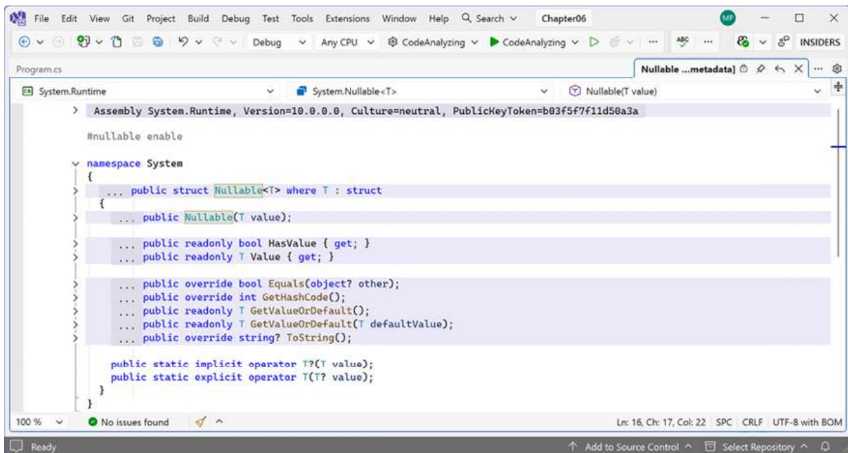
Figure 6.1: Revealing Nullable<T> members
