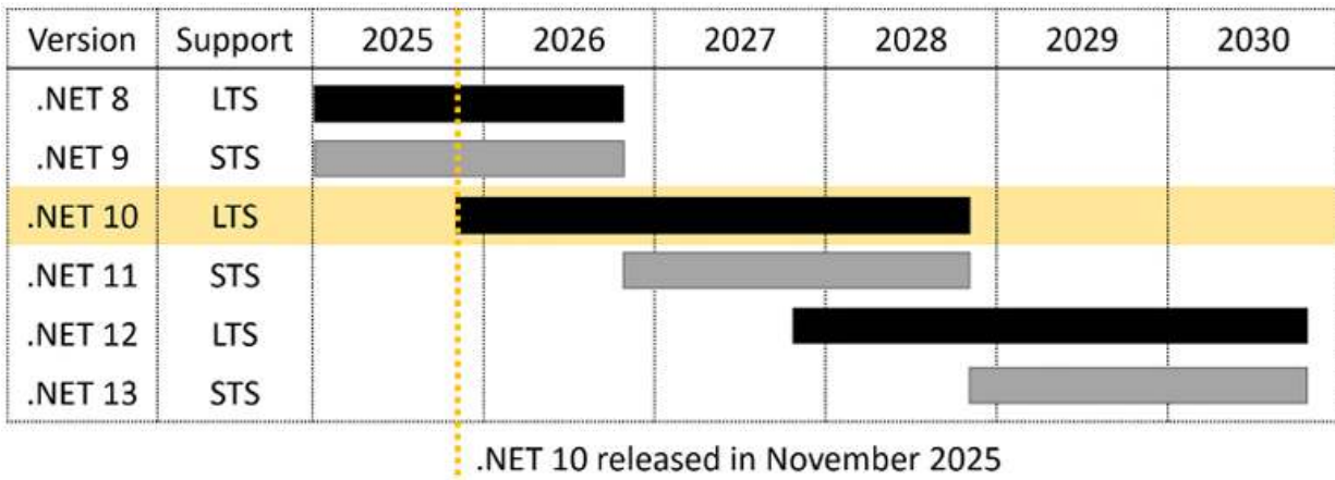
Figure 1.3: Support durations for recent and planned STS and LTS releases
