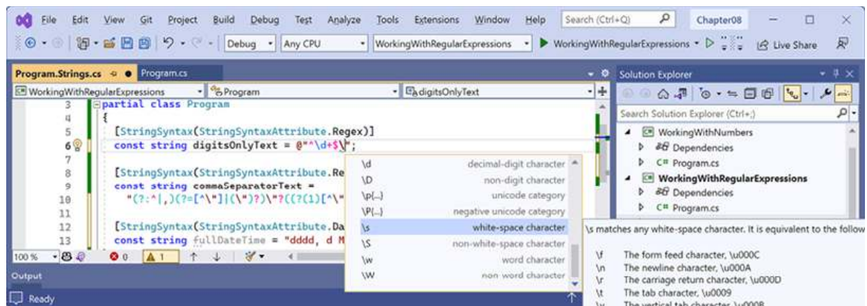
Figure 8.3: IntelliSense for writing a regular expression
