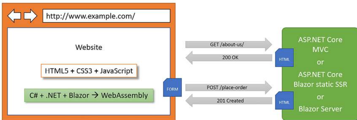
Figure 12.2: The use of C# and .NET to build websites on both the server side and client side
