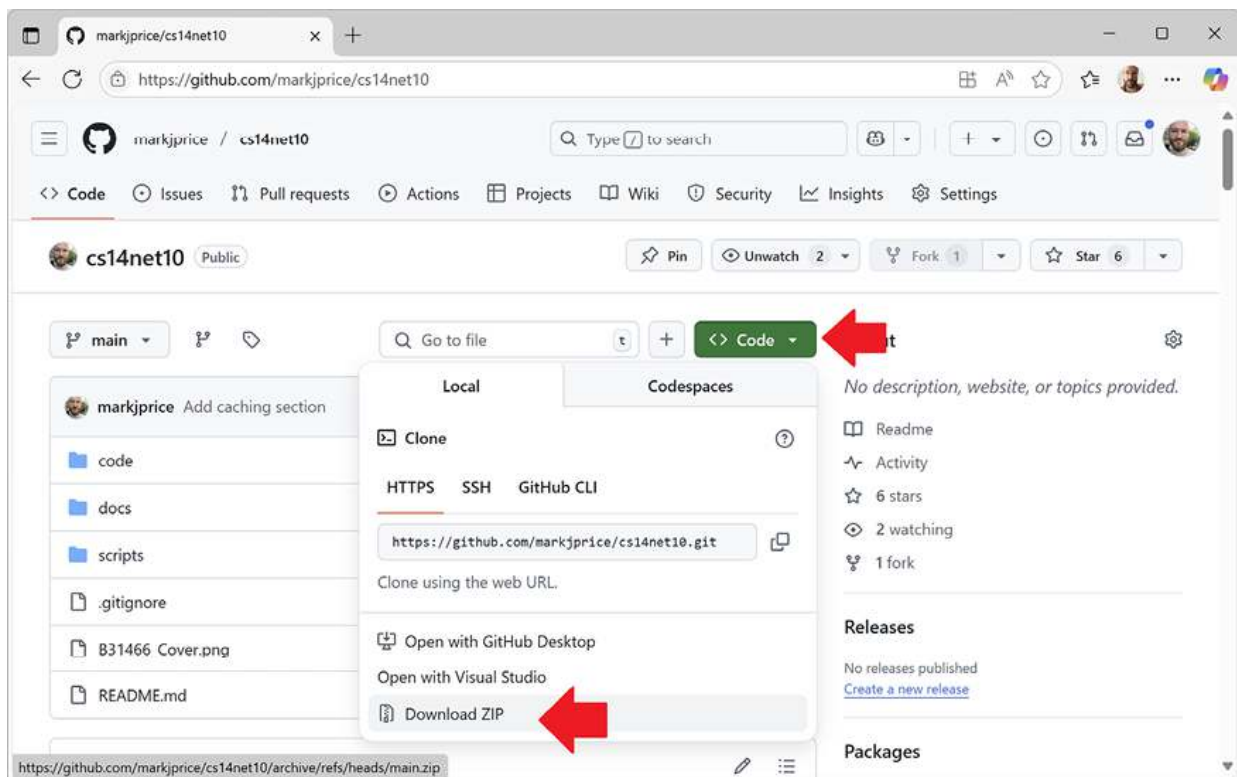
Figure 1.11: Downloading the repository as a ZIP file
