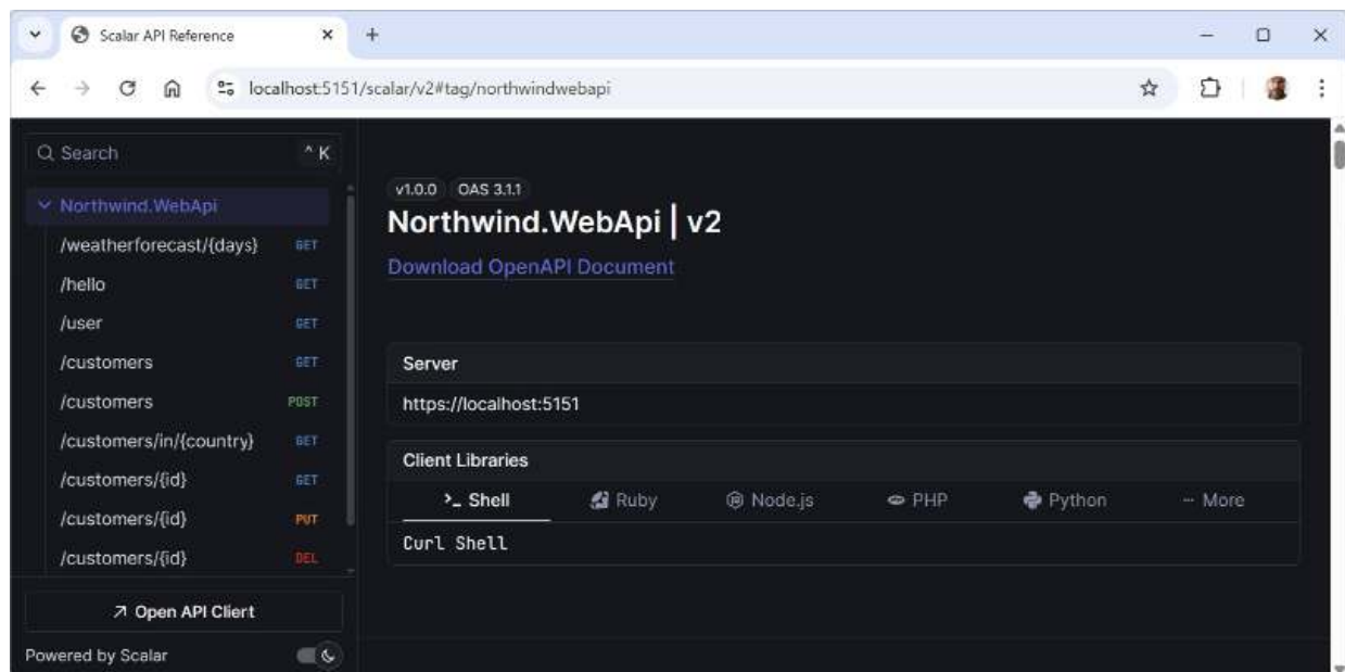
Figure 15.6: Scalar listing all endpoints in a web service
