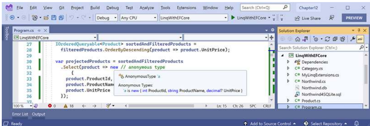
Figure 11.5: An anonymous type used during LINQ projection
