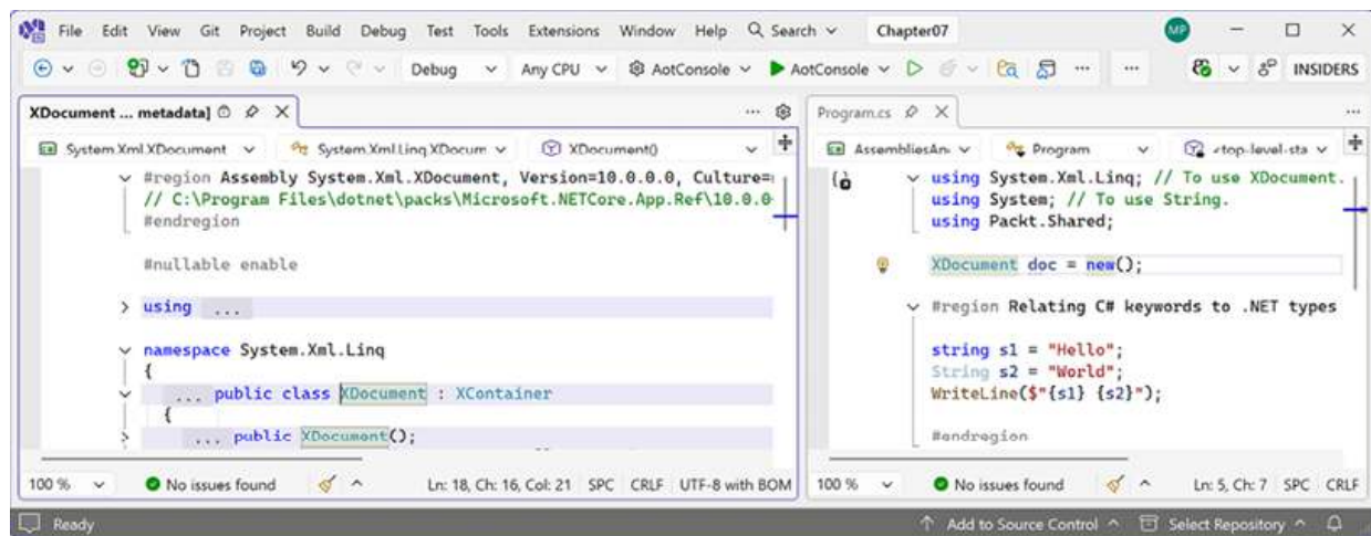
Figure 7.1: Assembly and namespace that contains the XDocument type
