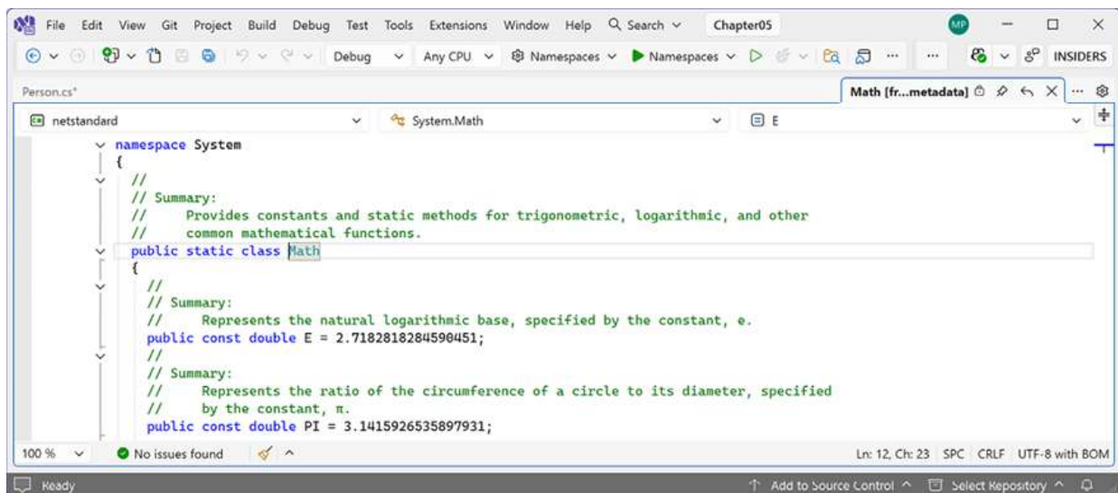
Figure 5.2: Examples of constants in the System.Math class
