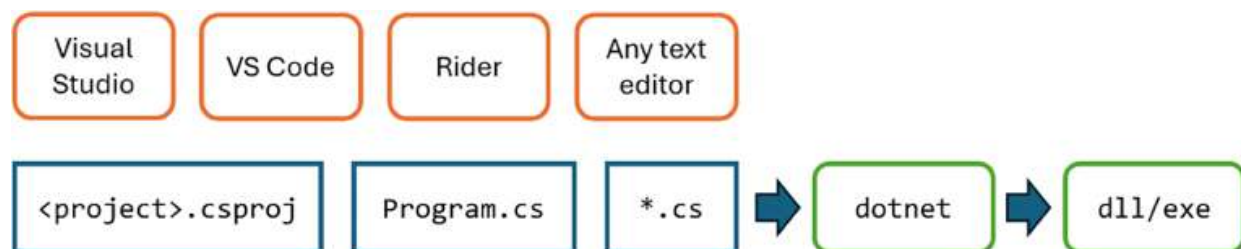
Figure 1.2: All code editors ultimately just change underlying text files
