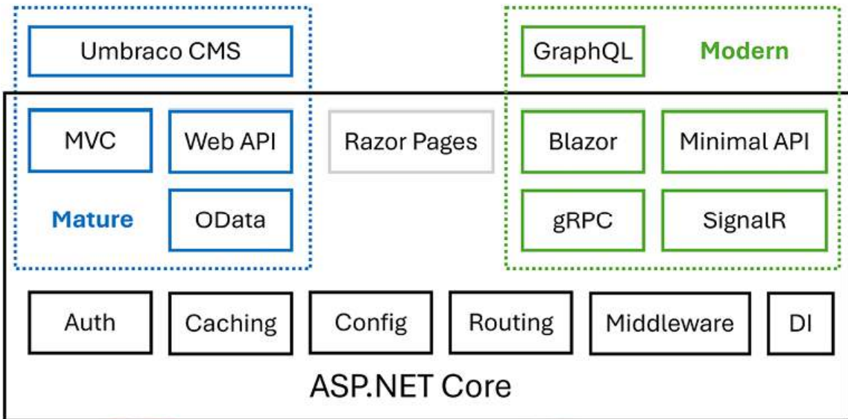
Figure 12.1: Modern or controller-based and shared ASP.NET Core components
