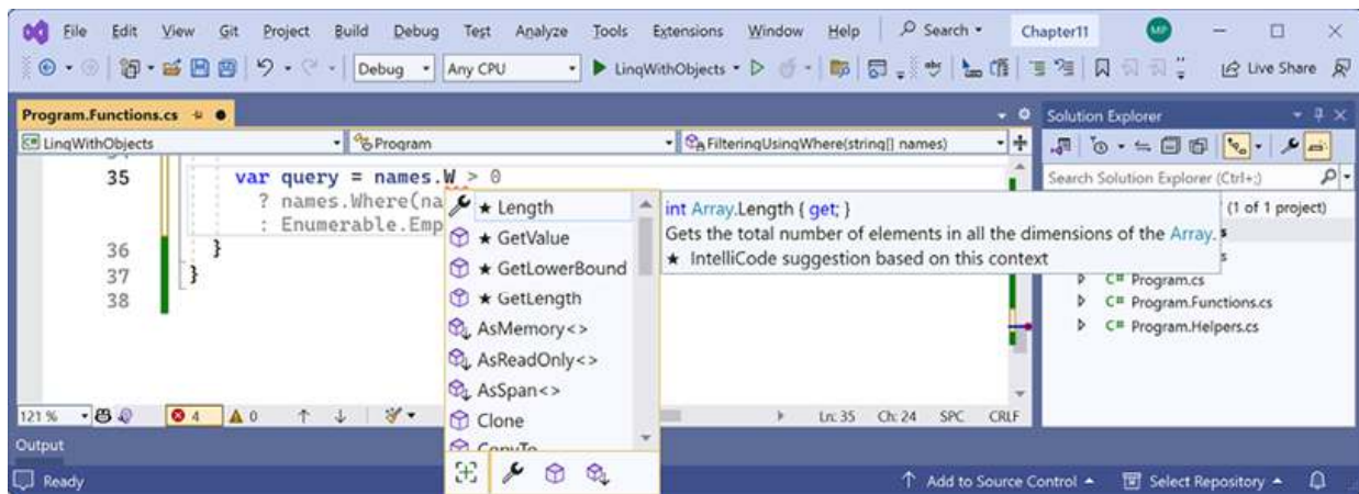
Figure 11.1: IntelliSense with the Where extension method missing
