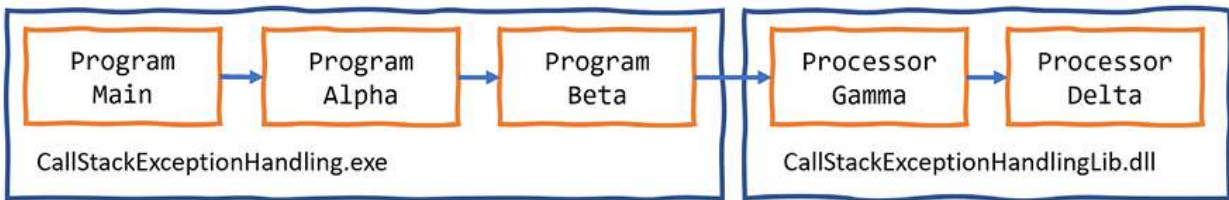
Figure 4.10: A chain of method calls that create a call stack
