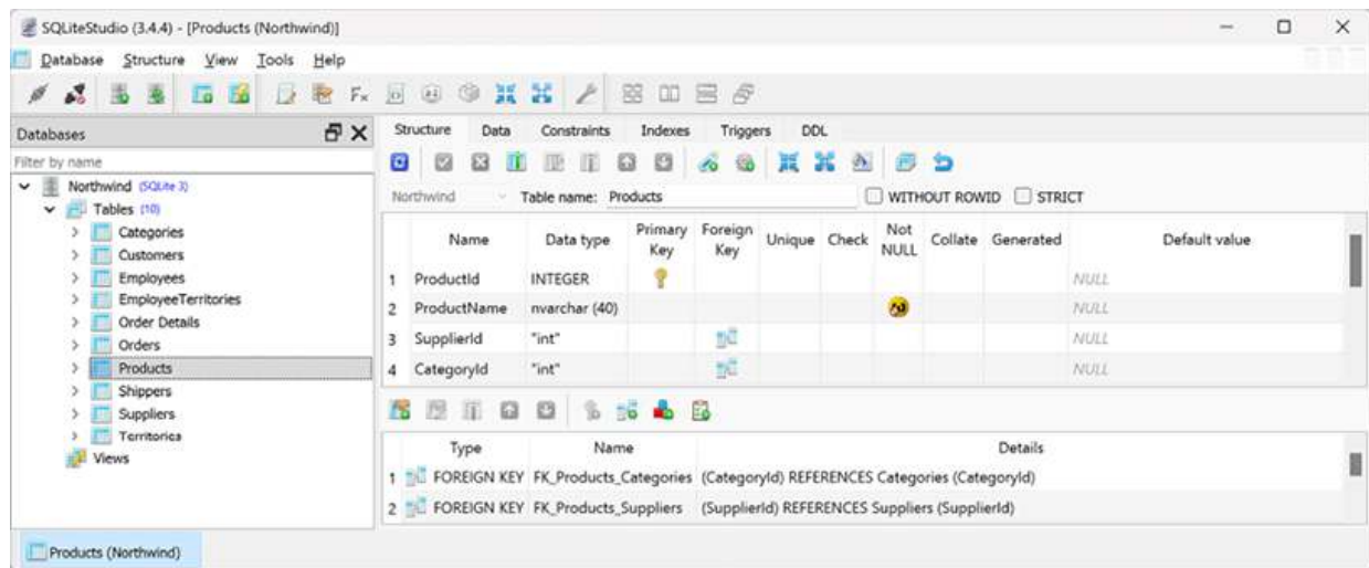
Figure 10.4: The table editor in SQLiteStudio showing the structure of the Products table
