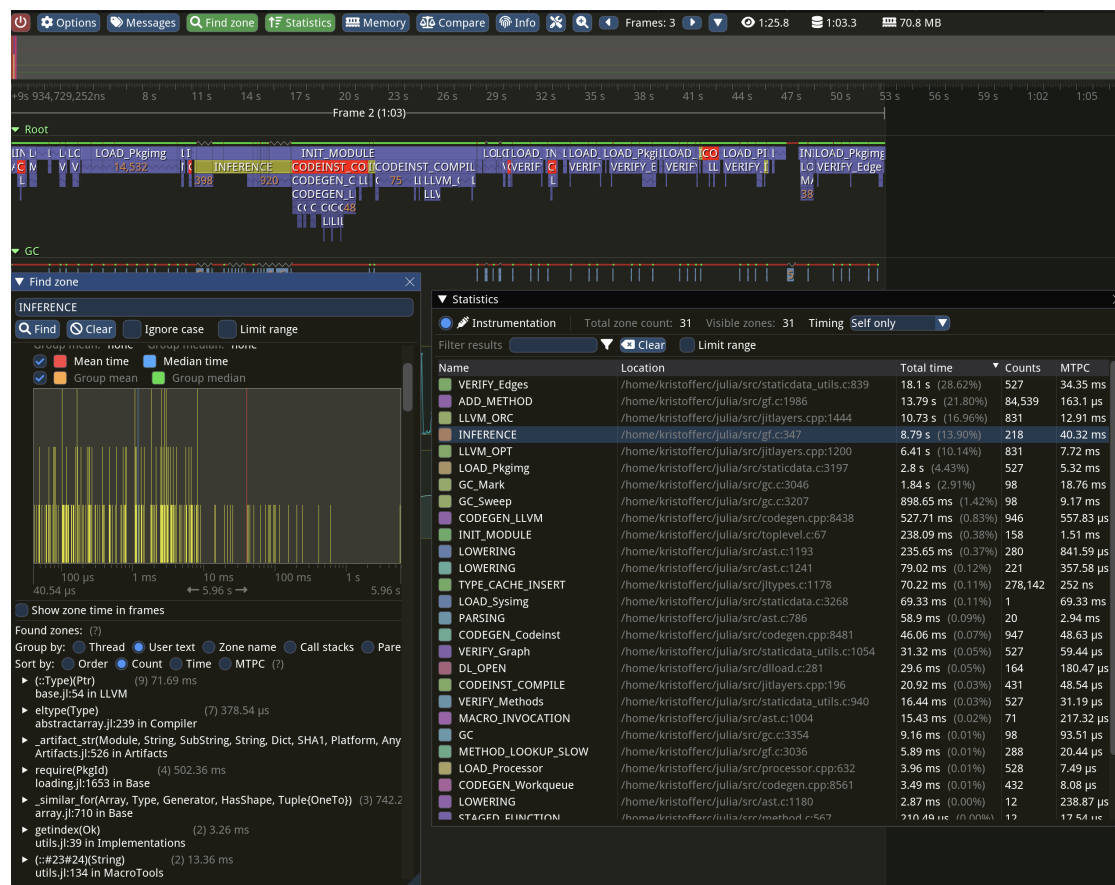
Figure 107.1: Typical Tracy usage
