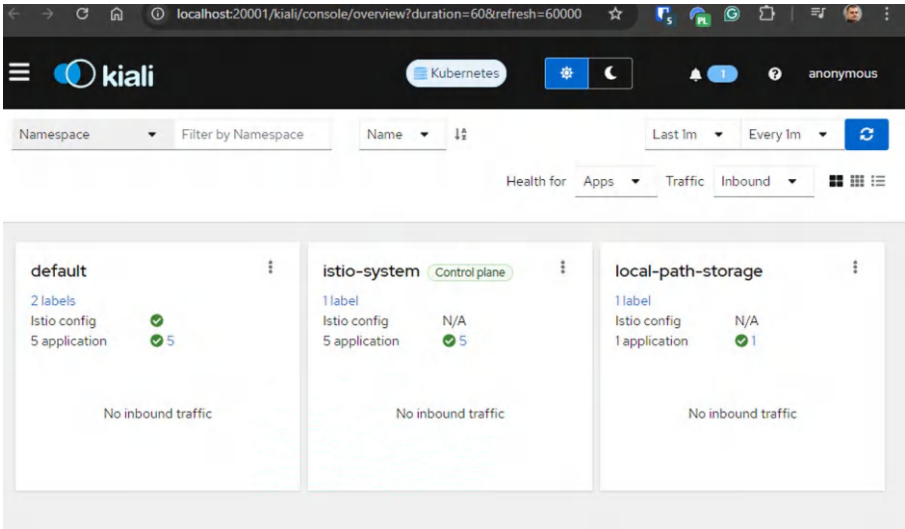
Figure 8-27. Kiali dashboard
