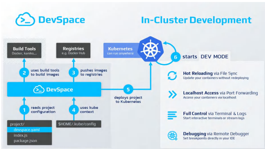
Figure 5-7. DevSpace workflow
