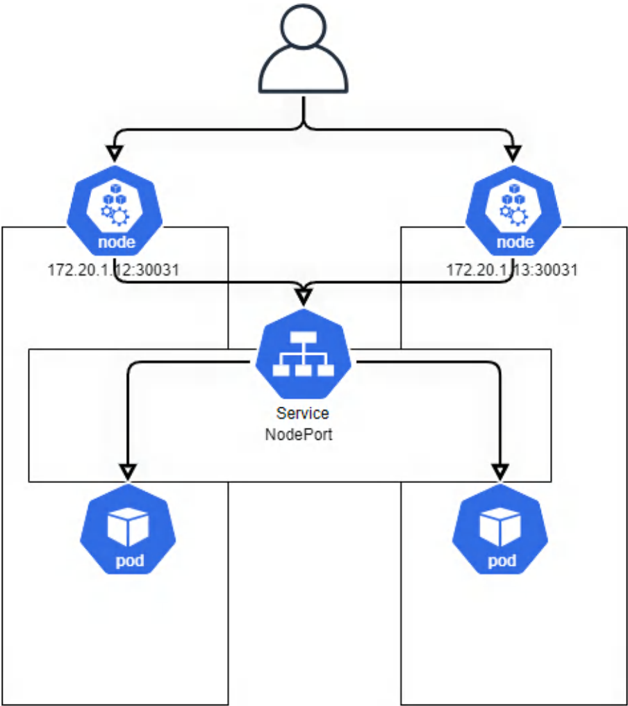
Figure 8-19. Flow of the NodePort service type
