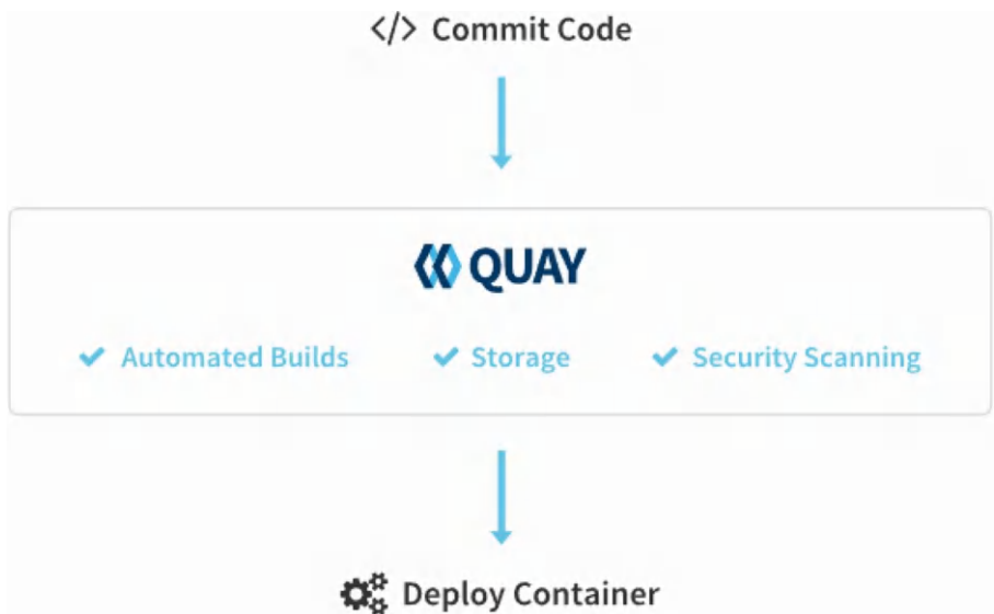
Figure 6-22. Quay workflow
