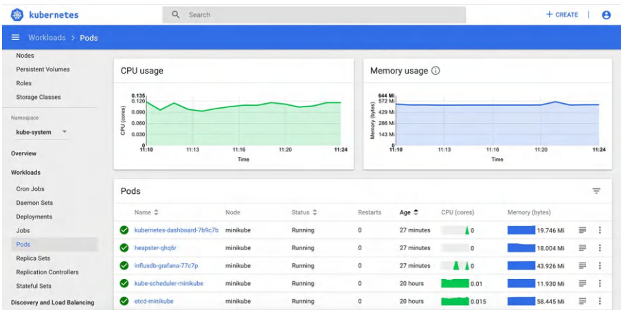
Figure 1-3. Kubernetes Dashboard
