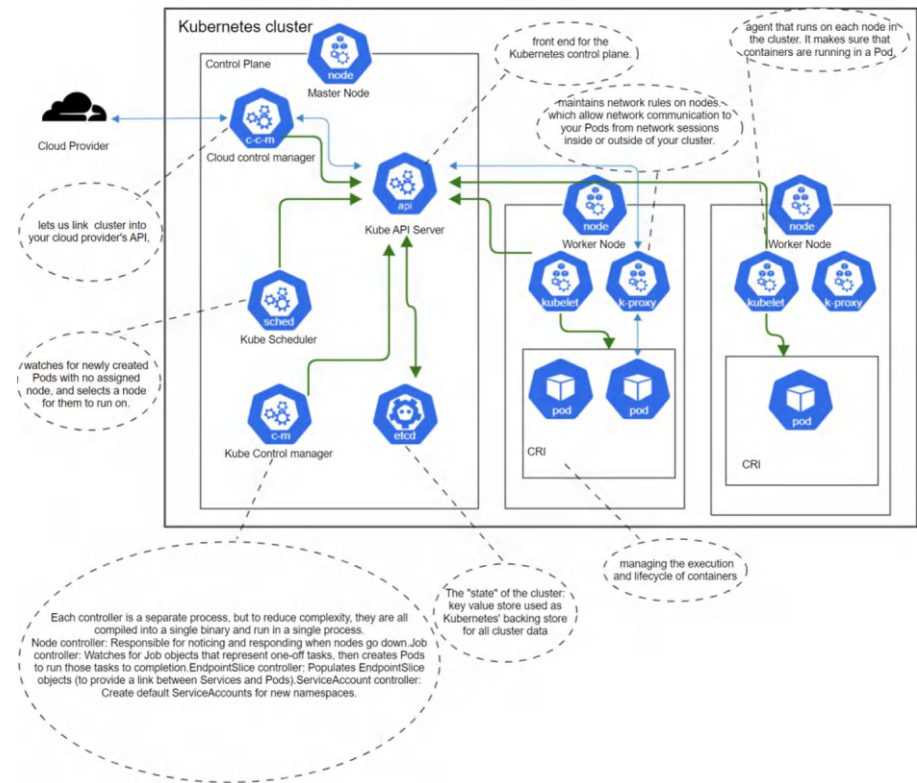
Figure 10-1. Kubernetes control plane components explanation
