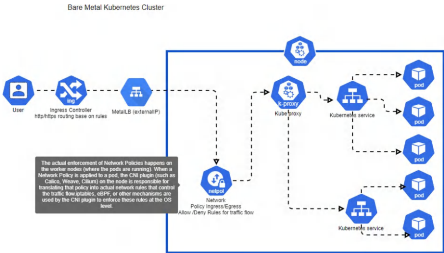
Figure 8-2. Traffic flow in a Kubernetes cluster
