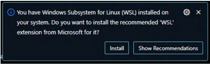
Figure 5-15. WSL extension
