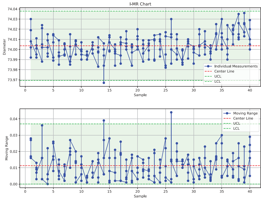
Figure 14.8 An I-MR chart, with the I-chart on top and the MR-chart below. The I-chart plots individual piston ring diameters for each sample, highlighting variation around the process mean. UCL and LCL lines indicate acceptable limits. The MR-chart tracks the moving range, or the difference between successive measurements, reflecting process variability. Lines connect data points from one sample to the next, illustrating changes in measurements and variability across samples.
