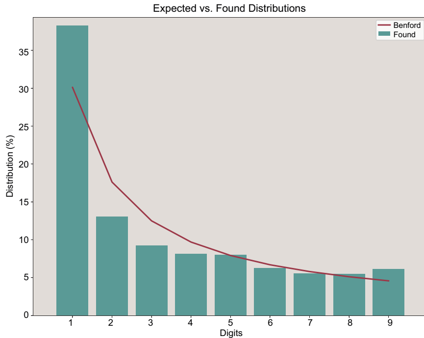
Figure 12.3 The distribution of leading digits in street addresses from East Baton Rouge Parish in Louisiana. The distribution closely resembles a perfect Benford distribution, where smaller leading digits are much more prevalent than larger leading digits. In fact, 1s, 2s, and 3s are the leading digits in 60.4% of the street addresses; in a perfect Benford distribution, those digits represent 60.2% of the observations.
