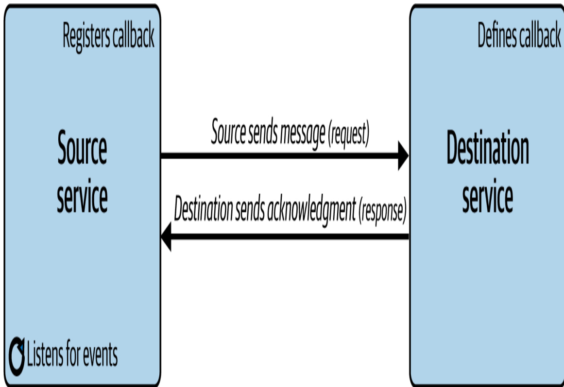
Figure 9-1. Callback architecture
