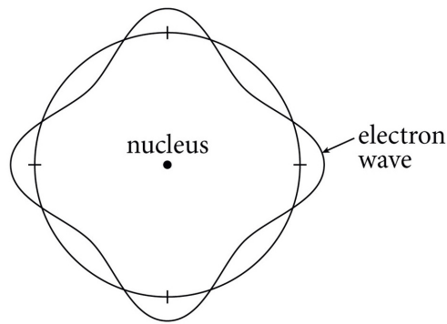
Allowed orbit
