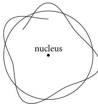
Forbidden orbit
