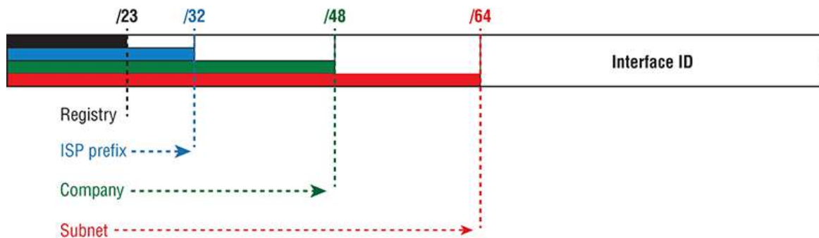
FIGURE 3.29 IPv6 global unicast addresses.
