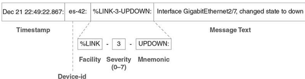
FIGURE 6.27 Anatomy of a Syslog message.
