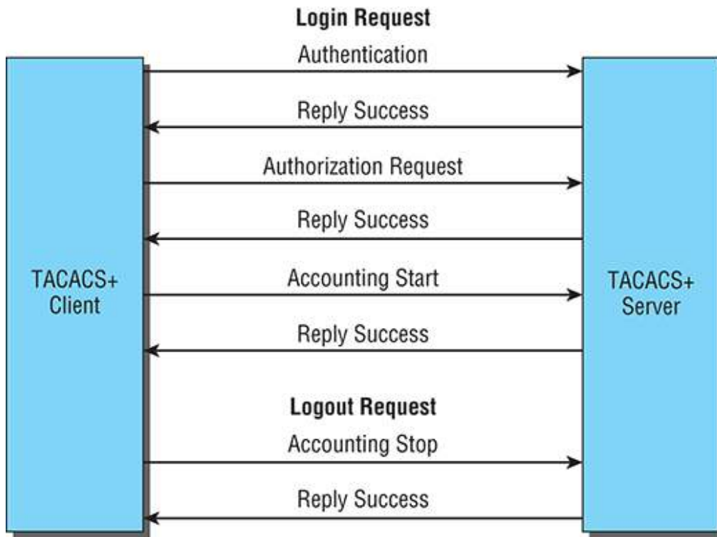
FIGURE 4.8 TACACS+ login and logout sequence.
