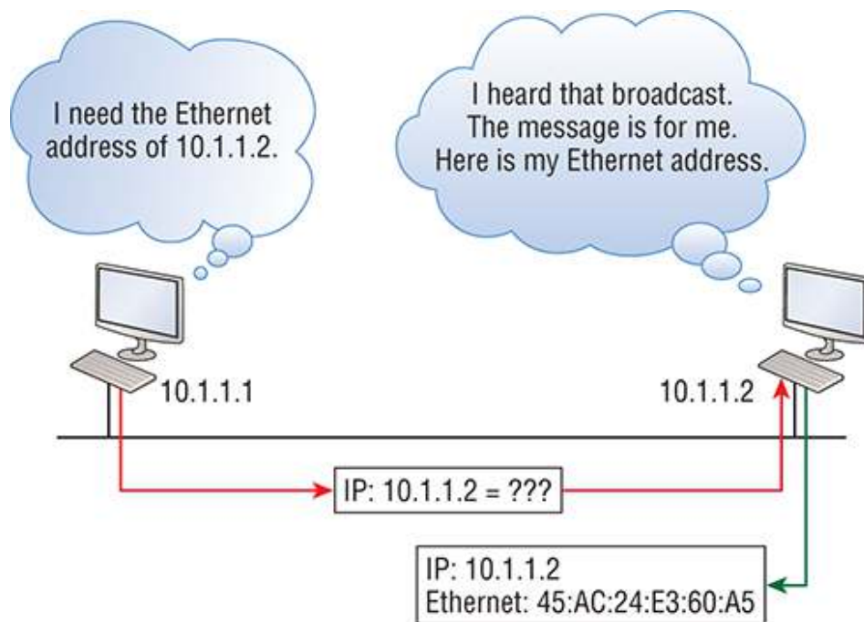
FIGURE 3.19 Local ARP broadcast.
