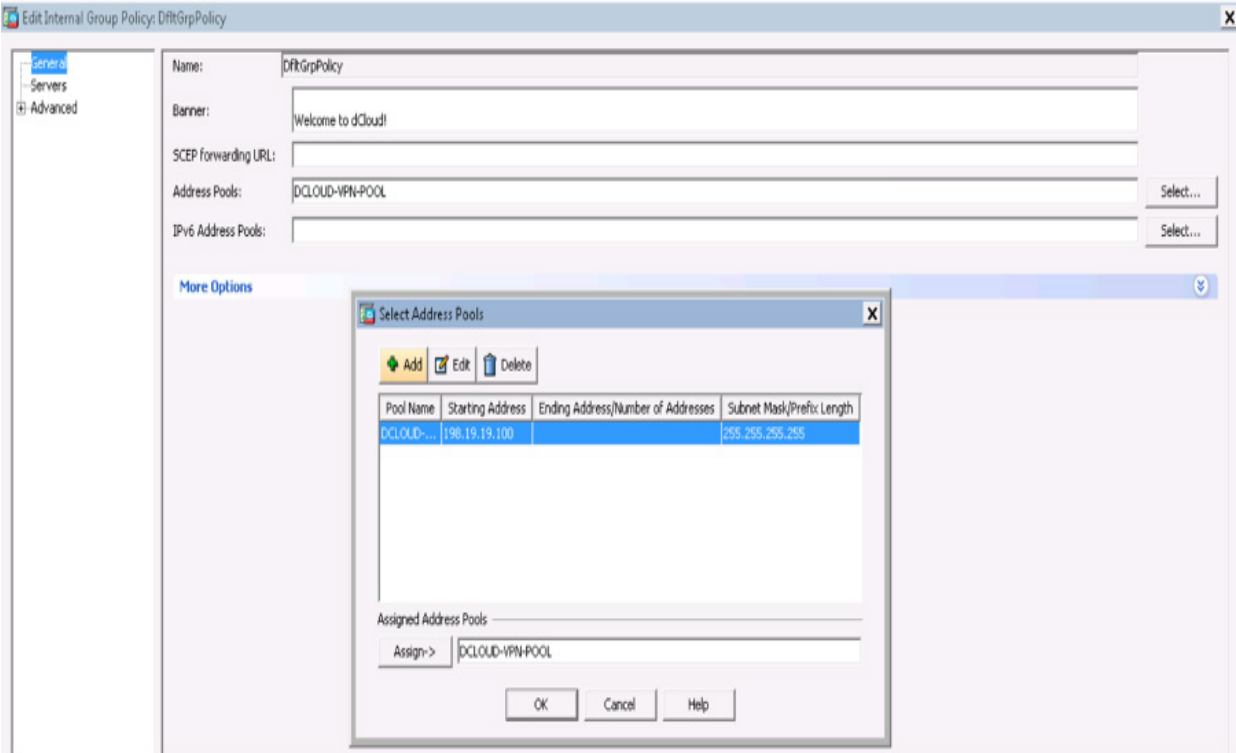
Figure 10-18 Address Pool Example with DfltGrpPolicy
