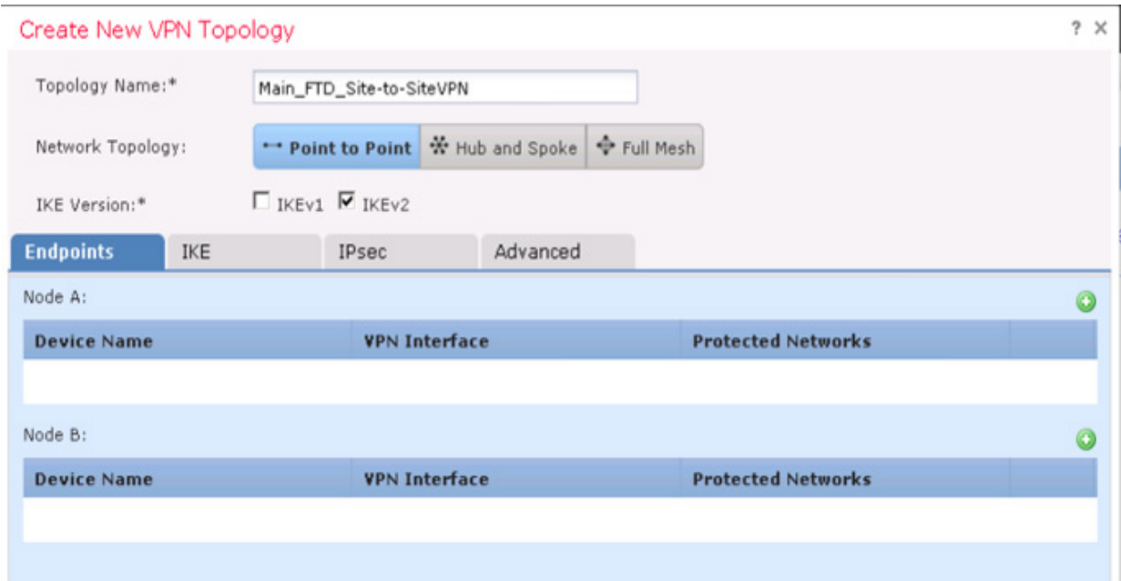
Figure 3-19 Configuring a New Site-to-Site VPN with Cisco Secure Firewall
