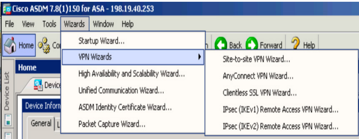
Figure 3-9 Accessing the Site-to-Site VPN Wizard in ASDM
