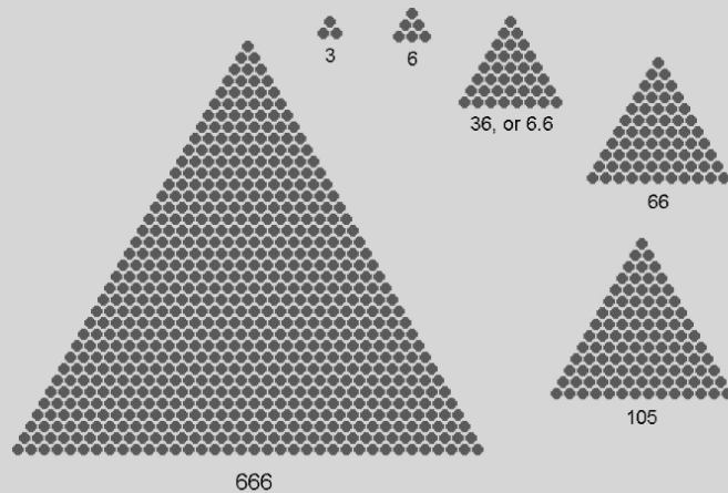
666-as-triangle with its triangular attributes
