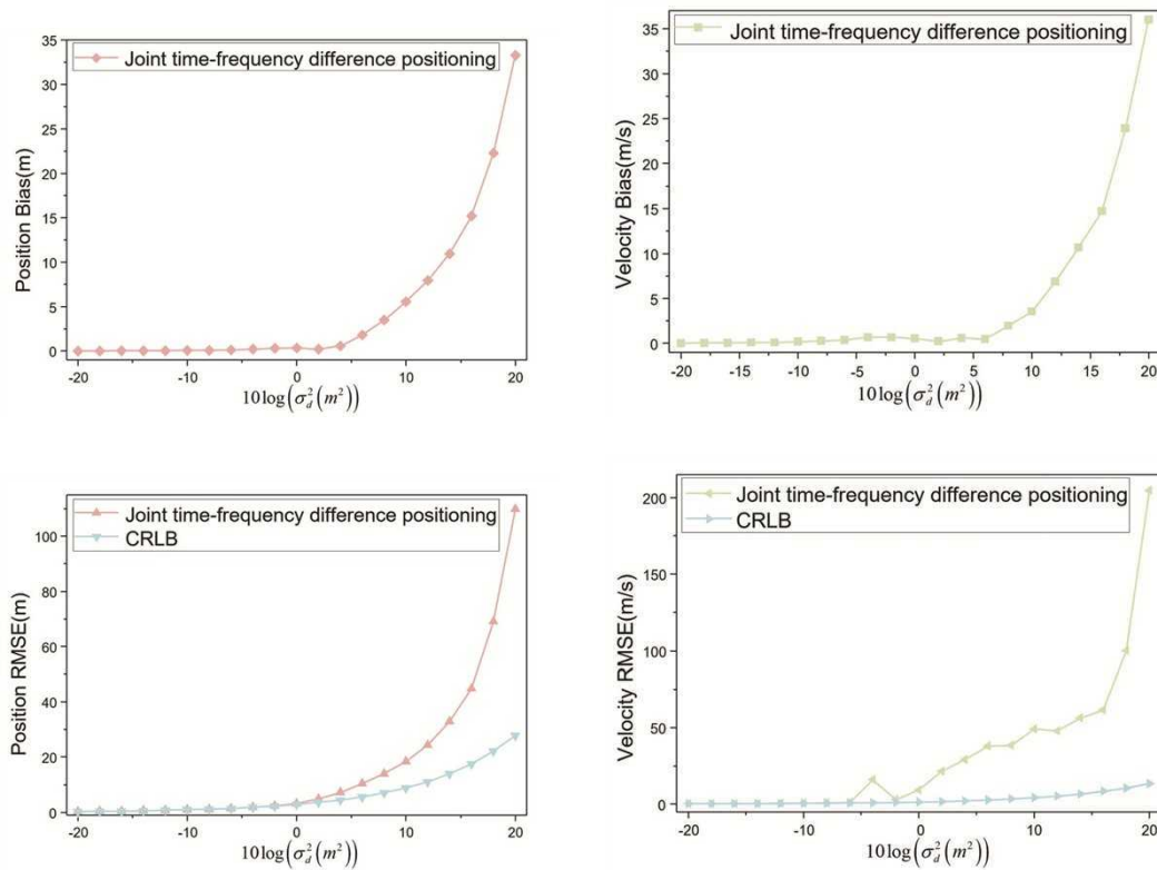
Figure 11. Positioning bias and RMSE ( \dot{R}_1(40,0,0) ).
