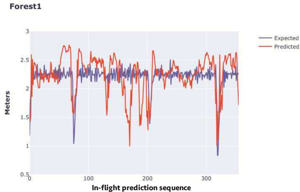
Figure 4. Predicted and expected displacement values along the route Forest1.
