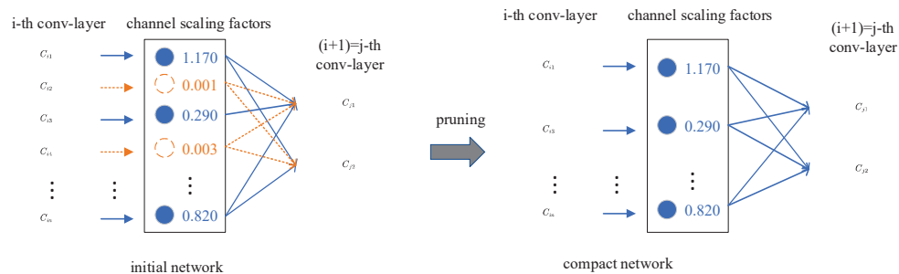
Figure 7. Pruning process diagram.
