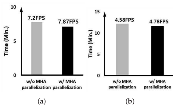
Figure 11. Comparing the MHA parallelization effect on the edge device: (a) 1 \times CSWinTT and (b) 2 \times CSWinTT.
