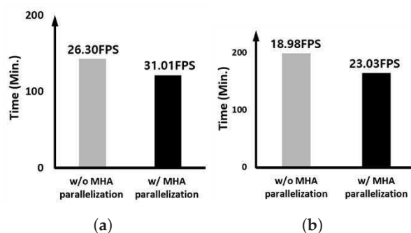
Figure 12. Comparing the MHA parallelization effect on the GPU server: (a) 1 \times CSWinTT and (b) 2 \times CSWinTT.
