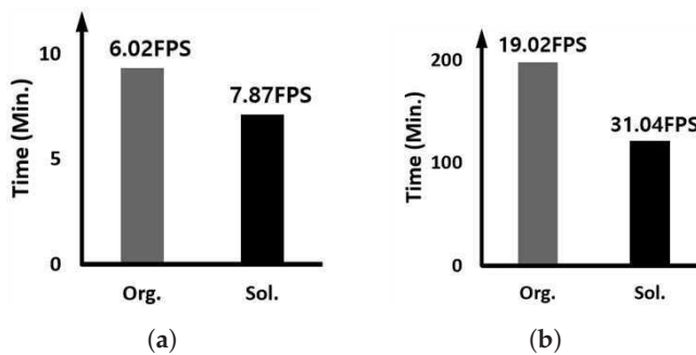
Figure 10. Comparing the execution time and speed when one CSWinTT tracker is running: (a) on the edge device and (b) on the GPU server.
