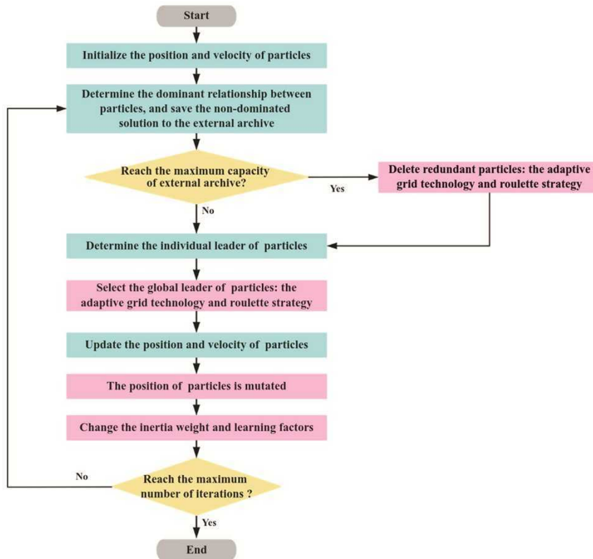
Figure 3. The improved MOPSO algorithm.
