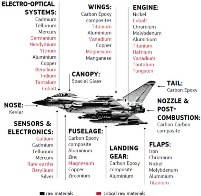
Fig. 6.1 Aircraft material requirements (European Commission, 2020: 73)
