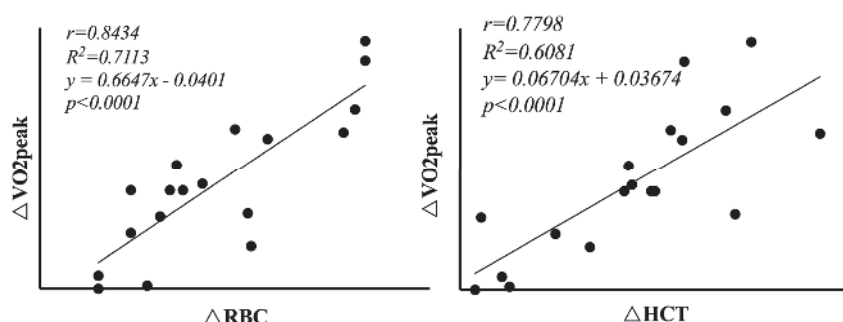
Figure 5. Linear regression model.
