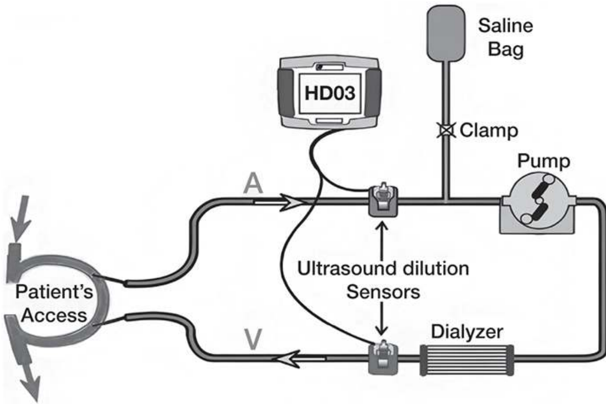
FIGURE 8.3: Setup to measure access recirculation by saline dilution and ultrasound detection. To measure access blood flow, the access needles need to be reversed (not shown). See text for description of the setup and method. (Image property of Transonic System Inc. Used with permission.)
