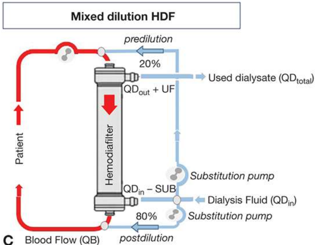
FIGURE 16.2: A. Schematic representation of online postdilution hemodiafiltration. B. Schematic representation of online predilution hemodiafiltration. C. Schematic representation of online mixed (pre + post) dilution hemodiafiltration. HDF, hemodiafiltration; UF, ultrafiltration.
