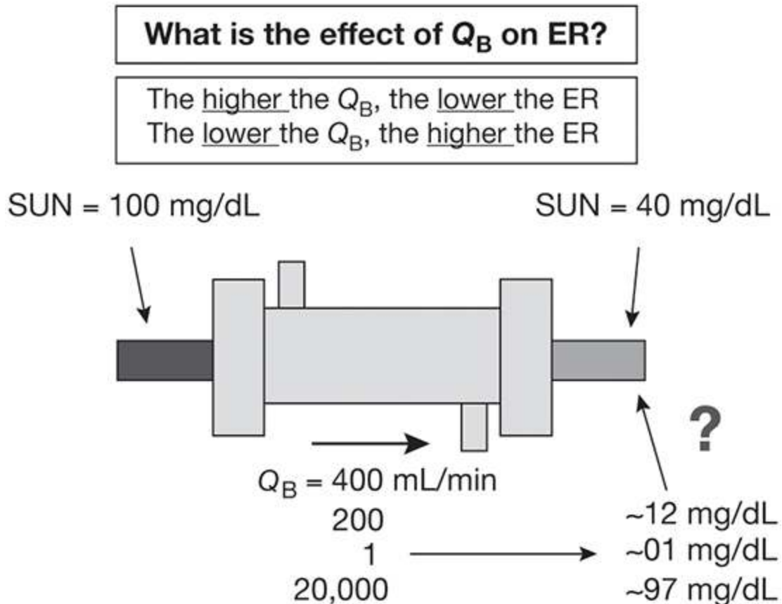
FIGURE 3.4: Effect of blood flow rate on the outlet serum urea nitrogen (SUN).
