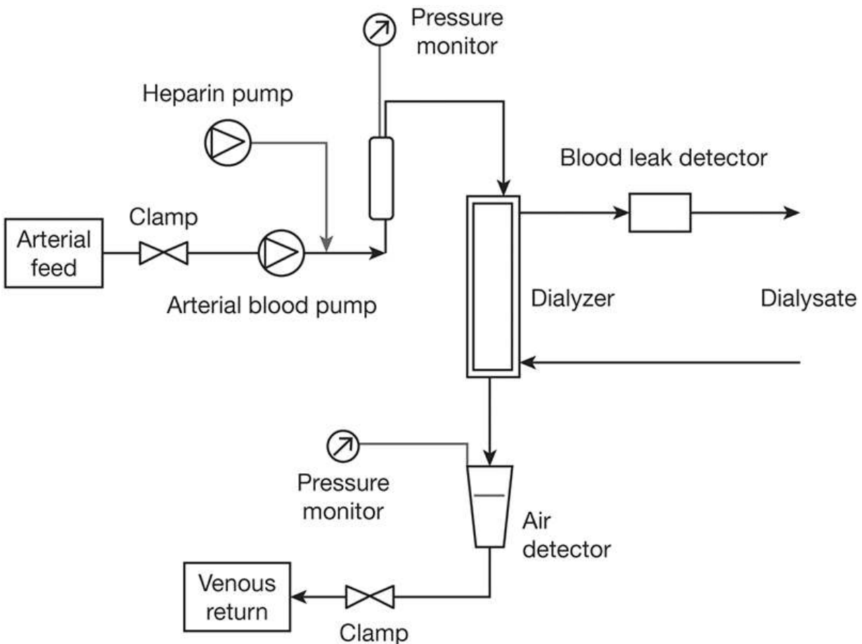
FIGURE 4.1: A typical blood circuit.
