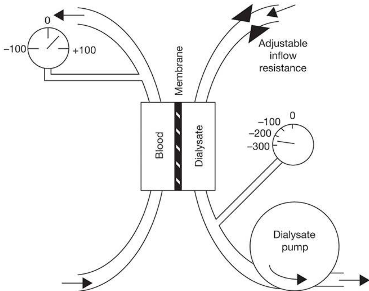
FIGURE 3.2: A dialyzer with blood flowing in one direction and dialysis solution flowing in the opposite direction. Hydrostatic pressure across the membrane (and ultrafiltration) is adjusted by varying the resistance to inflow of dialysis solution.
