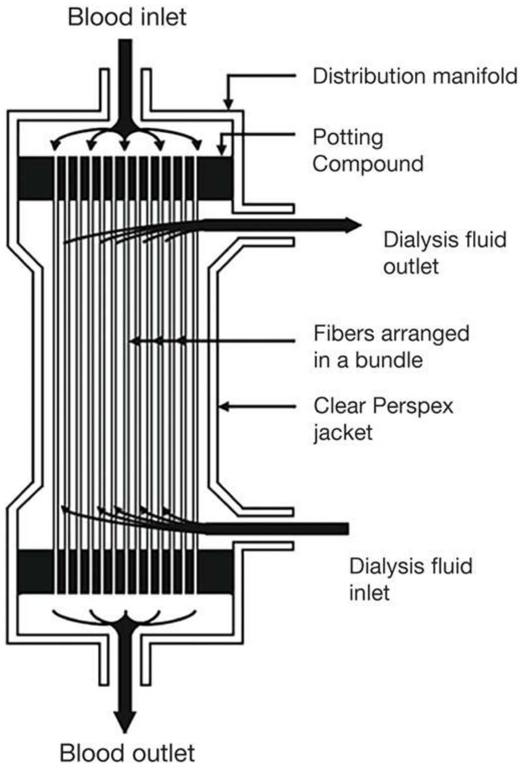
FIGURE 4.2: A schematic diagram of a typical hollow-fiber dialyzer. The patient's blood enters a distribution manifold at the dialyzer header that has been connected to the blood tubing set. Blood then flows through the fiber bundle, which is held in place at both ends by a polyurethane potting compound. Blood leaves the bundle via a second manifold at the distal end of the fiber bundle. The dialysis fluid flows in a countercurrent direction,
