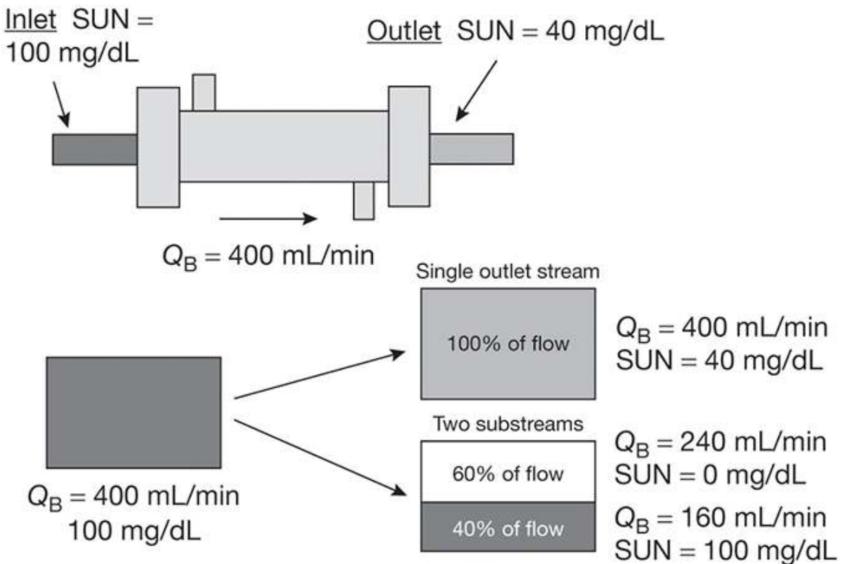
FIGURE 3.5: Concept of dialyzer clearance. The blood exiting the dialyzer can be looked at in two ways: (1) as one outlet stream where the solute concentration has been reduced by 60% (from 100 to 40 mg/dL) or (2) as two substreams: in one substream the solute concentration is unchanged, and in the other substream the solute has been completely removed. The flow rate of the cleared substream is the dialyzer "clearance" and is equal to the extraction ratio multiplied by the blood flow rate. SUN, serum urea nitrogen.
