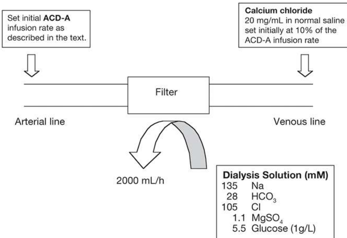
FIGURE 14.4: Circuit diagram for citrate slow continuous hemodialysis. The MgSO 4 level has been modified to 1.1 mM (vs 1.3 mM as originally depicted in the Swartz publication). ACD-A, anticoagulant citrate dextrose form A (Based on information in Swartz R, et al. Improving the delivery of continuous renal replacement therapy using regional citrate anticoagulation. Clin Nephrol. 2004;61:134-143.)
