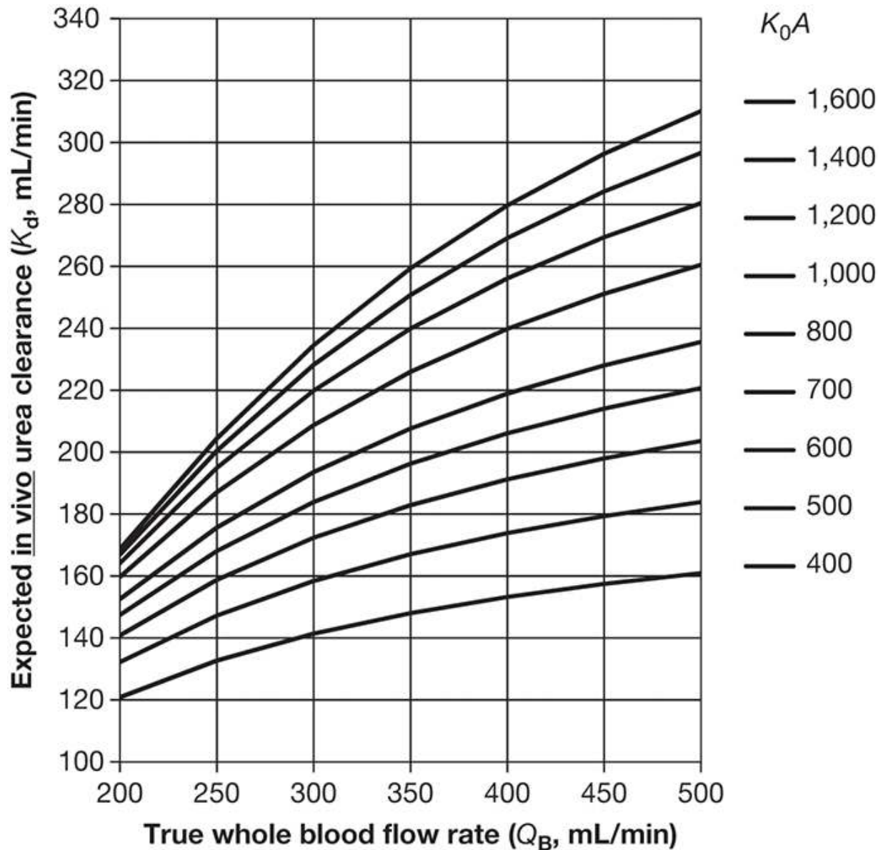
FIGURE 3.6: Relationship between blood flow rate ( Q_B ) and dialyzer blood water urea clearance ( K ) as a function of dialyzer efficiency ( K_0A ). Each isopleth (curved line) represents a different dialyzer having a different K_0A value. To use the nomogram, find the blood flow rate on the horizontal axis, then move up to the dialyzer K_0A being used, and read the expected dialyzer urea clearance on the vertical axis. Theoretical clearance values have been adjusted to more closely reflect expected values in vivo.
