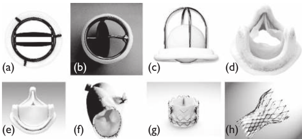
Fig. 4.3 Common types of heart valve prostheses. (a) Bileaflet mechanical valve (St Jude). (b) Monoleaflet mechanical valve (Medtronic Hall). (c) Caged ball valve (Starr-Edwards). (d) Stented porcine bioprosthesis (Medtronic Mosaic). (e) Stented pericardial bioprosthesis (Carpentier-Edwards Magna). (f) Stentless porcine bioprosthesis (Medtronic Freestyle). (g) Percutaneous bioprosthesis expanded over a balloon (Edwards Sapien). (h) Self-expandable percutaneous bioprosthesis (CoreValve).
