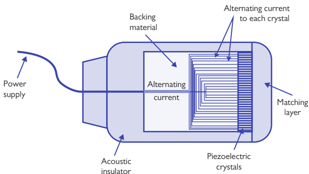
Fig. 12.2 Components of a transducer.
