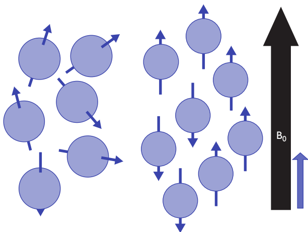
Fig. 12.31 Proton alignment. In the presence of an external magnetic field ( B_0 ), protons either align in a parallel or an antiparallel fashion to B_0 . As more protons align to B_0 , there is net magnetization in this direction.
