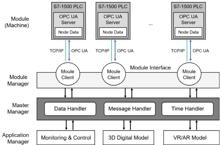
Fig. 1 Proposed digital twin model
