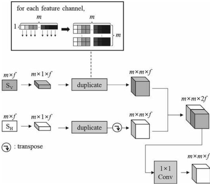
Fig. 3 Merging spatial feature maps of top and left blocks
