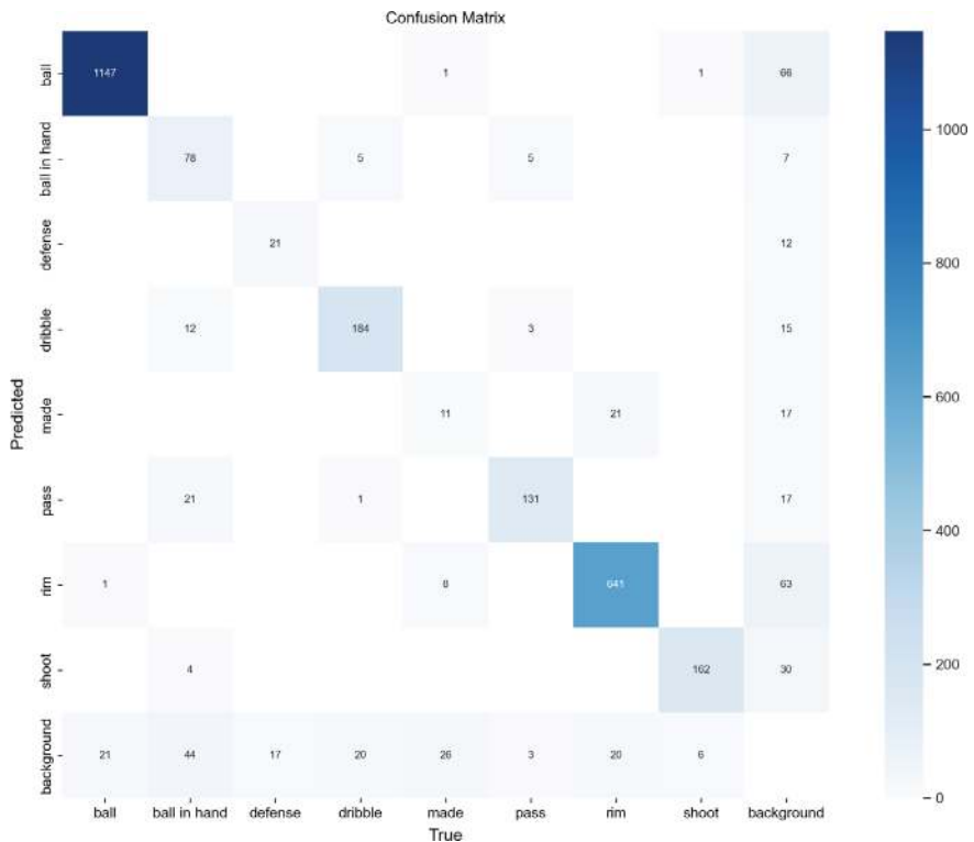
Fig. 10 Confusion matrix
