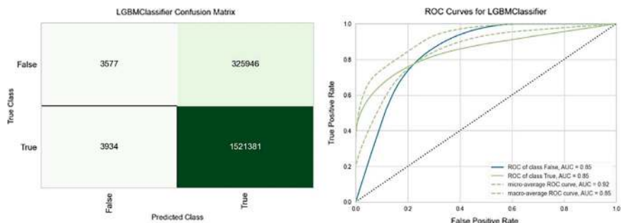
Fig. 1 Performance evaluation of the model. Left: confusion matrix for a single evaluation; right: ROC curve from 10 evaluations
