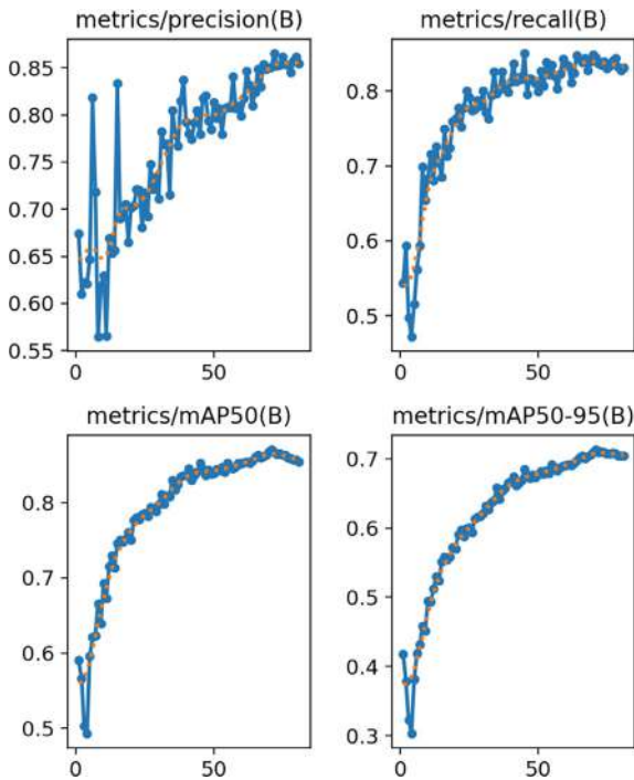
Fig. 8 The results of model training (Continue)
