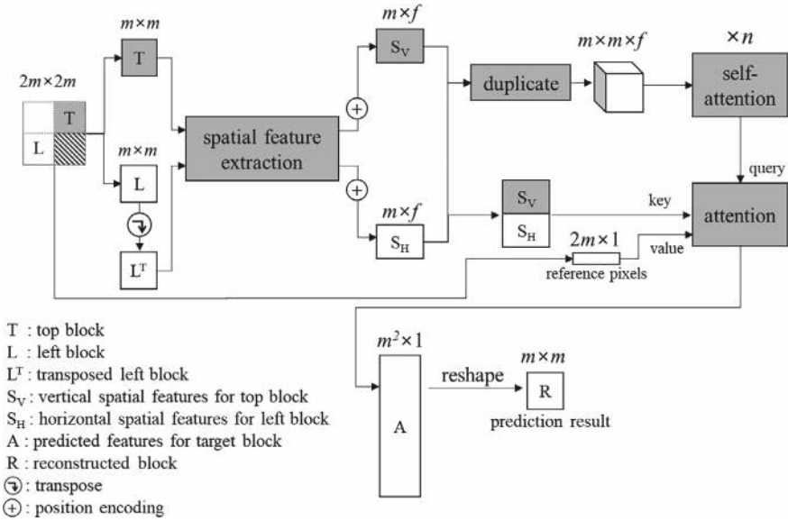
Fig. 1 Flow of the proposed method
