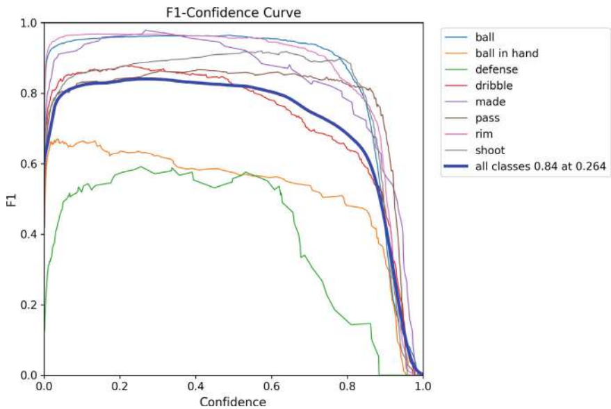
Fig. 9 F1-confidence curve
