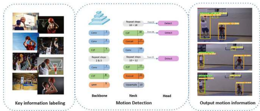
Fig. 2 Flow of motion recognition
