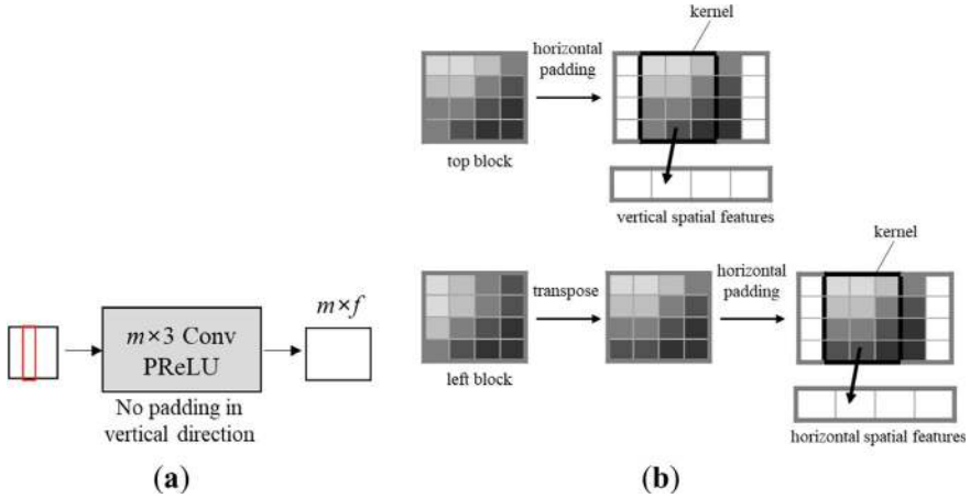
Fig. 2 Spatial feature extraction for reference pixels through CNN layer, a structure for spatial feature extraction and b spatial feature extractions for top and left blocks
