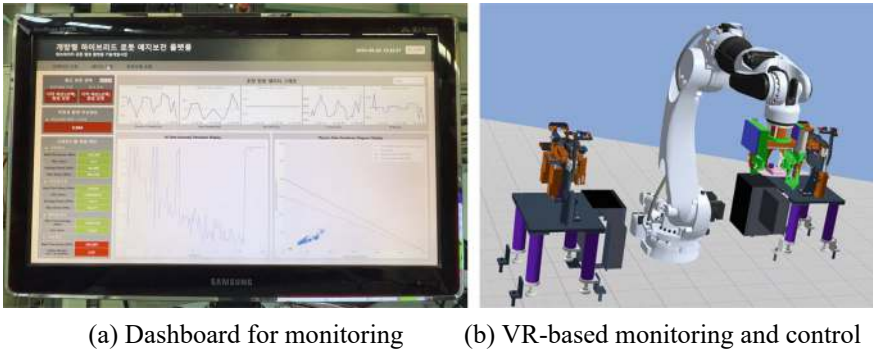
Fig. 7 Visualization and monitoring for assembly robot
