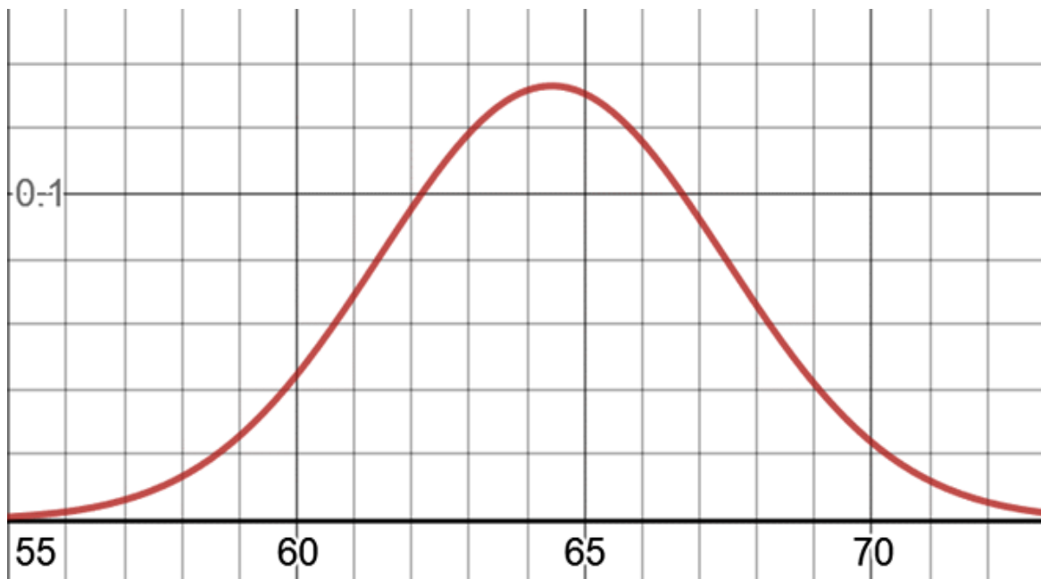
Figure 3-2. A normal distribution
