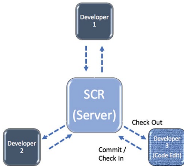
Figure 6-6. A centralized version control system
