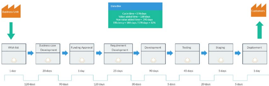
Figure 15-6. Value stream map for a software development process
