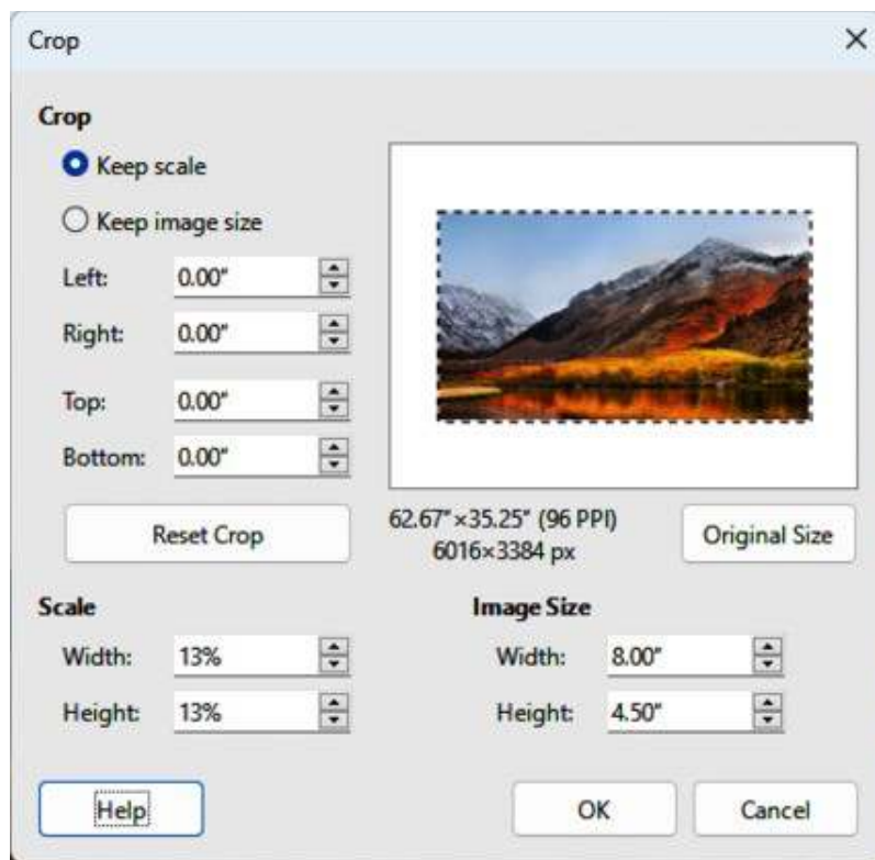
Figure 119: Crop dialog
