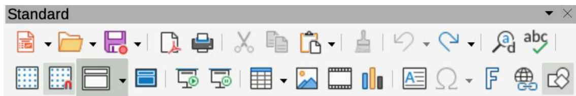
Figure 284: Standard toolbar
