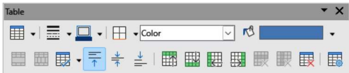
Figure 86: Table toolbar
