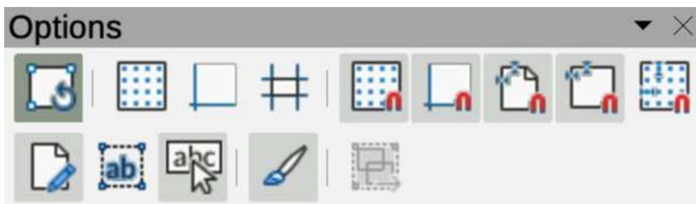
Figure 154: Options toolbar
