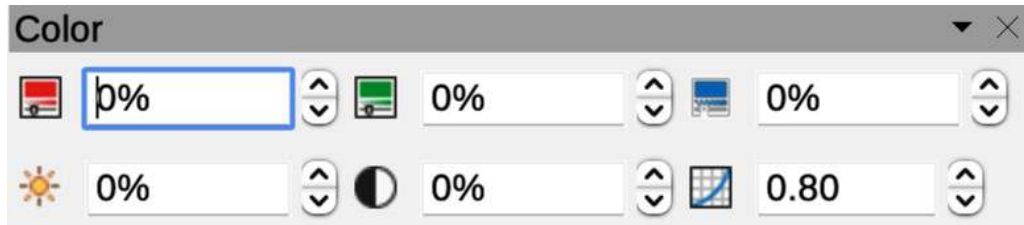
Figure 369: Color subtoolbar
