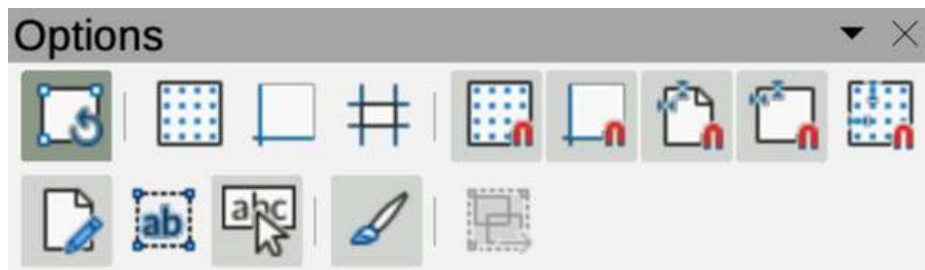
Figure 304: Options toolbar
