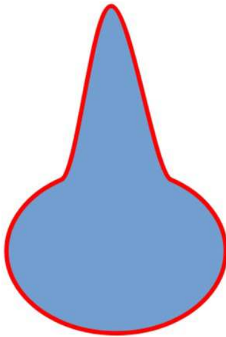
Figure 186: Example arrowhead
