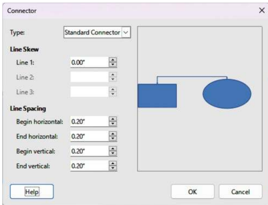
Figure 164: Connector dialog
