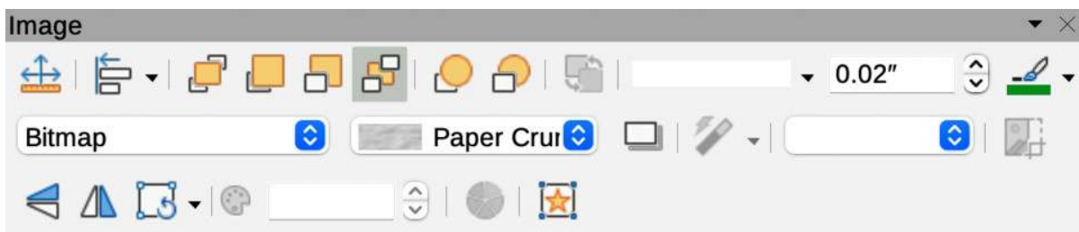
Figure 109: Image toolbar
