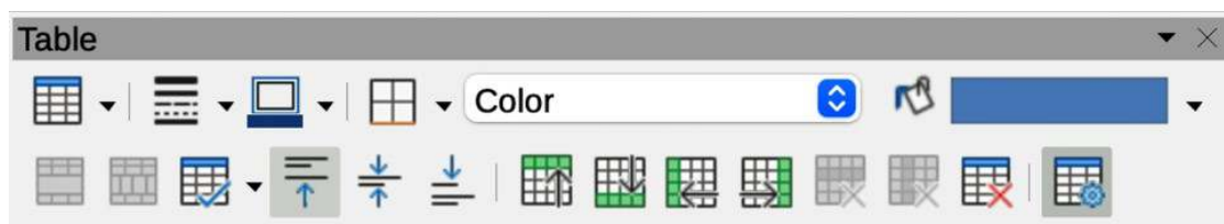
Figure 358: Table toolbar
