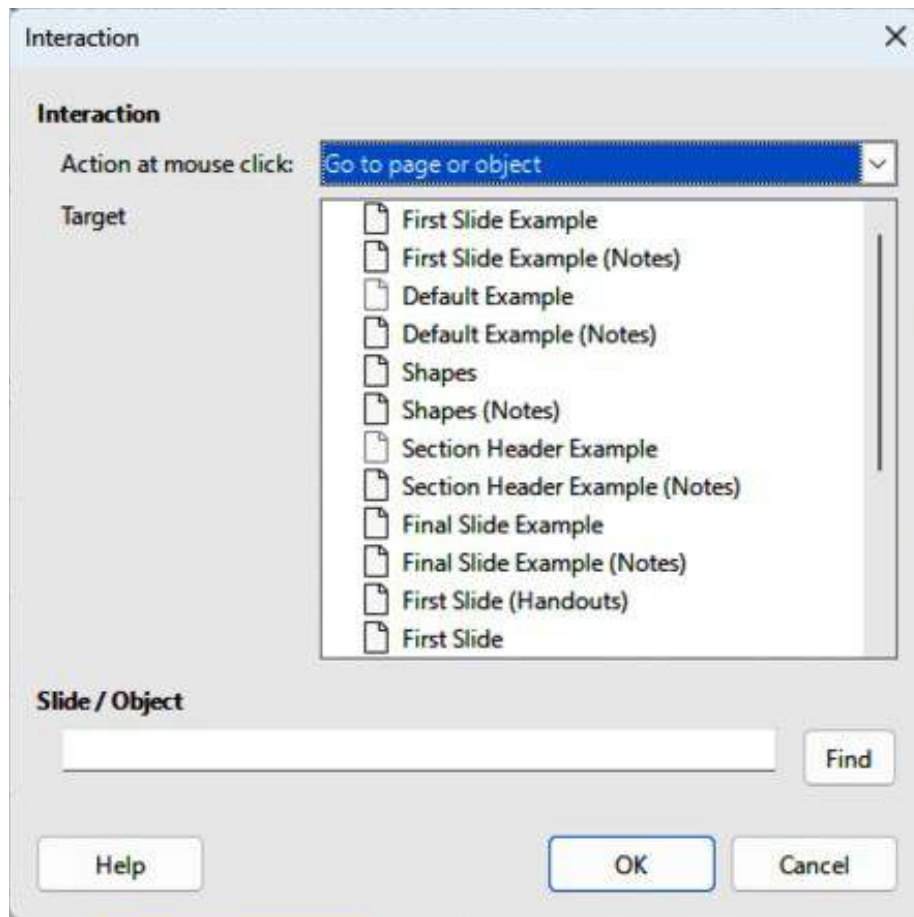
Figure 271: Interaction dialog
