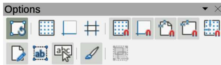
Figure 350: Options toolbar
