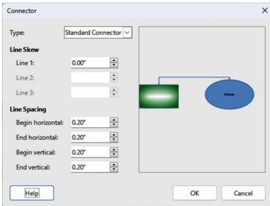
Figure 209: Connector dialog
