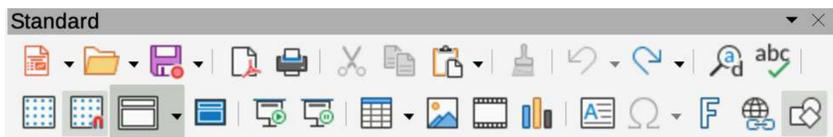
Figure 11: Standard toolbar
