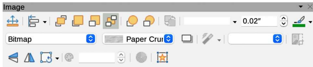
Figure 343: Image toolbar
