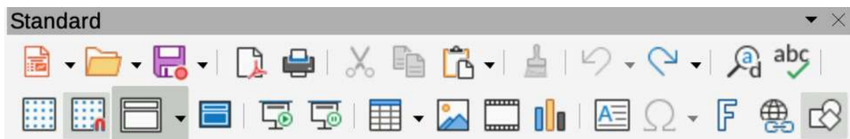
Figure 50: Standard toolbar
