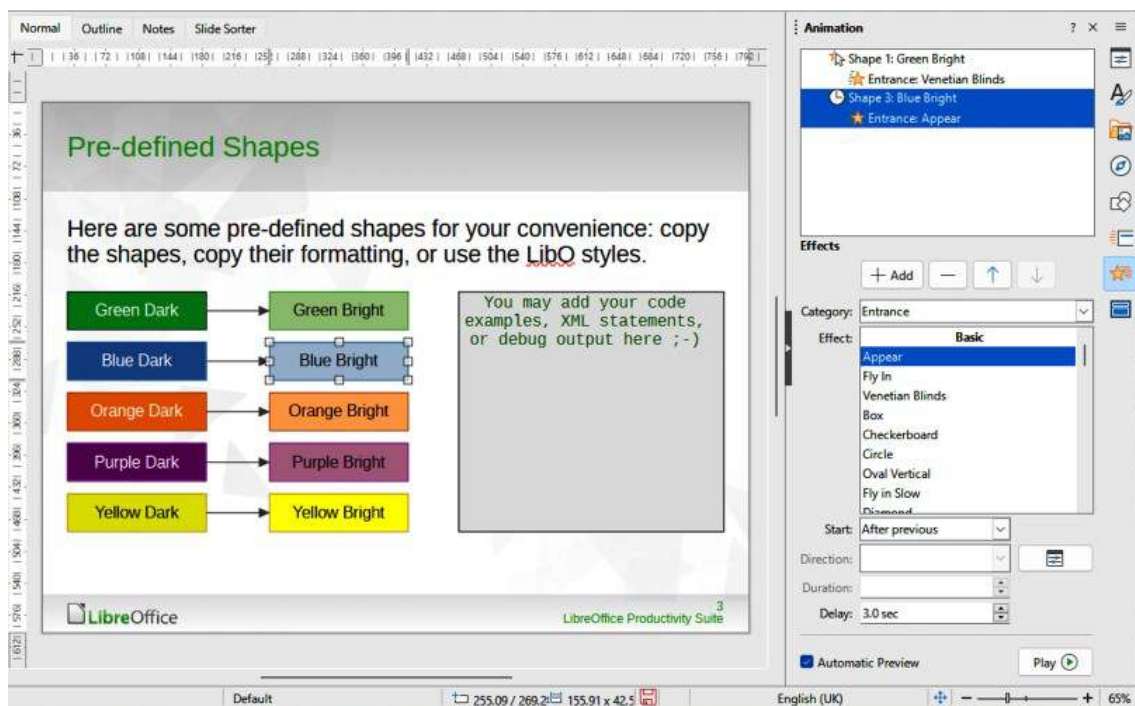
Figure 270: Example animation
