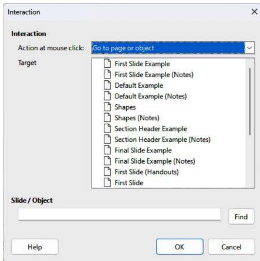
Figure 168: Interaction dialog
