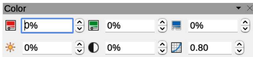
Figure 113: Color sub-toolbar
