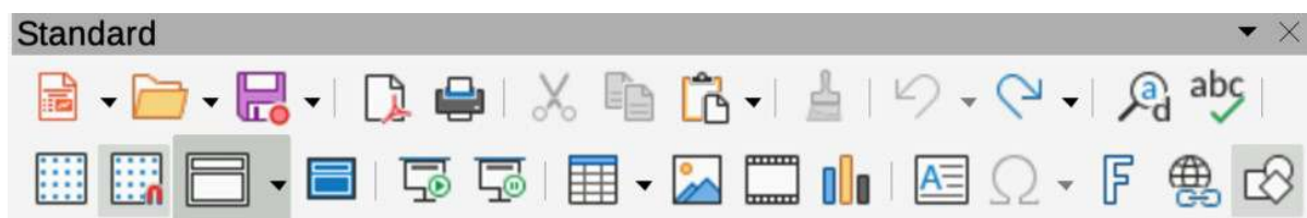
Figure 355: Standard toolbar
