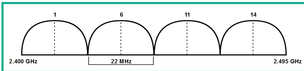
Figure 13.2 – Non-overlapping wireless channels
