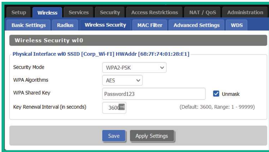
Figure 13.18 – Wireless router configurations
