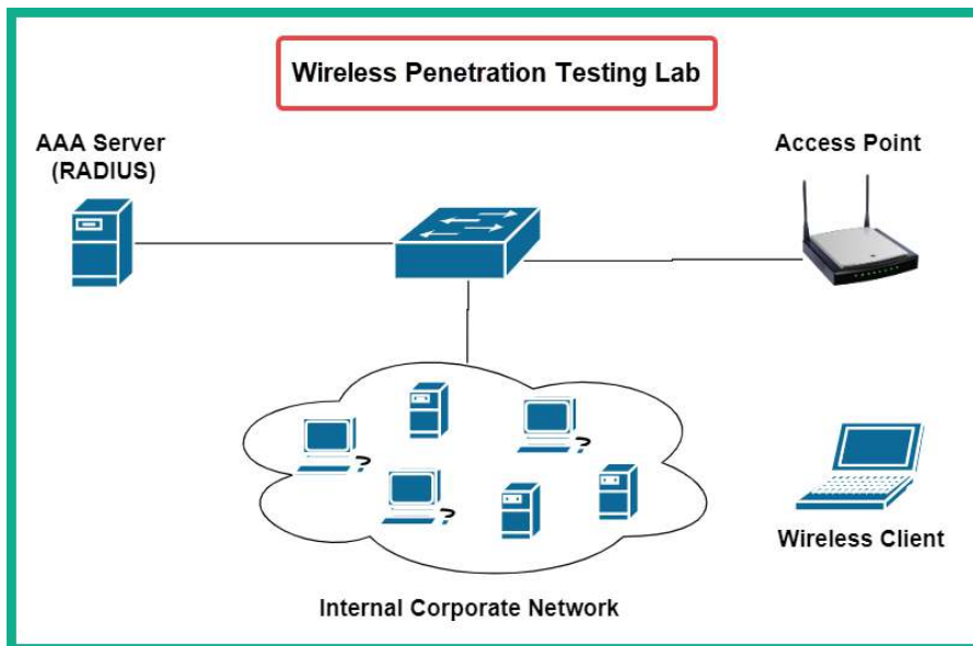
Figure 3.21 – Wireless penetration testing lab
