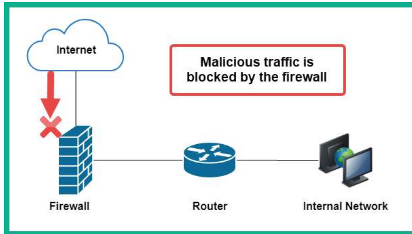
Figure 5.31 – Network-based firewall
