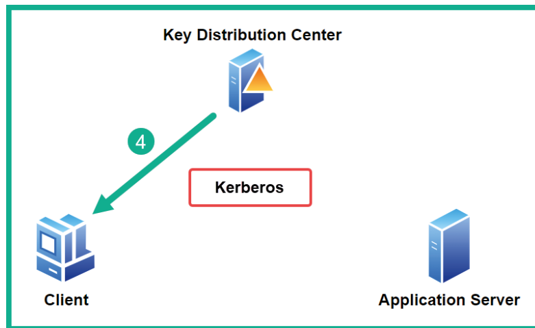
Figure 11.4 – Phase 4
