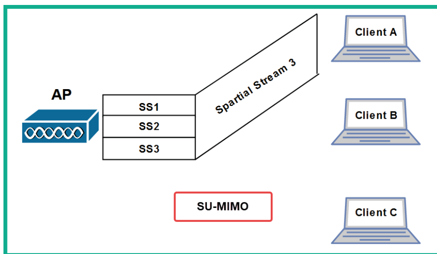
Figure 13.6 – SU-MIMO
