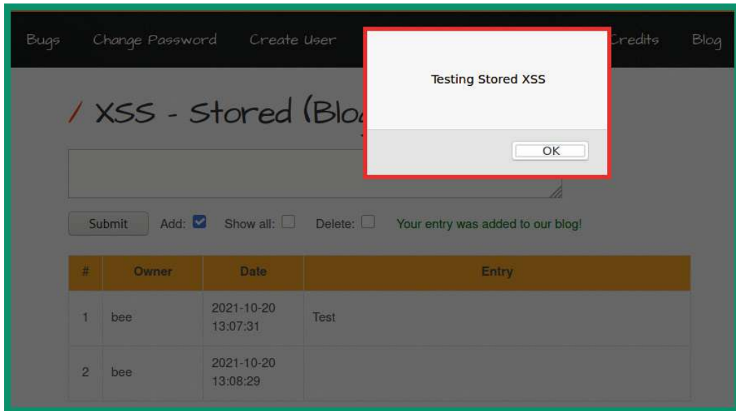
Figure 16.44 – Performing stored XSS
