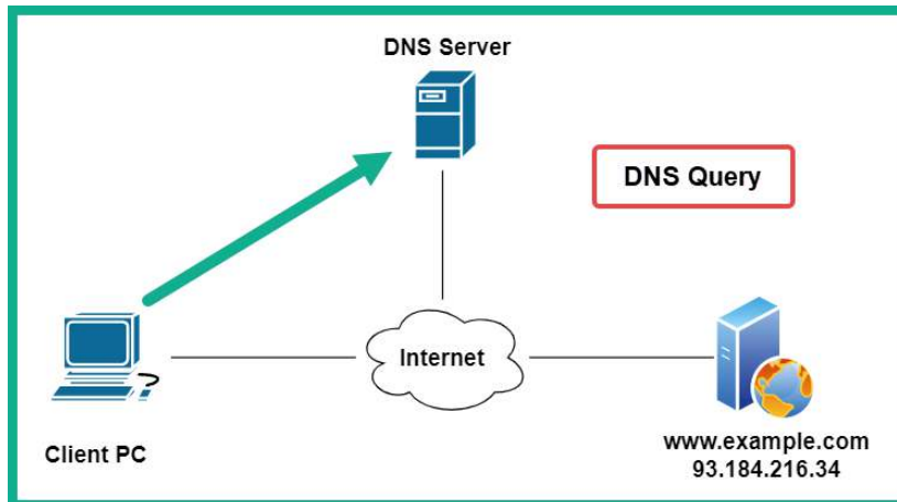
Figure 5.10 – DNS query
