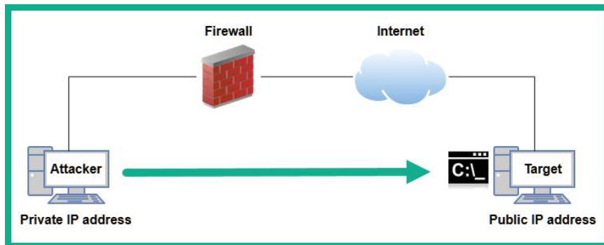
Figure 7.3 – Bind shell
