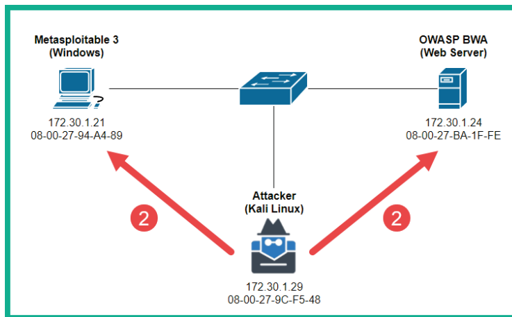
Figure 9.47 – Gratuitous ARP messages
