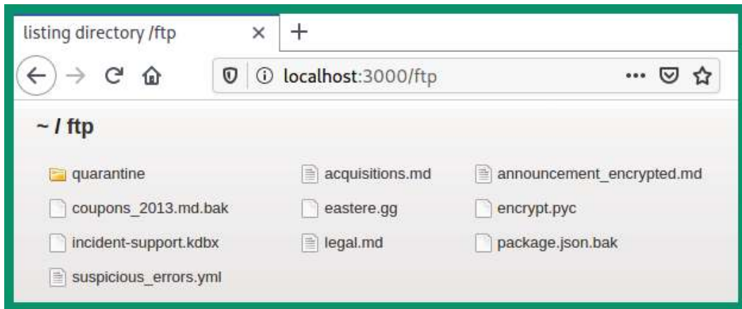
Figure 16.1 – Insecure directory
