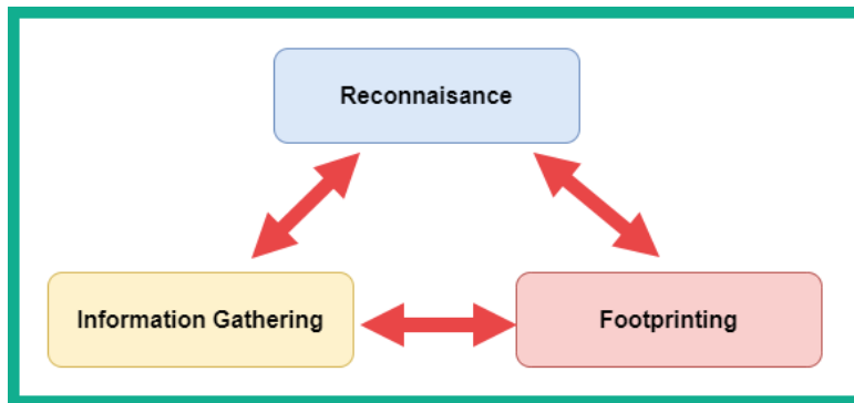
Figure 4.1 – Footprinting
