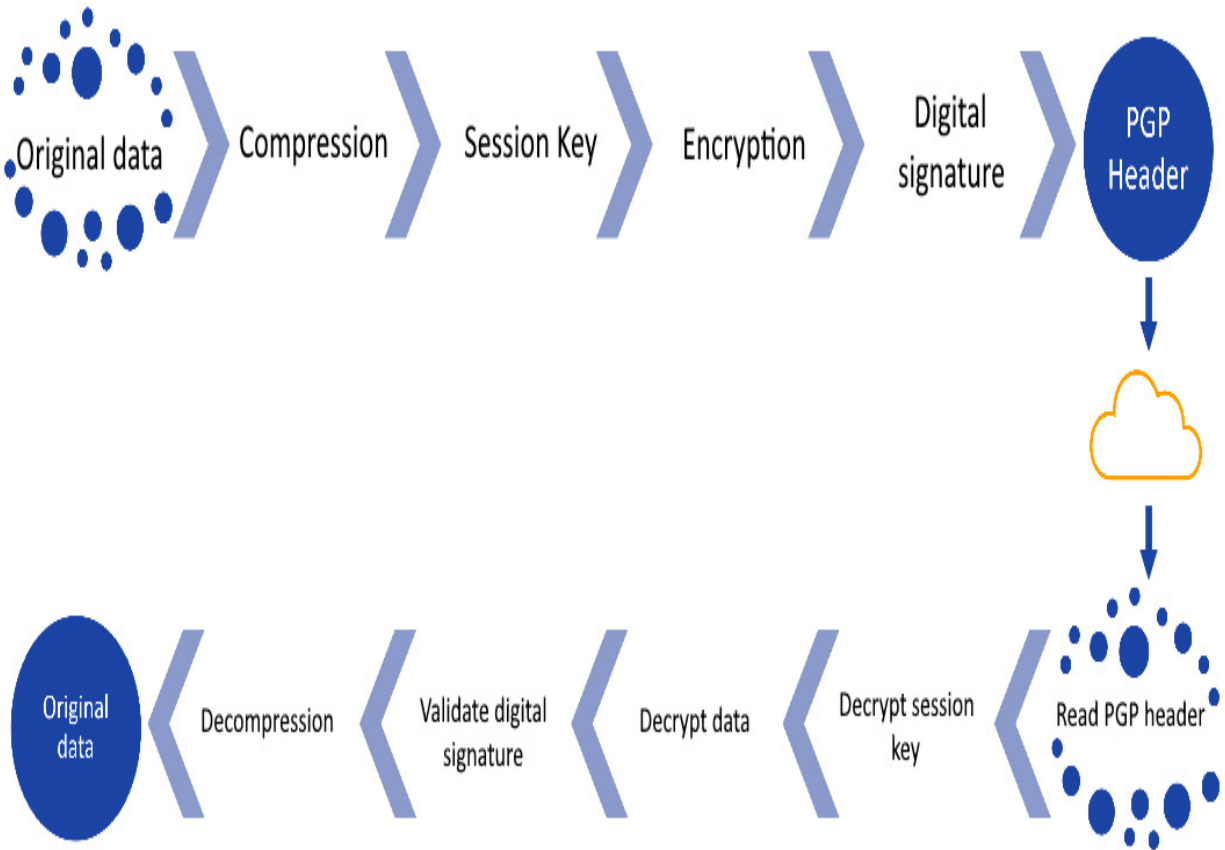
Figure 16.8 – PGP flow
