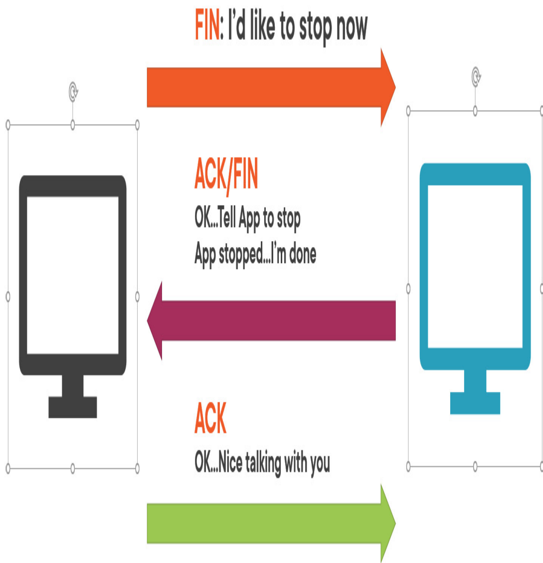
Figure 4.2 – Three-way handshake after transfer
