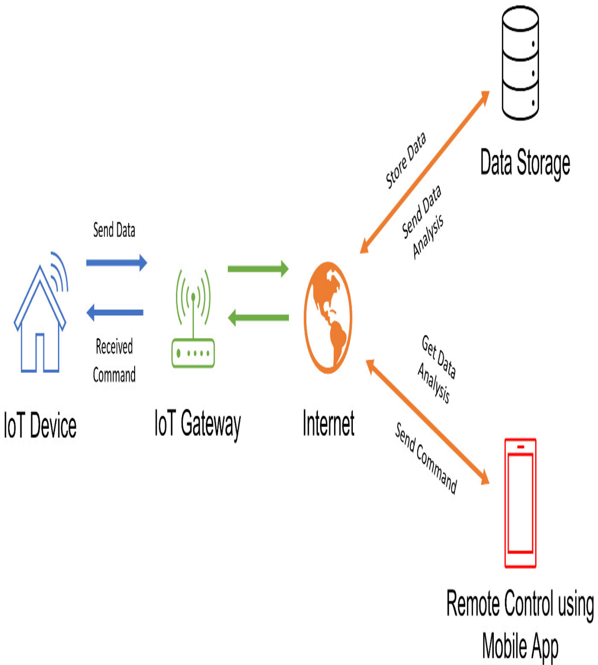
Figure 14.1 – Example of how IoT devices interoperate
