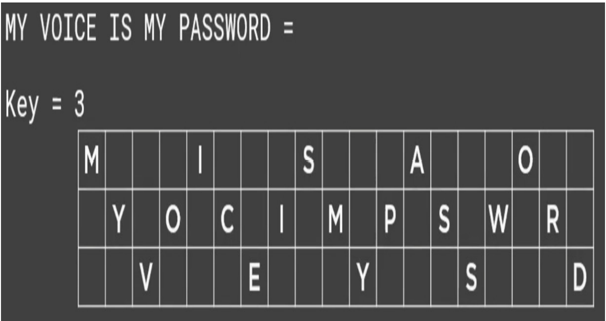
Figure 16.2 – Example of a rail fence cipher
