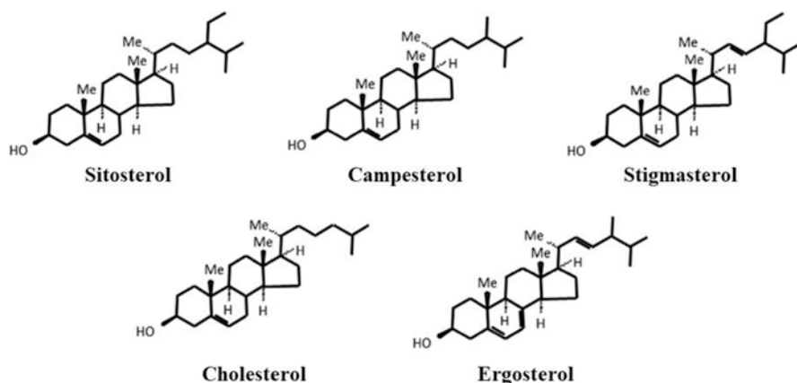
Fig. 2.3 Structural conformation of the main phytosterols (sitosterol, campesterol and stigmasterol), zoosterol (cholesterol) and mycoesterol (ergosterol). Based on (Bot 2019)
