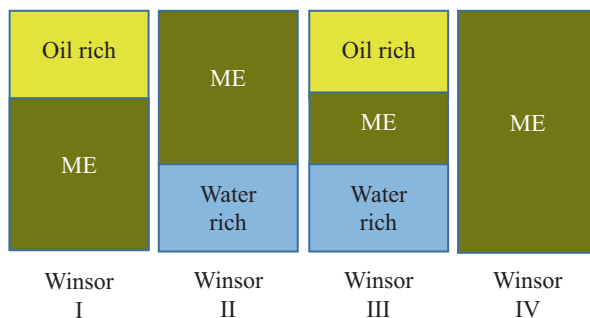
Fig. 12.2 Categorization of Winsor microemulsions
