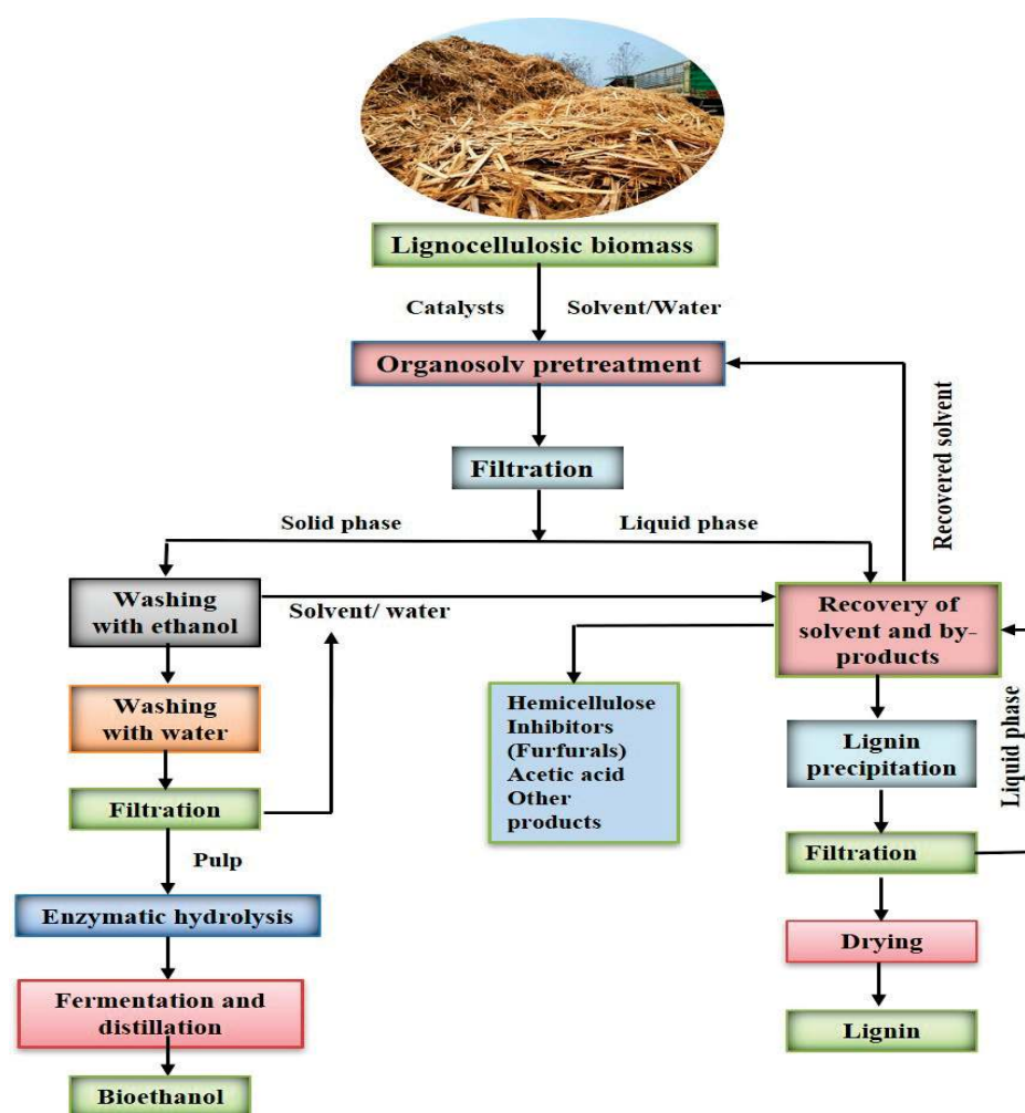
Figure 2. Schematic representation of steps in organosolv pretreatment of lignocellulosic feedstocks.
