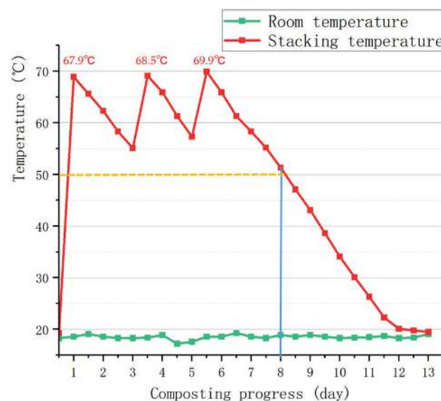
Figure 10. Temperature changes during composting process.
