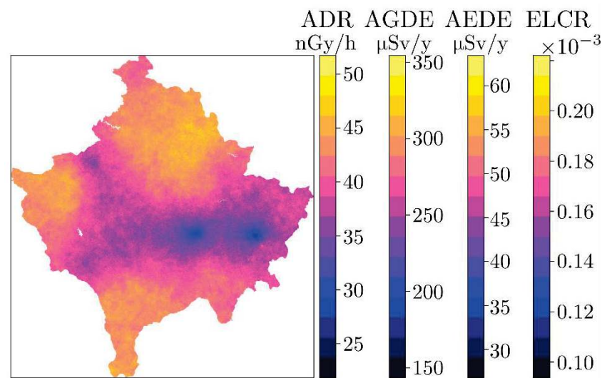
Figure 7. Distributions of radiological health risks and calculated parameters ADR, AGDE, AEDE, and ELCR.
