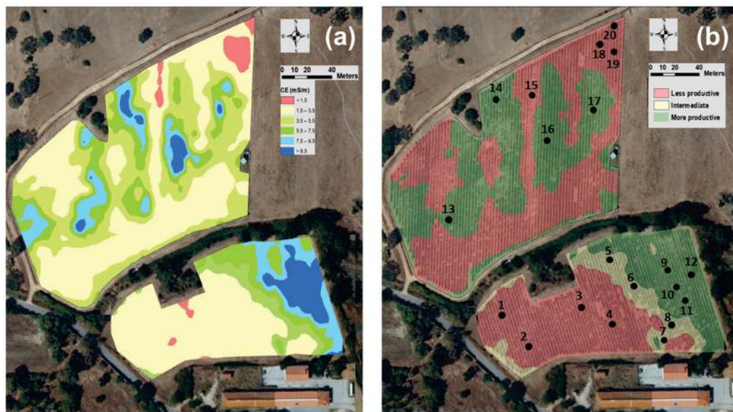
Figure 12. Soil apparent electrical conductivity ( EC_a ; (a)) and management zones (MZ; (b)) maps of white and red grapes fields (location of the twenty sampling points, twelve in white grapes area and eight in red grapes area).
