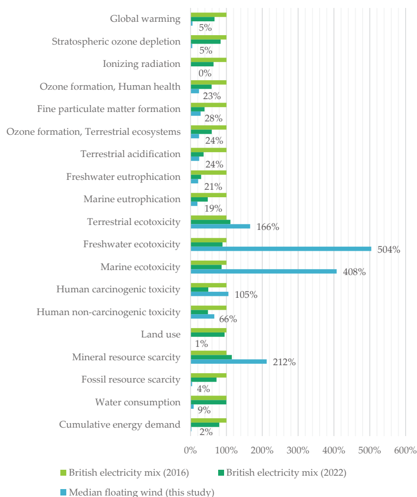
Figure 6. Comparison of the relative environmental performance of the ecoinvent unit process for 2016 British electricity mix [30], a modified process representative of 2022 generation by energy [42,43], and the median results of the four floating wind farms calculated in this study; 100% corresponds to the 2016 electricity mix results.
