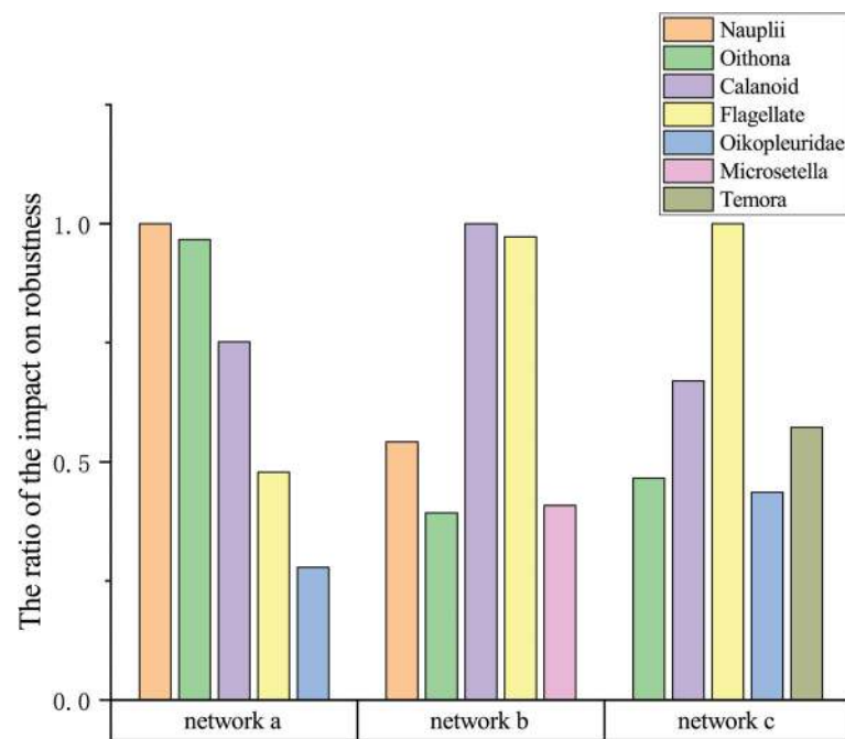
Figure 10. The top five genera of planktonic organisms with significant impacts on network robustness.
