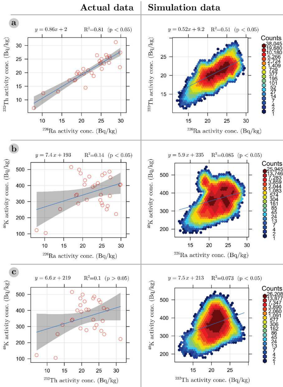
Figure 2. Correlation analysis of natural radioisotopes ( ^{226}\text{Ra} , ^{232}\text{Th} , ^{40}\text{K} ) versus each other for actual and simulation data. (a) Correlation between ^{226}\text{Ra} and ^{232}\text{Th} activity concentration, (b) Correlation between ^{226}\text{Ra} and ^{40}\text{K} activity concentration, (c) Correlation between ^{232}\text{Th} and ^{40}\text{K} activity concentration.
