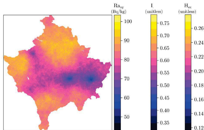
Figure 6. The values of radiological hazard parameters, based on measured and simulated data from the soil.
