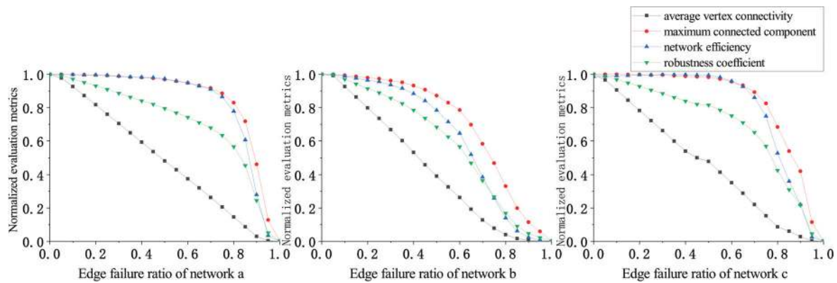
Figure 7. Changes in indicators under random edge attack.
