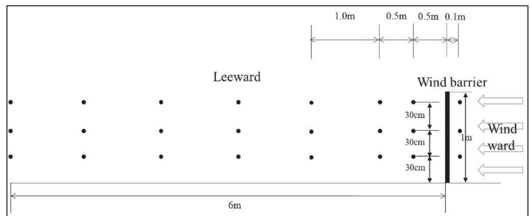
Figure 3. The 3 vertical measuring points in front of wind barriers and 3 vertical measuring points and 7 horizontal measuring points (i.e., 21 measuring points in total) behind wind barriers.
