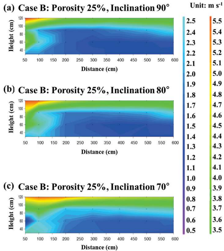
Figure 5. Visualization of the spatial distribution of the average wind velocity according to distance for Case B with a wind barrier porosity of 25% and an inclination of (a) 90°, (b) 80°, and (c) 70°.
