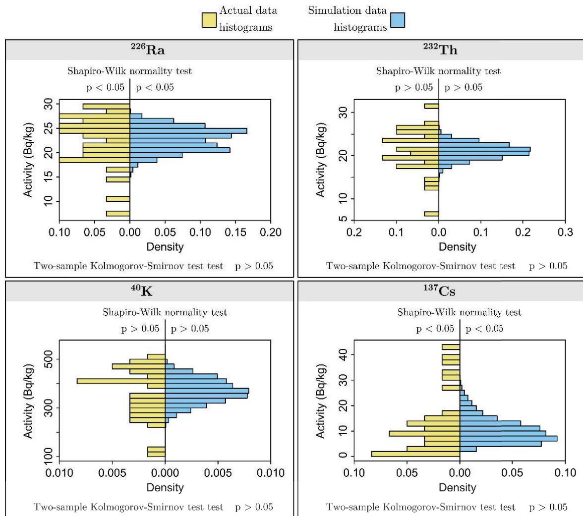
Figure 3. Frequency distributions of ^{226}\text{Ra} , ^{232}\text{Th} , ^{40}\text{K} , and ^{137}\text{Cs} concentrations for actual and simulation data.
