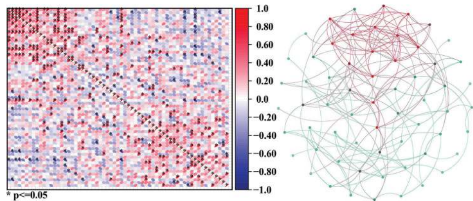
Figure 3. The correlation matrix of community b and the network b constructed based on the matrix.
