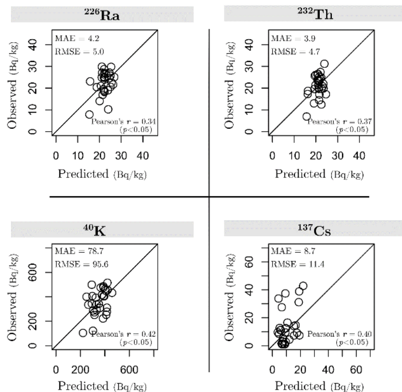
Figure 4. The cross-validation diagrams generated as a result of comparing the predicted values with the observed values for ^{226}\text{Ra} , ^{232}\text{Th} , ^{40}\text{K} , and ^{137}\text{Cs} .
