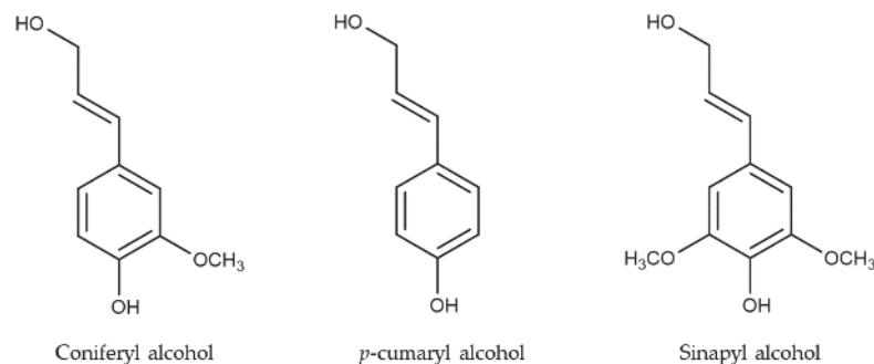
Figure 7. The main precursors of lignin.
