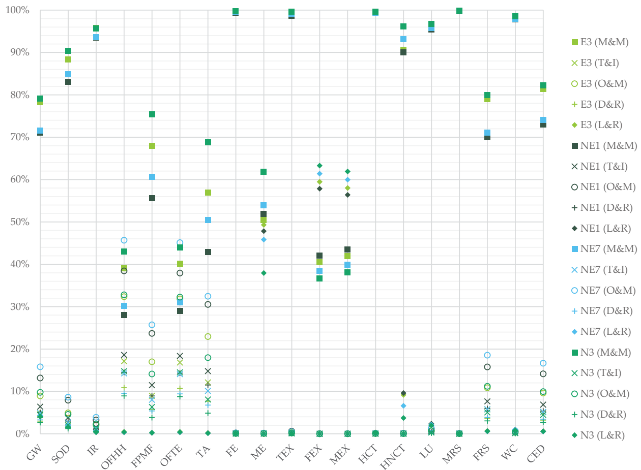
Figure 3. The relative contribution of life cycle stages to environmental impact categories: materials and manufacturing (M&M); transport and installation (T&I); operation and maintenance (O&M); decommissioning and removal (D&R); landfill and recycling (L&R).
