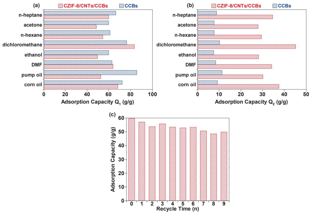
Figure 9. (a) Adsorption capacities Q_1 of CZIF-8/CNTs/CCBs and CCBs for oil or organic solvents. (b) Adsorption capacities Q_2 of CZIF-8/CNTs/CCBs and CCBs for oil or organic solvents. (c) Adsorption capacities of CZIF-8/CNTs/CCBs for n-heptane after 9 cycles.
