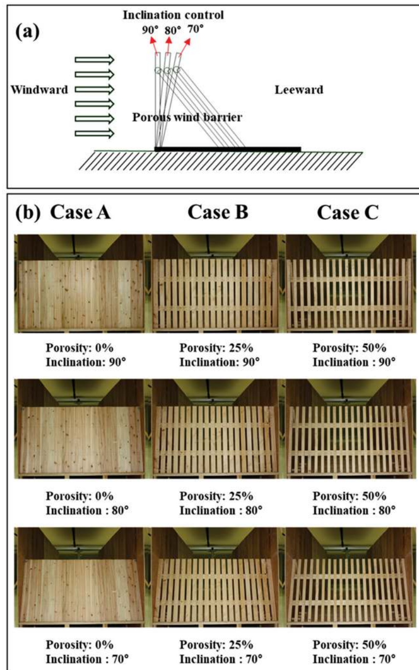
Figure 2. (a) Schematic diagram of porous and non-porous wind barriers at different inclinations and (b) three case studies (A, B, and C) with different porosities (0%, 25%, and 50%) and inclinations ( 90^\circ , 80^\circ , and 70^\circ ).
