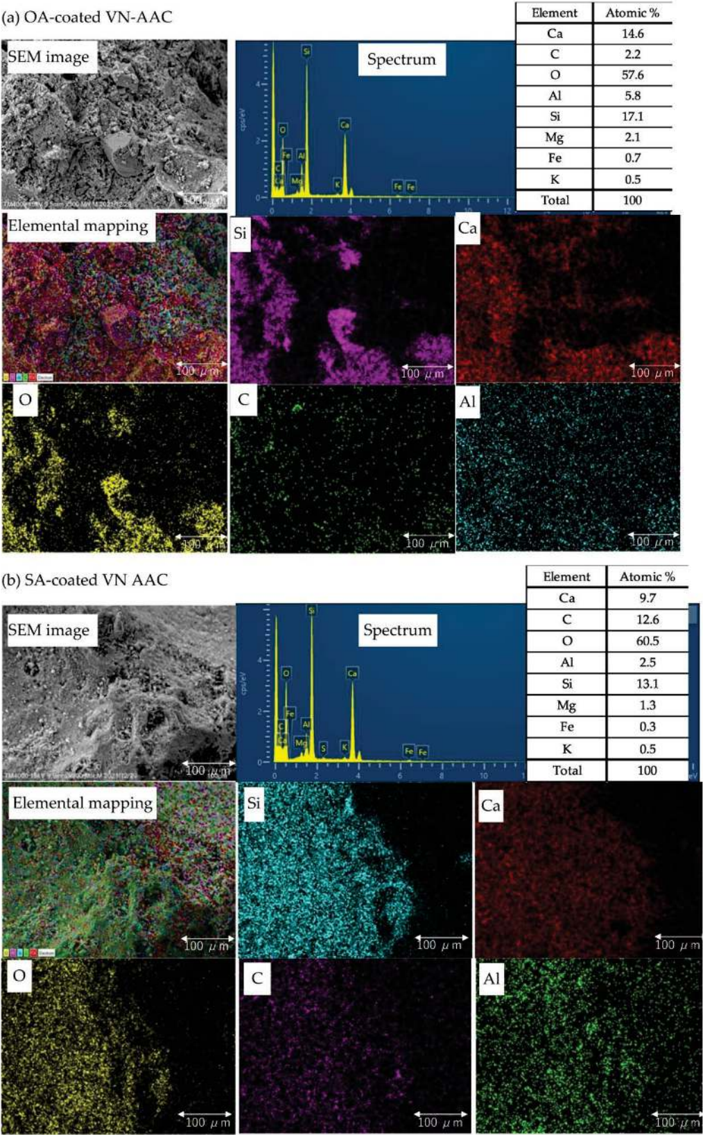
Figure 3. SEM-EDS images of (a) OA-coated VN-AAC grain (0.85–2.00 mm) at HA concentration = 14 g/kg and (b) SA-coated VN-AAC grain (0.85–2.00 mm) at HA concentration = 42 g/kg.
