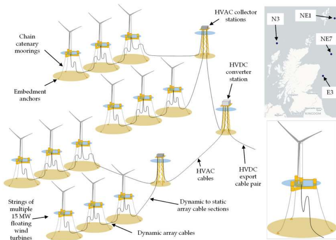
Figure 1. Overview of components included within the floating wind farms' reference flows; map of sites considered and general arrangement of the 15 MW reference wind turbine with platform. Diagrams adapted from [32,33], map adapted from [34]. Sites are labelled North 3, North East 1, North East 7 and East 3 (N3, NE1, NE7 and E3).
