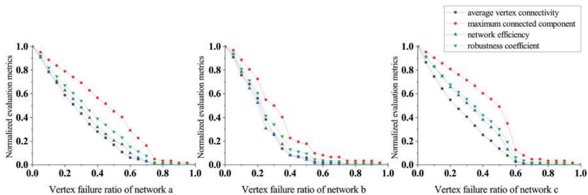
Figure 8. Changes in indicators under vertex betweenness centrality attack.
