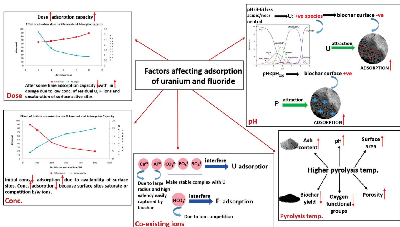
Figure 4. Effect of different parameters on the adsorption capacity and removal efficiency of U and F - , including biochar dose, initial concentration of U and F - , solution pH, pyrolysis temperature, and Co-existing ions.
