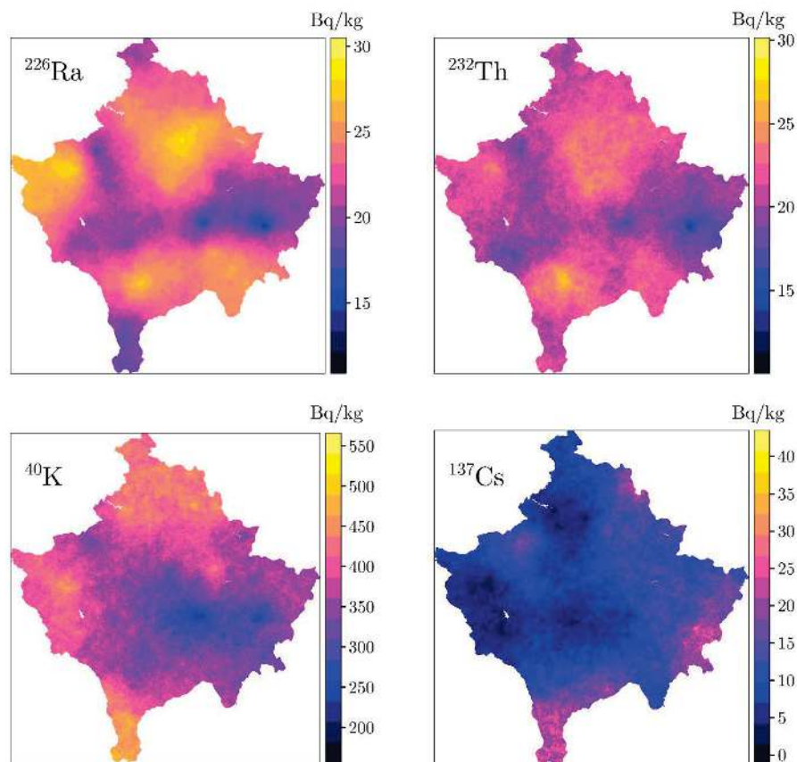
Figure 5. Distributions of radioactivity concentration for ^{226}\text{Ra} , ^{232}\text{Th} , ^{40}\text{K} , and ^{137}\text{Cs} .
