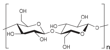
Figure 4. General chemical structure of cellulose.
