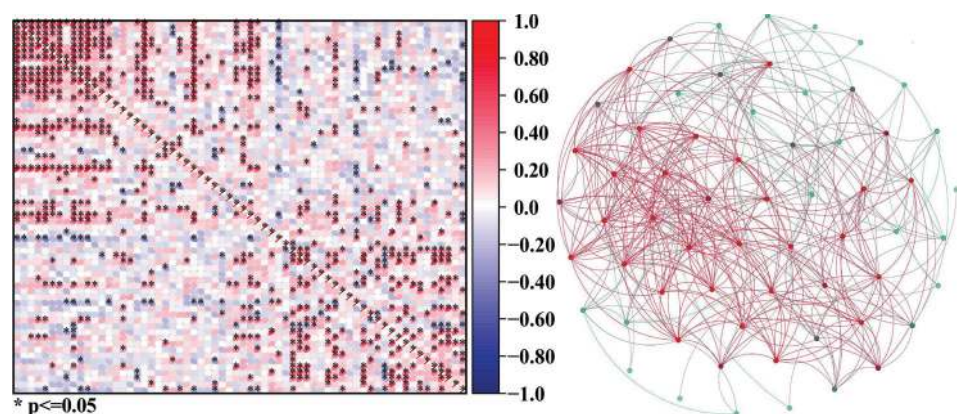
Figure 2. The correlation matrix of community a and its network a constructed based on the matrix; in the correlation matrix, the colors represent the strength of correlation, with * indicating p \leq 0.05 . In the network, the colors represent the tightness of connections, with red vertices having tighter connections than blue vertices.
