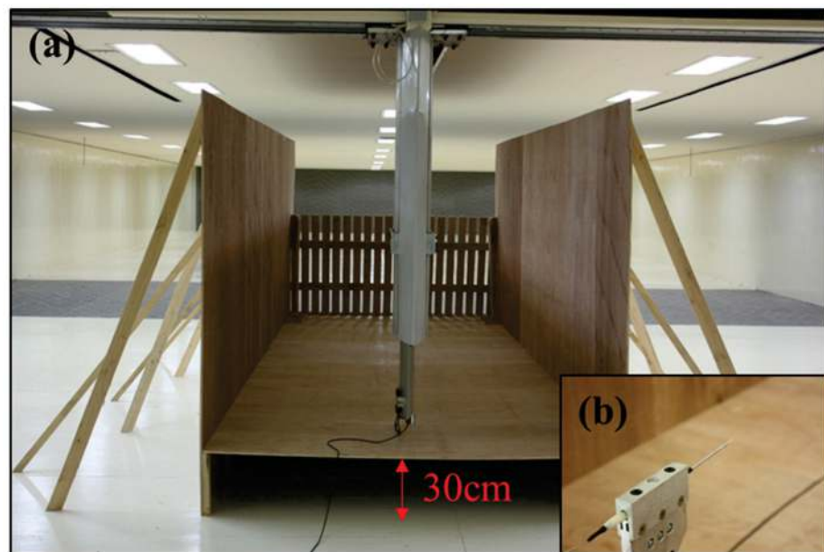
Figure 1. (a) Structure of a small-scale simulation model installed at a 30 cm height from the ground with a wind barrier and (b) a sensor for wind velocity.
