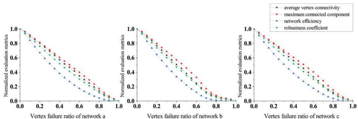
Figure 6. Changes in indicators under random vertex attack.
