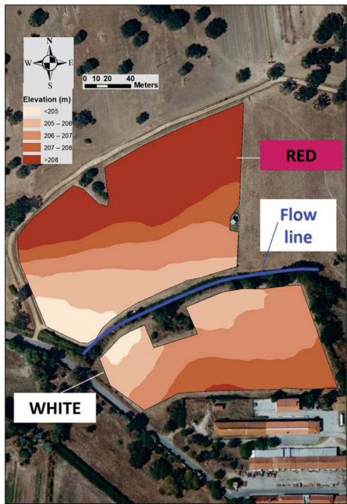
Figure 3. Altimetric map of the experimental field.
