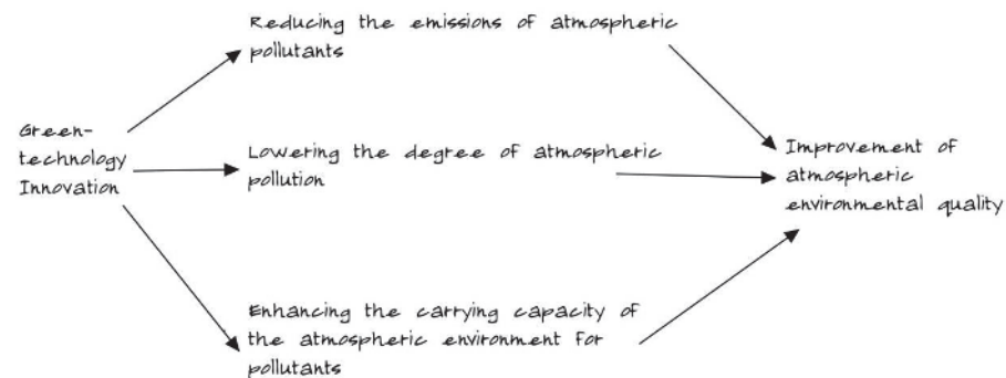
Figure 1. Schematic diagram illustrating the relationship between green technology innovation and air pollution.
