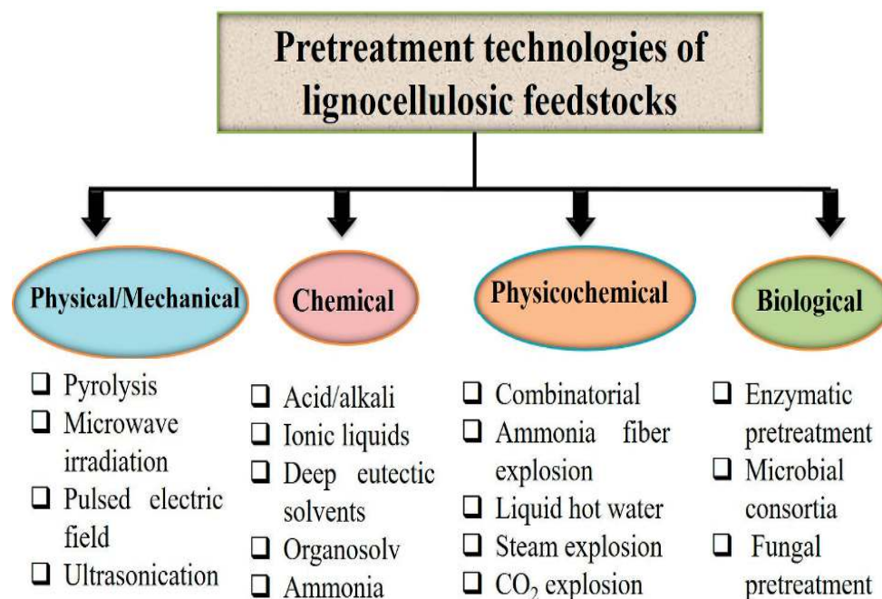
Figure 1. Different pretreatment technologies for breaking the inherent recalcitrant structure of lignocellulosic biomass.
