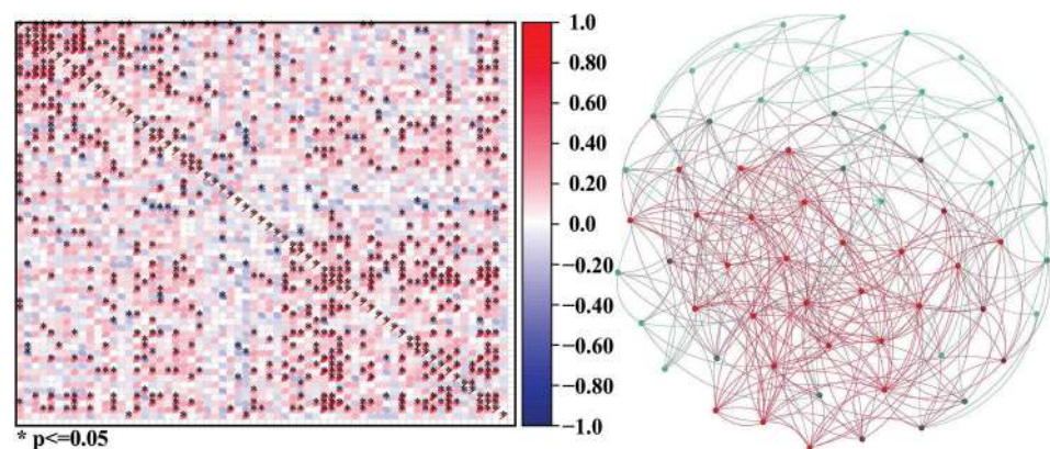
Figure 4. The correlation matrix of community c and the network c constructed based on the matrix.
