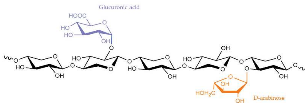
Figure 6. Chemical structure of xylan hemicellulose.
