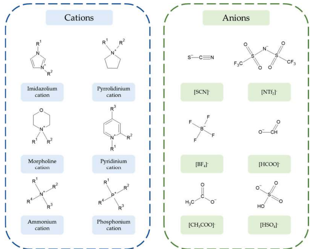
Figure 9. Ionic liquids cations and anions, which are the most frequently applied in biomass transformations (R—hydrogen atom or alkyl group).
