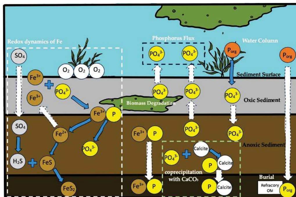
Figure 3. Simplified sediment Fe-P cycling and coprecipitation with \text{CaCO}_3 schematic. Modified from [36].
