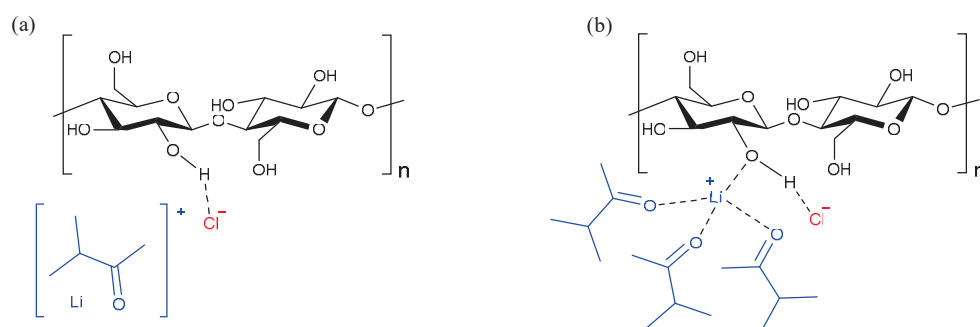
Figure 8. Proposed mechanisms of cellulose dissolving in \text{LiCl}/\text{DMAc} solution: (a) McCormick mechanism, (b) Morgenstern mechanism.
