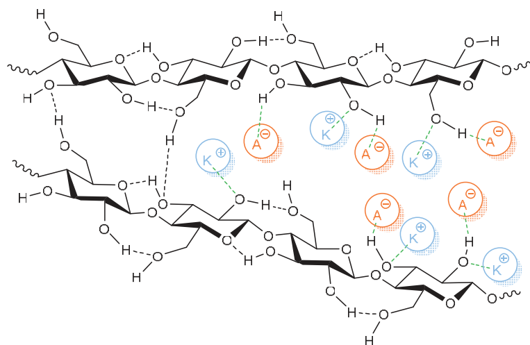
Figure 10. The mechanism of cellulose dissolution in ionic liquid.
