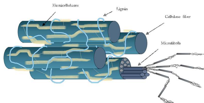
Figure 3. General structure of lignocellulose.
