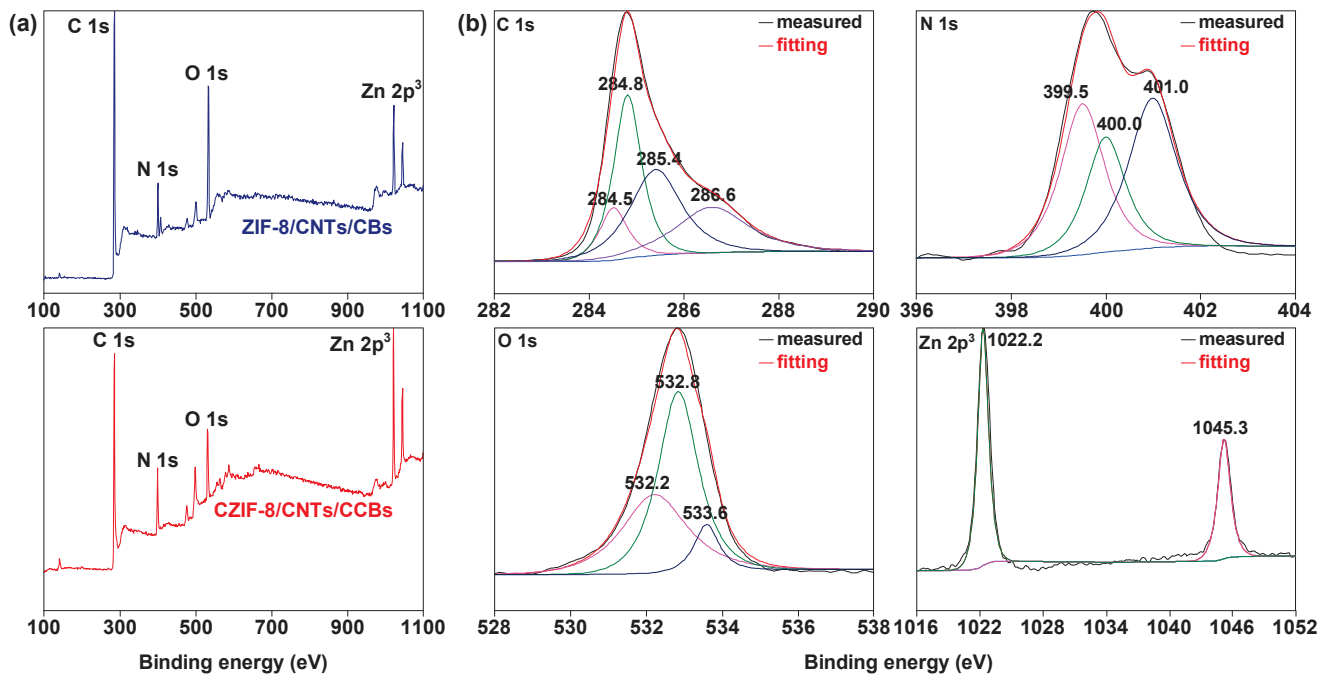
Figure 4. (a) XPS survey spectra of ZIF-8/CNTs/CBs and CZIF-8/CNTs/CCBs. (b) C 1s, N 1s, O 1s, and Zn 2p 3 spectra of ZIF-8/CNTs/CBs.
