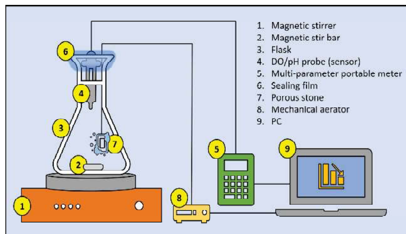
Figure 2. Laboratory respirometric apparatus.
