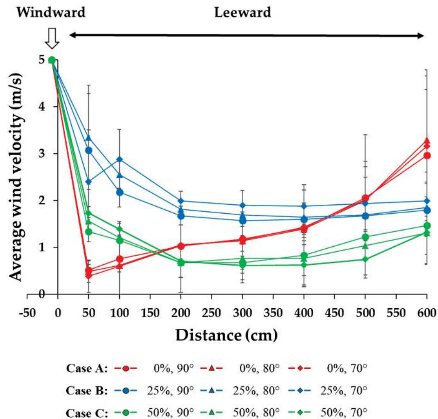
Figure 7. The relationship between average wind velocity (m/s) and distance (cm) on the windward and leeward sides of the wind barriers. The percentages (%) and degrees (°) in the legend represent the porosity and inclination of the wind barriers, respectively. The bars represent the standard deviation.
