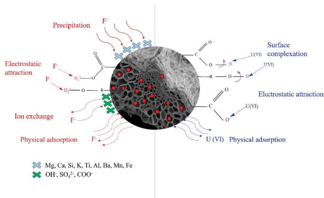
Figure 5. Schematic representation of major mechanisms of U and F - adsorption on biochar surface.
