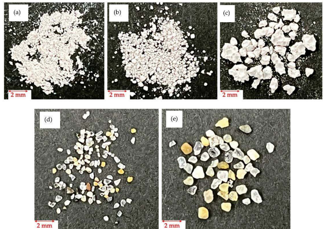
Figure 1. Samples: (a) VN-AAC (Grain size: 0.106–0.25 mm); (b) VN-AAC (Grain size: 0.25–0.85 mm); (c) VN-AAC (Grain size: 0.85–2.00 mm) (d) Sand (Grain size: 0.18–2.00 mm); (e) Sand (Grain size: 0.30–2.00 mm).
