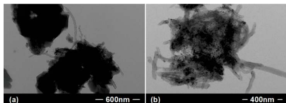
Figure 3. TEM images of ZIF-8/CNTs (a) and CZIF-8/CNTs (b).
