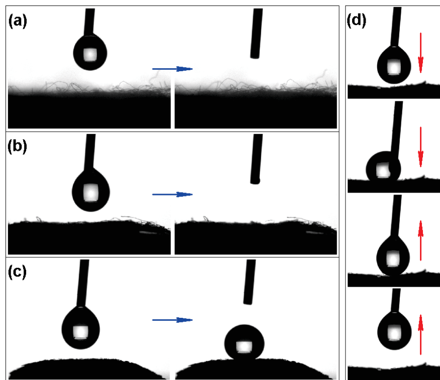
Figure 7. (a–c) The water static contact angle measurement for CCBs, ZIF-8/CNTs/CCBs, and CZIF-8/CNTs/CCBs. (d) Adhesion images of the water droplet on CZIF-8/CNTs/CCBs.
