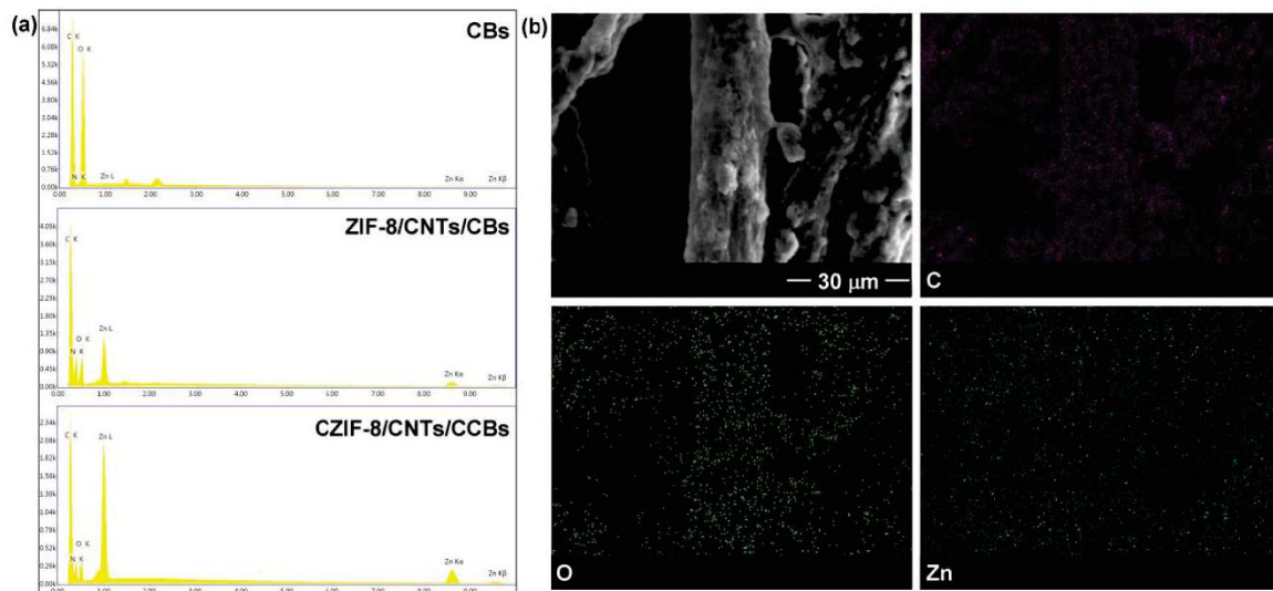
Figure 5. (a) Images of CBs, ZIF-8/CNTs/CBs, and CZIF-8/CNTs/CCBs EDS elemental analysis spectra. (b) Images of CZIF-8/CNTs/CCBs in EDS elemental mappings.
