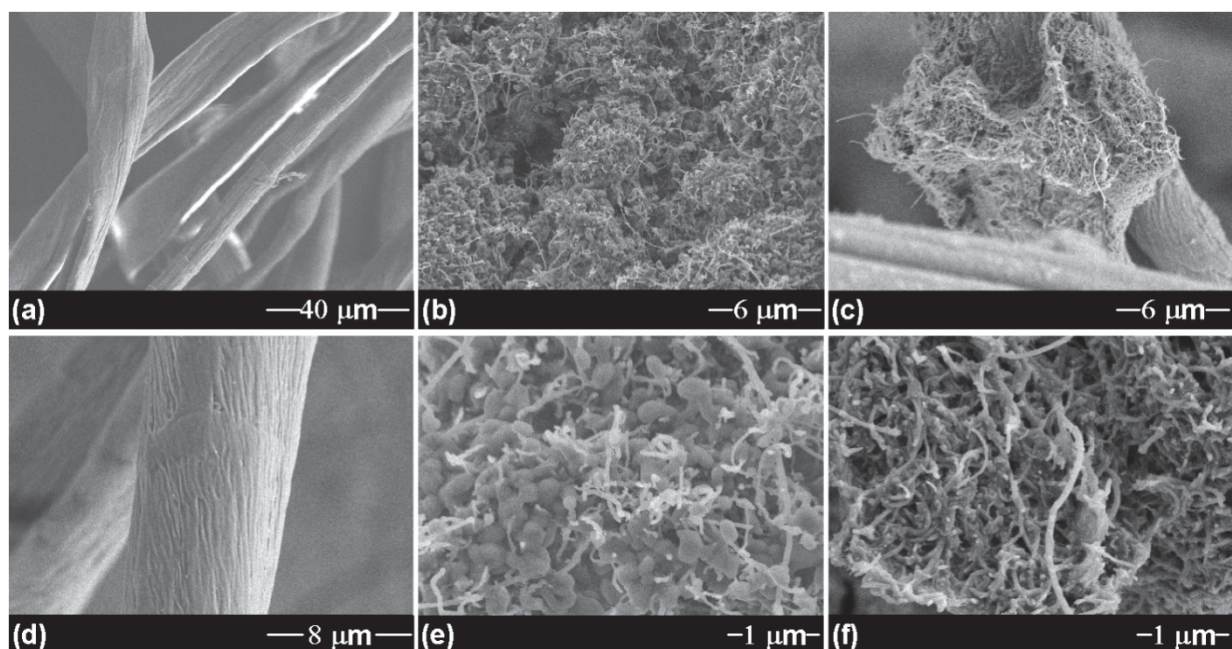
Figure 2. FE-SEM images of CBs (a,d), ZIF-8/CNTs/CBs (b,e), and CZIF-8/CNTs/CCBs (c,f).
