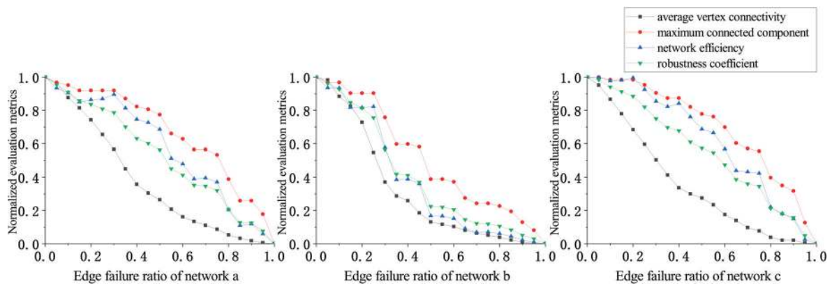
Figure 9. Change in indicators under edge betweenness centrality attack.
