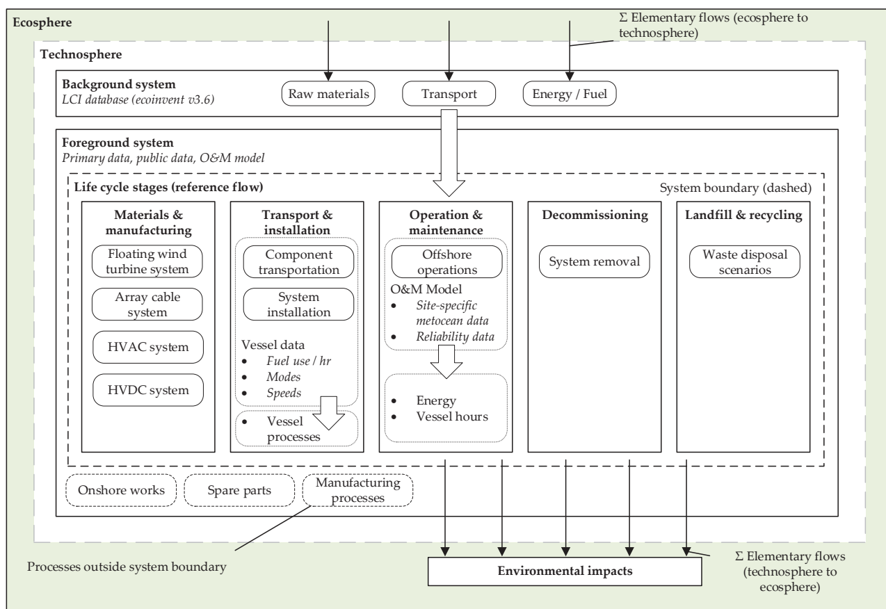
Figure 2. Schematic of the life cycle model, system boundary, life cycle stages, inventory assemblies, and processes, and the relationship with the COMPASS O&M model. White arrows indicate flows of data within the model, black arrows indicate elementary flows in the LCI.
