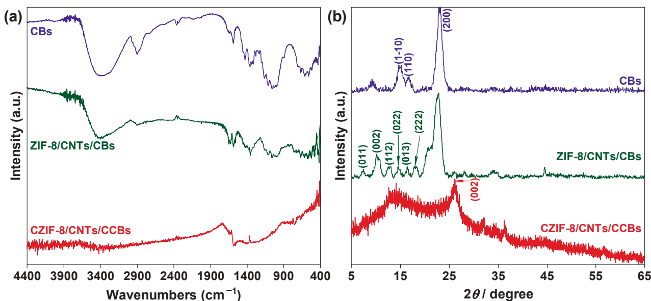
Figure 6. (a) FTIR spectra of CBs, ZIF-8/CNTs/CBs, and CZIF-8/CNTs/CCBs. (b) XRD patterns for CBs, ZIF-8/CNTs/CBs, and CZIF-8/CNTs/CCBs.
