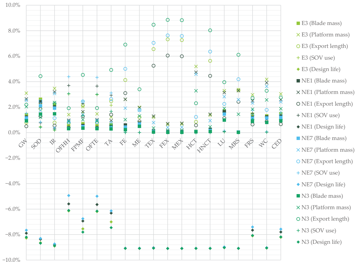
Figure 4. Sensitivity of impact categories to 10% increase in selected site and engineering design parameters for all four sites.
