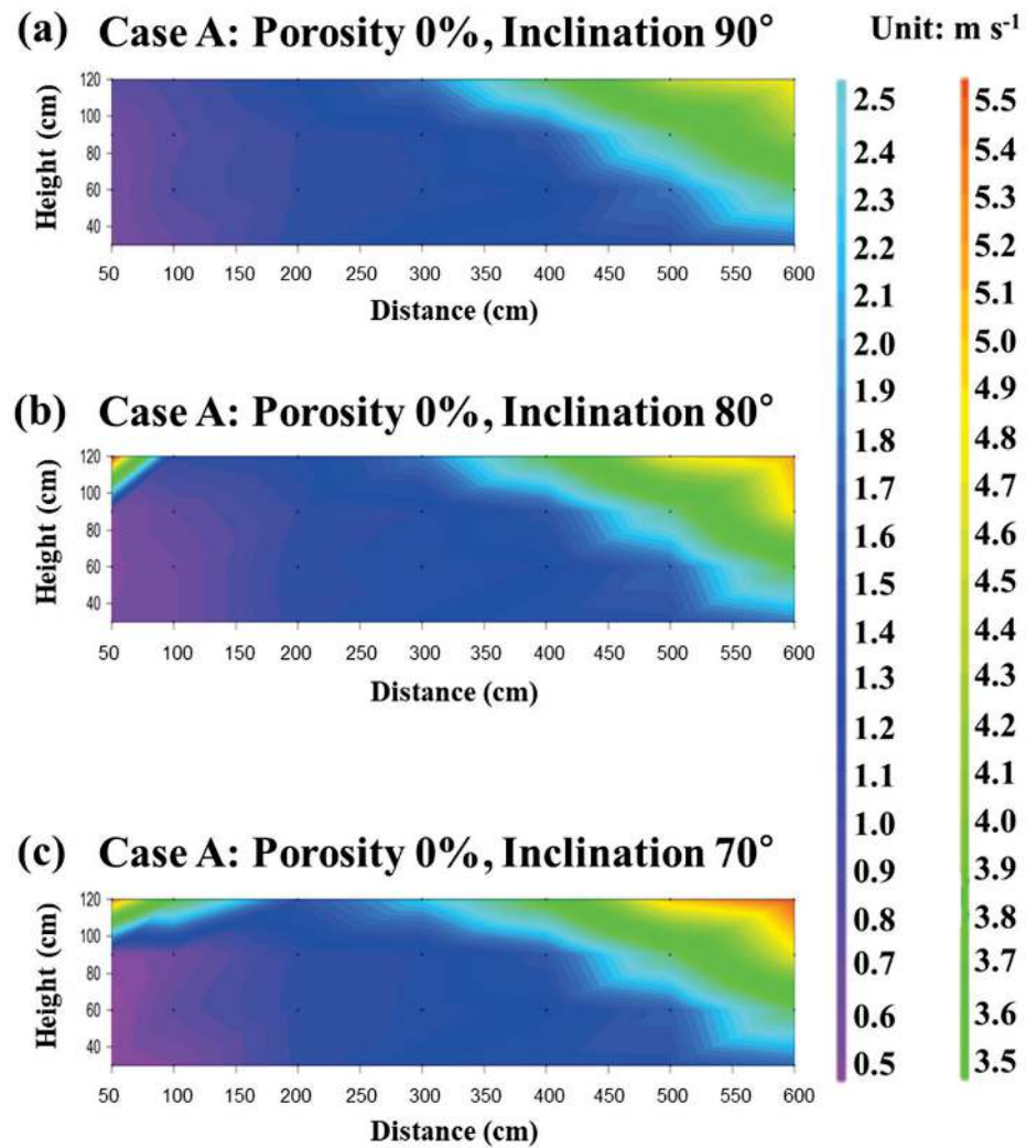
Figure 4. Visualization of the spatial distribution of the average wind velocity according to distance for Case A with a wind barrier porosity of 0% and an inclination of (a) 90°, (b) 80°, and (c) 70°.
