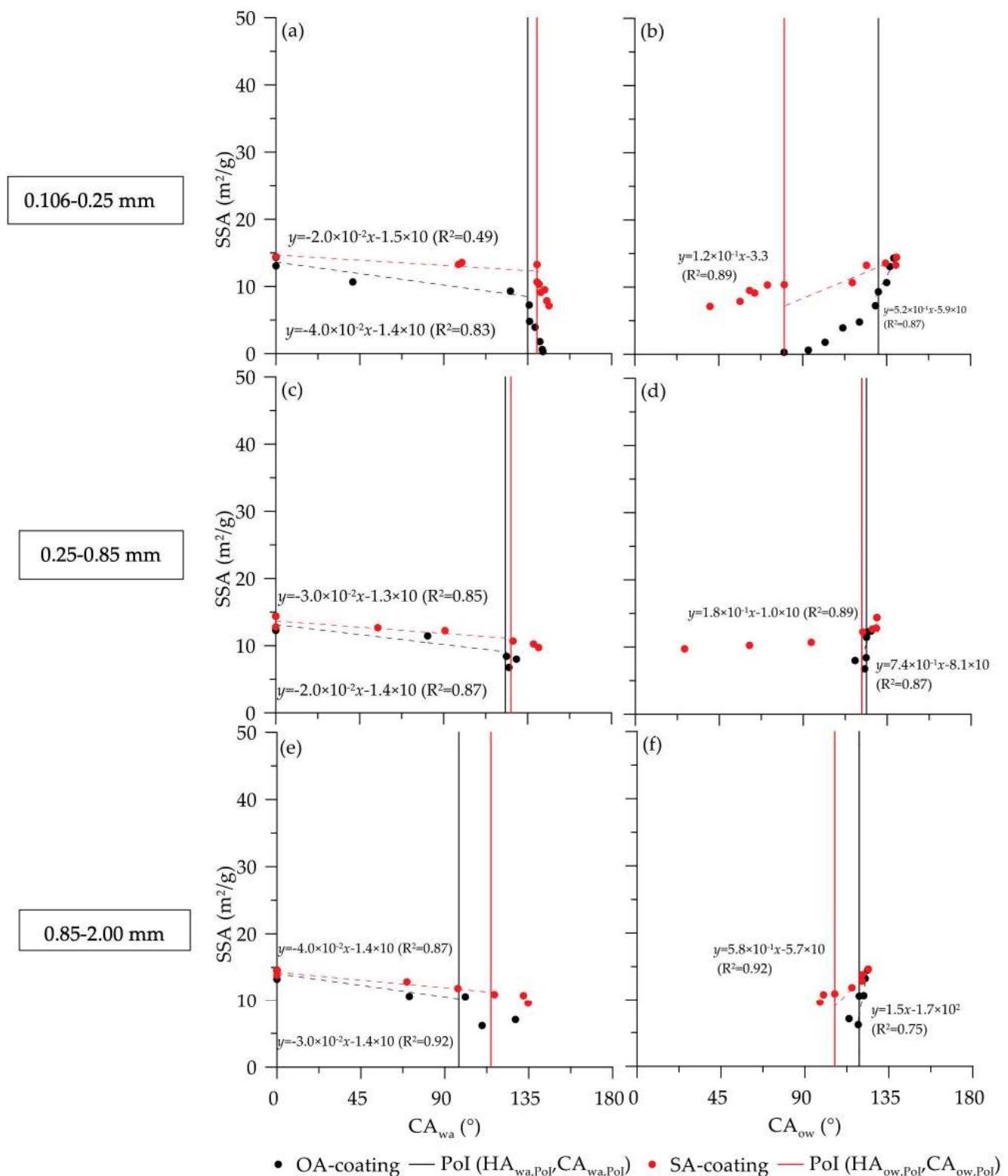
Figure 6. Relationships between SSA and CA wa /CA ow for OA- and SA-coated VN-AAC grains. OA-coated VN-AAC grain: (a,b) Grain size = 0.106–0.25 mm, (c,d) Grain size = 0.25–0.85 mm, and (e,f) Grain size = 0.85–2.00 mm.
