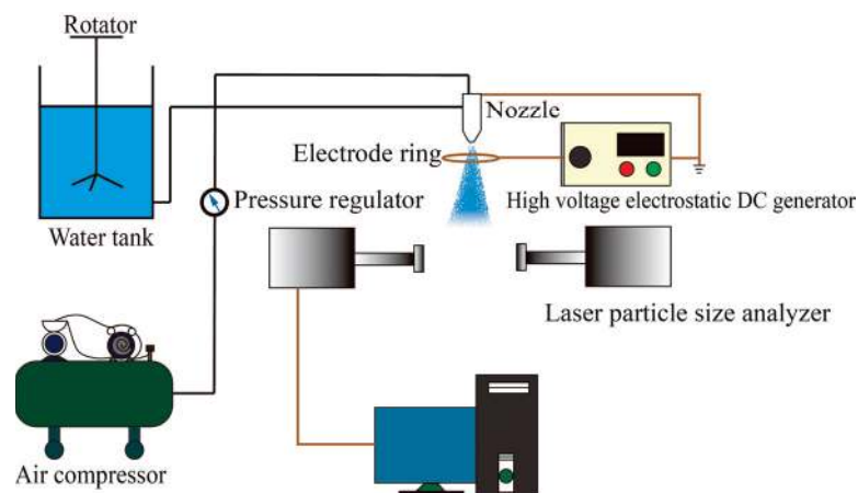
Figure 1. Schematic diagram of the experimental device.
