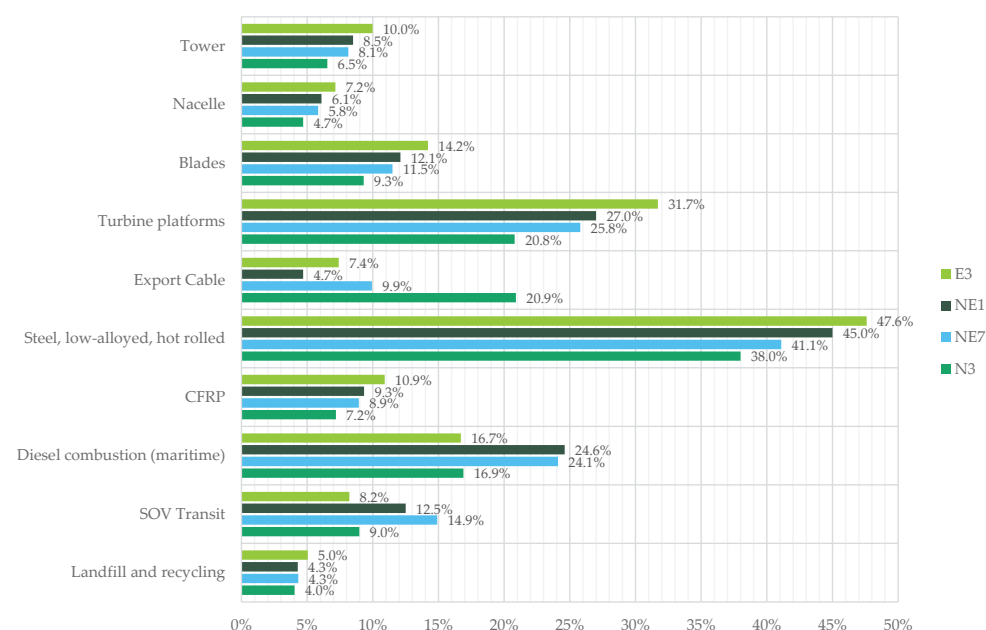
Figure 5. Main contributions to global warming by assemblies, processes, and vessel operations for all four sites.
