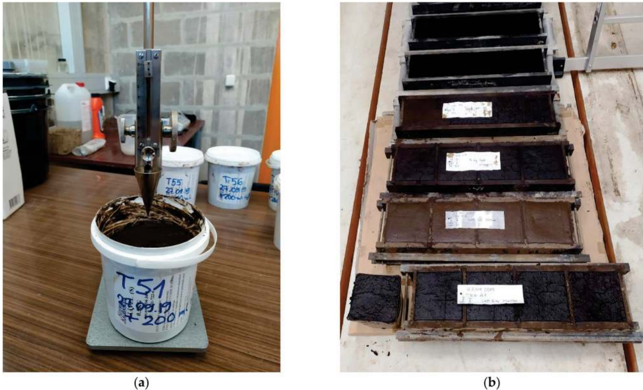
Figure 1. (a) Preliminary testing of the hardening of the specimens with the cone apparatus; (b) test specimens placed in containers.
