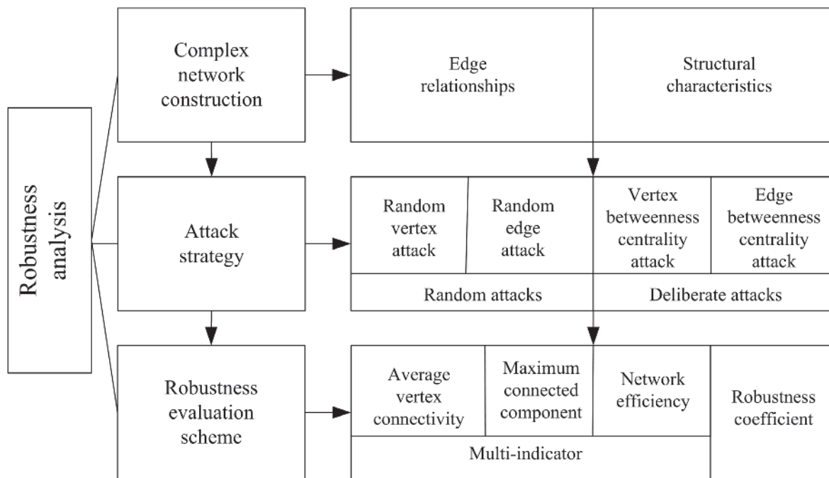
Figure 1. The approach to robustness analysis described in this paper consists of three essential components. First, the construction of a complex network relies on derived edge relationships. Second, attack strategies include two types of attacks, namely, random and deliberate. Finally, a robustness assessment scheme is derived from multi-indicator weighting.
