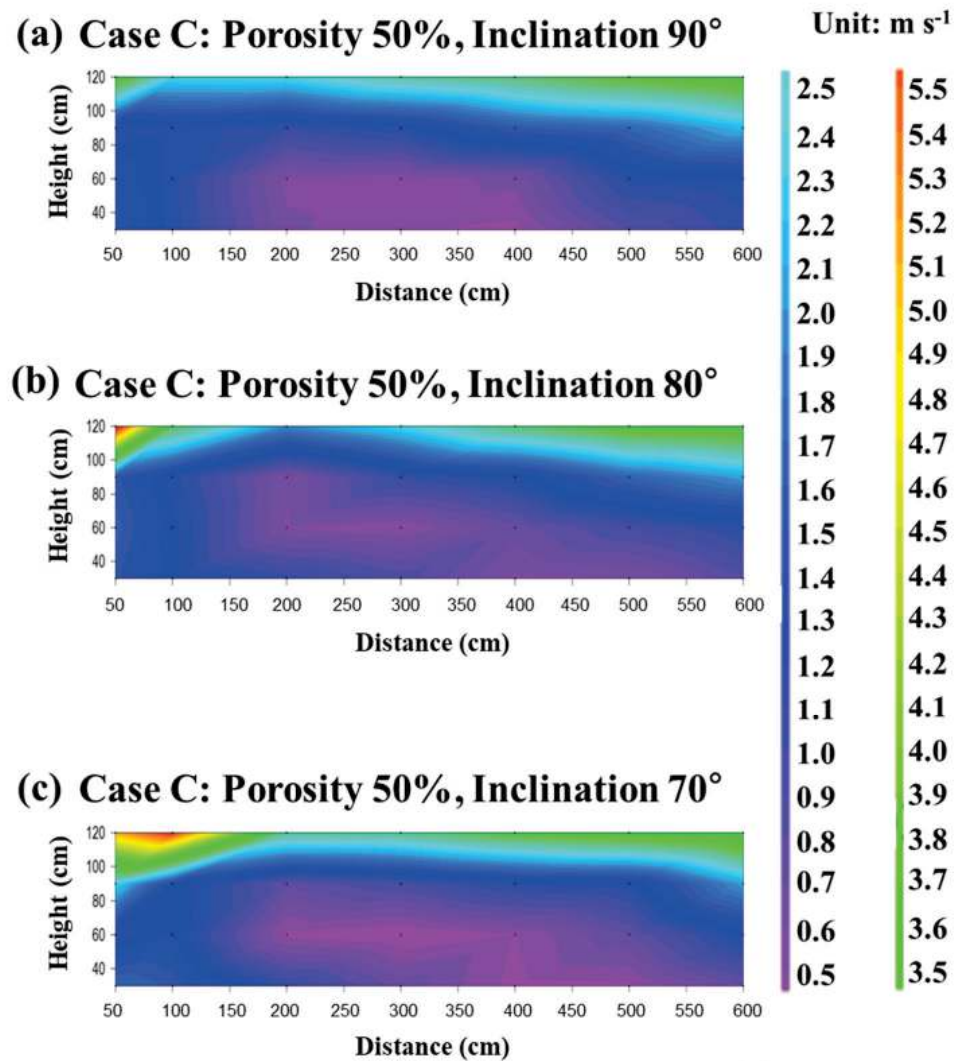
Figure 6. Visualization of the spatial distribution of the average wind velocity according to distance for Case C with a wind barrier porosity of 50% and an inclination of (a) 90°, (b) 80°, and (c) 70°.
