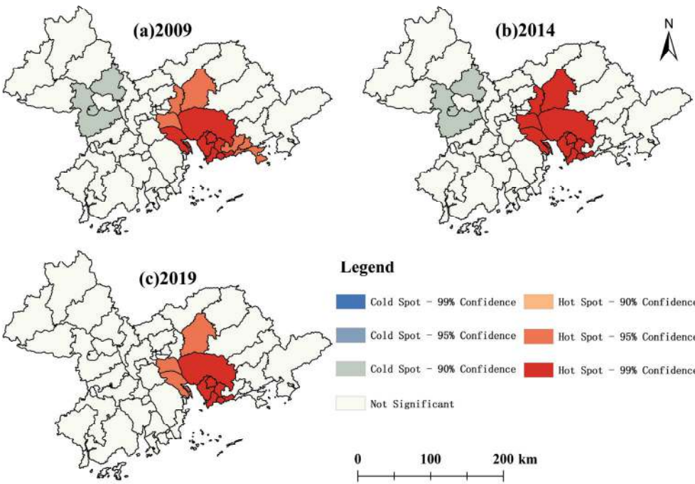
Figure 5. Pearl River Delta cold and hot spots in 2009–2019.
