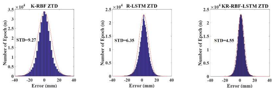
Figure 10. Error distribution of prediction results of K-RBF, R-LSTM, and KR-RBF-STLM models.
