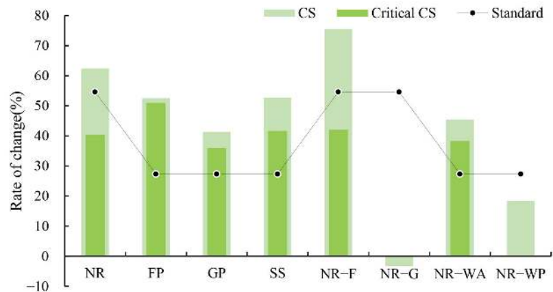
Figure 7. Rate of change in carbon sequestration and critical carbon sequestration by different PAs types from 2000 to 2020.
