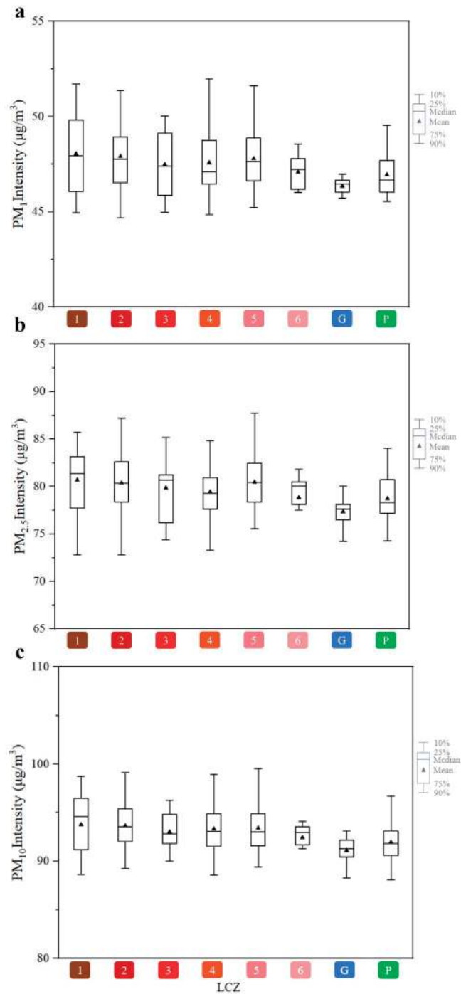
Figure 9. Statistical map particulate matter concentration under different LCZ land use classifications: (a) Statistical maps of \text{PM}_{10} concentrations under different LCZ land use classifications; (b) Statistical Map of \text{PM}_{2.5} Concentration under Different LCZ Land Use Classification; (c) Statistical maps of \text{PM}_{10} concentrations under different LCZ land use classifications.
