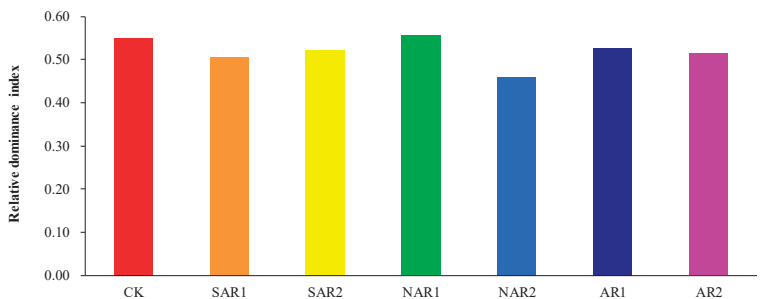
Figure 3. The relative dominance index of Amaranthus spinosus in mixed culture under acid deposition with different sulfur–nitrogen ratios. The value of the relative dominance index ranges from 0 to 1, and it means strong growth performance when the value of this index is higher than 0.5, while poor growth performance when the value of this index is less than 0.5. Abbreviations have the same meanings as presented in Figure 1.
