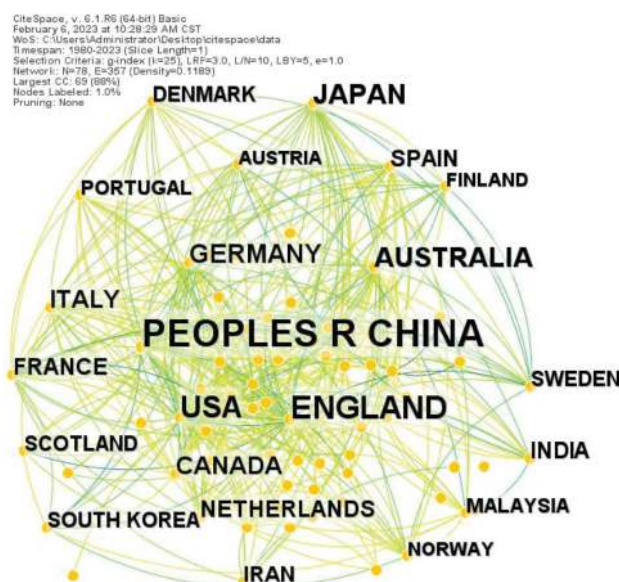
Figure 5. The geographical distribution and co-citation network for the study of low-carbon transition and public awareness/behavior. Note: the size of the label font in the figure represents the number of published documents, and the link between nodes represents the cooperative relationship between countries/regions.
