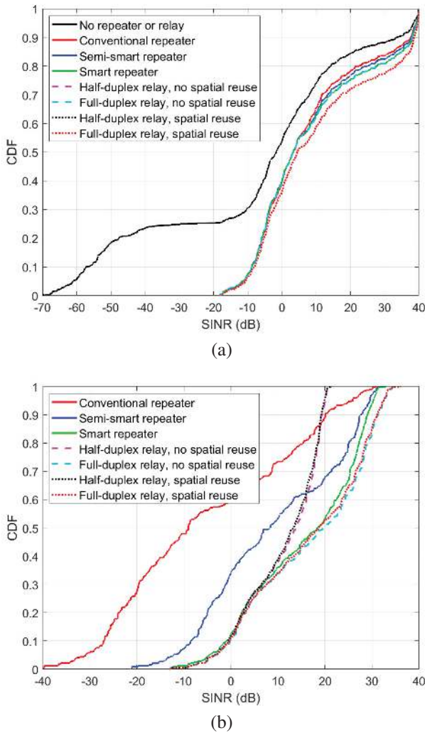
Figure 5.7 SINR CDFs for all UEs under different relaying methods: (a) Indirect UEs and (b) direct UEs.
