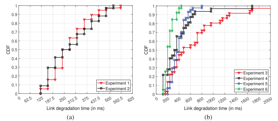
Figure 2.11 CDF of link degradation time for (a) hand blockage and (b) body blockage studies.
