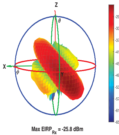
Figure 2.6 Beam patterns of the boresight beam with a 4 \times 1 microstrip patch array in freespace.
