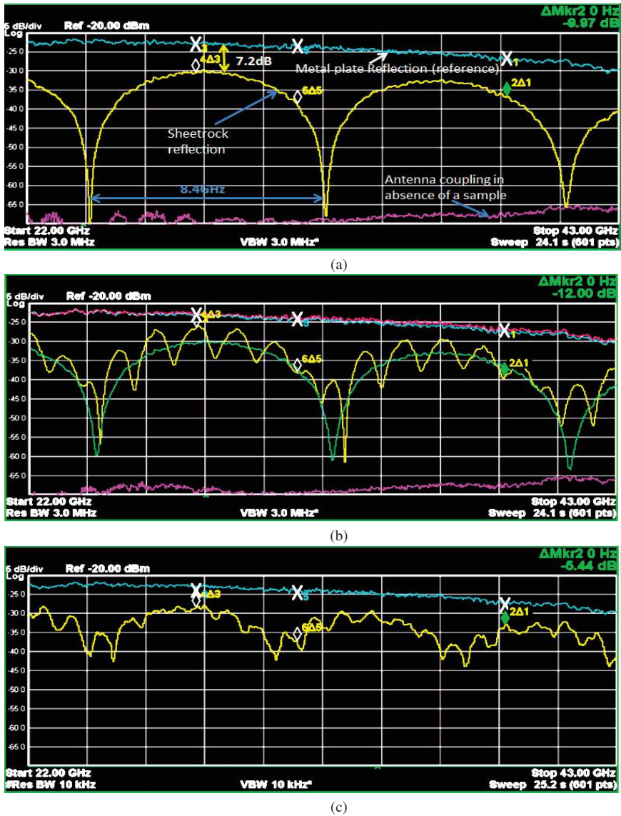
Figure 2.4 Material measurements illustrating reflection response over (a) sheetrock using perpendicular polarization. Response with (b) a structured partition wall and (c) an external wall in the Qualcomm Technologies building.
