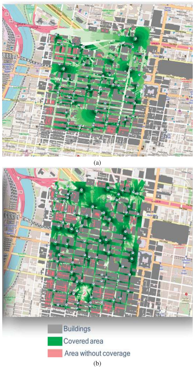
Figure 5.15 SNR coverage map when foliage (a) is not accounted for and (b) is accounted for. Map data from OpenStreetMap with license agreement covering this usage available at https://www.openstreetmap.org/copyright .
