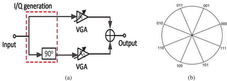
Figure 3.25 (a) Block diagram of a vector modulator phase shifter. (b) Phase selection diagram as a function of digital gain selection input bits.
