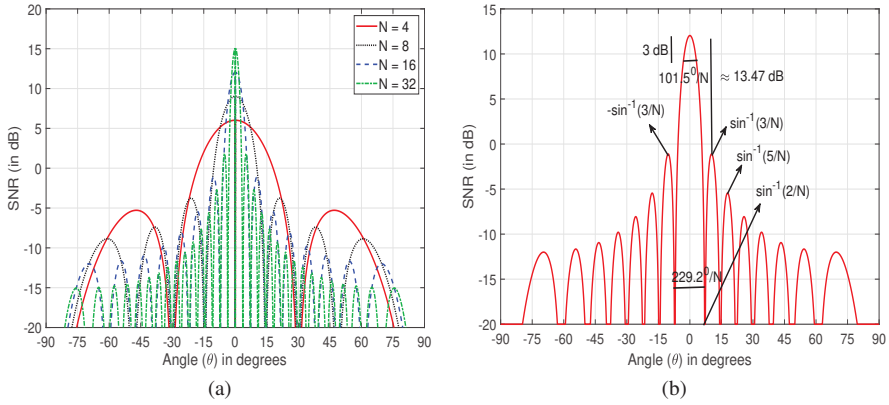
Figure 4.6 (a) \text{SNR}(\theta) vs. \theta for different N and d = \lambda/2 . (b) Beam properties with a beam implementing progressive phase shifts for N = 16 .
