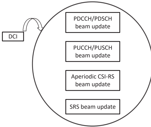
Figure 5.23 Beam management as seen in Rel. 17 where the DCI updates the beams for multiple downlink/uplink channels/RSSs.
