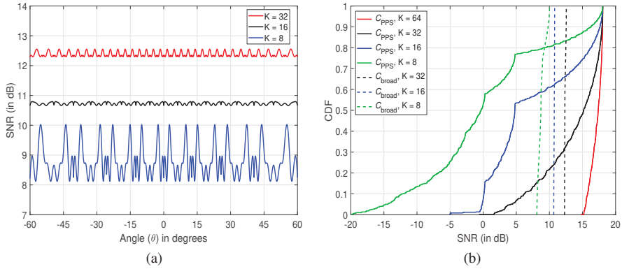
Figure 4.9 (a) \text{SNR}(\theta) vs. \theta for different broad beam codebooks with N = 64 . (b) CDF of \text{SNR}(\theta) over the coverage region with different codebooks with N = 64 .
