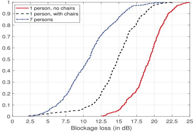
Figure 2.9 CDF of blockage loss in a stadium emulation.
