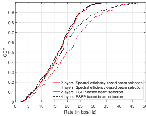
Figure 4.24 Comparison of rate CDFs with two and four layers schemes using a CDL-A channel structure.
