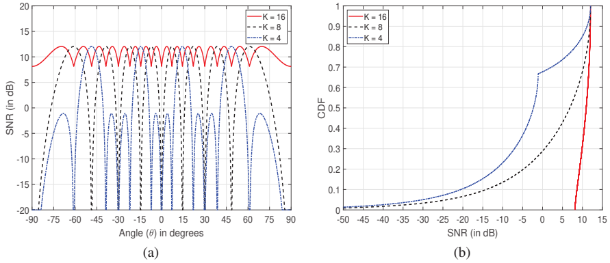
Figure 4.7 (a) \text{SNR}(\theta) vs. \theta for different progressive phase shift codebook sizes with N = 16 . (b) CDF of \text{SNR}(\theta) over \theta for different codebook sizes with N = 16 .
