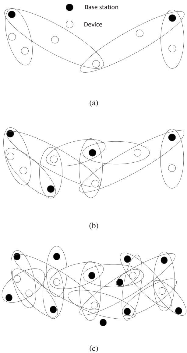
Figure 5.2 Illustration of three levels of network densification: (a) Normal density deployment. (b) Dense deployment. (c) Ultra dense deployment. Each ellipse corresponds to a directional link between the two nodes.
