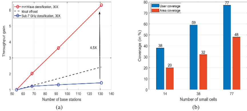
Figure 5.18 (a) Median throughput scaling as a function of the number of base stations. (b) User concentration in hotspots makes mmWave deployment valuable.
