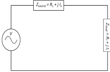
Figure 3.1 Circuit representation of an antenna with a source and a load.
