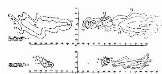
FIG. 7—Contours of constant intensity at 160 MHz and 480 MHz, taken at Wheaton, Illinois.
