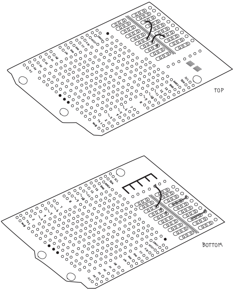
Figure 8-26. Connecting the negative screw terminals
