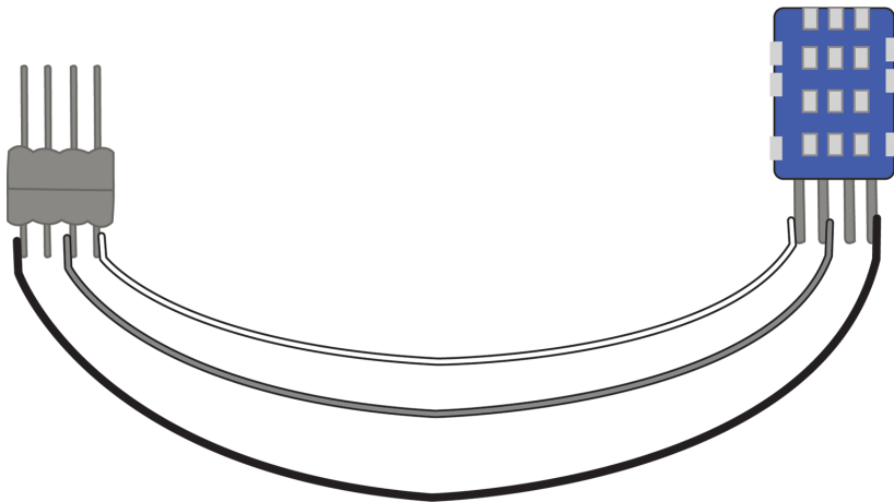
Figure 8-31. Adding long stranded wires and a male header to the DHT11 sensor
