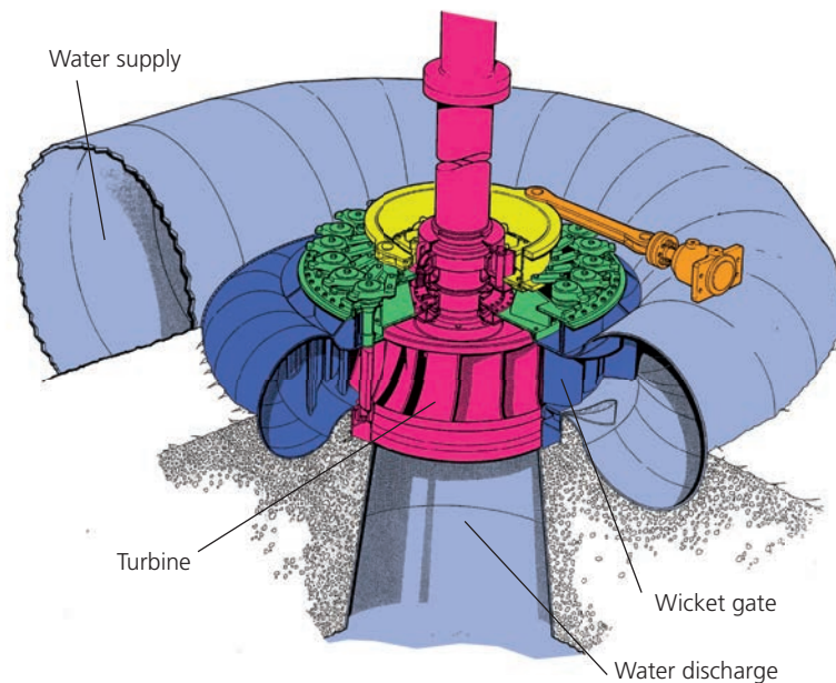
▲ Figure 1.45 Francis wheel turbine
