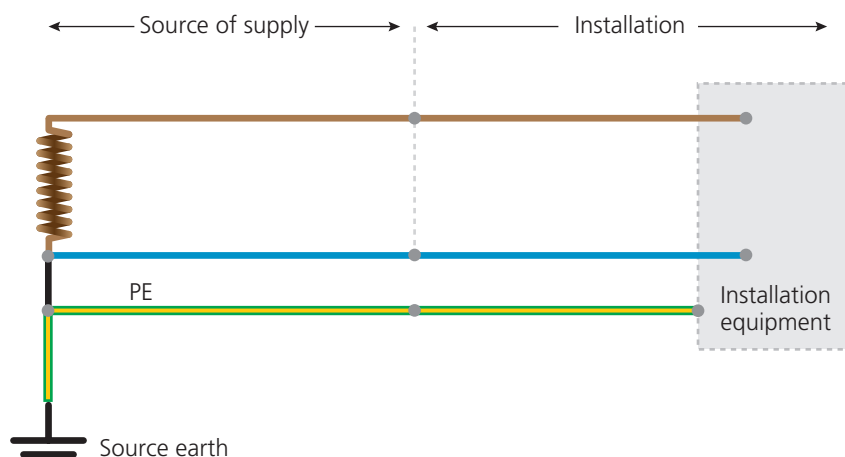
▲ Figure 2.7 Single-phase AC supply
