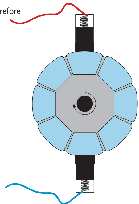
▲ Figure 2.68 A segmented commutator with carbon brushes making contact. This commutator would have four loops wound around the armature.
