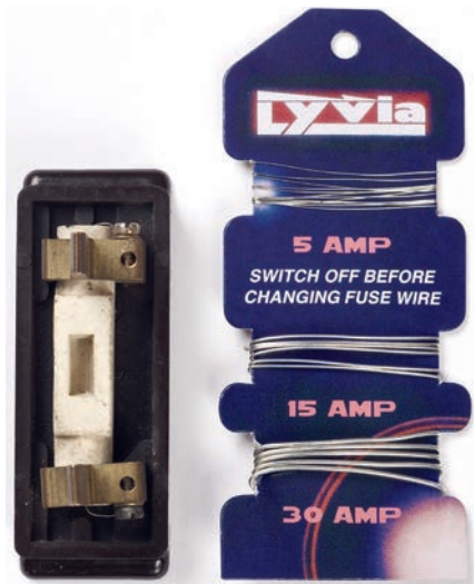
▲ Figure 2.88 Rewirable fuse and fuse wire card showing how wrong wire can easily be used
