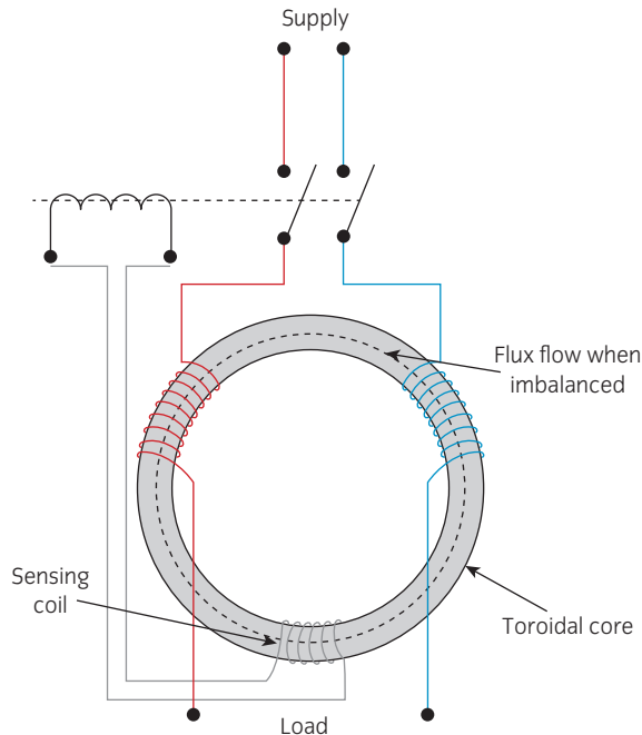
▲ Figure 2.91 Internal circuit diagram for an RCD
