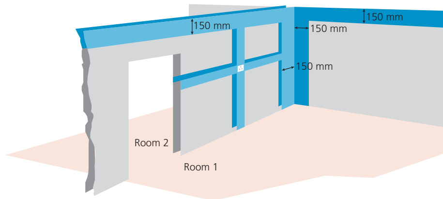
▲ Figure 3.19 Prescribed zones of protection
