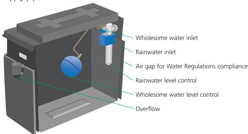
▲ Figure 1.52 Header tank with backflow protection
