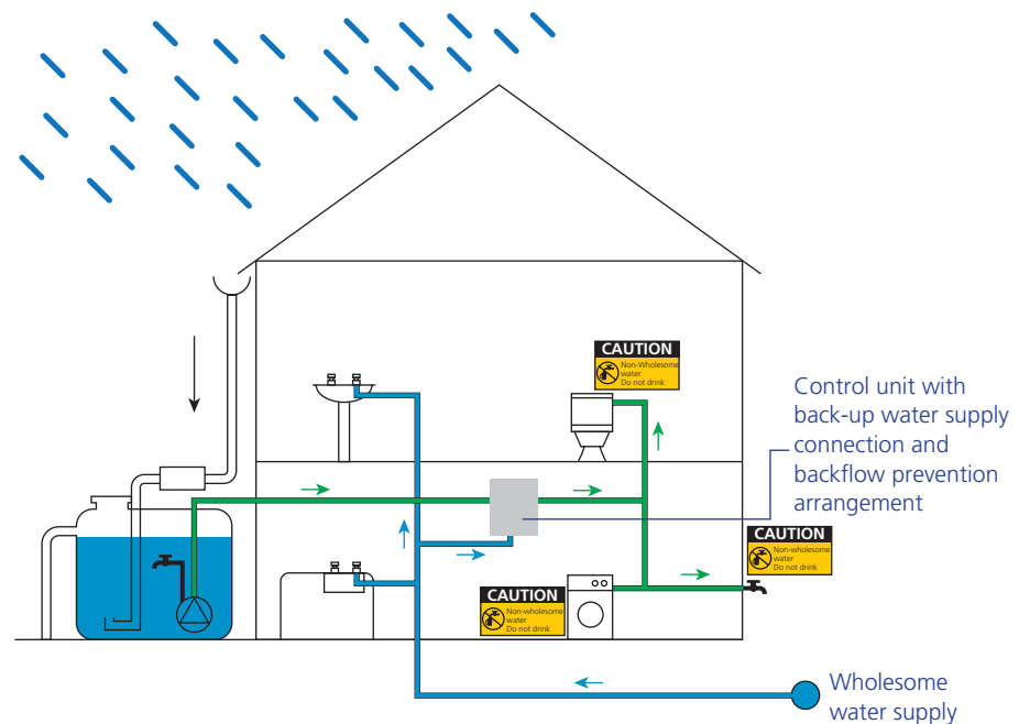
▲ Figure 1.53 Rainwater-harvesting pipework
