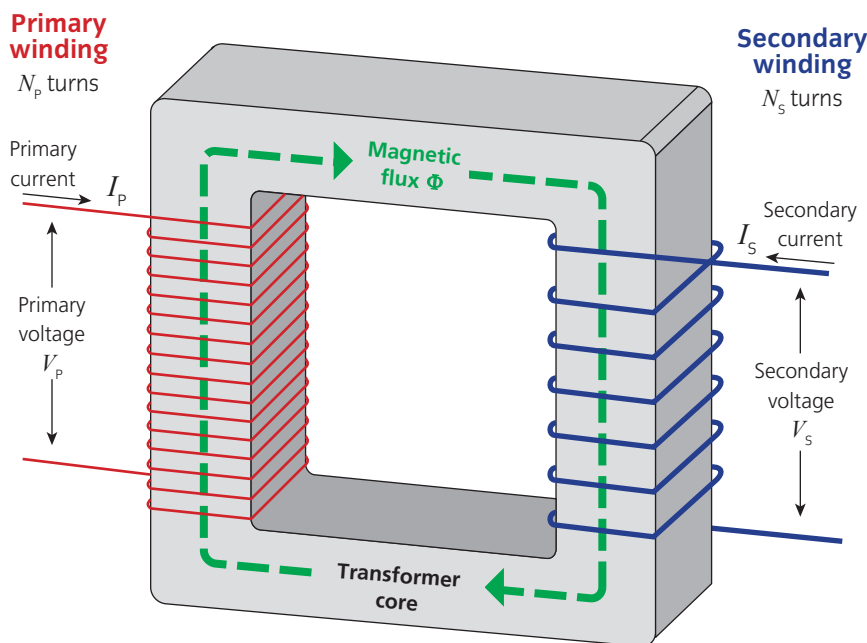
▲ Figure 2.18 Simple transformer arrangement
