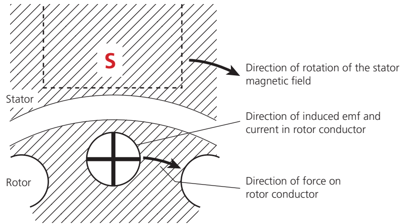
▲ Figure 2.77 Induction motor principles
