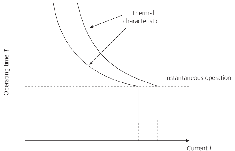
▲ Figure 3.21 Circuit-breaker characteristics
