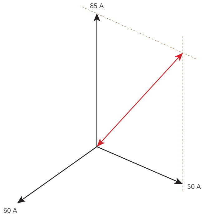
▲ Figure 2.60 Step 2 Construct a parallelogram with two of the phases and draw a line from the centre point of the phasor to the point where the two new lines meet
