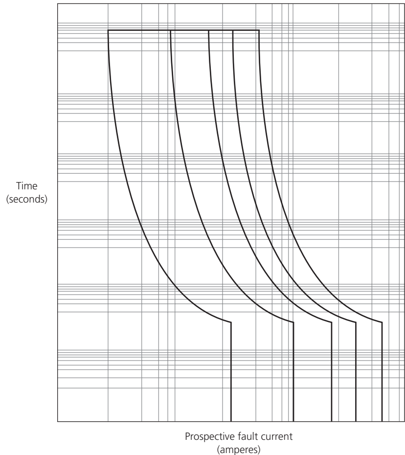
▲ Figure 3.14 Sample time–current characteristic graph
