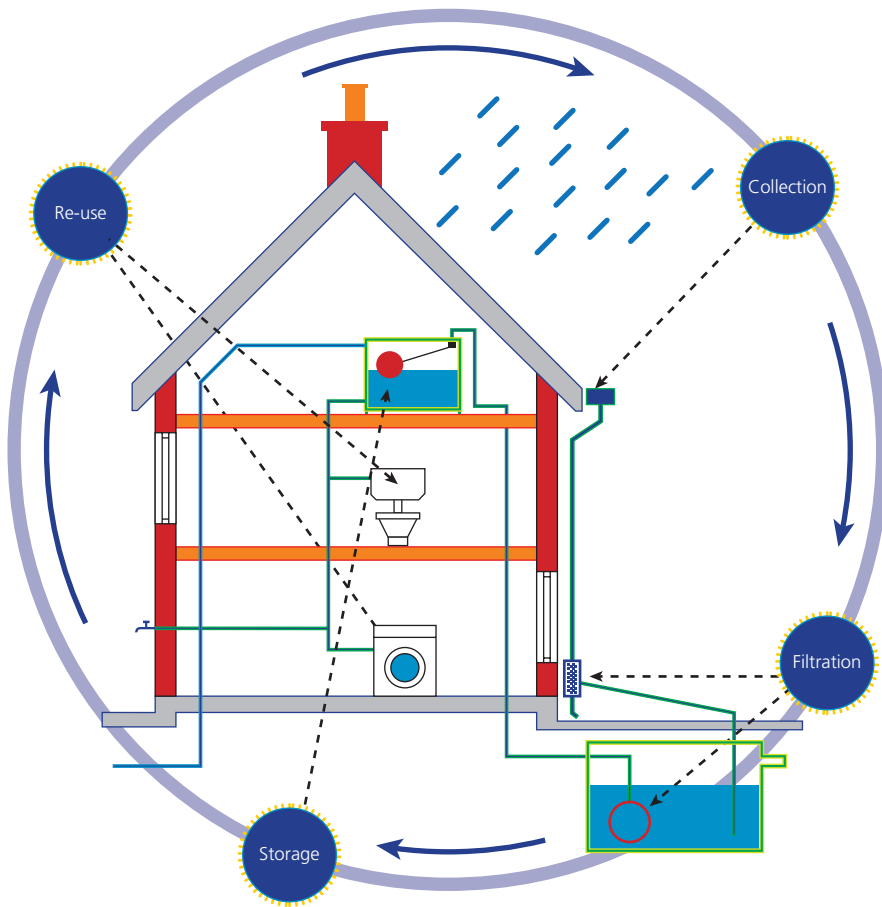
▲ Figure 1.51 Rainwater-harvesting cycle
