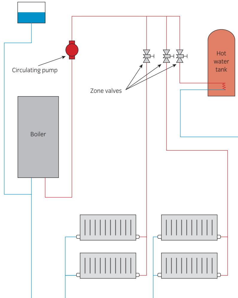
▲ Figure 2.130 Simplified central heating system
