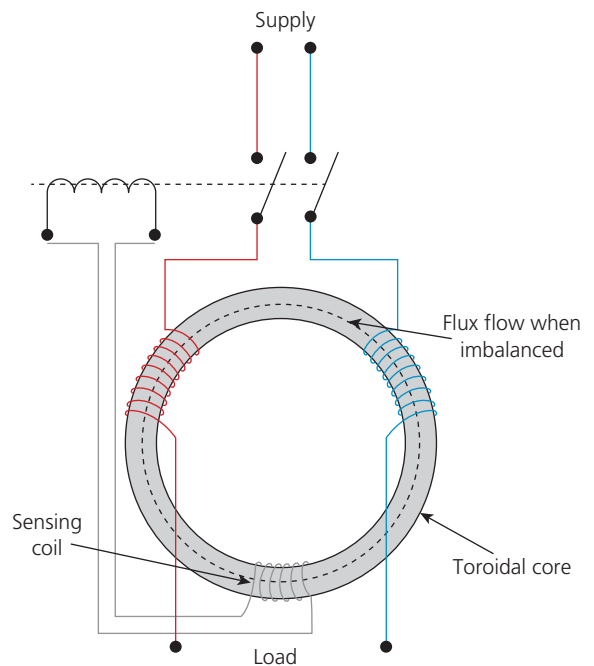
▲ Figure 3.15 Internal circuit diagram for an RCD
