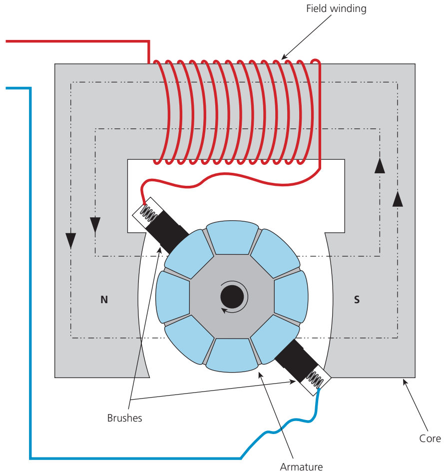
▲ Figure 2.82 Section through a universal motor
