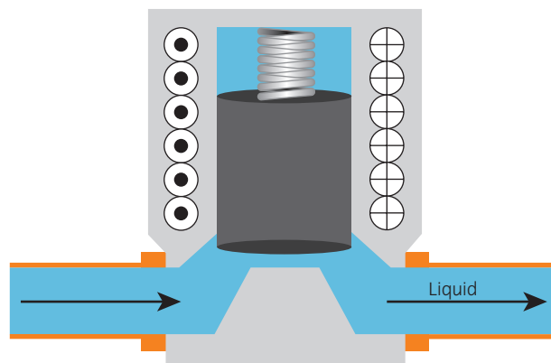
▲ Figure 2.94 Solenoid valve
