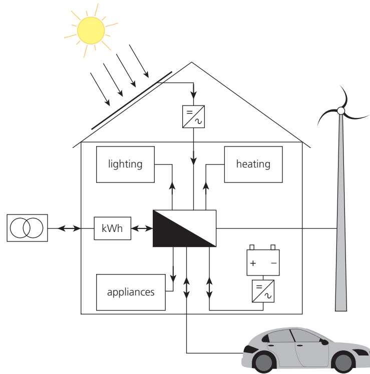
▲ Figure 3.23 A prosumer's installation which can consume energy from the public supply network as well as its own generator or electricity storage systems
