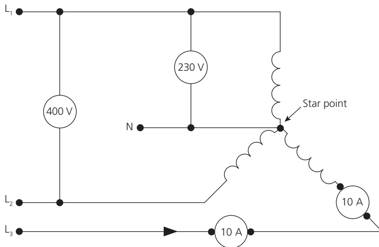
▲ Figure 2.65 Common phase and line currents in load
