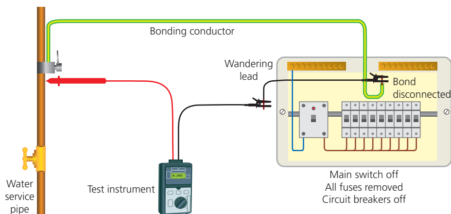
▲ Figure 6.27 Testing main protective bonding
