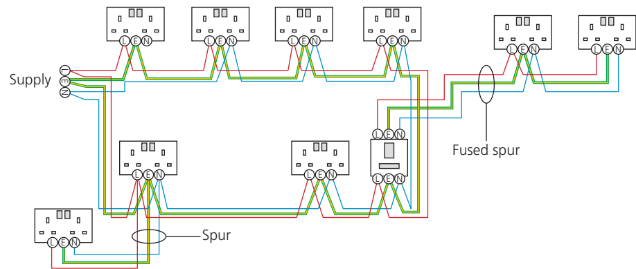
▲ Figure 5.3 Ring-final circuit showing spurs
