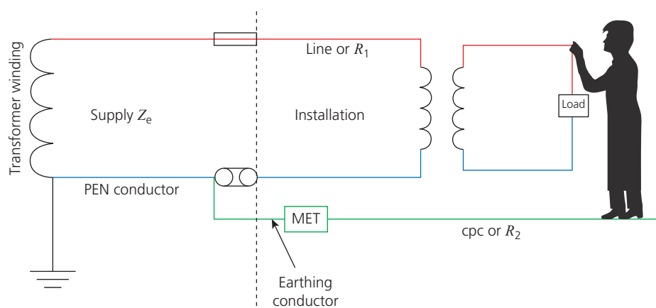
▲ Figure 3.9 Electrical separation means current cannot flow to earth as the earth is not part of the system
