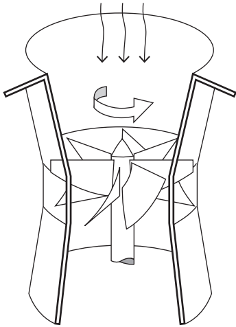
▲ Figure 1.44 Reaction turbine
