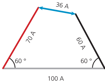
▲ Figure 2.63 In an unbalanced system, the gap (shown in light blue) represents the neutral current
