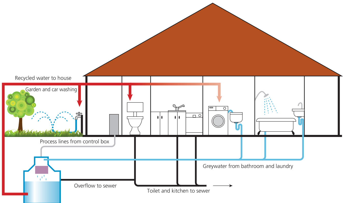
▲ Figure 1.55 Greywater reuse system
