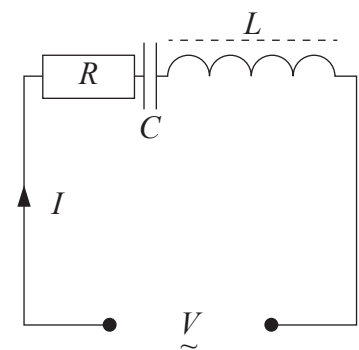
▲ Figure 2.43 RLC circuit containing all three components
