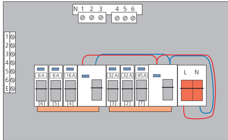
▲ Figure 5.6 Diagram of a split-way board showing three ways protected by one RCD and three ways protected by another. In total, the DB is 12-module
