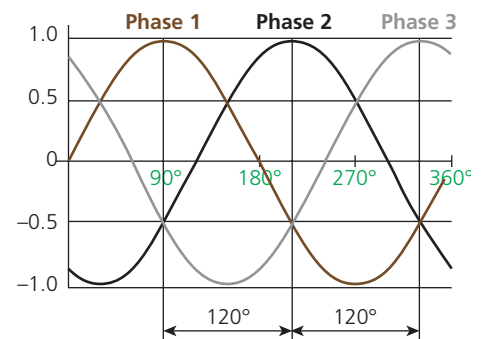
▲ Figure 2.11 Three-phase sine wave where each waveform is 120^\circ apart
