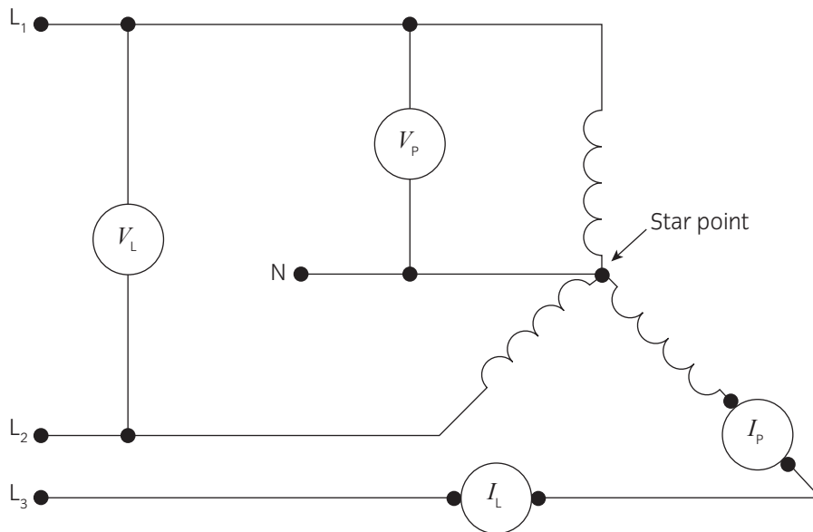
▲ Figure 2.64 Star-connected load
