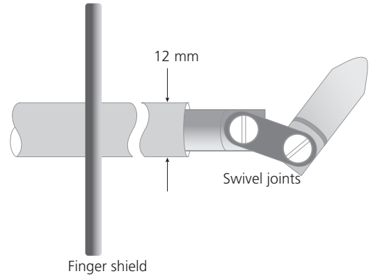
▲ Figure 6.15 British Standard finger (IPXXB)
