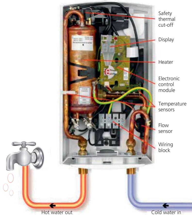
▲ Figure 2.127 Over-sink tank-type instantaneous water heater
