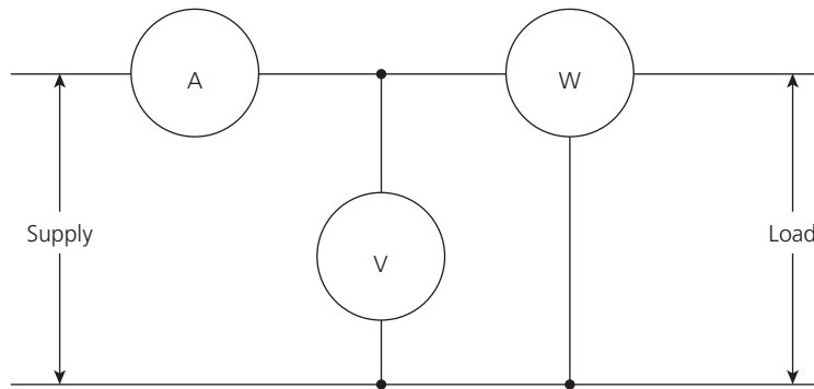
▲ Figure 2.56 Connection of instruments to calculate PF
