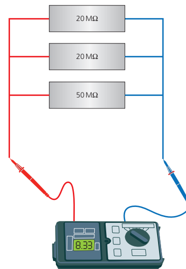
▲ Figure 6.31 The effects of testing parallel resistances
