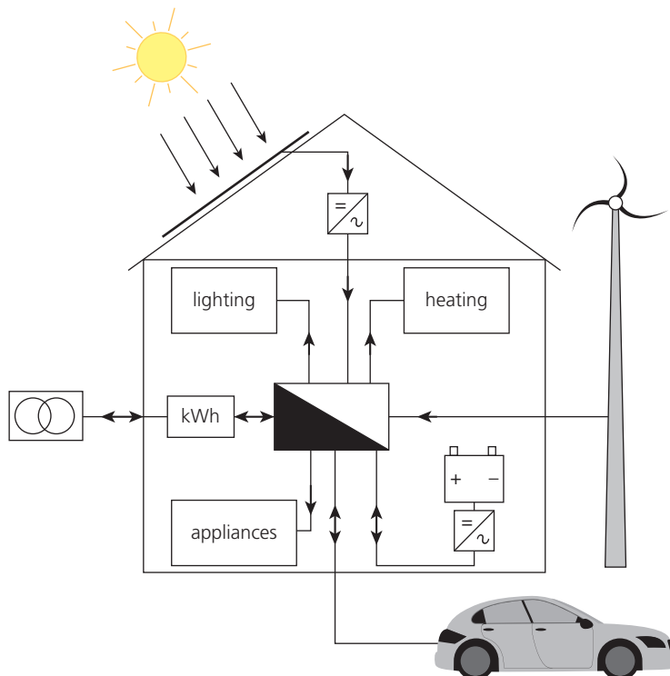
▲ Figure 2.58 A prosumer's installation which can consume energy from the public supply network as well as having its own generator or electricity storage systems
