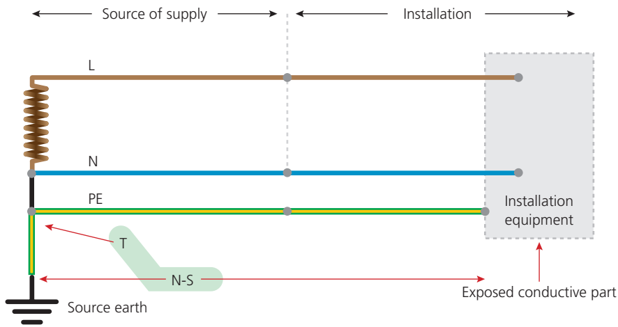
▲ Figure 3.5 TN-S earthing system
