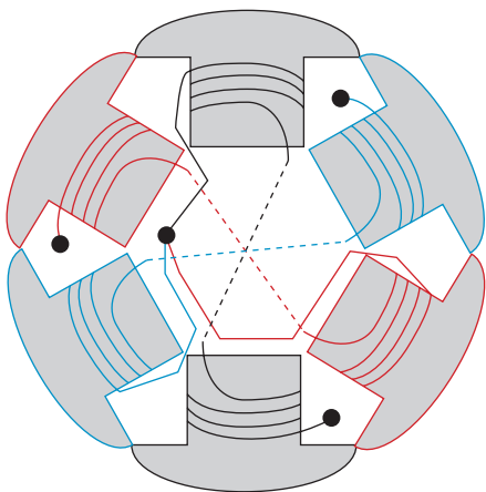
▲ Figure 2.2 Six-pole (three pairs) salient pole rotor (star wound) for an alternator
