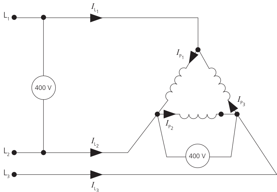
▲ Figure 2.67 Phase and line currents in the load
