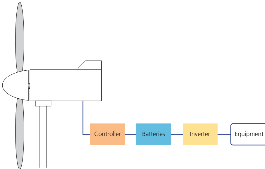
▲ Figure 1.33 Block diagram of an off-grid micro-wind system
