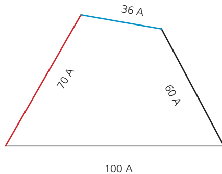
▲ Figure 2.10 This diagram represents an unbalanced system
