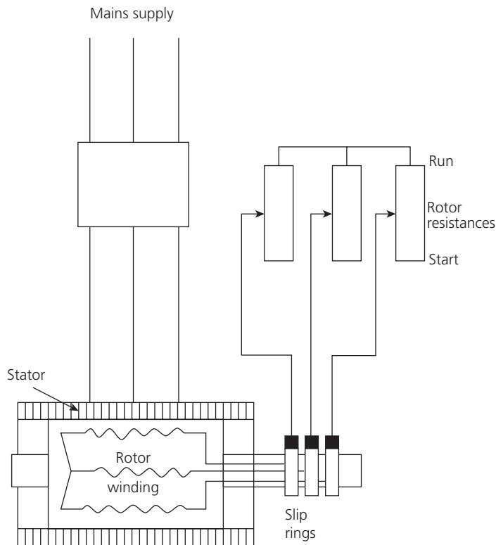
▲ Figure 2.78 Wound rotor arrangement
