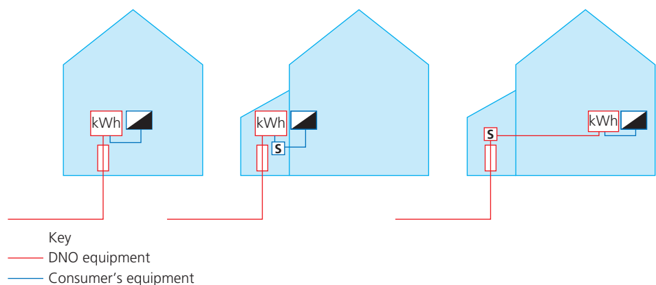
▲ Figure 5.1 Typical layouts indicating responsibility where the meter is in the house next to the CU, where the meter is external and the CU internal, where the cut-out is external and the meter internal
