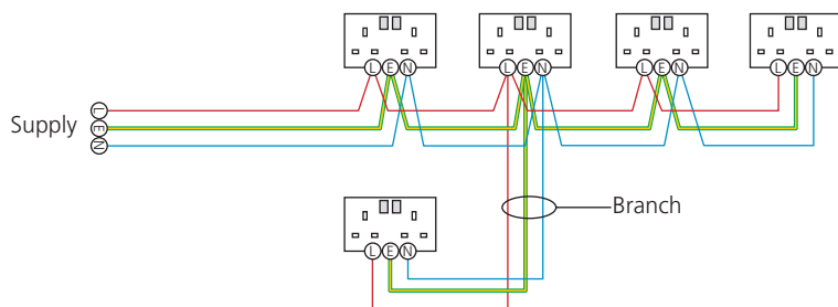
▲ Figure 5.2 Radial circuit showing branch
