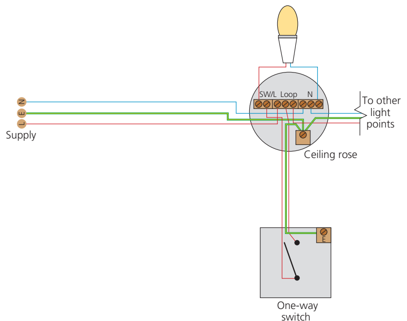
▲ Figure 5.4 A three-plate one-way lighting circuit
