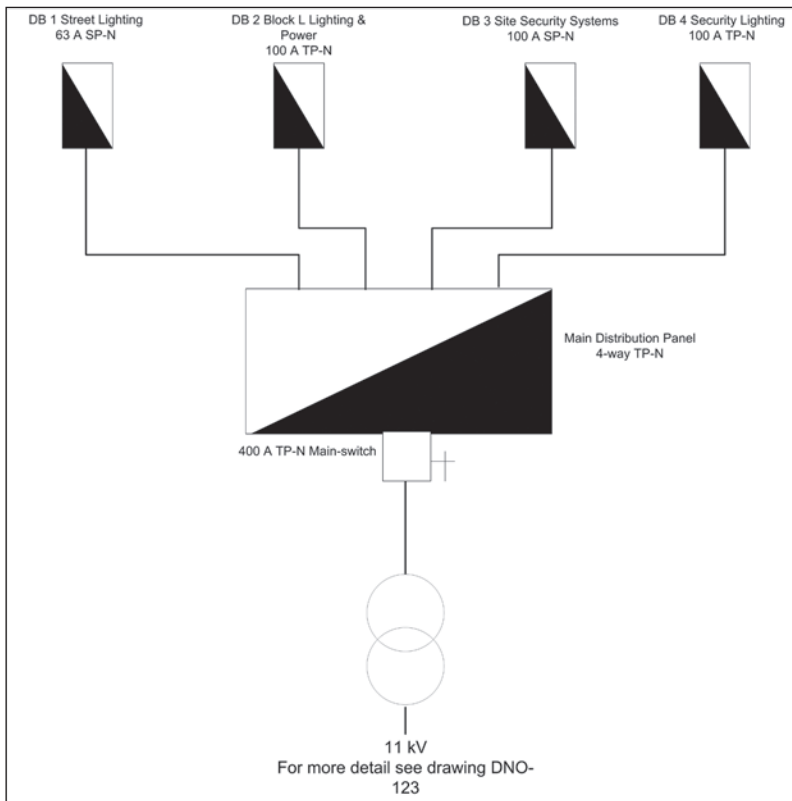
▲ Figure 4.3 Basic schematic drawing
