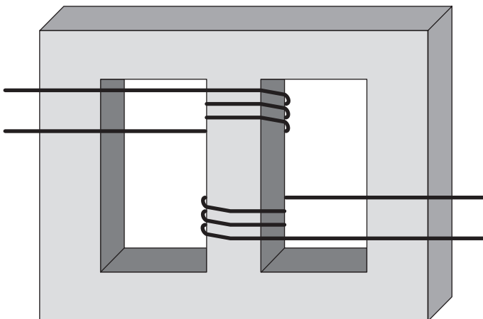
▲ Figure 2.21 Shell-type core
