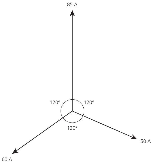
▲ Figure 2.59 Step 1 Construct a basic three-phase phasor to a suitable scale, ensuring the phases are 120^\circ apart (not to scale)
