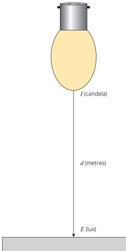
▲ Figure 2.100 The inverse square law is used to determine the illuminance (lux) of a surface
