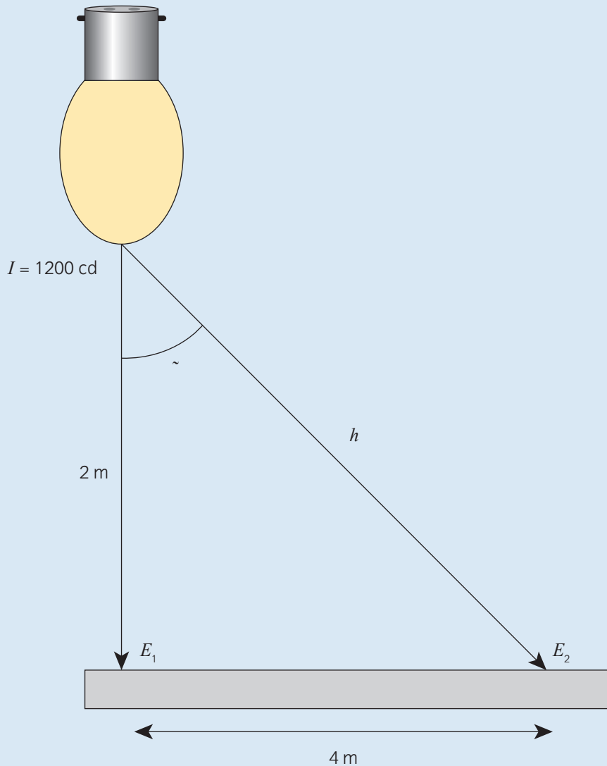
▲ Figure 2.103 Calculating illuminance directly below the source and 4 m away
