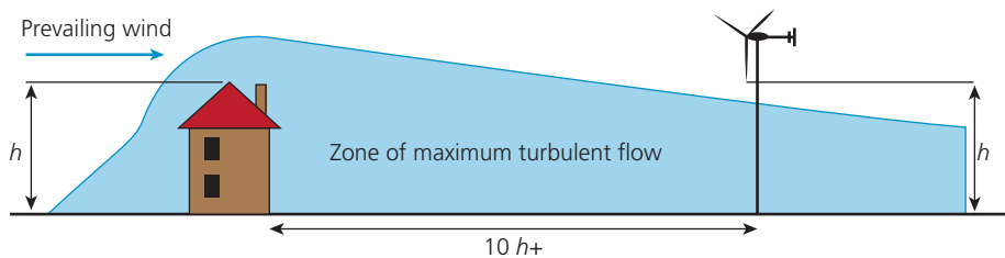
▲ Figure 1.36 Placement of micro-wind turbines to avoid obstacles
