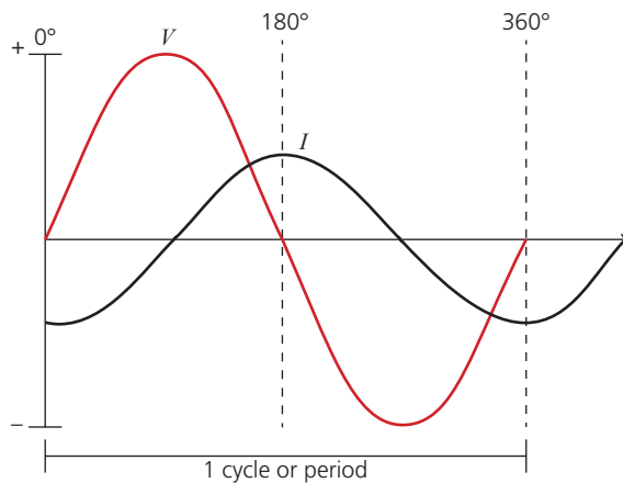
▲ Figure 2.30 Sine wave diagram showing phase shift
