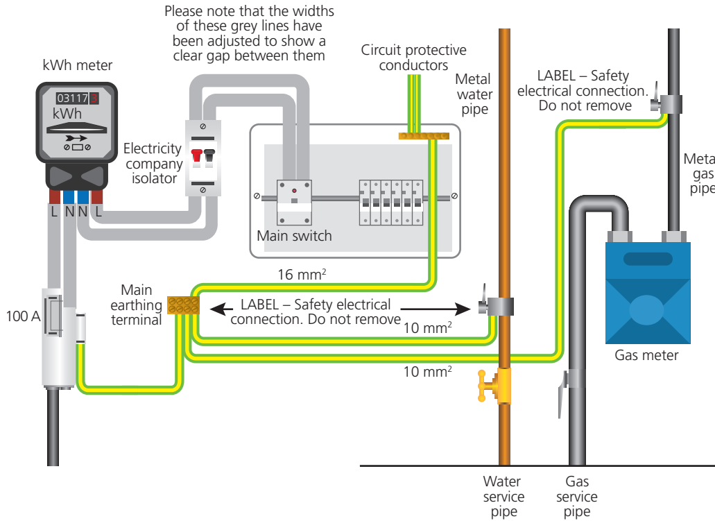
▲ Figure 3.2 Domestic TN-C-S earthing system
