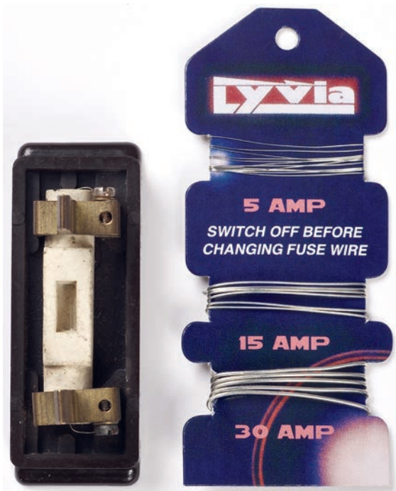
▲ Figure 3.11 Rewirable fuse and fuse wire card, showing how wrong wire can easily be used
