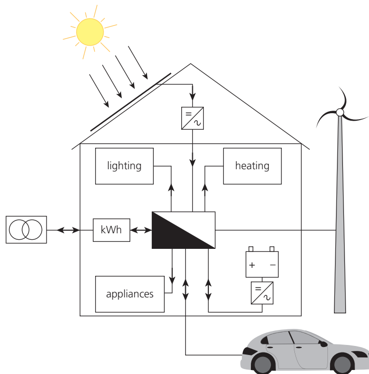
▲ Figure 5.14 A prosumer's installation which can consume energy from the public supply network as well as from its own generator or electricity storage systems
