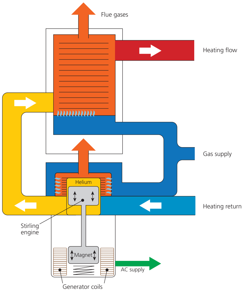
▲ Figure 1.49 Component parts of a micro-CHP boiler
