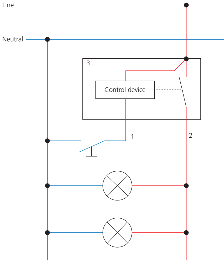
▲ Figure 3.17 Example showing where neutral switching is permissible
