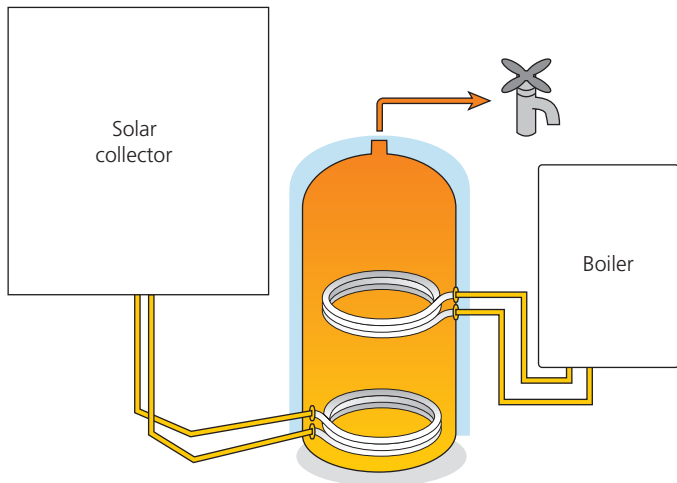
▲ Figure 1.5 Twin-coil cylinder
