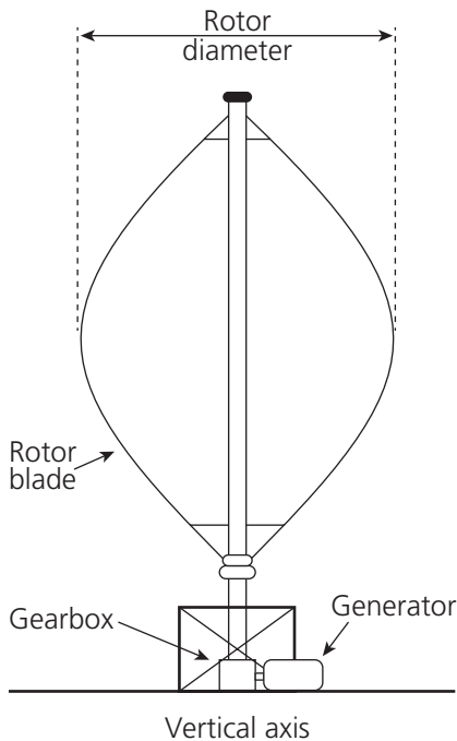
▲ Figure 1.31 Vertical-axis wind turbine
