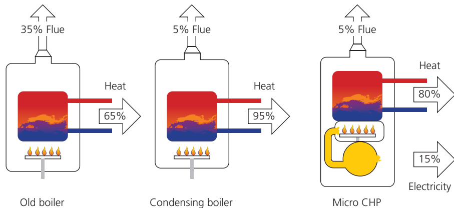
▲ Figure 1.48 The efficiency of different boilers
