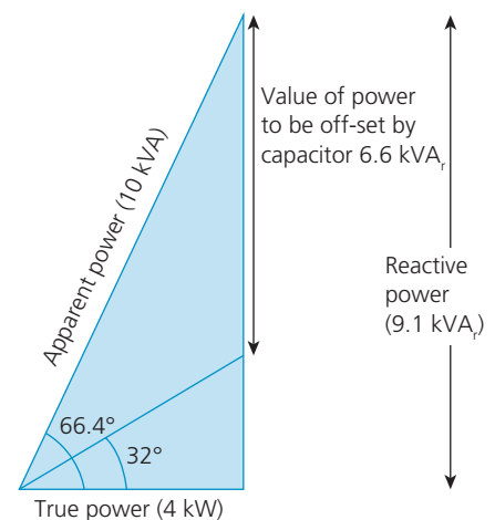
▲ Figure 2.51 Power triangle showing correction of power factor (not to scale)
