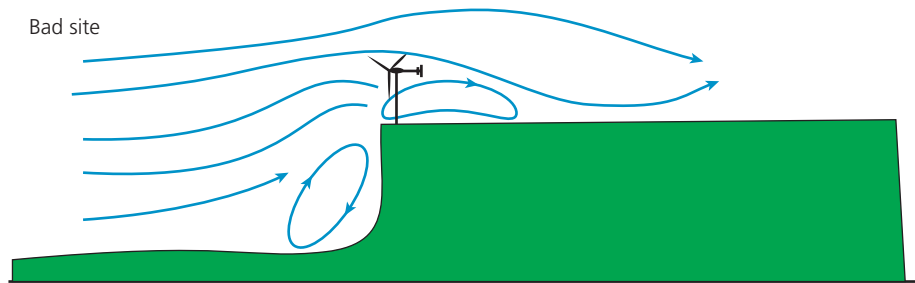
▲ Figure 1.35 An unsuitable site for a micro-wind turbine
