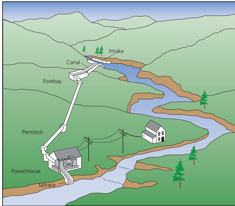
▲ Figure 1.38 The component parts of a micro-hydro system
