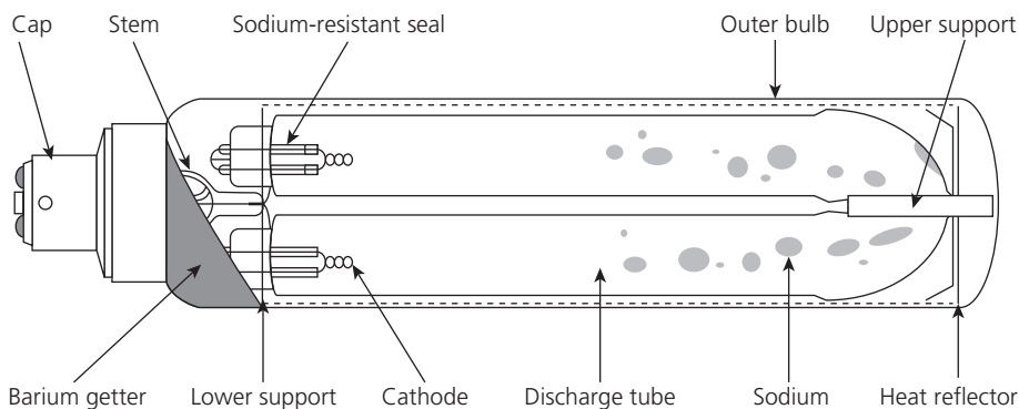
▲ Figure 2.108 Low-pressure sodium lamp
