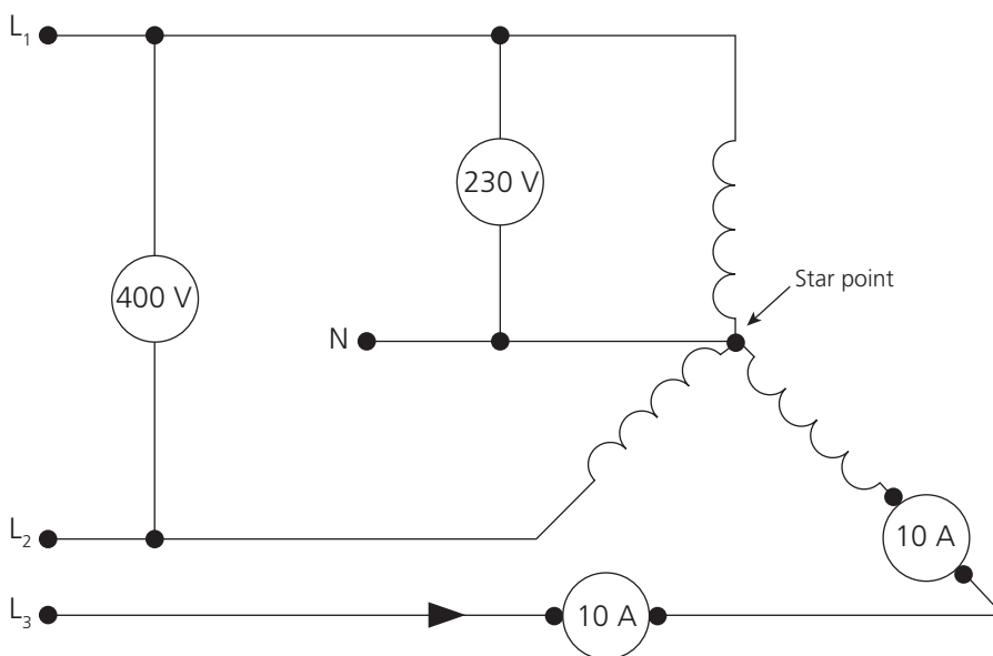
▲ Figure 2.14 Common phase and line currents in load
