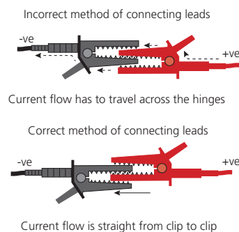
▲ Figure 6.25 Always connect leads correctly
