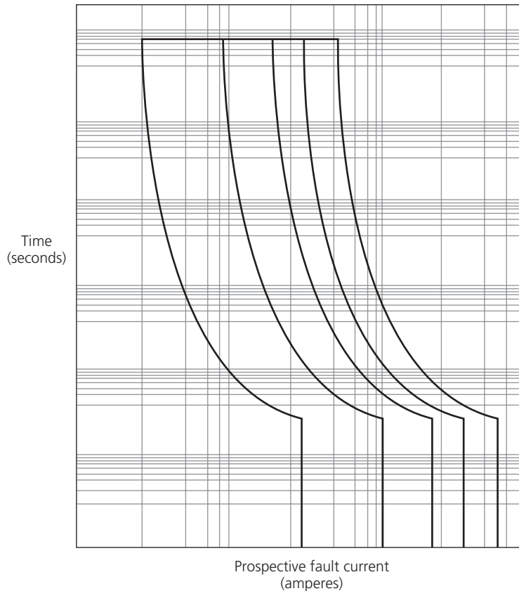
▲ Figure 2.97 Sample time–current characteristic graph which is found in Appendix 3 of BS 7671: 2018 (2022)
