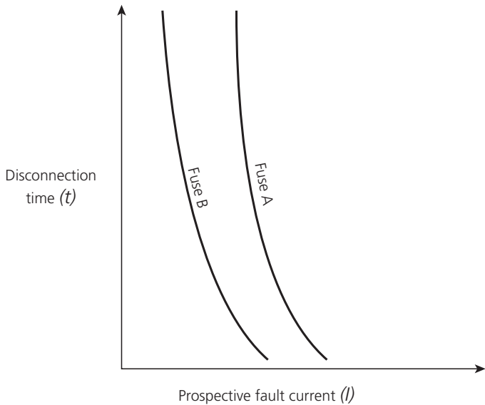
▲ Figure 3.20 Fuse characteristics
