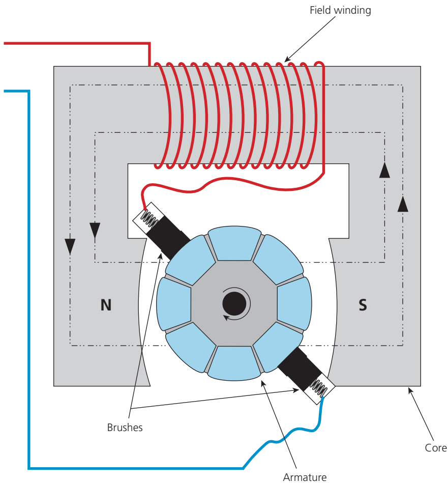
▲ Figure 2.70 Simplified series motor arrangement
