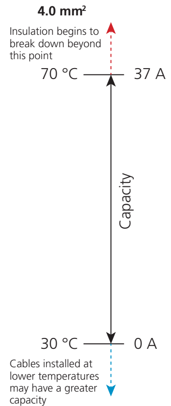
▲ Figure 5.9 PVC/PVC flat twin, 70°C thermoplastic, 30°C ambient temperature
