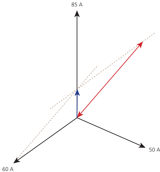
▲ Figure 2.61 Step 3 Now construct another parallelogram between the new line and the remaining phase. Where the two new parallelogram lines intersect represents the neutral current value to the scale selected
