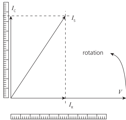
▲ Figure 2.47 Constructing a phasor for a parallel circuit
