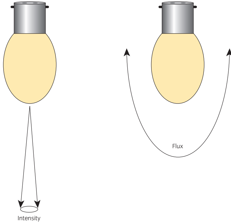
▲ Figure 2.99 Candela is the rating of intensity. The rating of total light output in all directions is the lumen.
