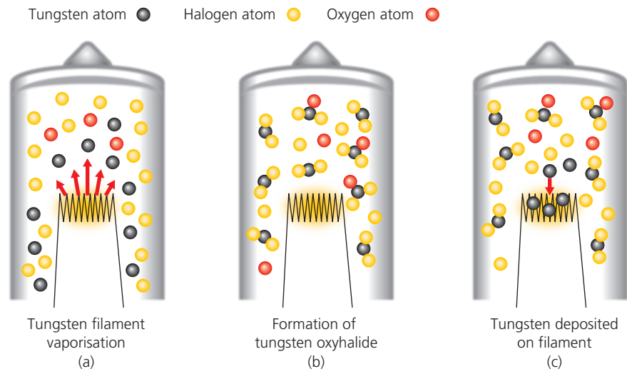
▲ Figure 2.104 Halogen regenerative cycle
