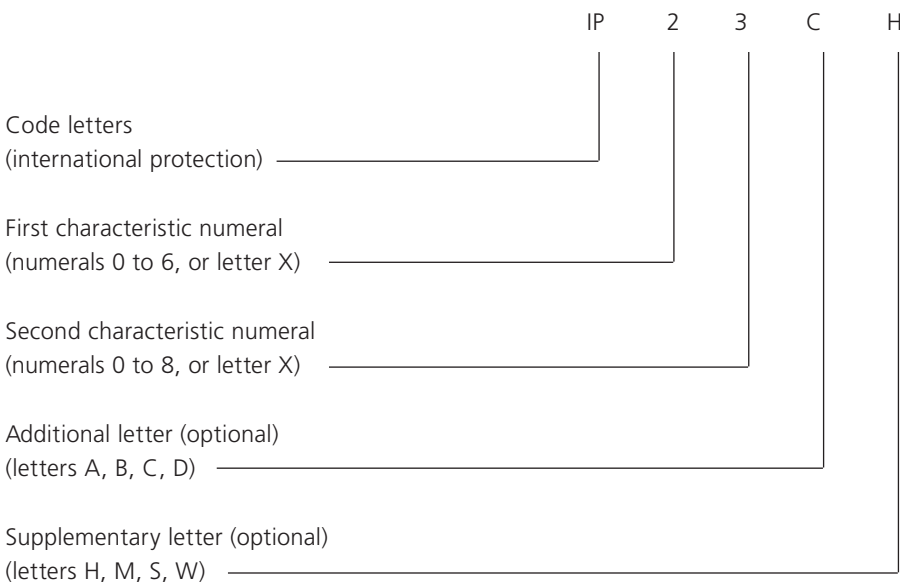
▲ Figure 6.14 IP code designated numbers and letters
