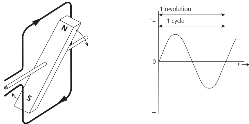
▲ Figure 2.73 Two-pole machine and output
