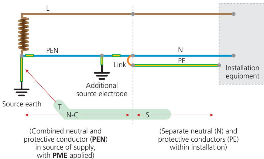
▲ Figure 3.3 TN-C-S earthing system
