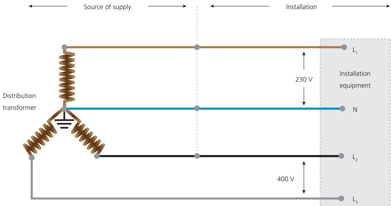
▲ Figure 2.12 Three-phase AC supply
