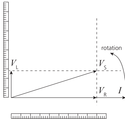
▲ Figure 2.42 Drawing in the supply voltage
