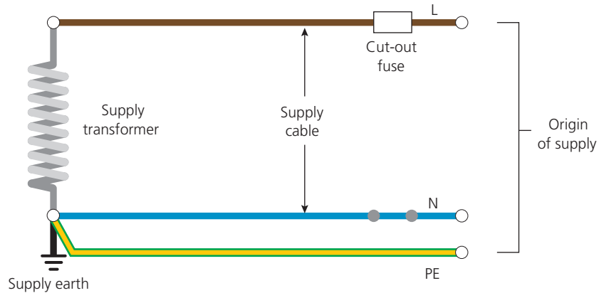
▲ Figure 6.33 Simple representation for a TN-S system
