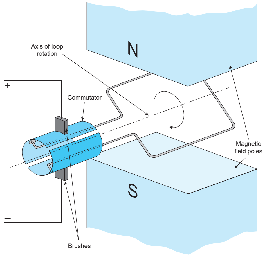
▲ Figure 2.69 A simple generator arrangement
