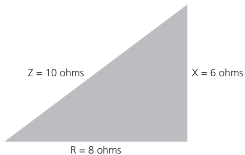
Scaled triangle resulting in an impedance (Z) of 10 Ω
