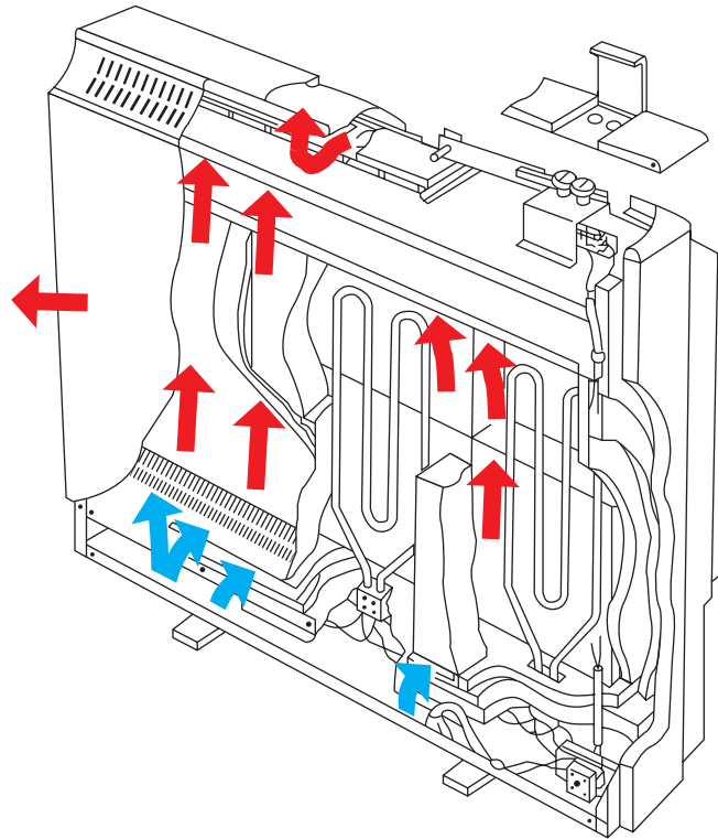
▲ Figure 2.121 Electric storage heater
