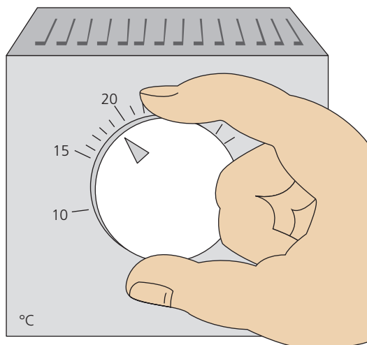
▲ Figure 2.129 Simple thermostat with bimetal
