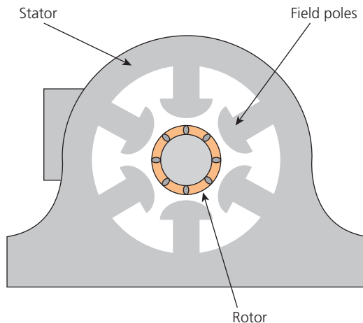
▲ Figure 2.76 Component parts of a six-pole cage induction motor
