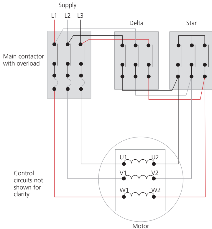
▲ Figure 2.84 Star-delta starter arrangement
