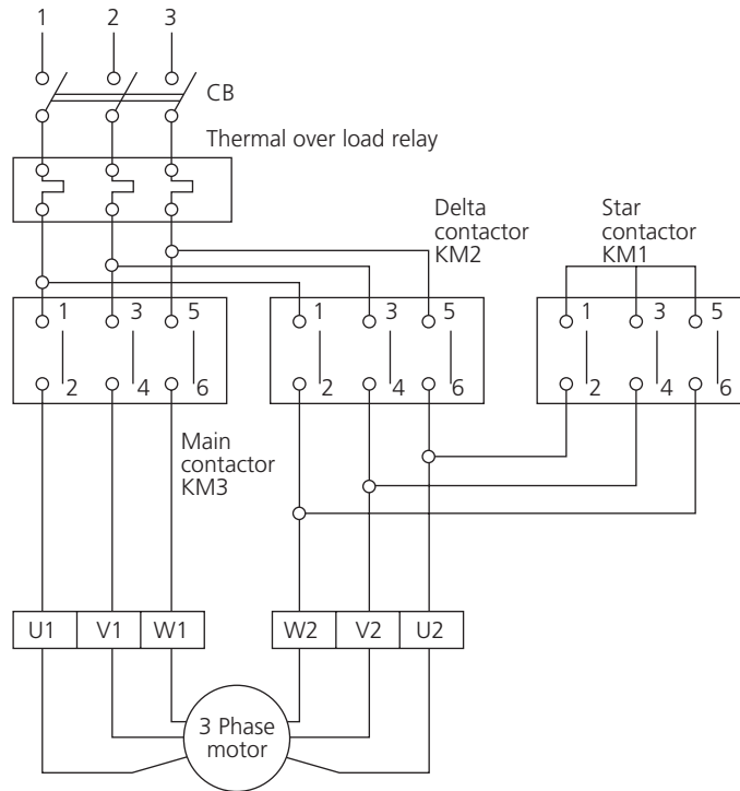
▲ Figure 4.5 Typical circuit diagram
