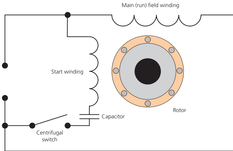
▲ Figure 2.80 Capacitor start motor
