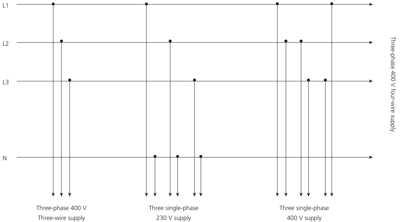
▲ Figure 2.8 Three-phase four-wire distribution system
