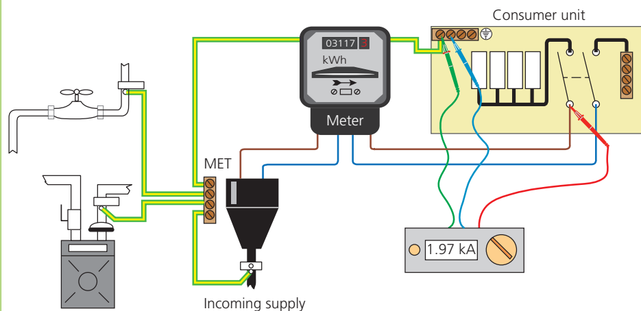
▲ Figure 6.38 Sometimes when testing prospective fault current using a three-lead tester, you may have to double up on the earth and neutral leads to get the most accurate results
