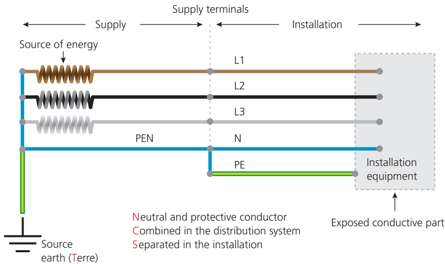
▲ Figure 6.34 A three-phase supply for a TN-C-S installation
