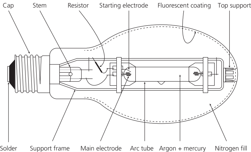
▲ Figure 2.107 High-pressure mercury lamp
