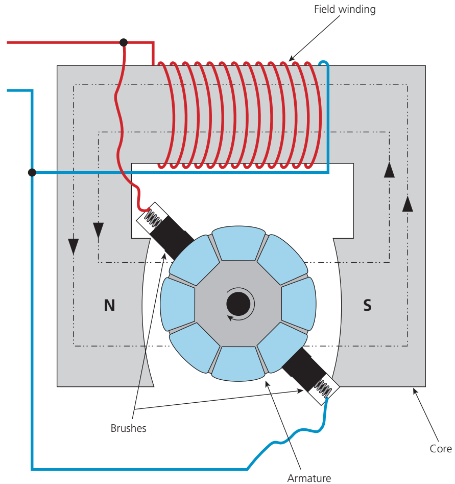
▲ Figure 2.71 Simplified shunt motor arrangement
