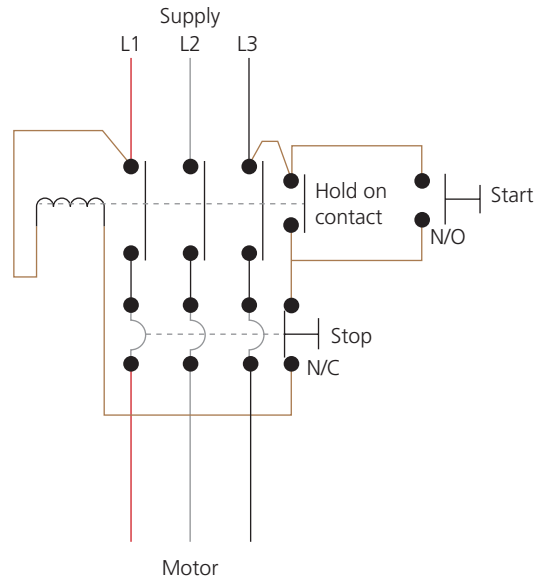
▲ Figure 2.83 Direct online (DOL) starter
