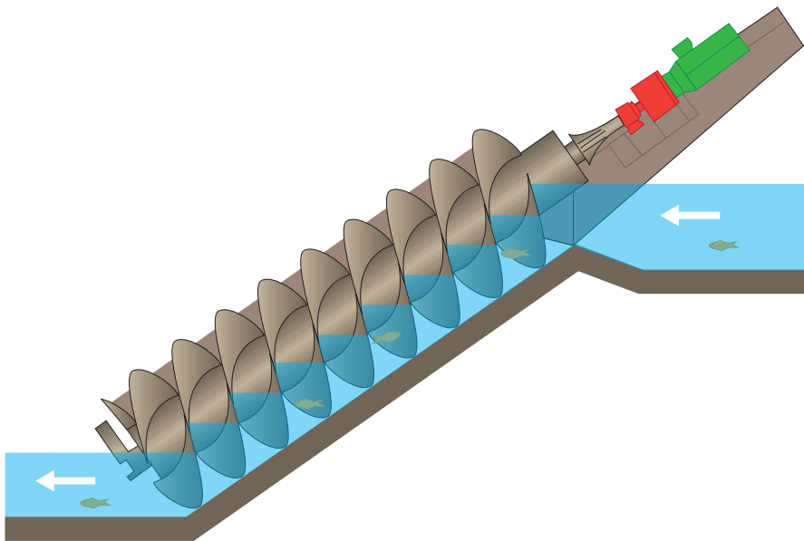
▲ Figure 1.47 Reverse Archimedes' screw
