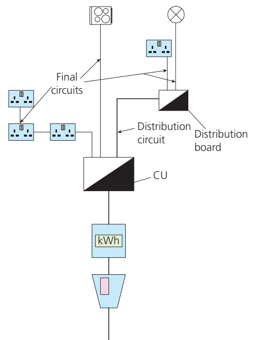
▲ Figure 5.5 Final and distribution circuits in a simple installation
