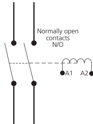
▲ Figure 2.93 Typical contactor
