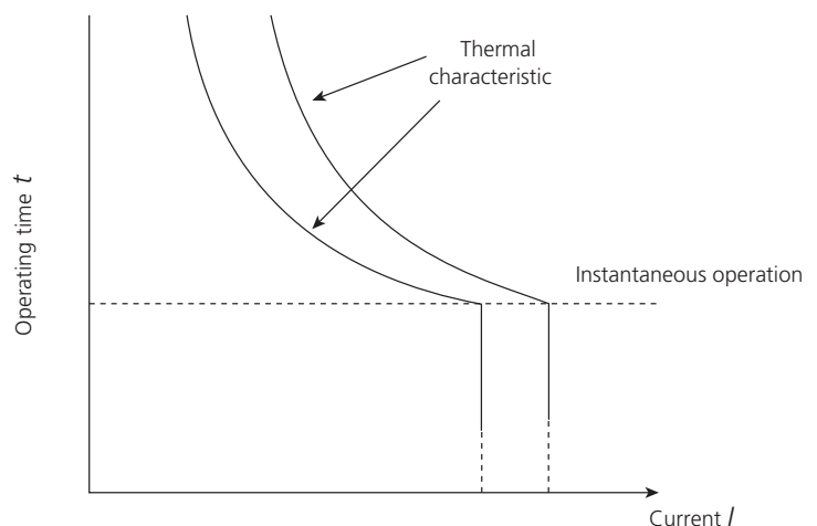
▲ Figure 5.8 Circuit-breaker characteristics
