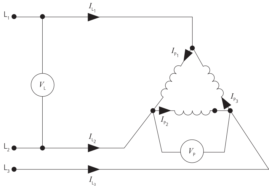
▲ Figure 2.15 Delta-connected load similar to delta-connected supply
