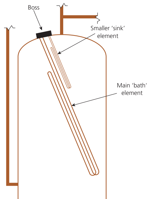
▲ Figure 2.125 Cylinder element arrangements
