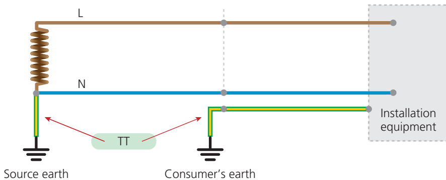
▲ Figure 3.6 TT earthing system
