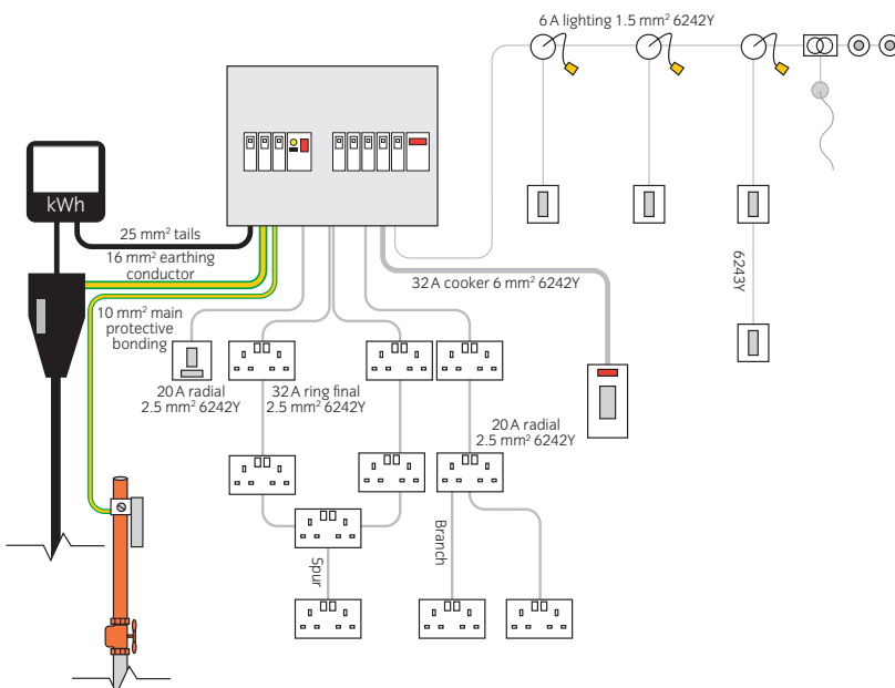
▲ Figure 4.4 Typical wiring drawing
