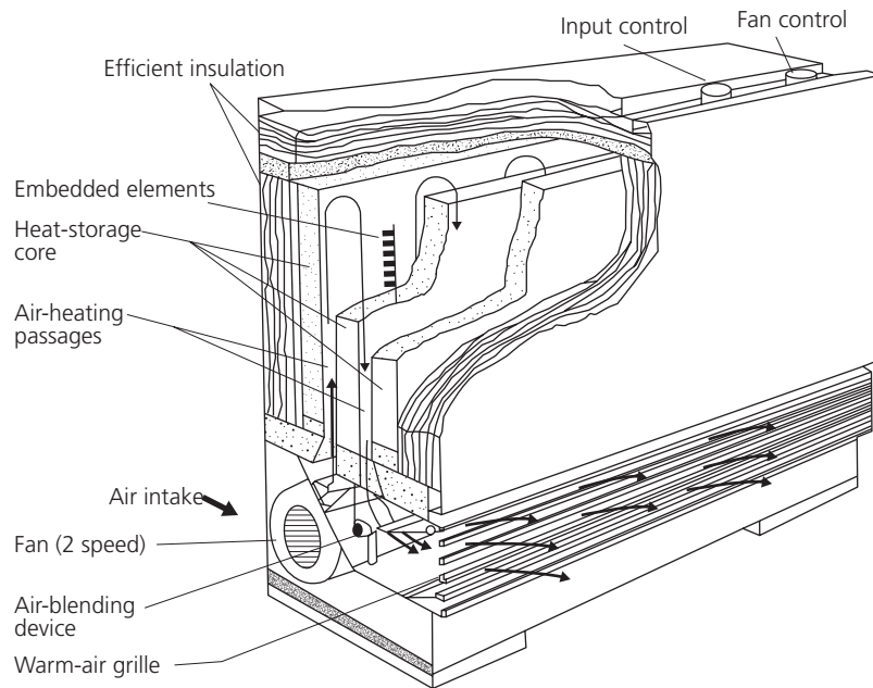
▲ Figure 2.122 Fan-assisted storage heater
