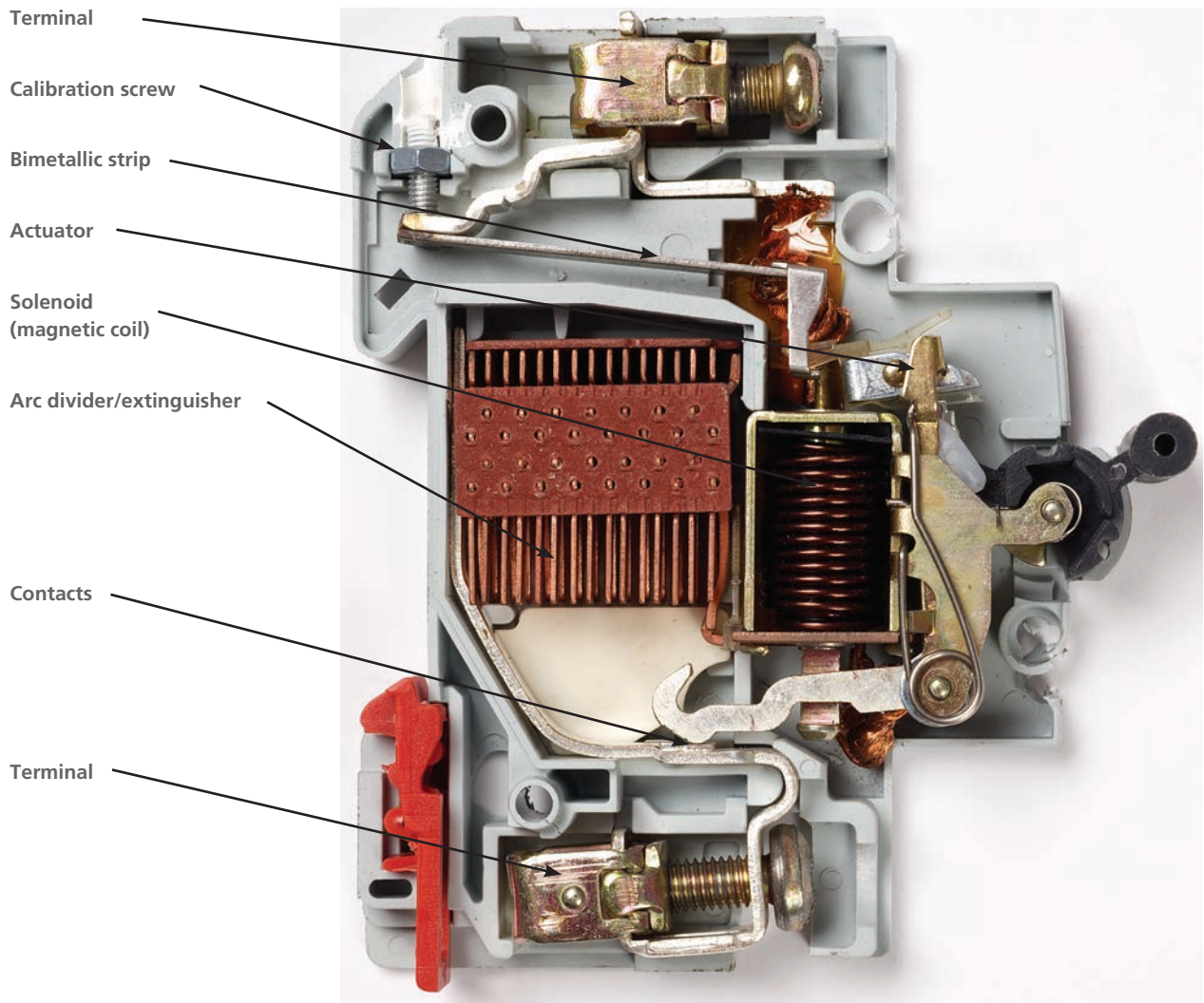
▲ Figure 3.13 Section through a circuit breaker
