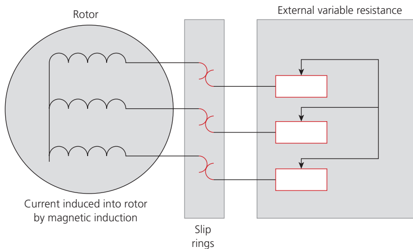
▲ Figure 2.85 Rotor resistance control circuit (stator field winding and supply circuits are not shown for clarity)
