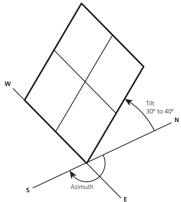
PV array facing south at fixed tilt
