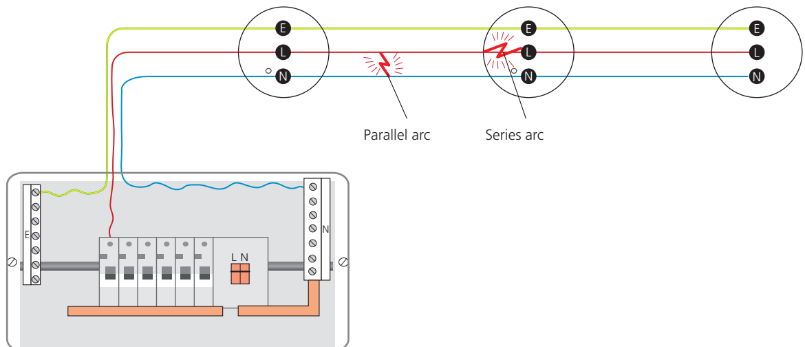
▼ Figure 2.98 Series and parallel arcs in a circuit
