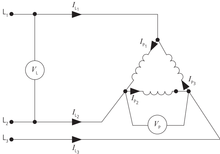
▲ Figure 2.66 Delta-connected load similar to delta-connected supply
