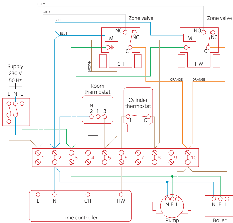
▲ Figure 2.132 Typical domestic central heating circuit diagram
