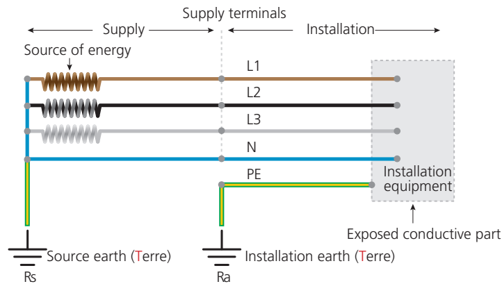
▲ Figure 6.35 A three-phase supply for a TT installation
