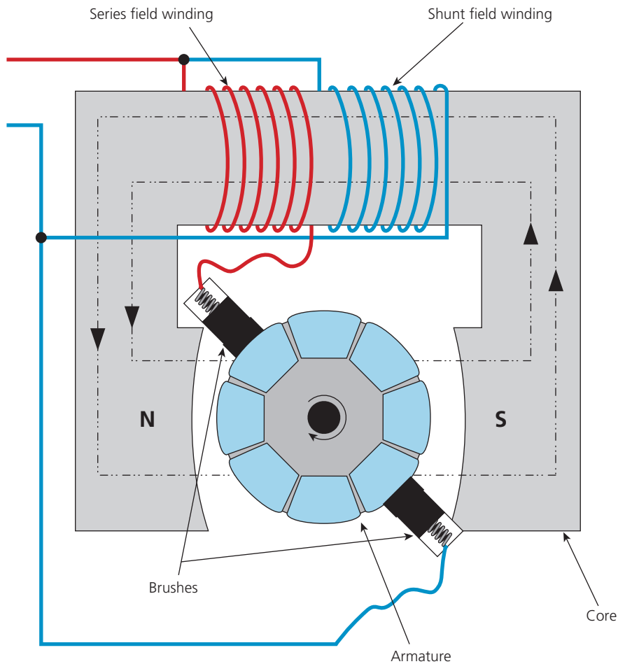
▲ Figure 2.72 Compound motor arrangement
