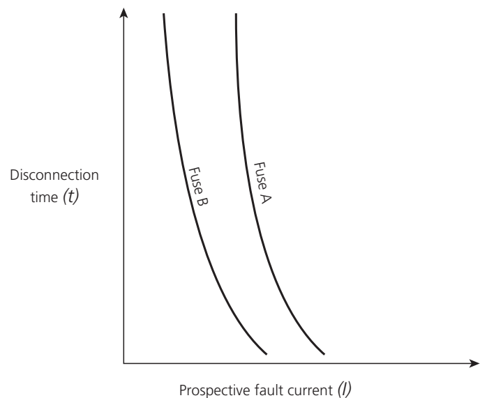
▲ Figure 5.7 Fuse characteristics
