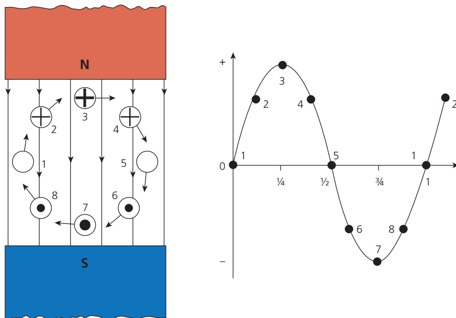
▲ Figure 2.4 The emf generated per phase per rotation
