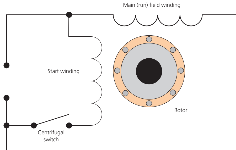
▲ Figure 2.79 Split-phase induction motor
