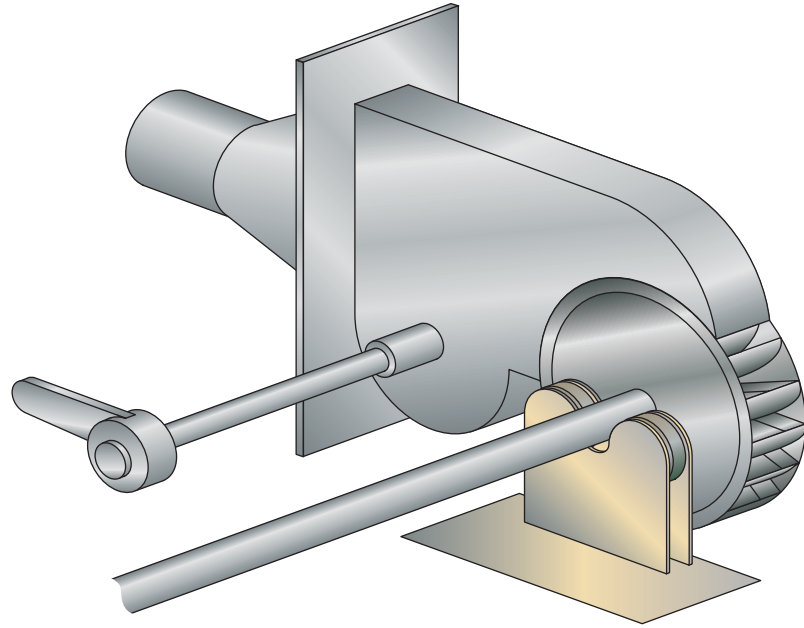
▲ Figure 1.43 Cross-flow or Banki turbine
