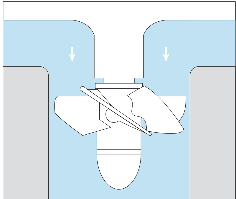
▲ Figure 1.46 Kaplan or propeller turbine
