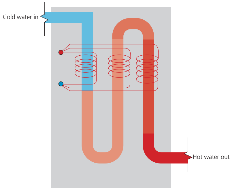
▲ Figure 2.128 Elements around the water pipe in an instantaneous water heater
