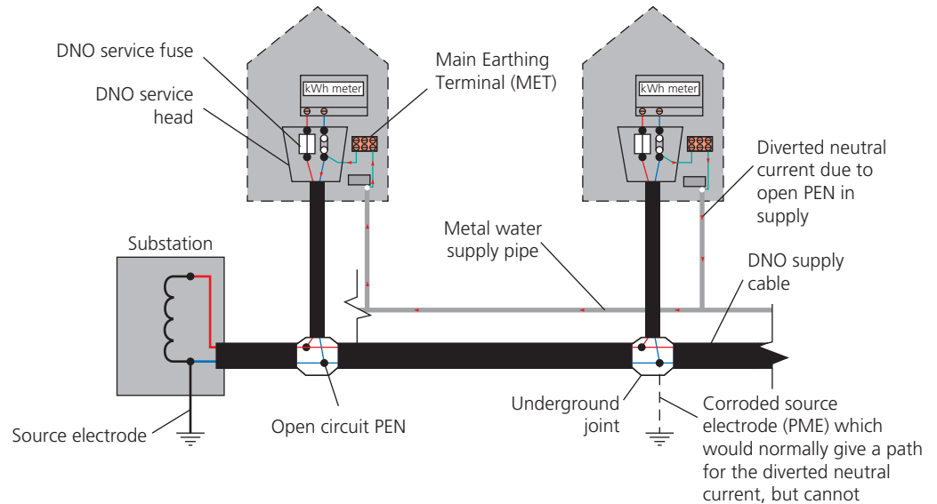
▲ Figure 3.4 The risk of diverted neutral current due to an open circuit PEN conductor
