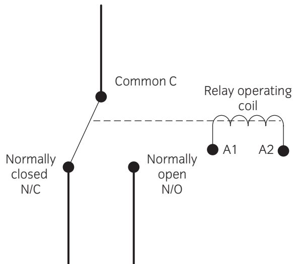
▲ Figure 2.87 Relay showing contact positions
