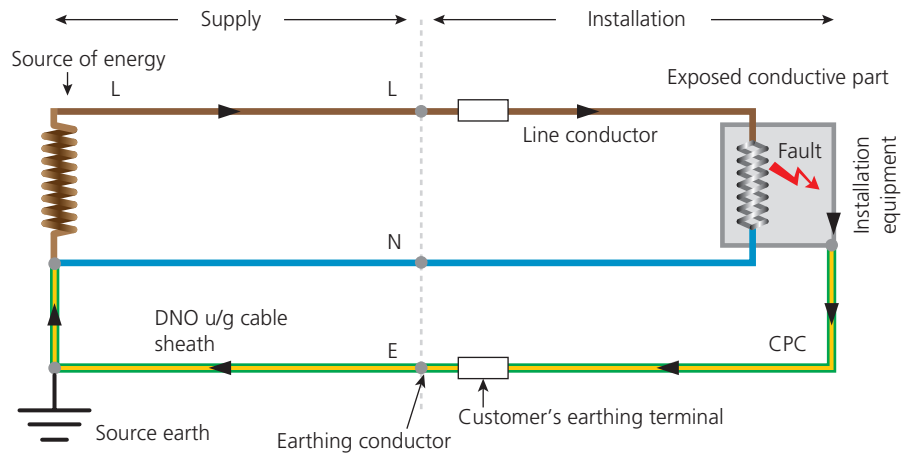
▲ Figure 2.17 Earth fault loop
