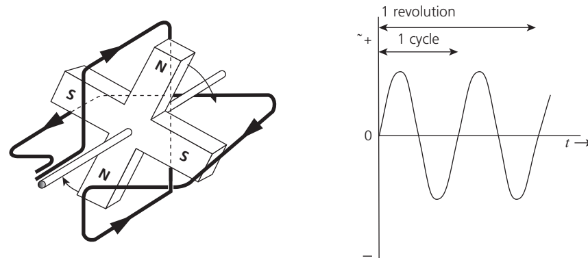
▲ Figure 2.74 Four-pole machine and output
