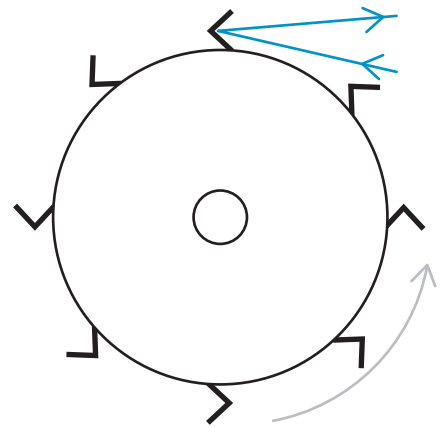
▲ Figure 1.40 Impulse turbine
