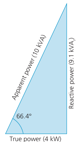
▲ Figure 2.50 Power triangle for example calculation (not to scale)
