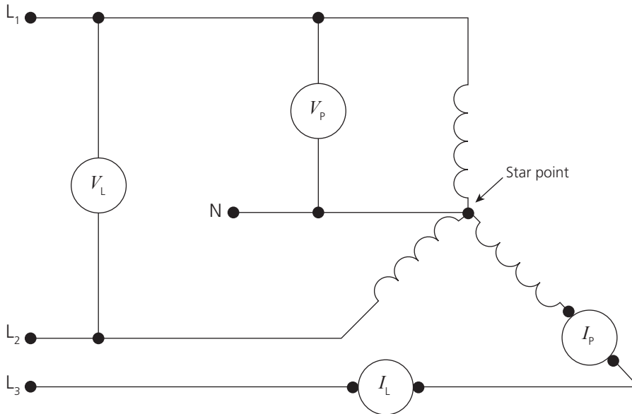
▲ Figure 2.13 Star-connected load
