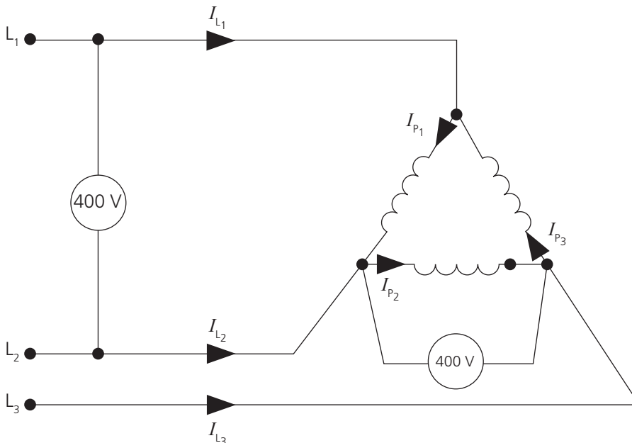
▲ Figure 2.16 Phase and line currents in the load
