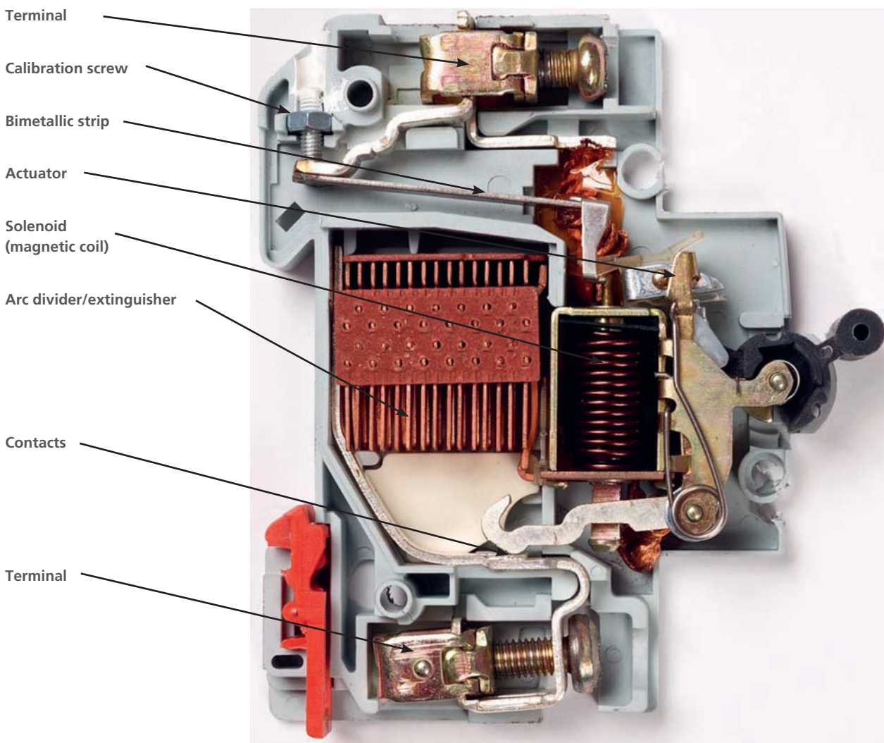
▲ Figure 2.90 Section through a circuit breaker
