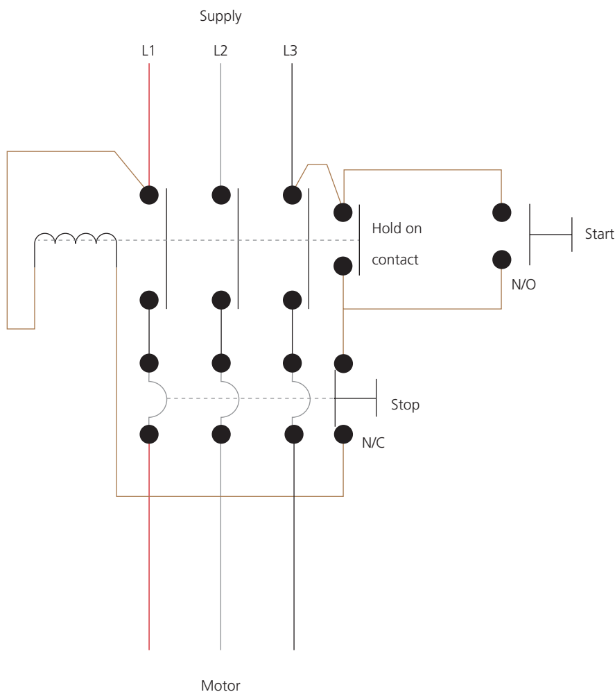
▲ Figure 2.95 A typical example of a contactor: direct online (DOL) starter arrangement
