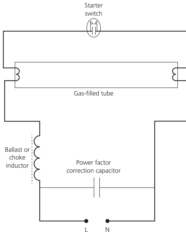
▲ Figure 2.105 How control gear works in a discharge lamp
