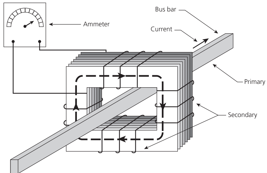
▲ Figure 2.19 A current transformer with secondary winding around the primary conductor
