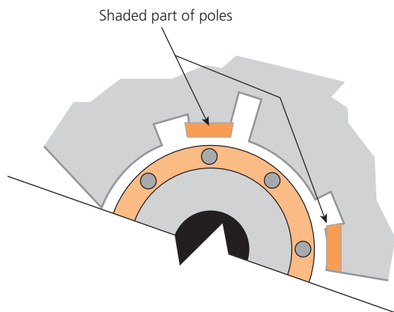
▲ Figure 2.81 Shaded-pole motor
