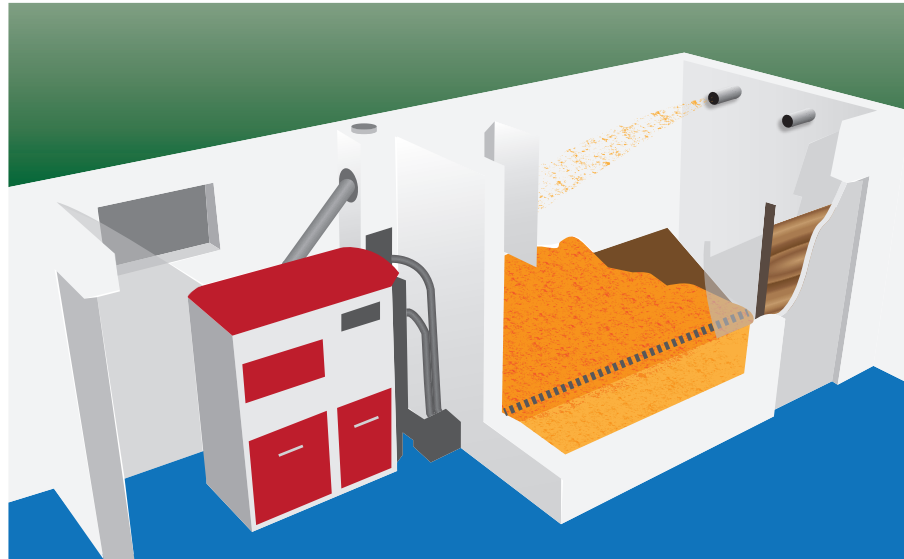
▲ Figure 1.19 Biomass boiler with suction feed system
