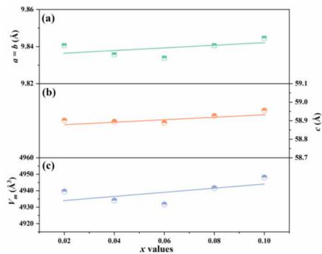
Figure 3. Lattice parameter changes (a) a and b , (b) c , and (c) V_m of CZ_{1-x}N_x ceramics as a function of x values.
