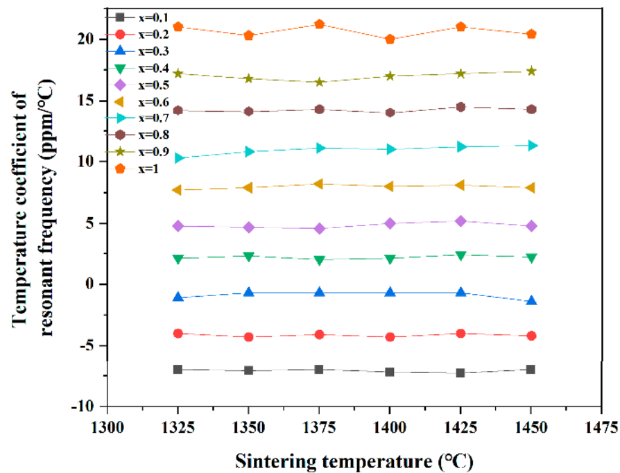
Figure 6. Temperature coefficients of resonant frequency of \text{Ba}[(\text{Zn}_x\text{Co}_{1-x})_{1/3}(\text{Nb}_{0.5}\text{Ta}_{0.5})_{2/3}]\text{O}_3 ceramics sintered at different temperatures.
