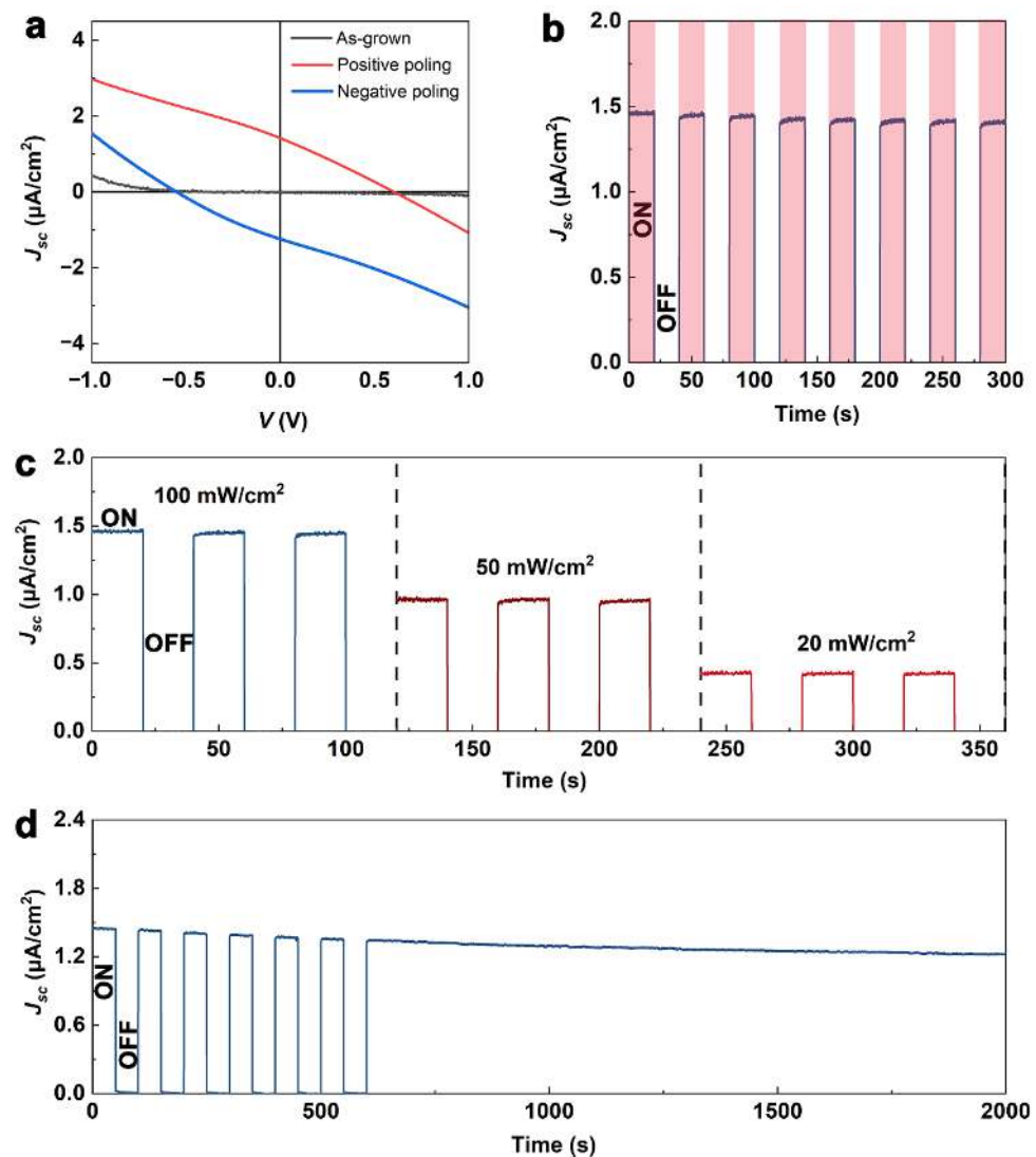
Figure 7. (a) J - V characteristics under different polarization states and (b) time-dependent J_{\text{sc}} ; (c) J_{\text{sc}} at different light intensities; (d) stability diagram of J_{\text{sc}} under sunlight.
