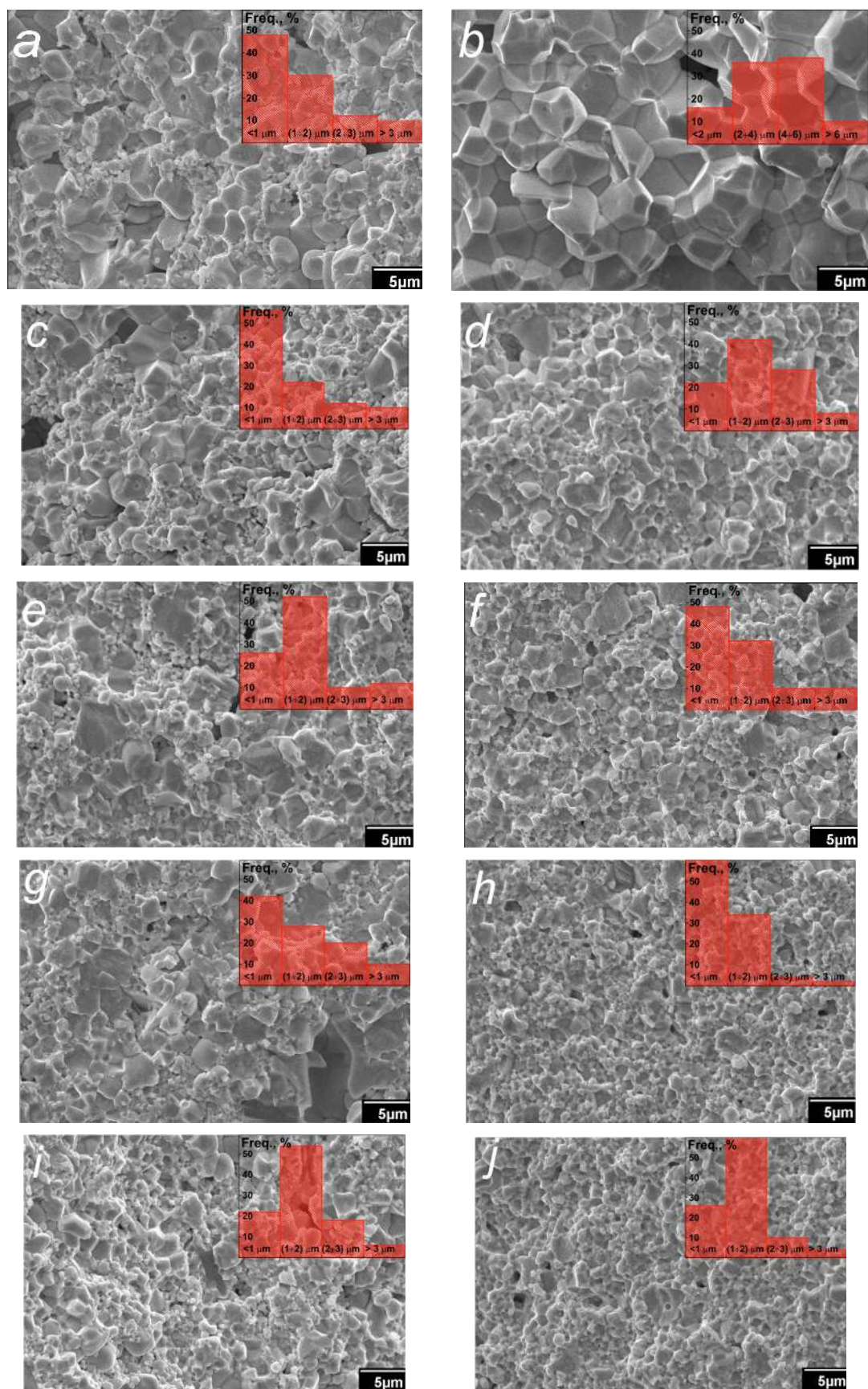
Figure 6. Microstructure of the studied ceramics: (a) BF-0.29BT, (b) BF-0.29BTm, (c) BF-0.30BT, (d) BF-0.30BTm, (e) BF-0.31BT, (f) BF-0.31BTm, (g) BF-0.32BT, (h) BF-0.32BTm, (i) BF-0.33BT, (j) BF-0.33BTm. Histograms with grain size distribution are shown in the insets.
