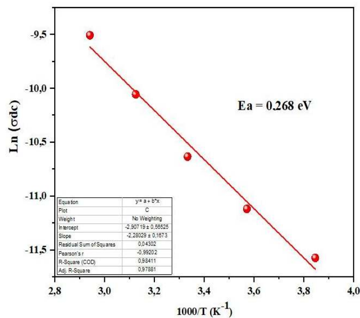
Figure 11. Variation of \ln(\sigma_{dc}) as a function of (1000/T) for (\text{Sr}_{0.75}\text{Ag}_{0.25})(\text{NiNb})_{0.5}\text{O}_3 perovskite.
