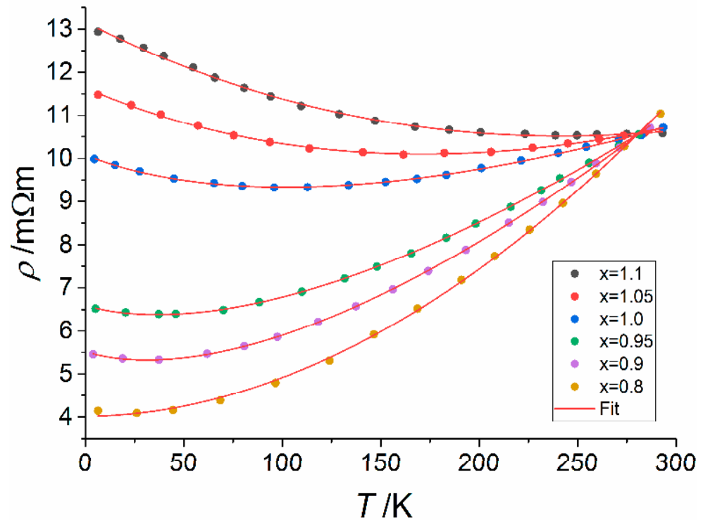
Figure 3. Fit of resistivity data from [74] of nonstoichiometric Sr 2 Fe x Mo 2-x O 6 ceramics prepared by solid-state reaction and sintered for 12 h at 1280 °C in a stream of 5% H 2 /Ar to Equation (14).
