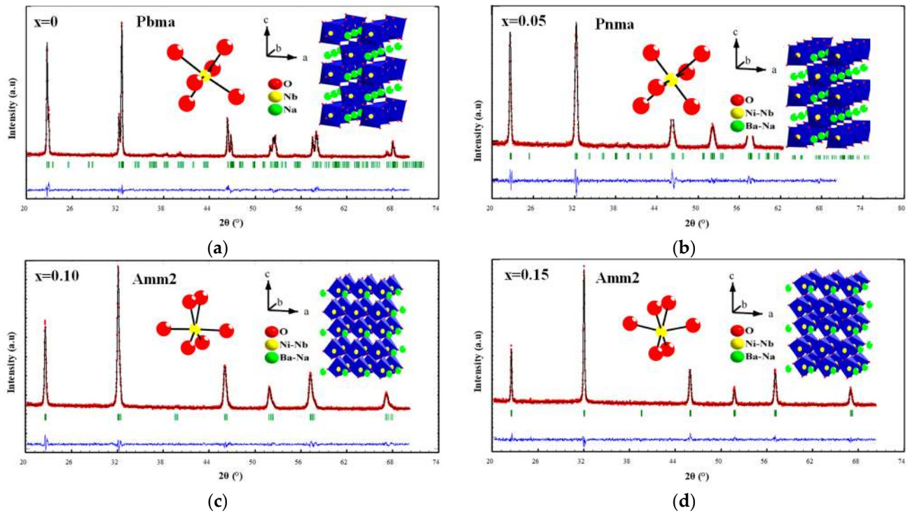
Figure 2. The Rietveld pattern obtained from X-ray powder diffraction of the \text{NBNNO}_x ceramics. (a) NNO; (b) \text{NBNNO}_{0.05} ; (c) \text{NBNNO}_{0.10} ; (d) \text{NBNNO}_{0.15} . The points represent the experimental profile, and the red solid line corresponds to the calculated profile. Positions of the Bragg reflections are indicated by green vertical bars. The blue curve at the bottom of the figure represents the discrepancy between the experimental and calculated profiles. The crystal structures were plotted inside using the “Diamond” program.
