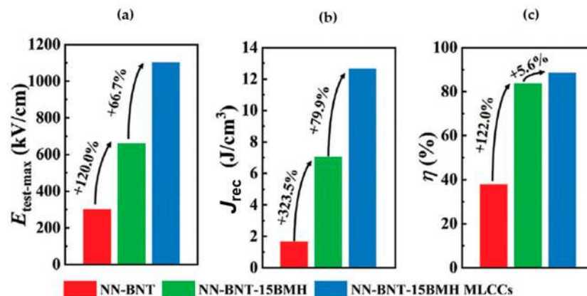
Figure 12. (a) Comparison between E_{\text{test-max}} , J_{\text{rec}} and \eta of NN-BNT, (b) NN-BNT-15BMH ceramic, (c) NN-BNT-15BMH MLCCs [124].
