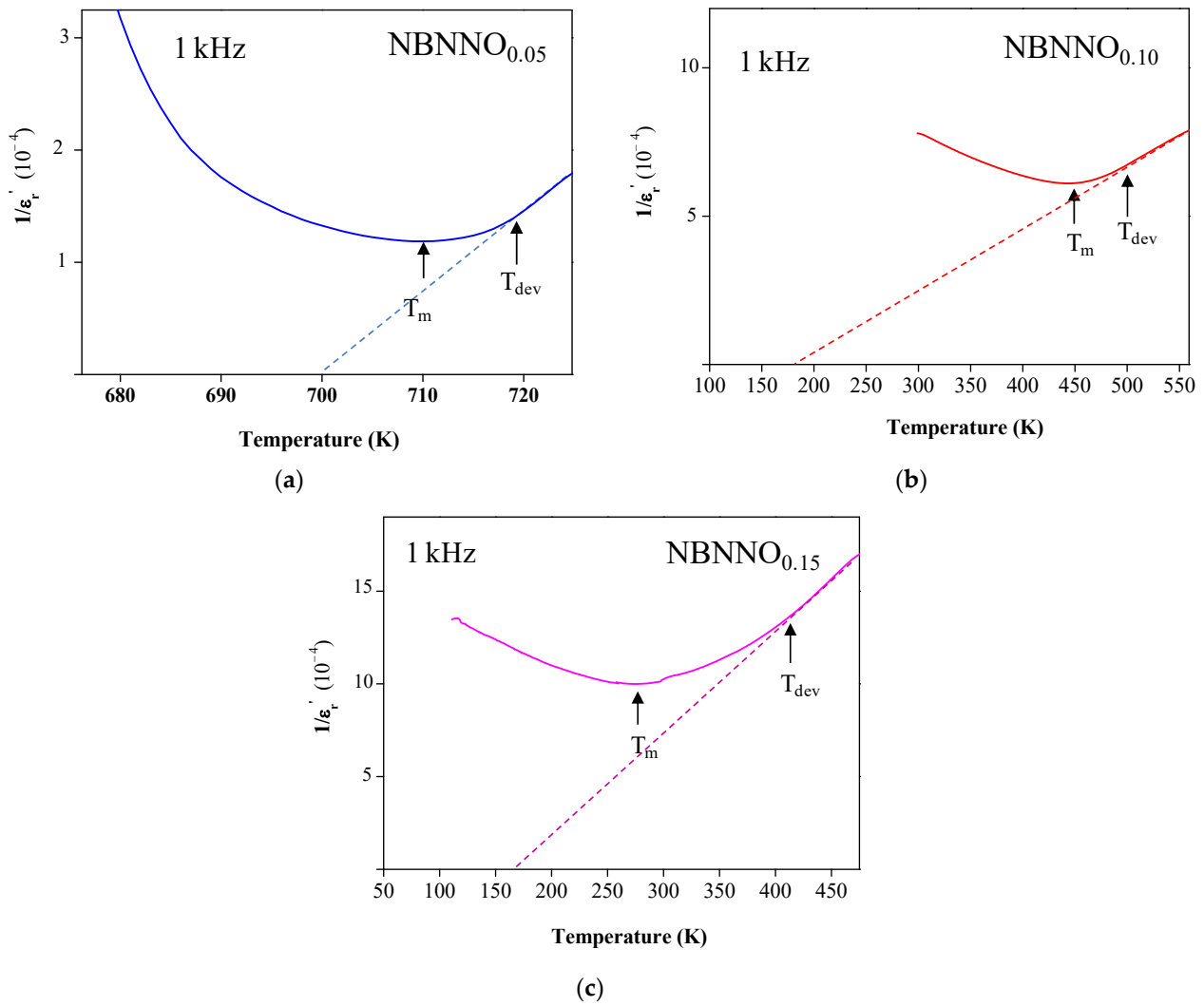
Figure 15. Temperature dependence of the inverse dielectric constant for the doped \text{NBNNO}_x ceramics at 1 kHz: (a) \text{NBNNO}_{0.05} ; (b) \text{NBNNO}_{0.10} ; (c) \text{NBNNO}_{0.15} . Solid lines represent the experimental data, while dotted lines indicate the extrapolation of the linear fit to the Curie–Weiss law. T_m marks the temperature of the dielectric constant maximum, and T_{dev} denotes the temperature above which the dielectric constant follows the Curie–Weiss law. The deviation from the Curie–Weiss law is illustrated for the first dielectric transition.
