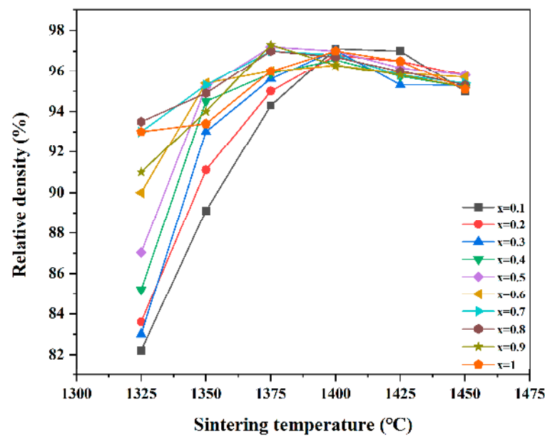
Figure 3. Relative density of Ba[(Zn x Co 1-x ) 1/3 (Nb 0.5 Ta 0.5 ) 2/3 ]O 3 ceramics sintered at different temperatures.
