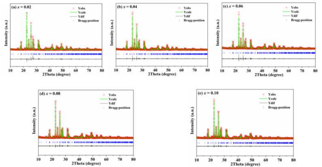
Figure 2. Rietveld refinement of CZ_{1-x}N_x ceramics at the optimal sintering temperature with different x values.
