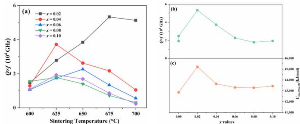
Figure 8. \text{CZ}_{1-x}\text{N}_x ceramics (a) Q \times f at a sintering temperature of 600 °C to 700 °C, (b) Q \times f , and (c) U_{ave.(\text{Mo-O})} at the optimal sintering temperature as a function of x values.
