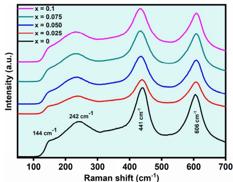
Figure 2. Raman spectra of rutile \text{Ti}_{1-x}\text{Zr}_x\text{O}_2 ( x = 0\text{--}0.1 ).
