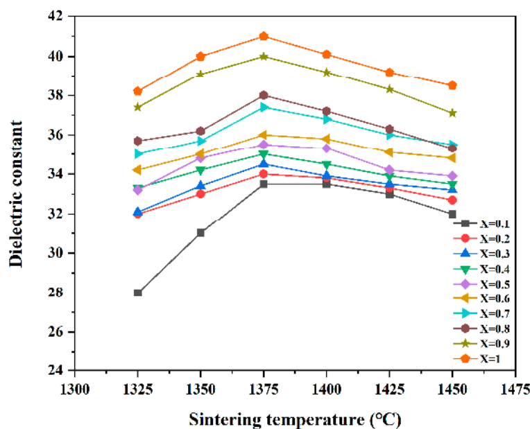
Figure 4. \epsilon_r values of Ba[(Zn x Co 1-x ) 1/3 (Nb 0.5 Ta 0.5 ) 2/3 ]O 3 ceramics sintered at different temperatures.
