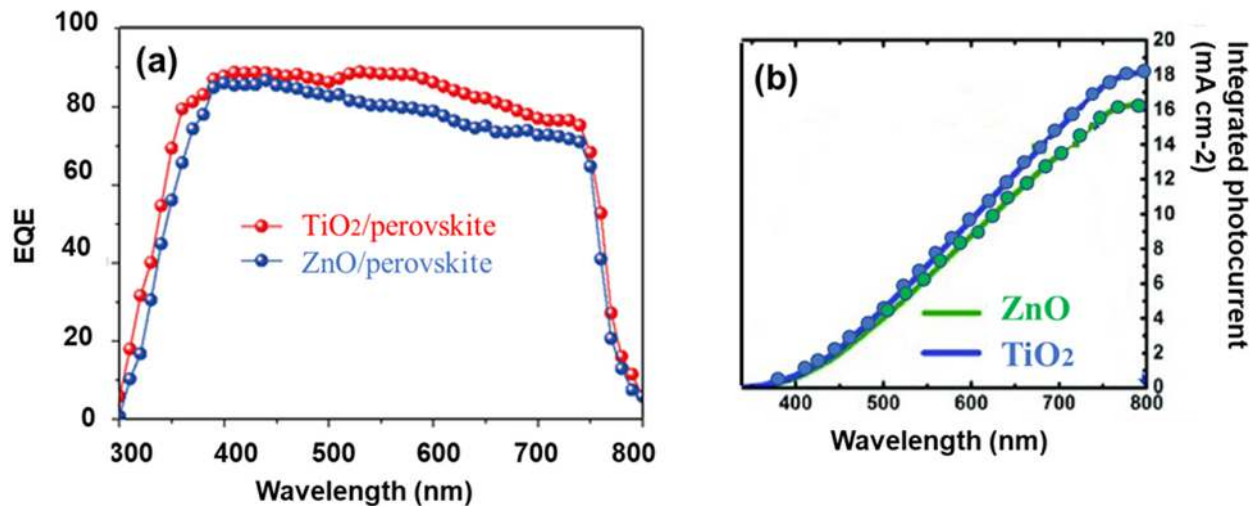
Figure 7. (a) EQE spectra for TiO 2 , ZnO photoanodes; (b) integral current density for TiO 2 and ZnO photoanodes.
