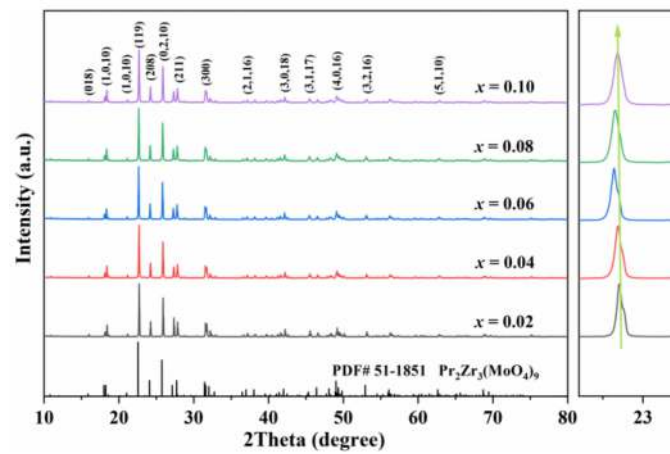
Figure 1. XRD patterns of CZ_{1-x}N_x ceramics sintered at the optimal temperature with different x values.
