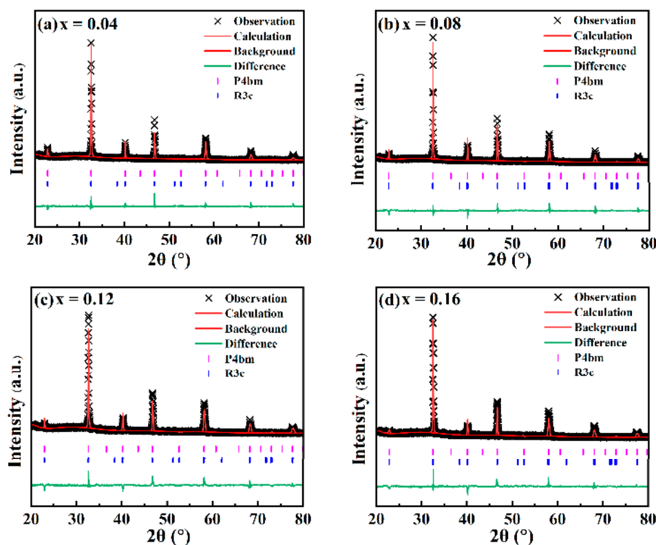
Figure 2. Rietveld Refined XRD Patterns of \text{NBT-xCaHfO}_3 ceramics: (a) x = 0.4 , (b) x = 0.08 , (c) x = 0.12 , and (d) x = 0.16 .
