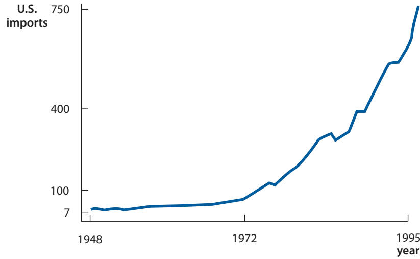
Figure 10.3 Nominal U.S. imports during the years 1948–1995 (in billions of U.S. dollars).
