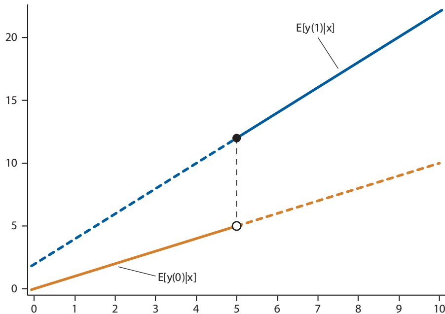
Figure 19.2 A Sharp RD Design with Linear Conditional Means.
