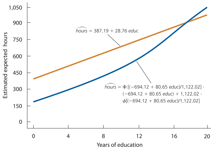
Figure 17.3 Estimated expected values of hours with respect to education for the linear and Tobit models.
