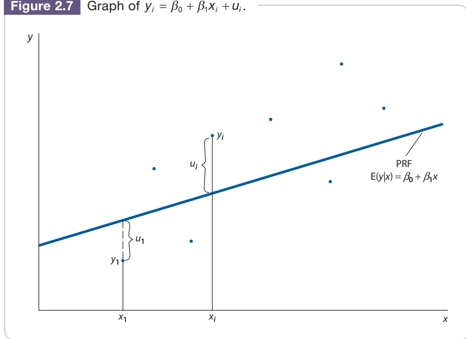
Figure 2.7 Graph of y_i = \beta_0 + \beta_1 x_i + u_i .
