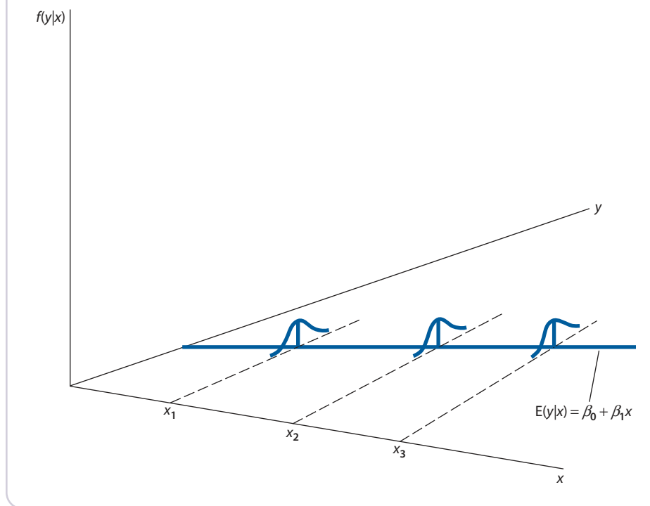
Figure 2.8 The simple regression model under homoskedasticity.
