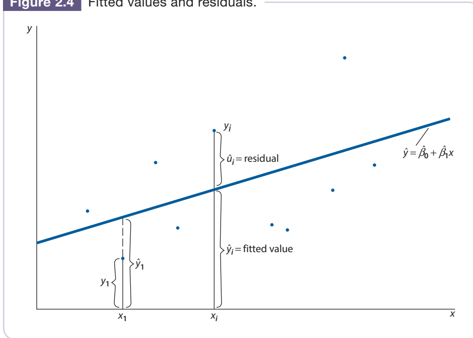
Figure 2.4 Fitted values and residuals.
