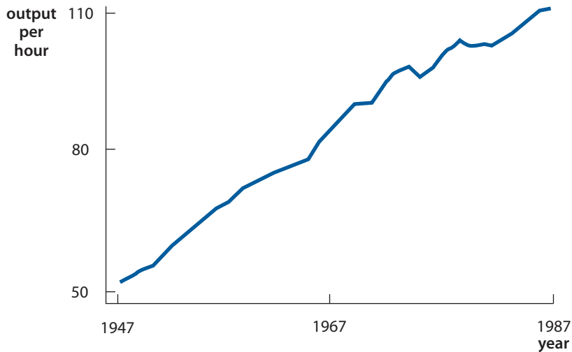
Figure 10.2 Output per labor hour in the United States during the years 1947–1987; 1977 = 100.
