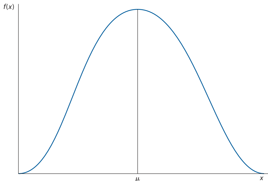
Figure B.3 A symmetric probability distribution.
