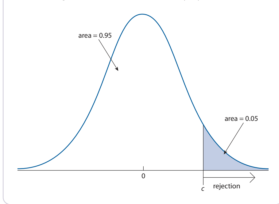
Figure C.5 Rejection region for a 5% significance level test against the one-sided alternative \mu > \mu_0 .
