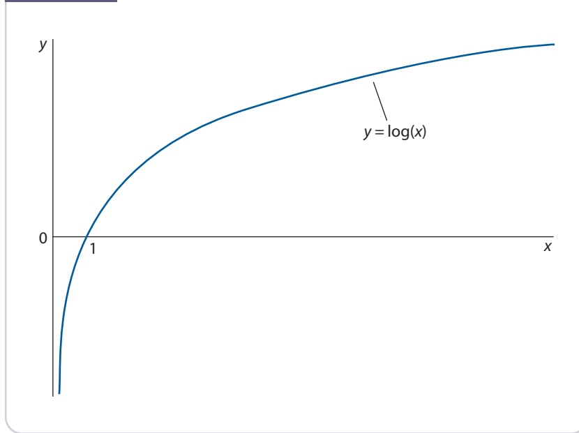
Figure A.4 Graph of y = \log(x) .
