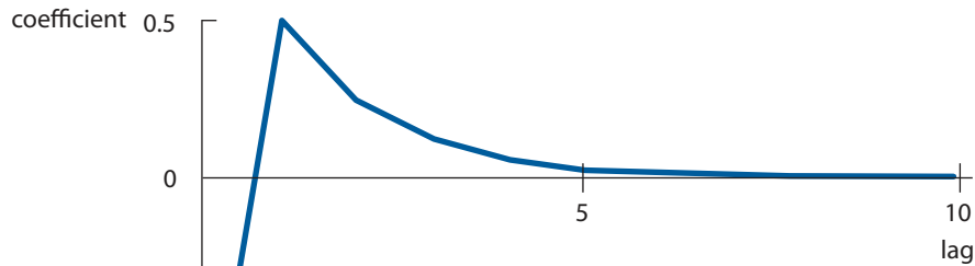
Figure 18.1 Lag distribution for the rational distributed lag (18.16) with \rho = 0.5 , \gamma_0 = -1 , and \gamma_1 = 1 .
