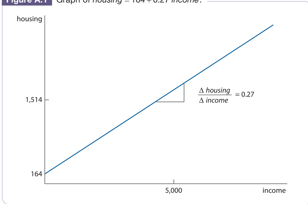
Figure A.1 Graph of \text{housing} = 164 + 0.27 \text{ income} .
