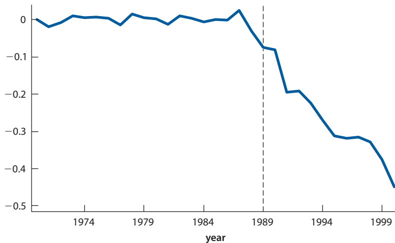
Figure 18.5 Detrended d\bar{y}_t using pre-intervention data and midwestern control states
