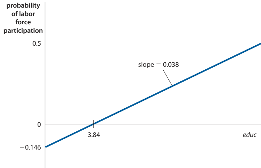
Figure 7.3 Estimated relationship between the probability of being in the labor force and years of education, with other explanatory variables fixed.
