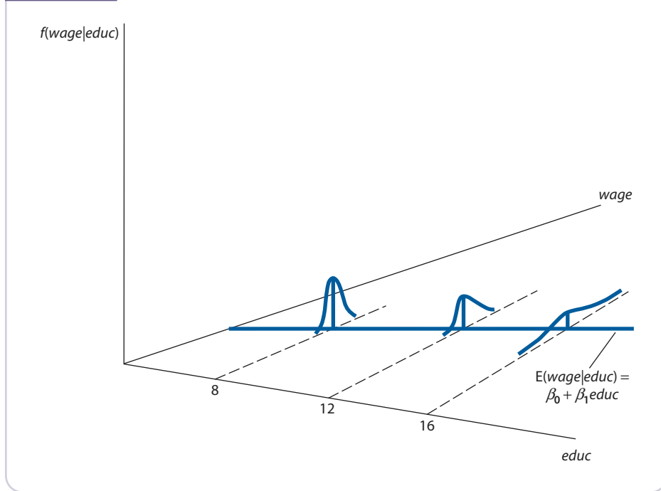
Figure 2.9 \text{Var}(\text{wage}|\text{educ}) increasing with \text{educ} .
