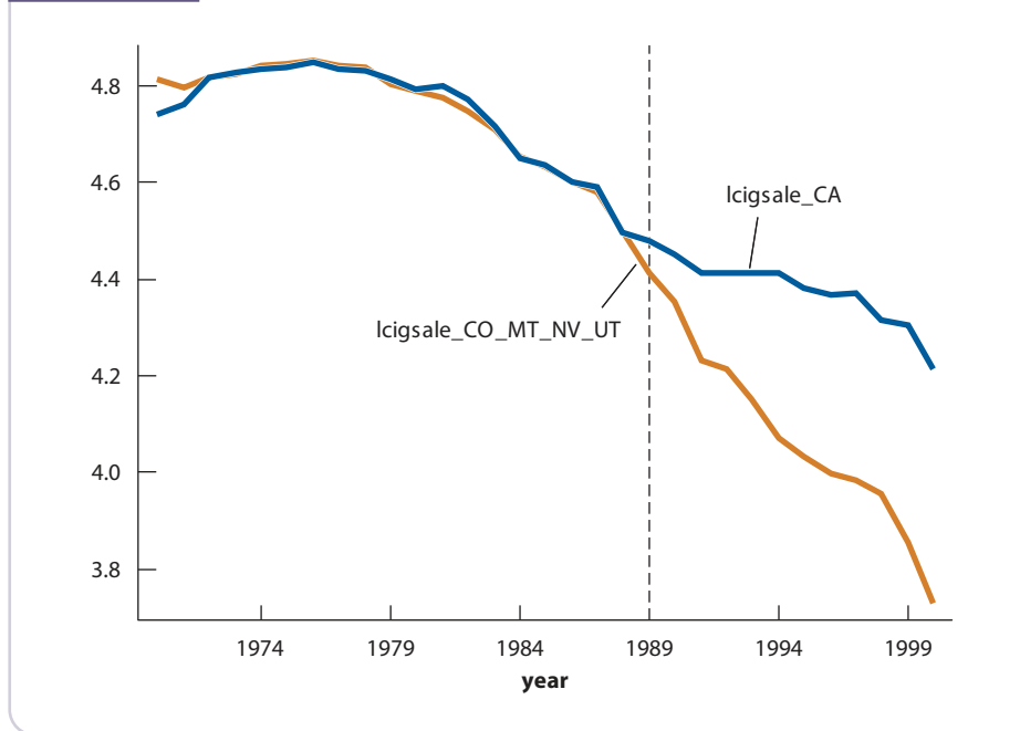
Figure 18.3 Using CO, MT, NV, and UT as Controls for CA
