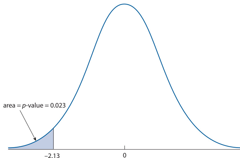
Figure C.8 The p -value when t = -2.13 with 19 degrees of freedom for the one-sided alternative \mu < 0 .
