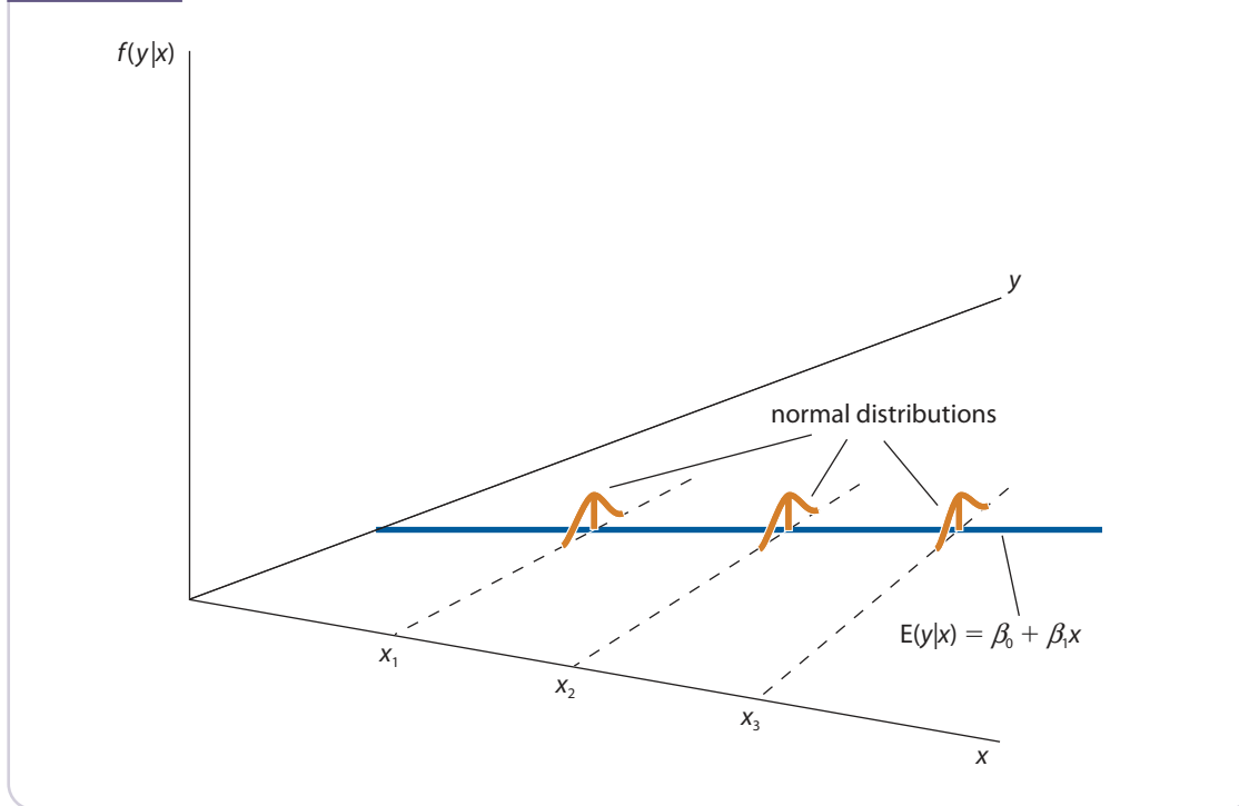
Figure 4.1 The homoskedastic normal distribution with a single explanatory variable.
