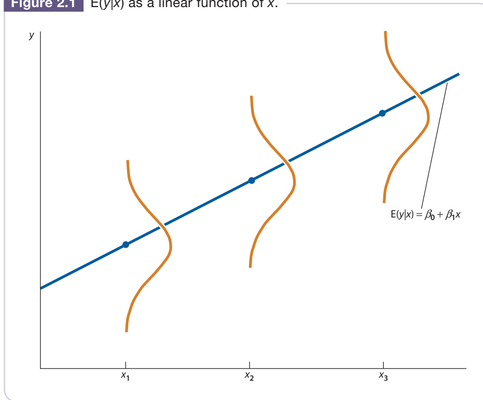
Figure 2.1 E(y|x) as a linear function of x .
