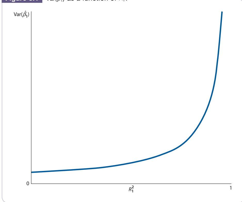
Figure 3.1 \text{Var}(\hat{\beta}_1) as a function of R_1^2 .
