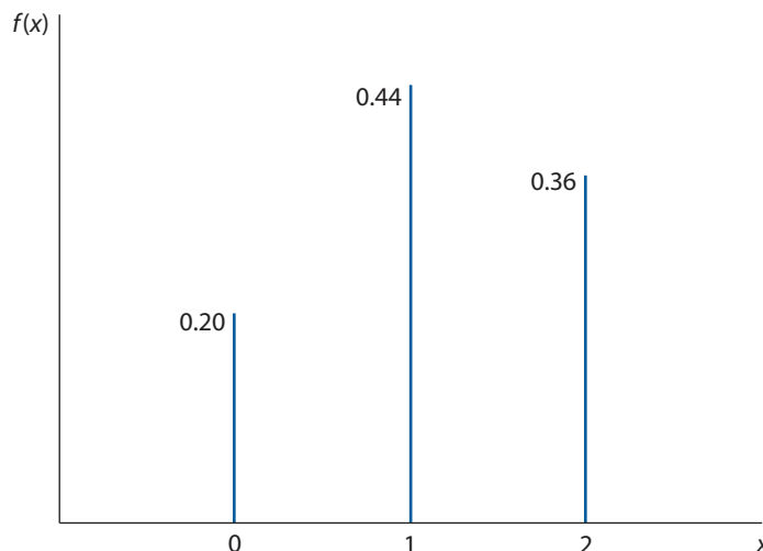
Figure B.1 The pdf of the number of free throws made out of two attempts.
