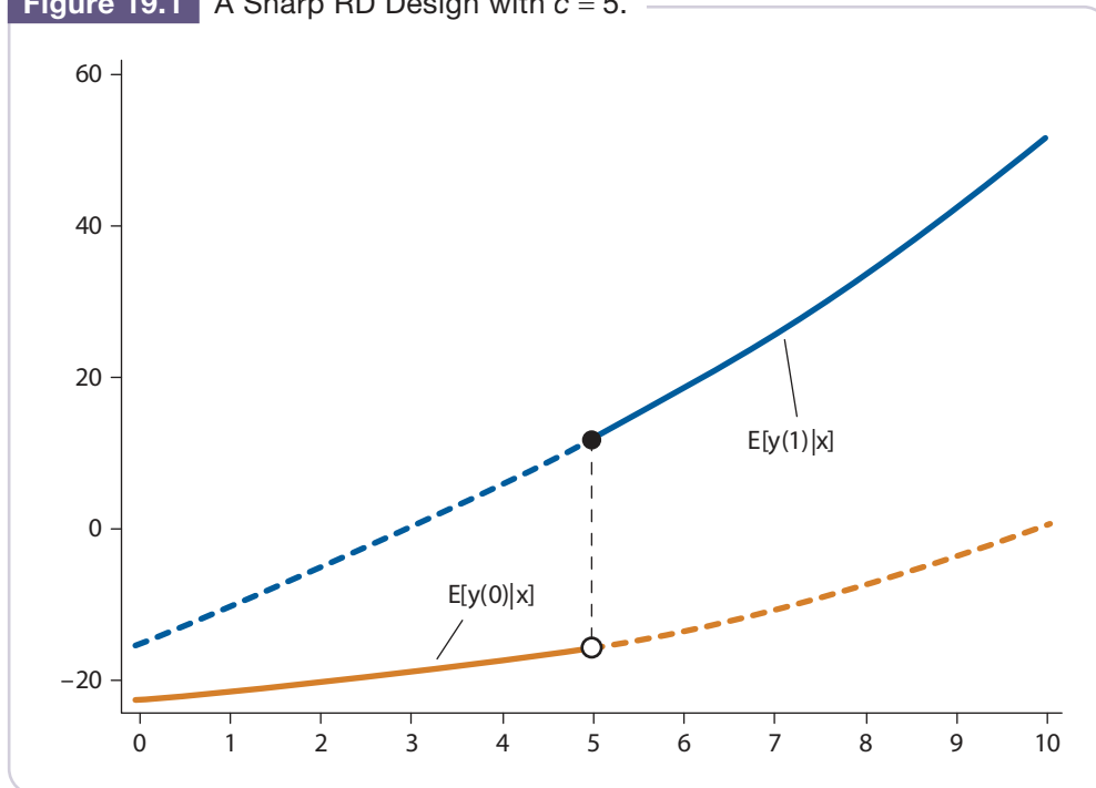
Figure 19.1 A Sharp RD Design with c = 5 .
