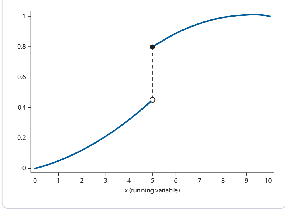
Figure 19.4 Probability of Treatment in a Fuzzy RD Design.
