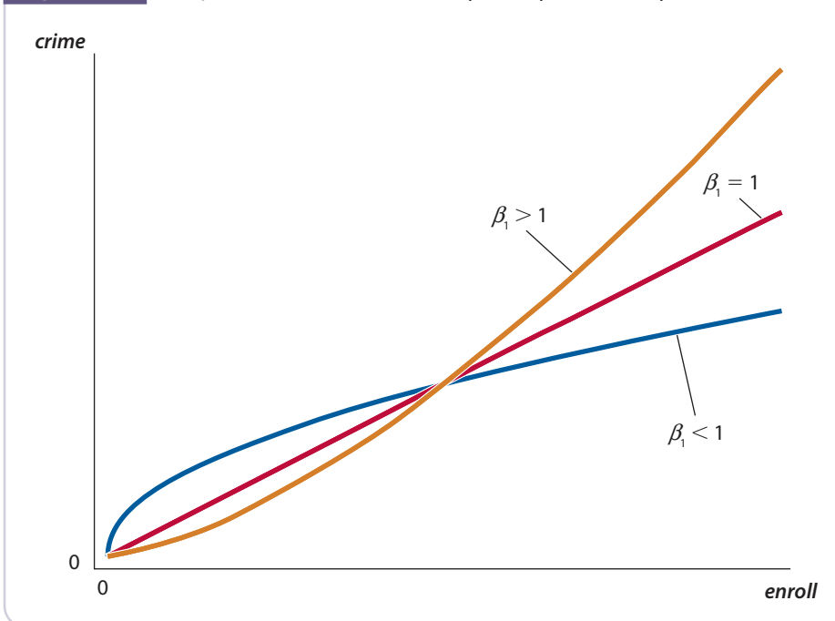
Figure 4.5 Graph of \text{crime} = \text{enroll}^{\beta_1} for \beta_1 < 1 , \beta_1 = 1 , and \beta_1 > 1 .
