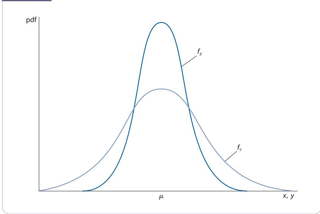
Figure B.4 Random variables with the same mean but different distributions.
