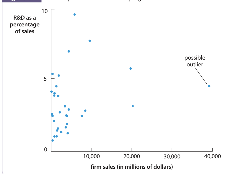
Figure 9.1 Scatterplot of R&D intensity against firm sales.
