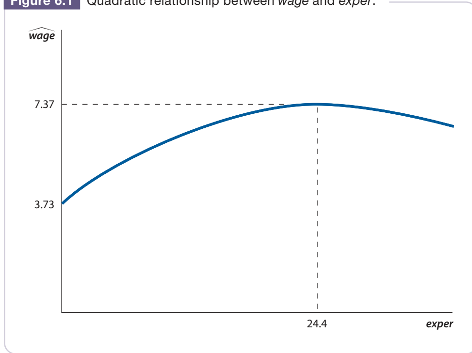
Figure 6.1 Quadratic relationship between \widehat{wage} and exper .
