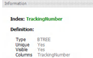
Figure 19.3 Information about the TrackingNumber index of the shipment table, viewed in MySQL Workbench
