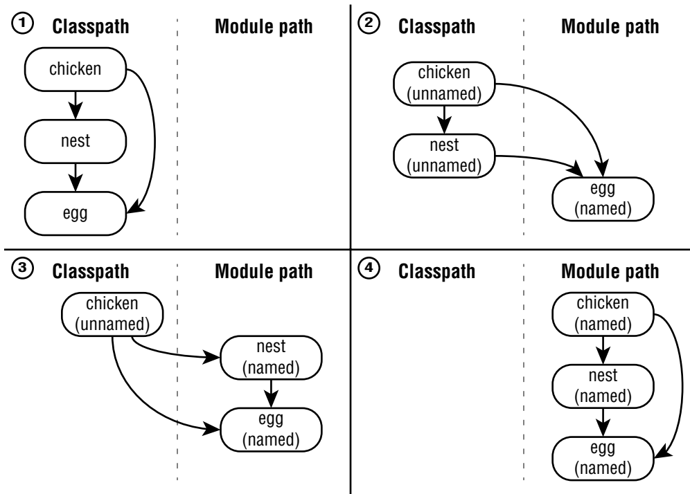
FIGURE 12.16 Bottom-up migration
