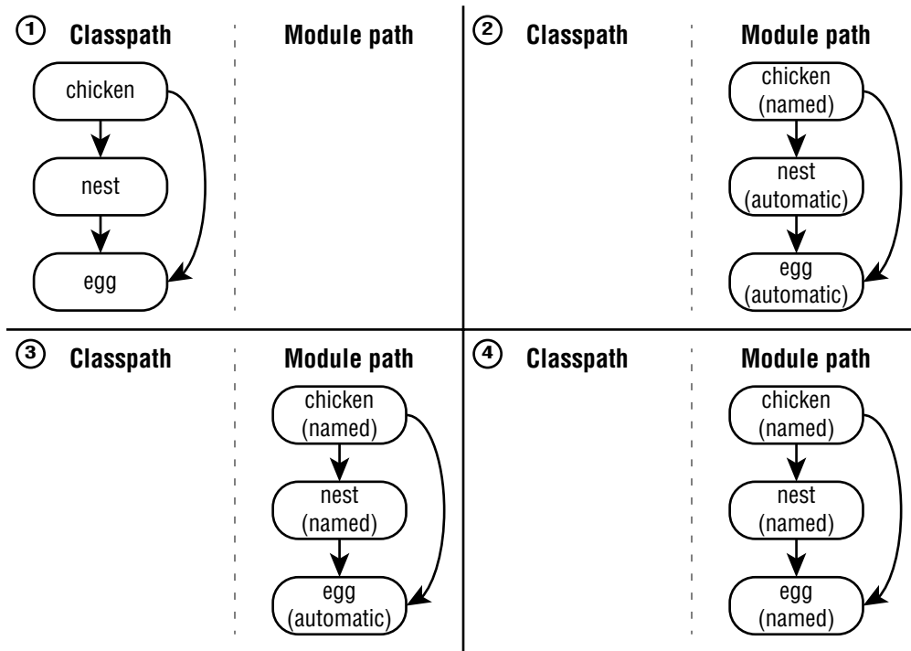
FIGURE 12.17 Top-down migration
