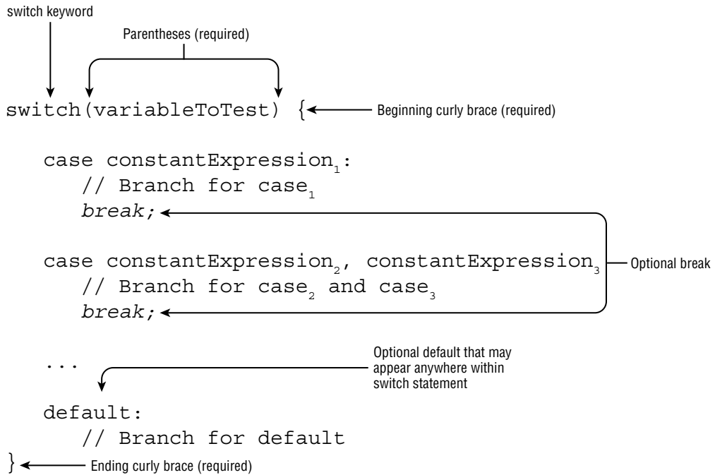
FIGURE 3.3 The structure of a switch statement
