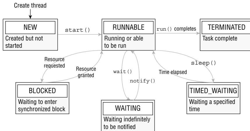
FIGURE 13.2 Thread states
