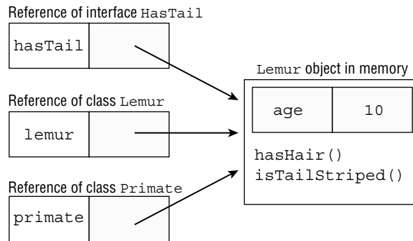
FIGURE 7.8 Object vs. reference
