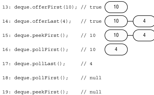
FIGURE 9.6 Working with a Deque
