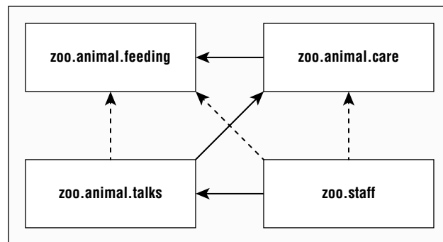
FIGURE 12.12 Transitive dependency version of our modules
