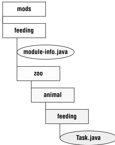
FIGURE 12.4 Module zoo.animal.feeding directory structure
