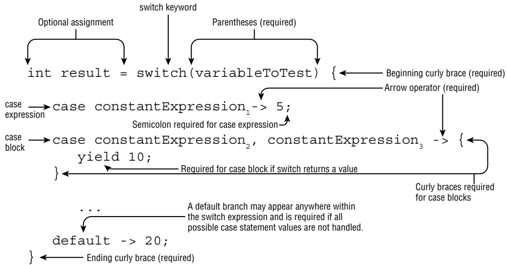
FIGURE 3.4 The structure of a switch expression
