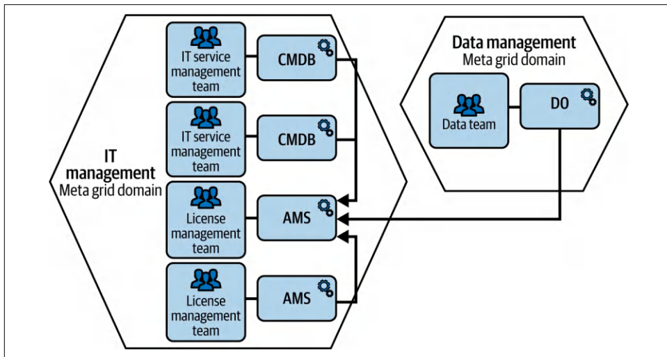
Figure 11-2. FinOps architecture
