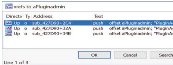
Figure 11.20: String cross-references in IDA
