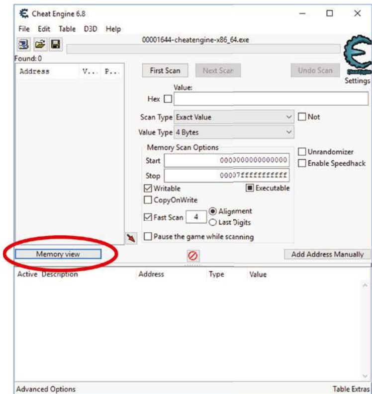
Figure 11.10: Viewing memory in Cheat Engine
