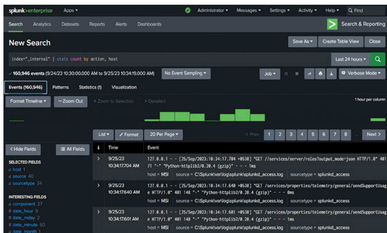
Figure 1.2: Splunk Search
