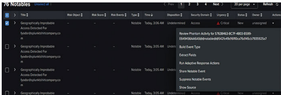
Figure 6.6: Notable events
