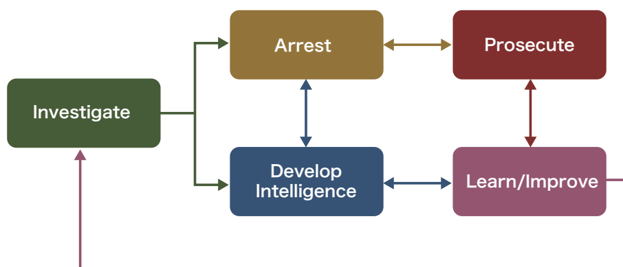
Figure 8-6. Procedural Remediation
