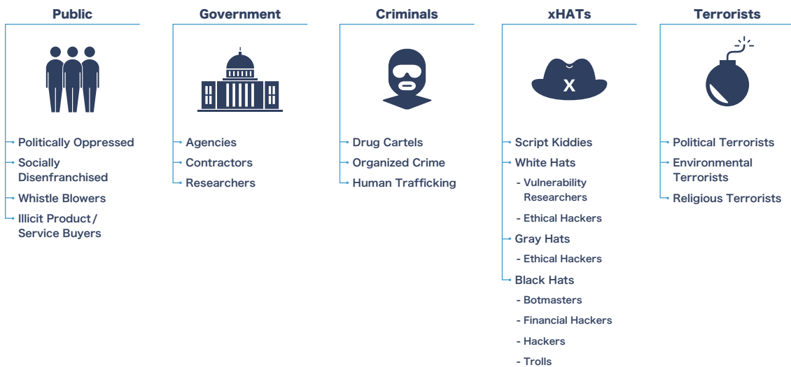
Figure 4-5. Darknet Profiles
