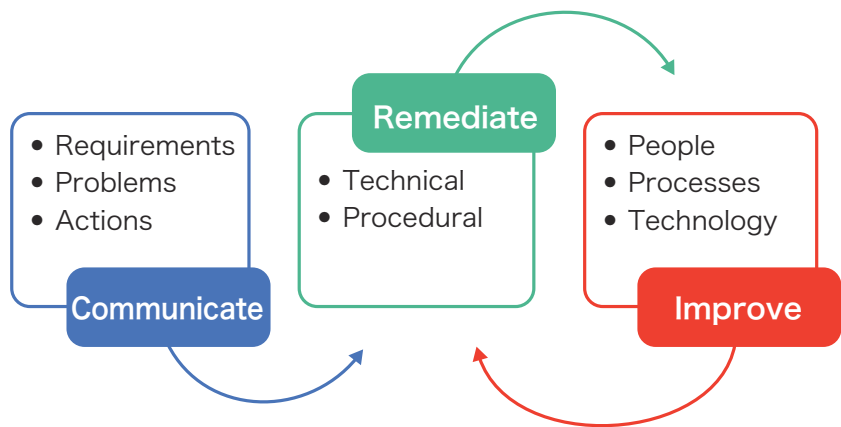
Figure 8-11. Improving Resolution
