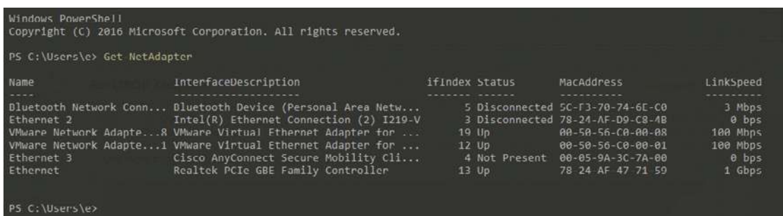
Figure 6-14. Windows POWERSHELL Get-NetAdapter
