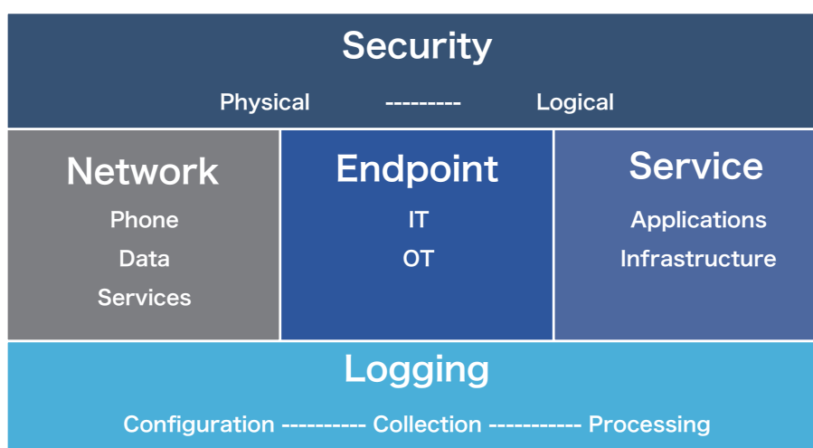
Figure 6-39. Logging
