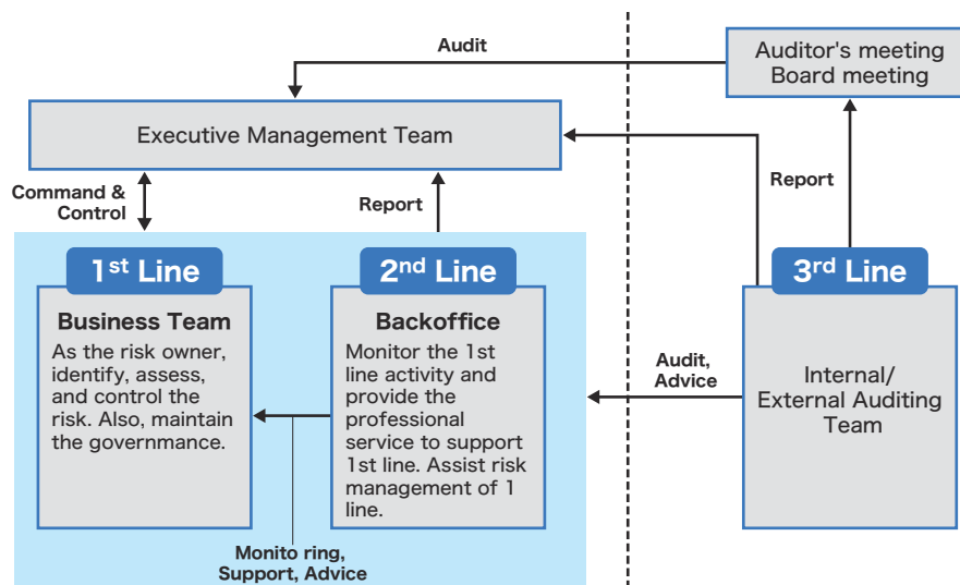
Figure 10-12. Three-line Model
