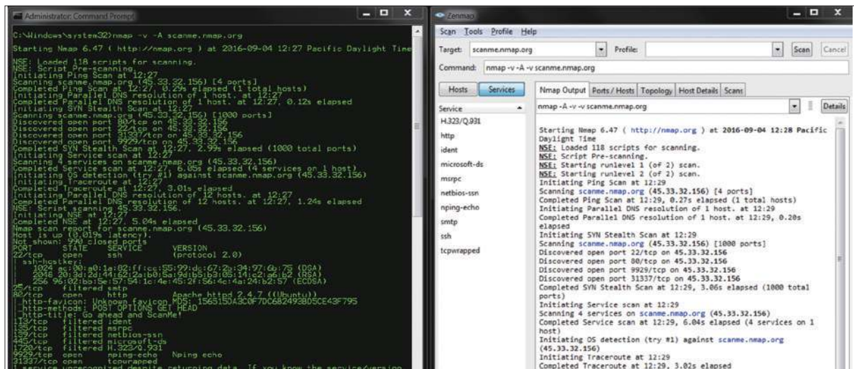
Figure 6-31. NMAP
