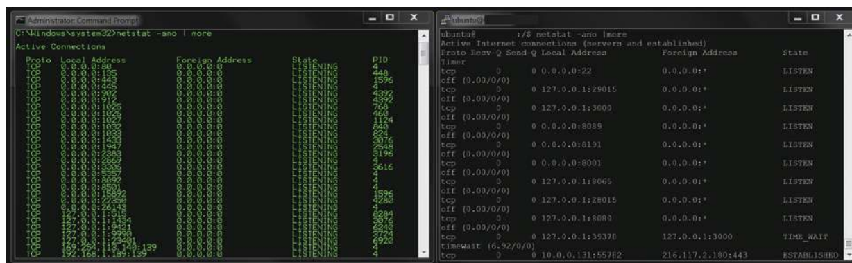
Figure 6-15. Windows and Linux netstat -ano
