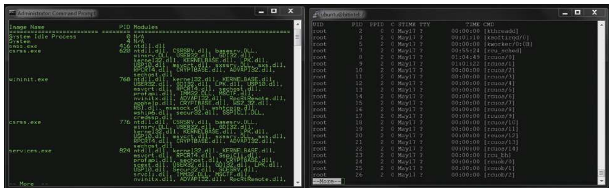
Figure 6-16. Windows TASKLIST /M and Linux ps -df
