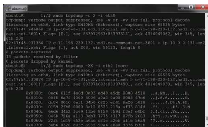
Figure 6-18. Linux tcpdump
