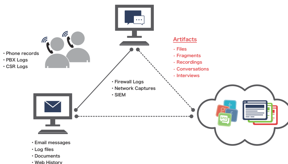
Figure 3-8. Internal Artifacts
