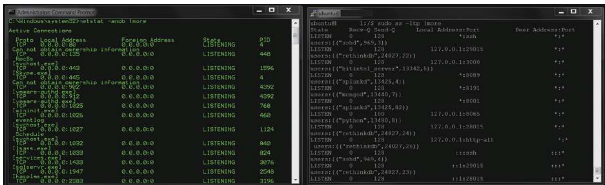
Figure 6-17. Windows NETSTAT -ANOB and Linux ss -ltip
